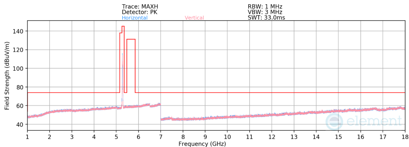
Plot 7-718. RSE above 1GHz Antenna 2a (11ax – Ch.56 – RU52)
