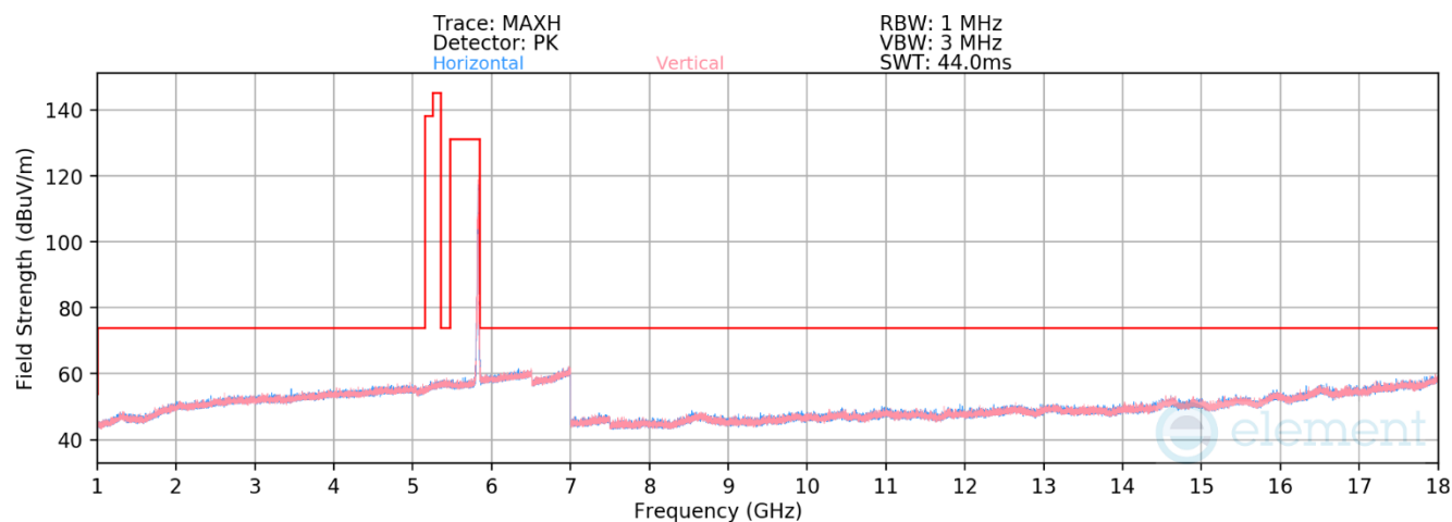
Plot 7-701. RSE above 1GHz Antenna 4a (11ax – Ch.165 – RU26)
