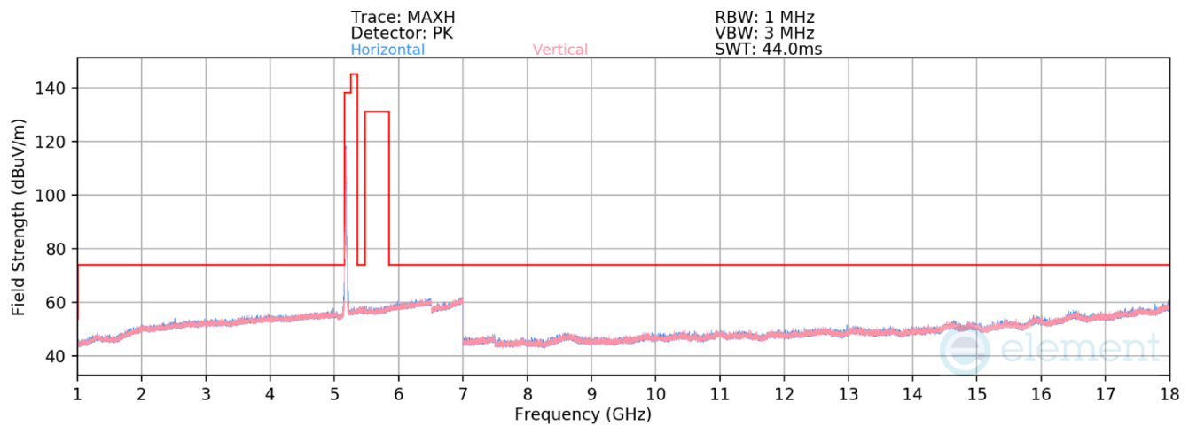
Plot 7-714. RSE above 1GHz Antenna 2a (11ax – Ch.36 – RU26)
