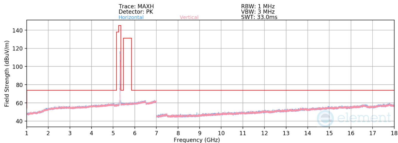
Plot 7-719. RSE above 1GHz Antenna 2a (11ax – Ch.64 – RU52)
