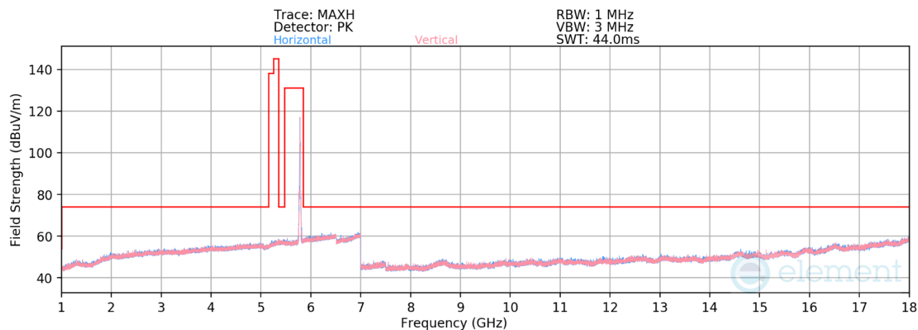
Plot 7-724. RSE above 1GHz Antenna 2a (11ax – Ch.157 – RU26)
