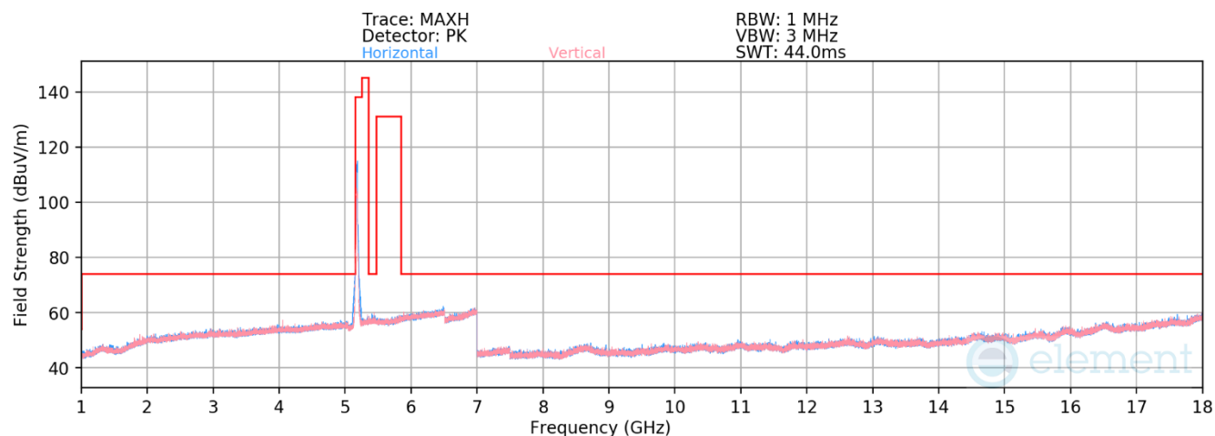
Plot 7-678. RSE above 1GHz Antenna WF5B (11ax – Ch.36 – RU242)
