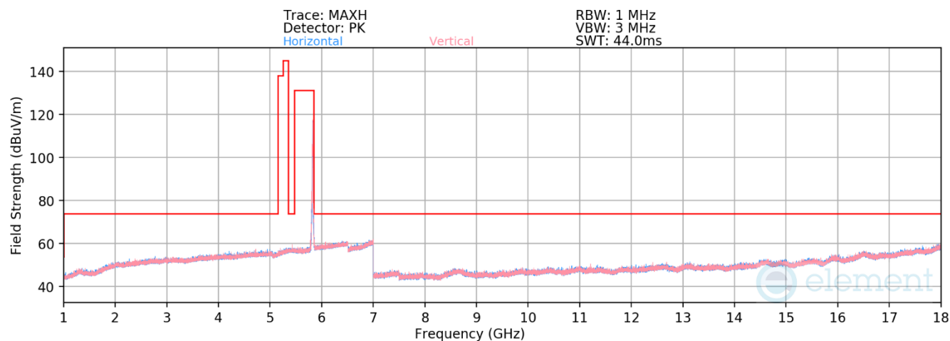
Plot 7-725. RSE above 1GHz Antenna 2a (11ax – Ch.165 – RU26)
