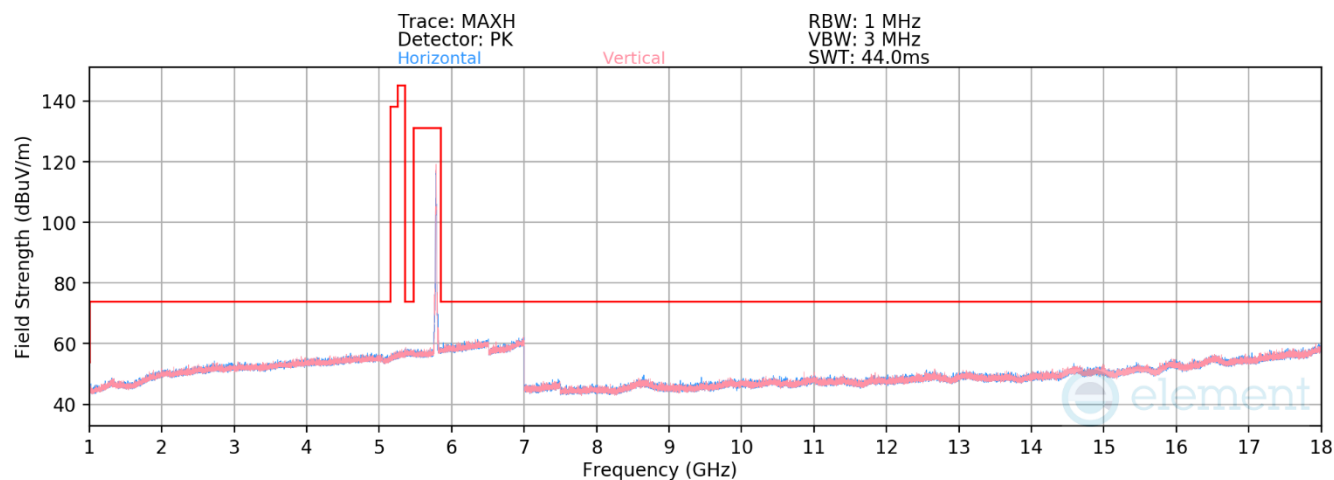
Plot 7-700. RSE above 1GHz Antenna 4a (11ax – Ch.157 – RU26)
