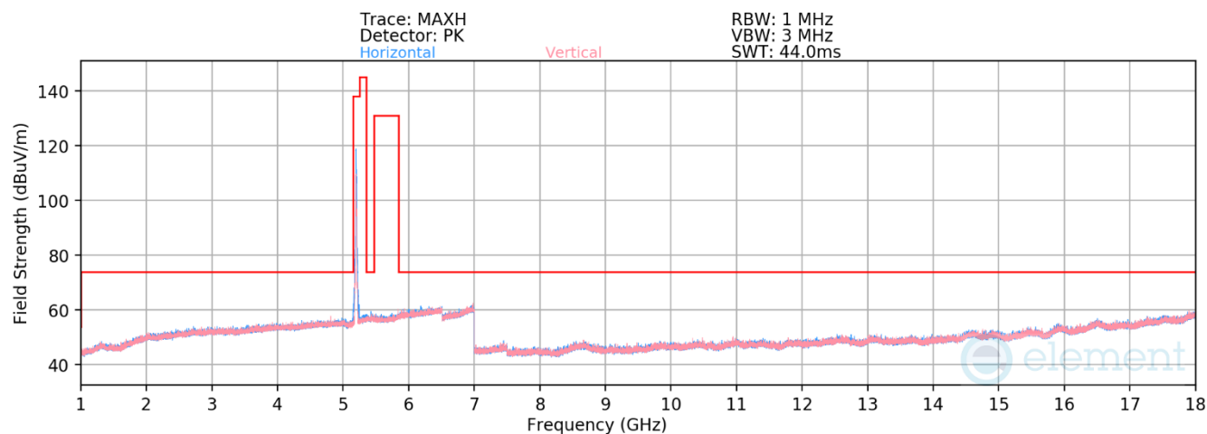
Plot 7-667. RSE above 1GHz Antenna WF5B (11ax – Ch.40 – RU26)
