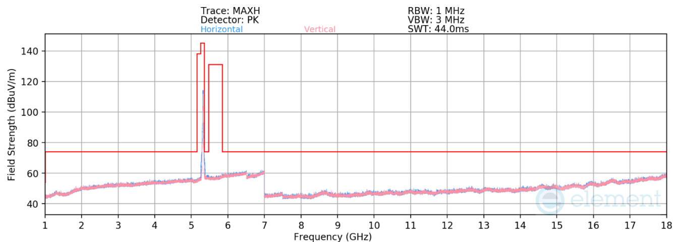
Plot 7-683. RSE above 1GHz Antenna WF5B (11ax – Ch.64 – RU242)
