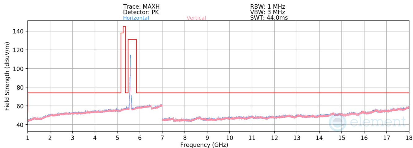
Plot 7-685. RSE above 1GHz Antenna WF5B (11ax – Ch.116 – RU242)
