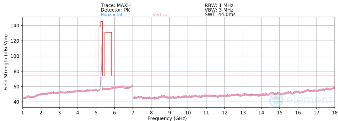
Plot 7-759. RSE above 1GHz CDD Primary (11ax – Ch.56 – RU242)
