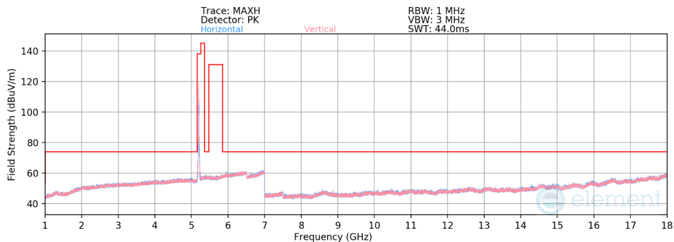
Plot 7-771. RSE above 1GHz CDD Diversity (11ax - Ch.40 - RU26)
