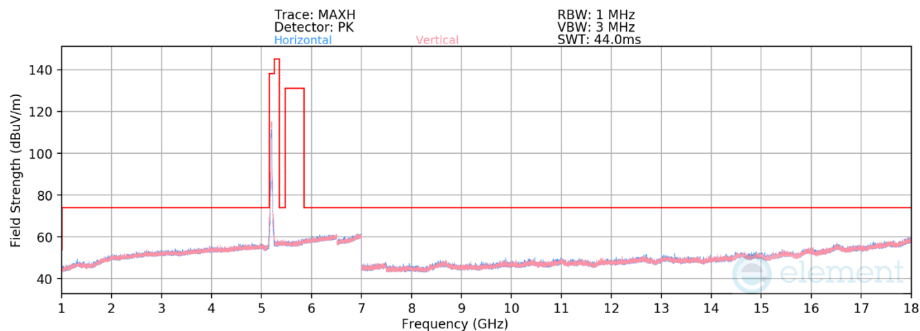
Plot 7-755. RSE above 1GHz CDD Primary (11ax – Ch.40 – RU242)
