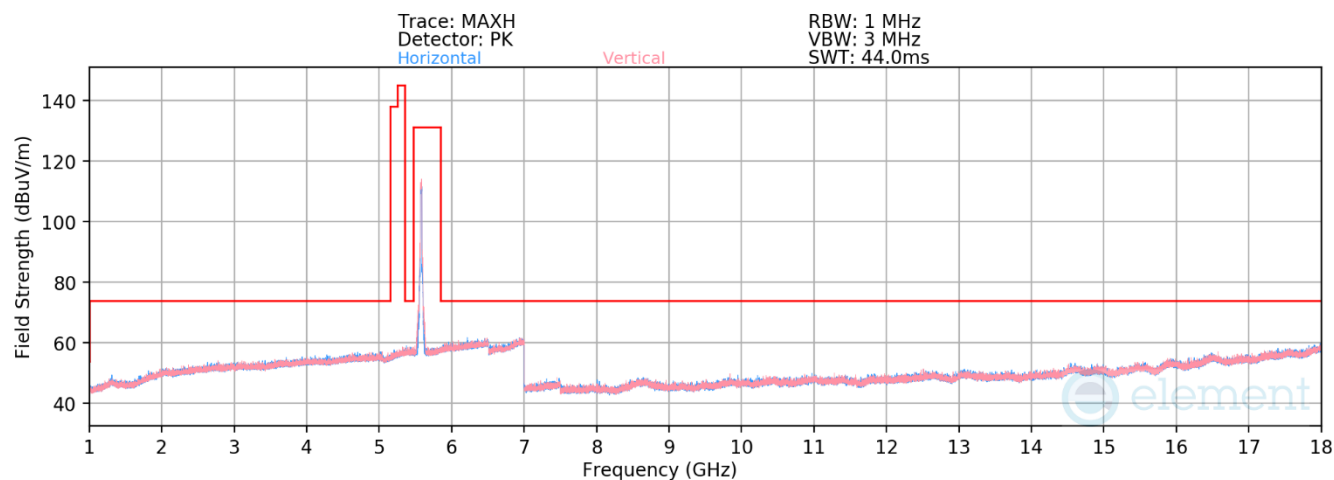
Plot 7-763. RSE above 1GHz CDD Primary (11ax – Ch.116 – RU242)
