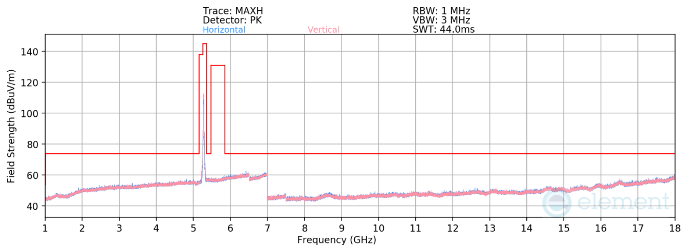
Plot 7-791. RSE above 1GHz CDD Diversity (11ax - Ch.56 - RU242)
