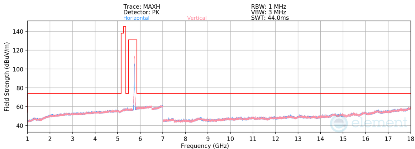
Plot 7-798. RSE above 1GHz CDD Diversity (11ax – Ch.149 – RU242)
