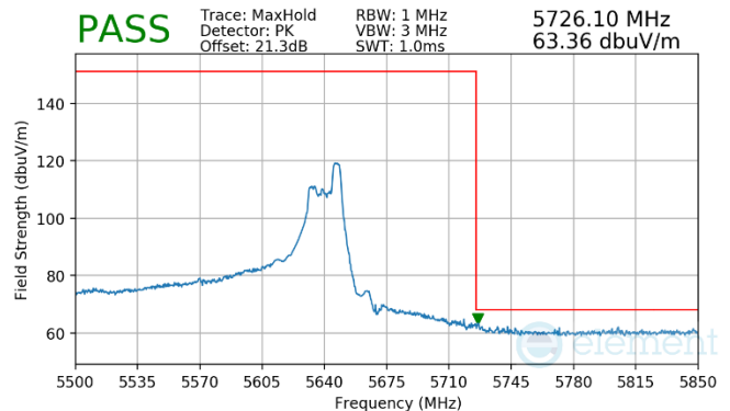
Plot 7-854. (FCC Only) Antenna WF5B (Pk, RU52, Index 37, Ch.114 (U), MCS11)
