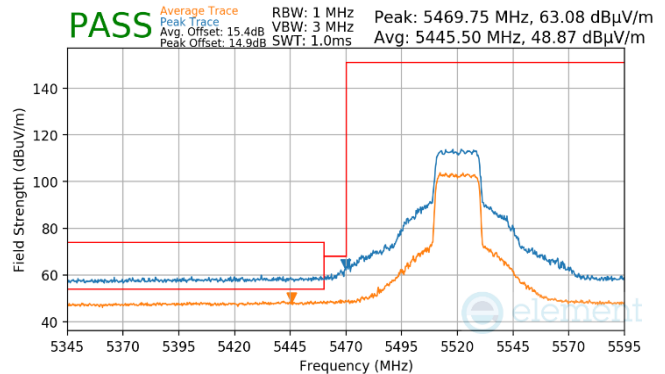
Plot 7-984. CDD Primary (Pk & Avg, RU242, Index 61, Ch.104, MCS11)
