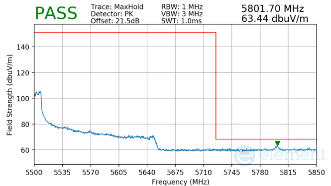
Plot 7-1022. (FCC Only) CDD Primary (Pk, RU52, Index 37, Ch.114 (U), MCS11)
