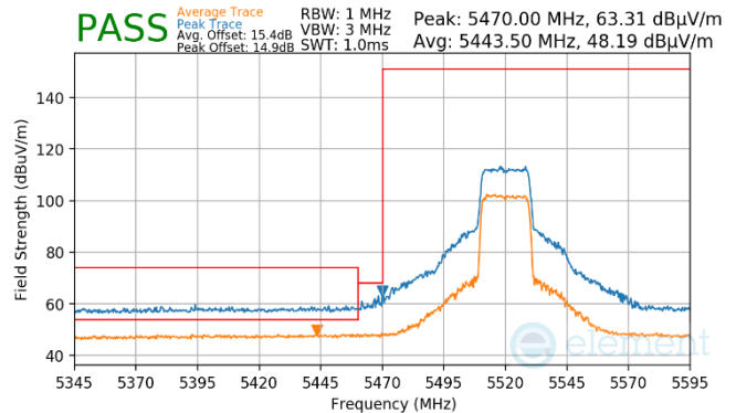
Plot 7-1038. CDD Diversity (Pk & Avg, RU242, Index 61, Ch.104, MCS11)
