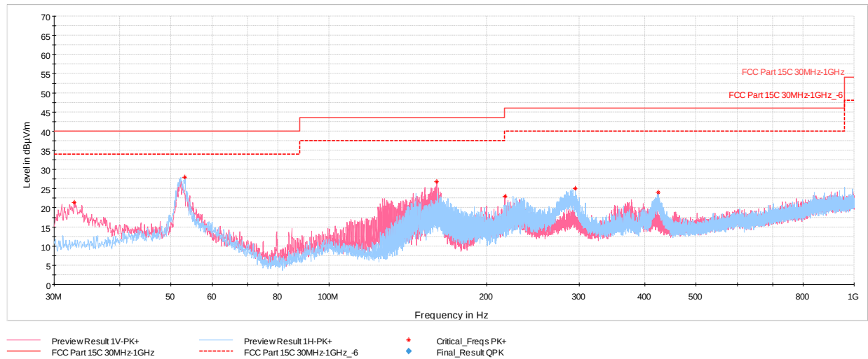
Plot 7-1081. RSE below 1GHz CDD Primary (RU26 – Ch.40), with Laptop
