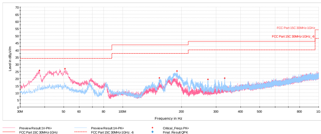
Plot 7-1084. RSE below 1GHz CDD Diversity (RU242 – Ch.40), with AC/DC Adapter
