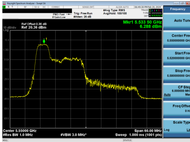
Plot 7-201. PSD Antenna WFSB (40MHz BW 11ax Index 37 - RU52 - Ch.110)
