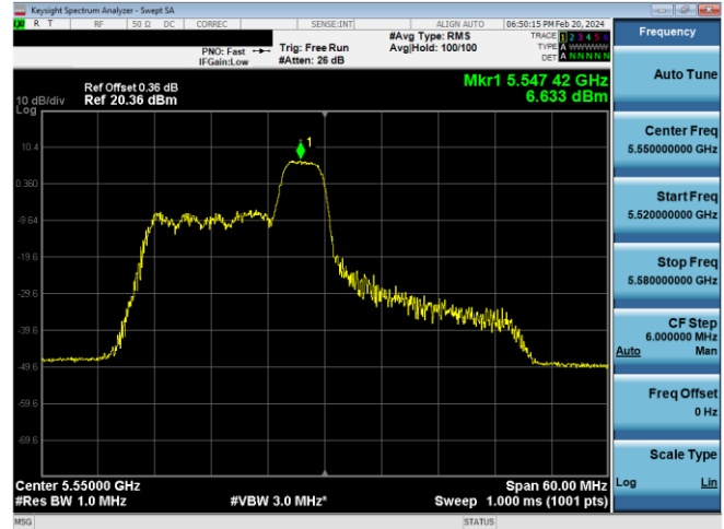
Plot 7-202. PSD Antenna WFSB (40MHz BW 11ax Index 40 - RU52 - Ch.110)
