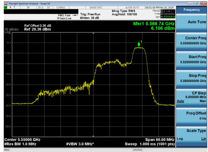
Plot 7-203. PSD Antenna WFSB (40MHz BW 11ax Index 44 - RU52 - Ch.110)
