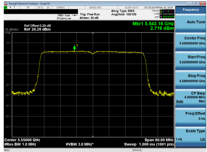
Plot 7-204. PSD Antenna WFSB (40MHz BW 11ax - RU484 - Ch.110)
