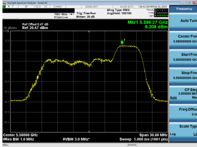
Plot 7-199. PSD Antenna WFSB (20MHz BW 11ax Index 40 - RU52 - Ch.116)
