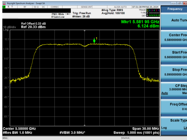
Plot 7-200. PSD Antenna WFSB (20MHz BW 11ax - RU242 - Ch.116)
