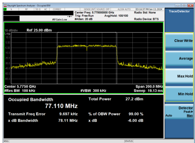
Plot 7-156. 6dB BW & 99% OBW Antenna 4a (80MHz BW 11ax – RU996 – Ch.155)
