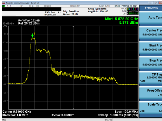
Plot 7-205. PSD Antenna WFSB (80MHz BW 11ax Index 37 - RU52 - Ch.122)
