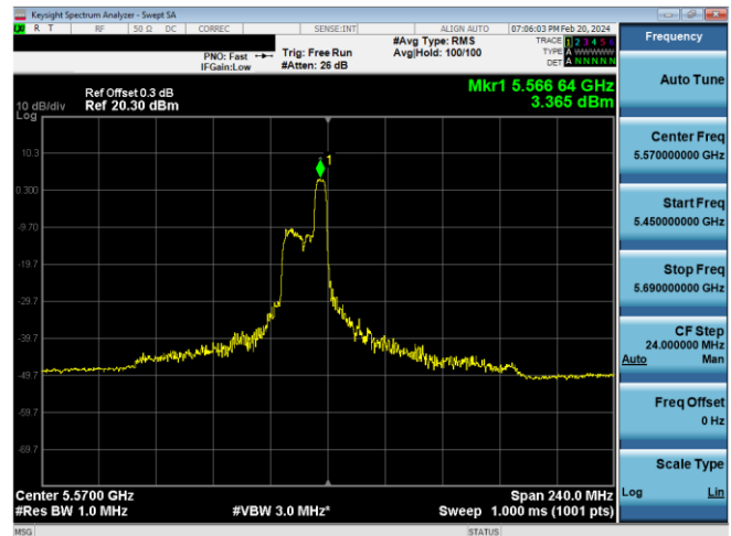
Plot 7-210. PSD Antenna WFSB (160MHz BW 11ax Index 52 - RU52 - Ch.114 (L))
