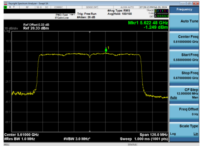
Plot 7-208. PSD Antenna WFSB (80MHz BW 11ax - RU996 - Ch.122)
