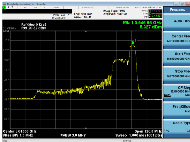
Plot 7-207. PSD Antenna WFSB (80MHz BW 11ax Index 52 - RU52 - Ch.122)
