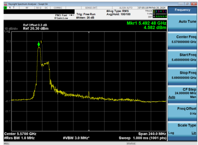
Plot 7-209. PSD Antenna WFSB (160MHz BW 11ax Index 37 - RU52 - Ch.114 (L))
