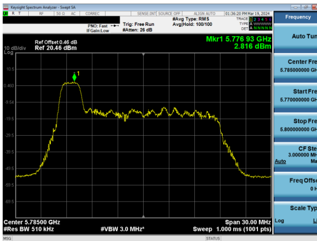
Plot 7-471. PSD CDD Primary Antenna 4a (20MHz BW 11ax Index 0 - RU26 - Ch.157)
