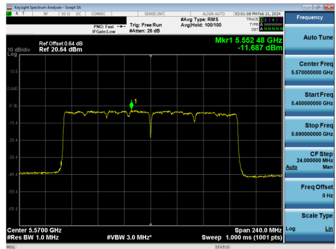
Plot 7-469. PSD CDD Primary Antenna 4a (160MHz BW 11ax - RU996x2 - Ch.114)
