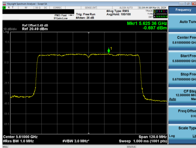
Plot 7-461. PSD CDD Primary Antenna 4a (80MHz BW 11ax - RU96 - Ch.122)
