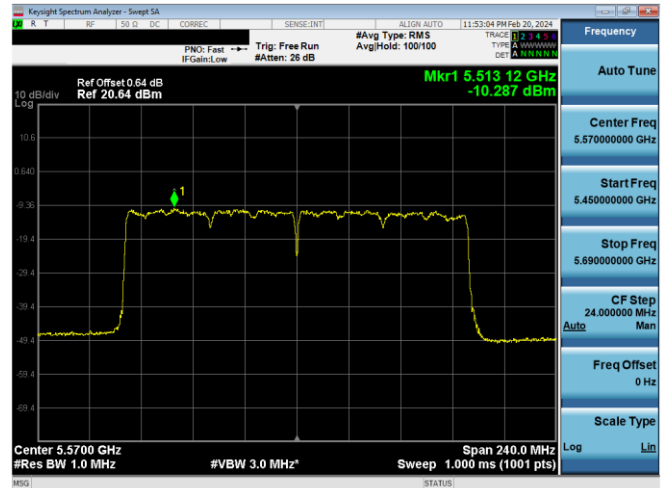
Plot 7-468. PSD CDD Primary Antenna WF5B (160MHz BW 11ax - RU996x2 - Ch.114)
