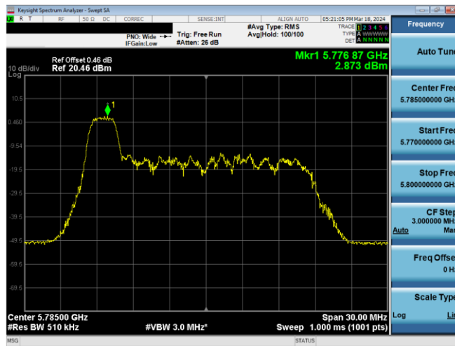
Plot 7-470. PSD CDD Primary Antenna WF5B (20MHz BW 11ax Index 0 - RU26 - Ch.157)
