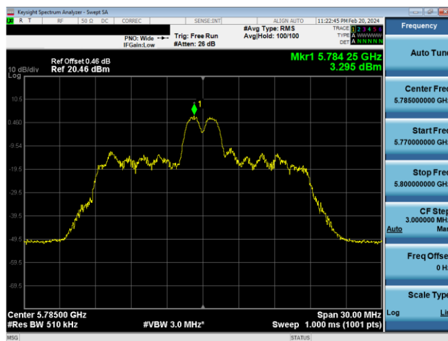
Plot 7-472. PSD CDD Primary Antenna WF5B (20MHz BW 11ax Index 4 - RU26 - Ch.157)
