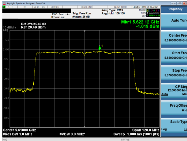
Plot 7-460. PSD CDD Primary Antenna WF5B (80MHz BW 11ax - RU96 - Ch.122)
