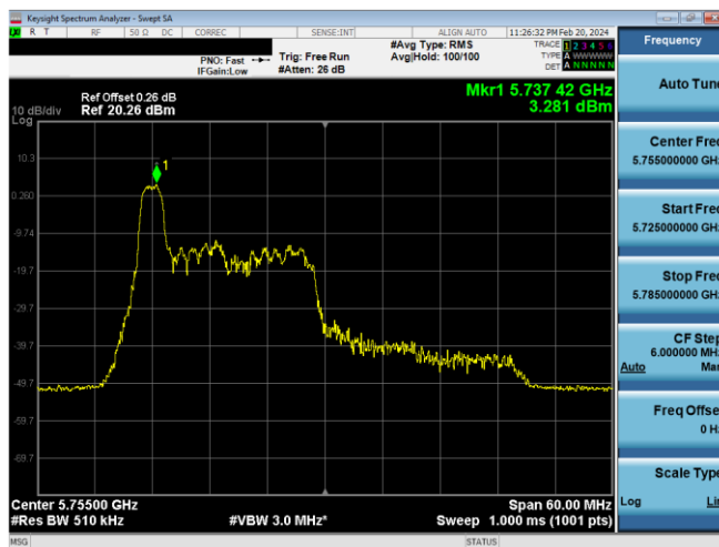
Plot 7-478. PSD CDD Primary Antenna WF5B (40MHz BW 11ax Index 0 - RU26 - Ch.151)
