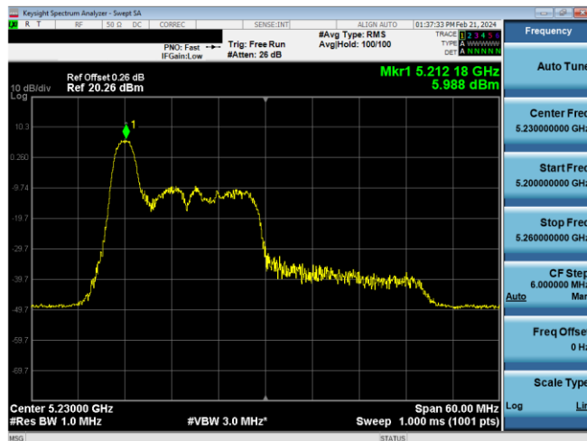
Plot 7-532. PSD CDD Diversity Antenna WFSB (40MHz BW 11ax Index 0 - RU26 - Ch.46)
