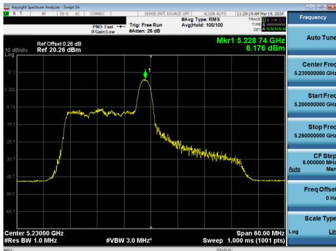
Plot 7-534. PSD CDD Diversity Antenna WFSB (40MHz BW 11ax Index 8 - RU26 - Ch.46)
