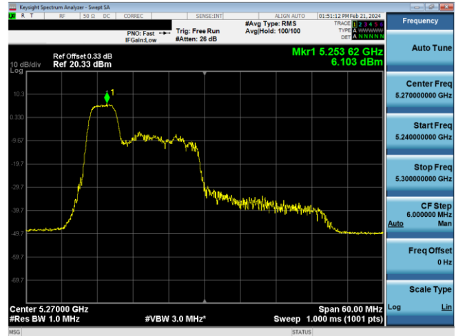
Plot 7-564. PSD CDD Diversity Antenna WF5B (40MHz BW 11ax Index 37 - RU52 - Ch.54)
