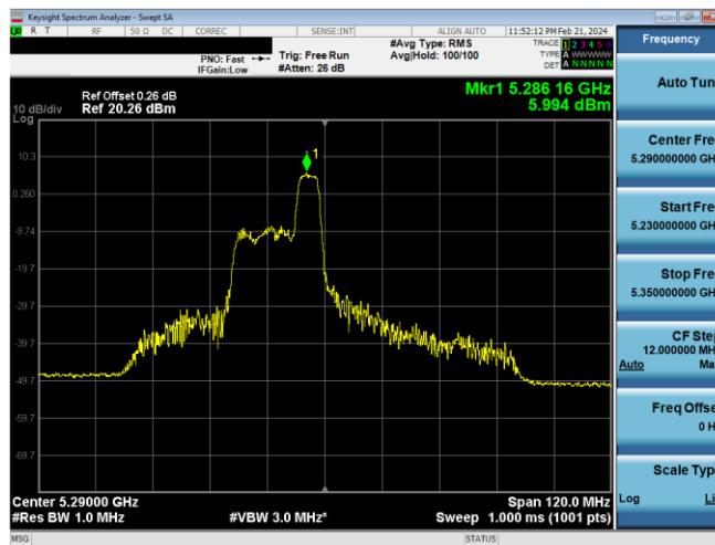
Plot 7-575. PSD Diversity CDD Antenna 2a (80MHz BW 11ax Index 44 - RU52 - Ch.58)
