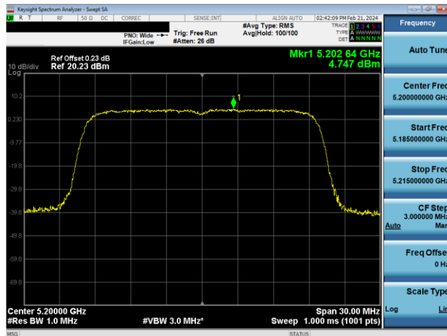
Plot 7-530. PSD CDD Diversity Antenna WFSB (20MHz BW 11ax- RU242 - Ch.40)
