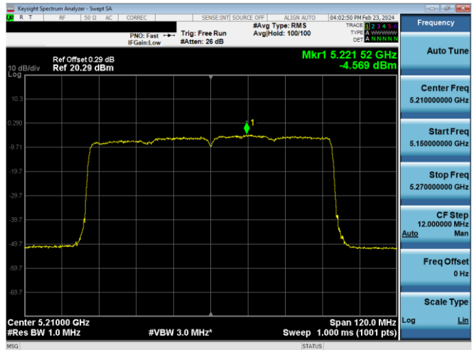
Plot 7-658. ISSED PSD CDD Diversity Antenna WF5B (80MHz BW 11ax - RU996 - Ch.42)
