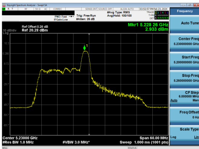
Plot 7-646. ISED PSD SDM Diversity Antenna WF5B (40MHz BW 11ax Index 8 - RU26 - Ch.46)
