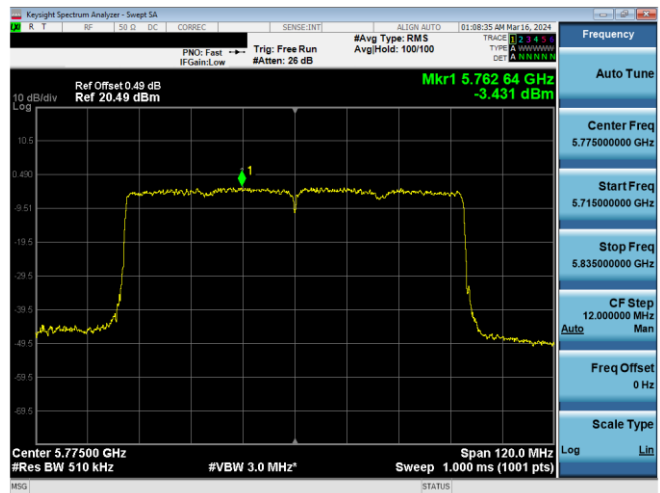
Plot 7-634. PSD CDD Diversity Antenna WF5B (80MHz BW 11ax - RU996 - Ch.155)
