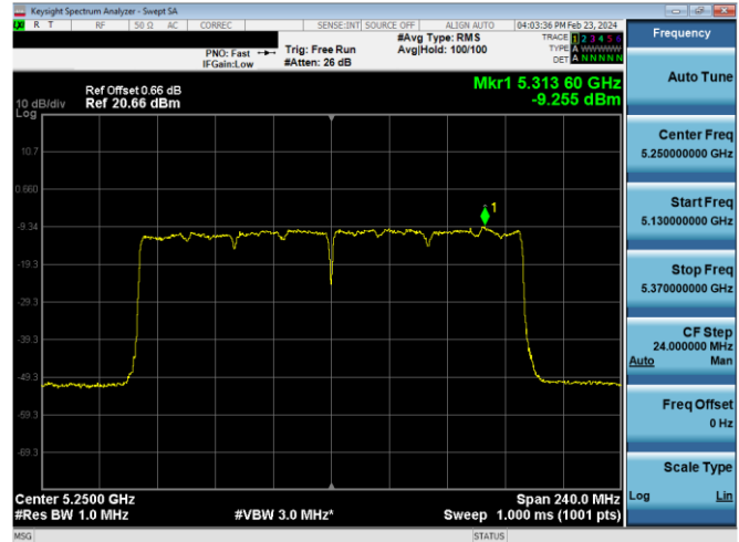
Plot 7-664. ISED PSD CDD Diversity Antenna WF5B (160MHz BW 11ax - RU996x2 - Ch.50)
