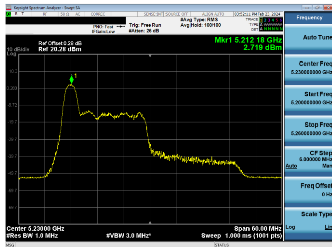
Plot 7-644. ISED PSD SDM Diversity Antenna WF5B (40MHz BW 11ax Index 0 - RU26 - Ch.46)
