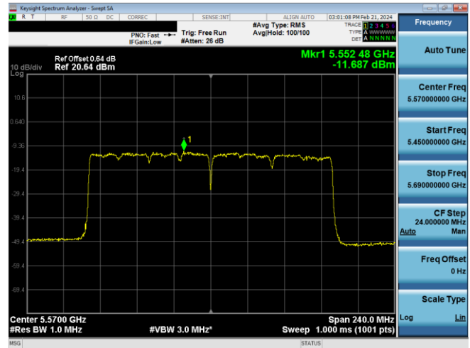
Plot 7-610. PSD CDD Diversity Antenna WF5B (160MHz BW 11ax - RU996x2 - Ch.114)
