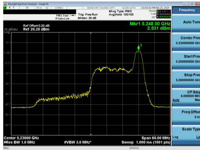
Plot 7-648. ISSED PSD SDM Diversity Antenna WF5B (40MHz BW 11ax Index 17 - RU26 - Ch.46)
