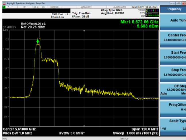
Plot 7-596. PSD CDD Diversity Antenna WF5B (80MHz BW 11ax Index 37 - RU52 - Ch.122)
