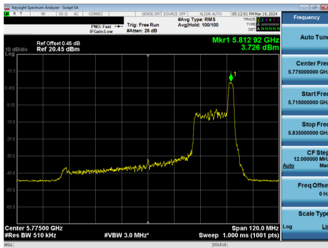
Plot 7-632. PSD CDD Diversity Antenna WF5B (80MHz BW 11ax Index 36 - RU26 - Ch.155)
