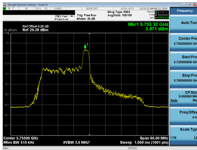
Plot 7-623. PSD CDD Diversity Antenna 2a (40MHz BW 11ax Index 8 - RU26 - Ch.151)
