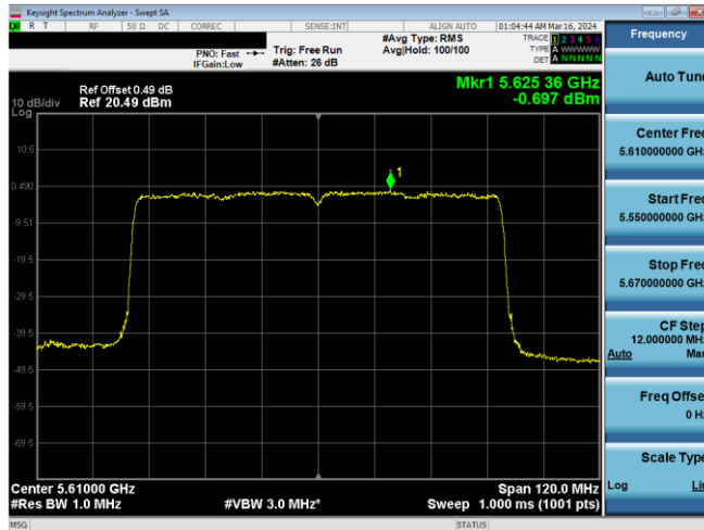
Plot 7-602. PSD CDD Diversity Antenna WF5B (80MHz BW 11ax - RU996 - Ch.122)
