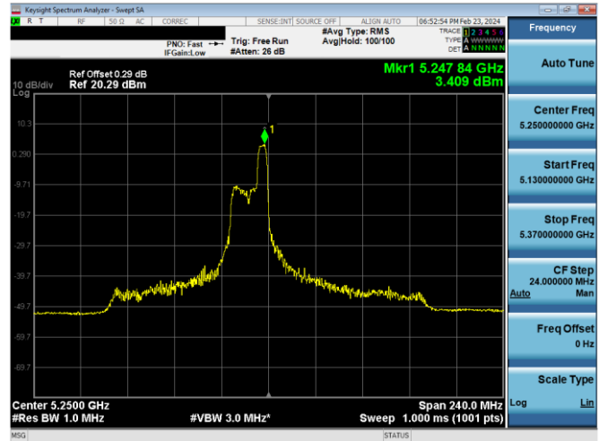
Plot 7-663. ISED PSD SDM Diversity Antenna 2a (160MHz BW 11ax Index 52 - RU52 - Ch.50(L))
