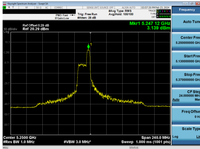
Plot 7-662. ISED PSD SDM Diversity Antenna WF5B (160MHz BW 11ax Index 52 - RU52 - Ch.50(L))
