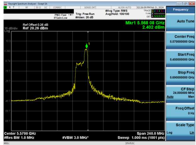
Plot 7-606. PSD CDD Diversity Antenna WF5B (160MHz BW 11ax Index 52 - RU52 - Ch.114 (L))
