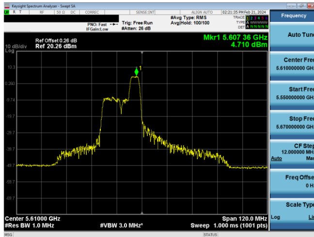
Plot 7-598. PSD CDD Diversity Antenna WF5B (80MHz BW 11ax Index 44 - RU52 - Ch.122)
