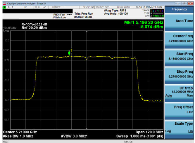
Plot 7-659. ISSED PSD CDD Diversity Antenna 2a (80MHz BW 11ax - RU996 - Ch.42)
