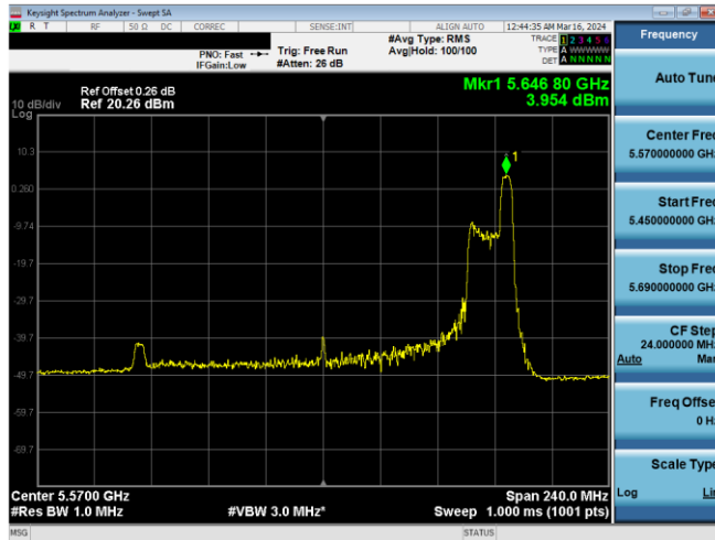
Plot 7-608. PSD CDD Diversity Antenna WF5B (160MHz BW 11ax Index 52 - RU52 - Ch.114 (U))
