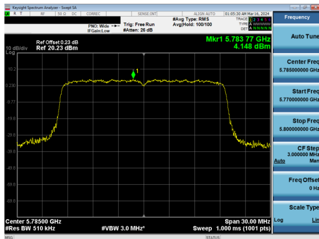
Plot 7-618. PSD CDD Diversity Antenna WF5B (20MHz BW 11ax - RU242 - Ch.157)
