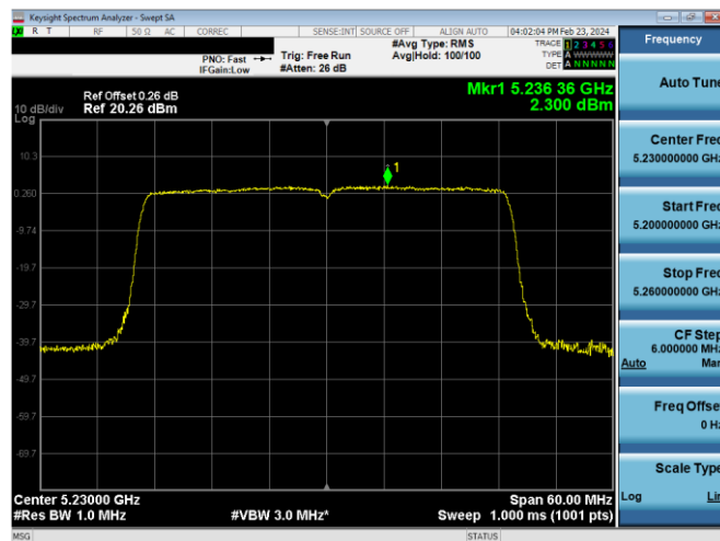
Plot 7-650. ISSED PSD SDM Diversity Antenna WF5B (40MHz BW 11ax - RU484 - Ch.46)
