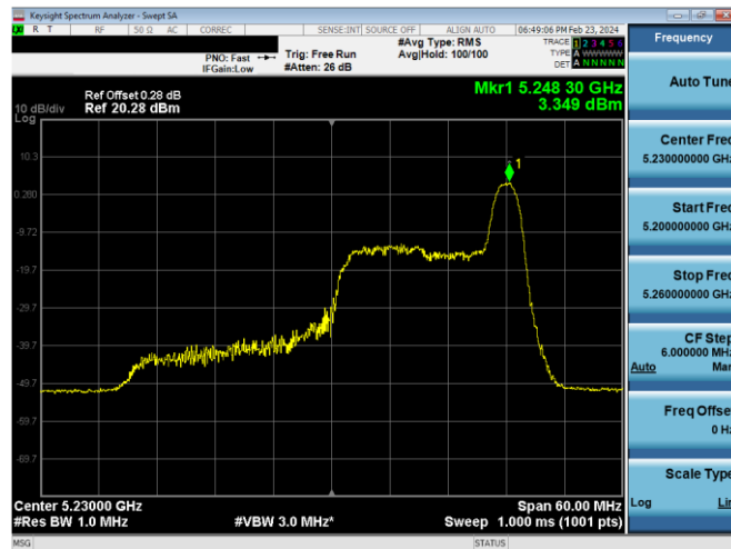
Plot 7-649. ISSED PSD SDM Diversity Antenna 2a (40MHz BW 11ax Index 17 - RU26 - Ch.46)
