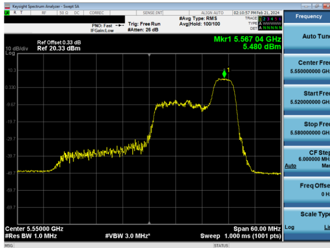
Plot 7-592. PSD CDD Diversity Antenna WF5B (40MHz BW 11ax Index 44 - RU52 - Ch.110)
