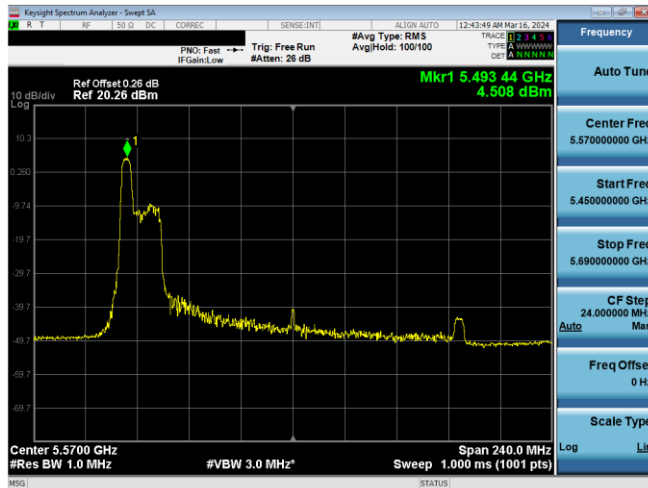
Plot 7-604. PSD CDD Diversity Antenna WF5B (160MHz BW 11ax Index 37 - RU52 - Ch.114 (L))
