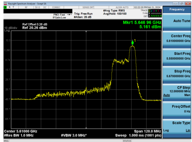
Plot 7-600. PSD CDD Diversity Antenna WF5B (80MHz BW 11ax Index 52 - RU52 - Ch.122)
