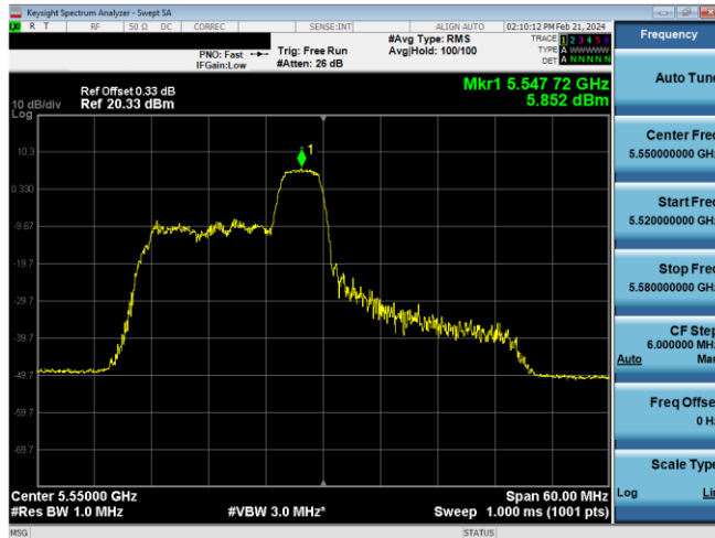
Plot 7-590. PSD CDD Diversity Antenna WF5B (40MHz BW 11ax Index 40 - RU52 - Ch.110)
