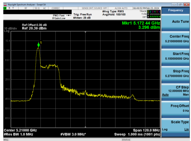
Plot 7-653. ISSED PSD SDM Diversity Antenna 2a (80MHz BW 11ax Index 0 - RU26 - Ch.42)
