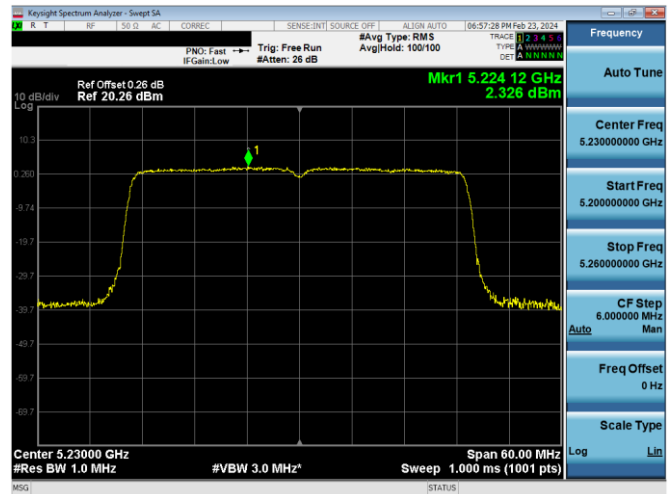
Plot 7-651. ISSED PSD SDM Diversity Antenna 2a (40MHz BW 11ax - RU484 - Ch.46)
