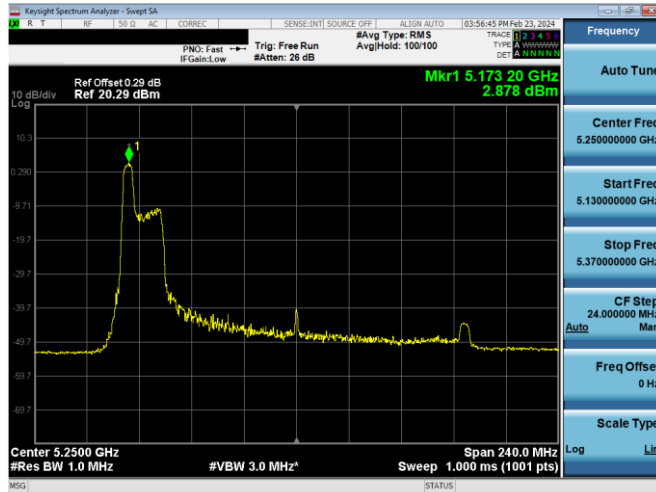
Plot 7-660. ISED PSD SDM Diversity Antenna WF5B (160MHz BW 11ax Index 37 - RU52 - Ch.50(L))
