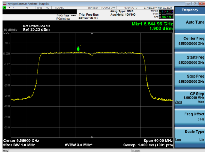
Plot 7-594. PSD CDD Diversity Antenna WF5B (40MHz BW 11ax - RU484 - Ch.110)
