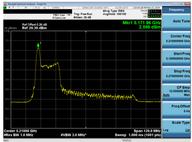
Plot 7-652. ISSED PSD SDM Diversity Antenna WF5B (80MHz BW 11ax Index 0 - RU26 - Ch.42)
