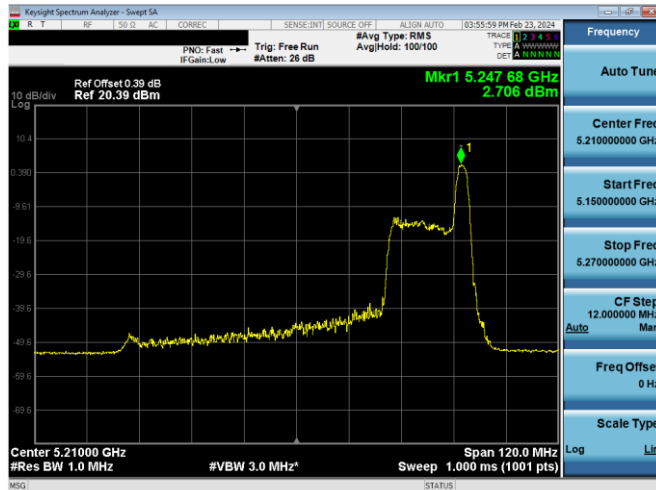
Plot 7-656. ISSED PSD SDM Diversity Antenna WF5B (80MHz BW 11ax Index 36 - RU26 - Ch.42)
