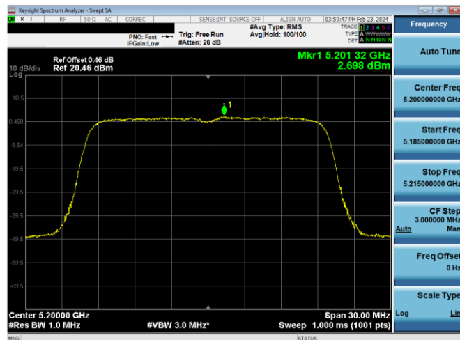
Plot 7-642. ISED PSD SDM Diversity Antenna WF5B (20MHz BW 11ax- RU242 - Ch.40)
