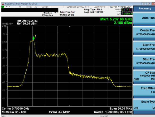
Plot 7-620. PSD CDD Diversity Antenna WF5B (40MHz BW 11ax Index 0 - RU26 - Ch.151)
