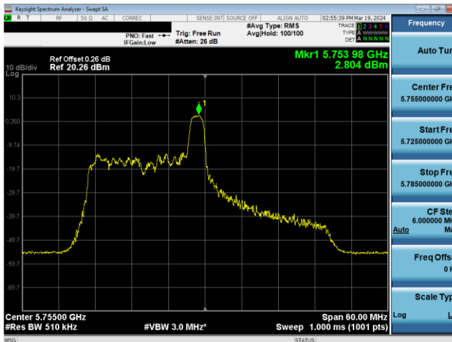
Plot 7-622. PSD CDD Diversity Antenna WF5B (40MHz BW 11ax Index 8 - RU26 - Ch.151)
