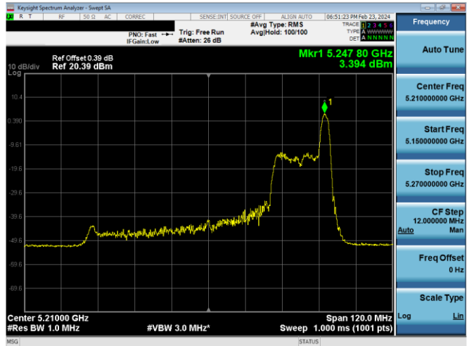
Plot 7-657. ISSED PSD SDM Diversity Antenna 2a (80MHz BW 11ax Index 36 - RU26 - Ch.42)
