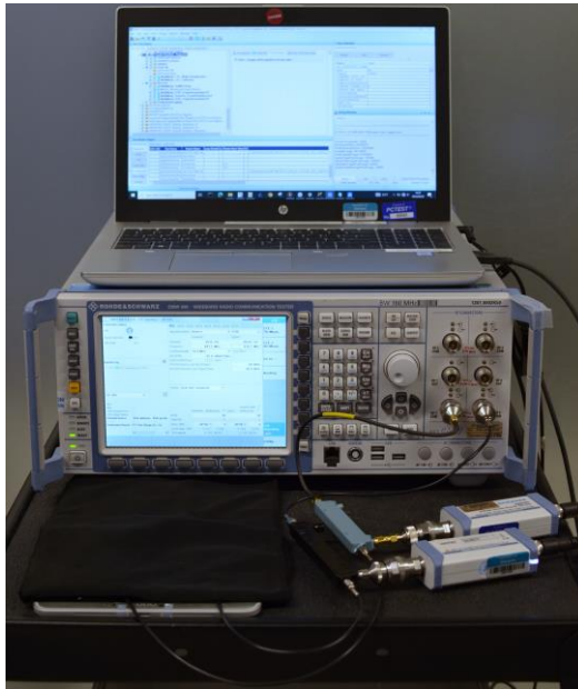
Test Setup Photo 5 – Conducted Test Setup (Figure 5-1d)
