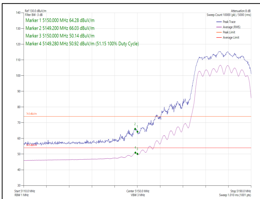
Figure 13 - 802.11n HT20 CDD, Cores 0-1 - 5180 MHz Band Edge Frequency 5150 MHz
