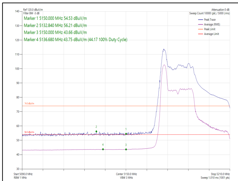
Figure 33 - 802.11ax HE40, Core 1, 26-0 - 5190 MHz Band Edge Frequency 5150 MHz
