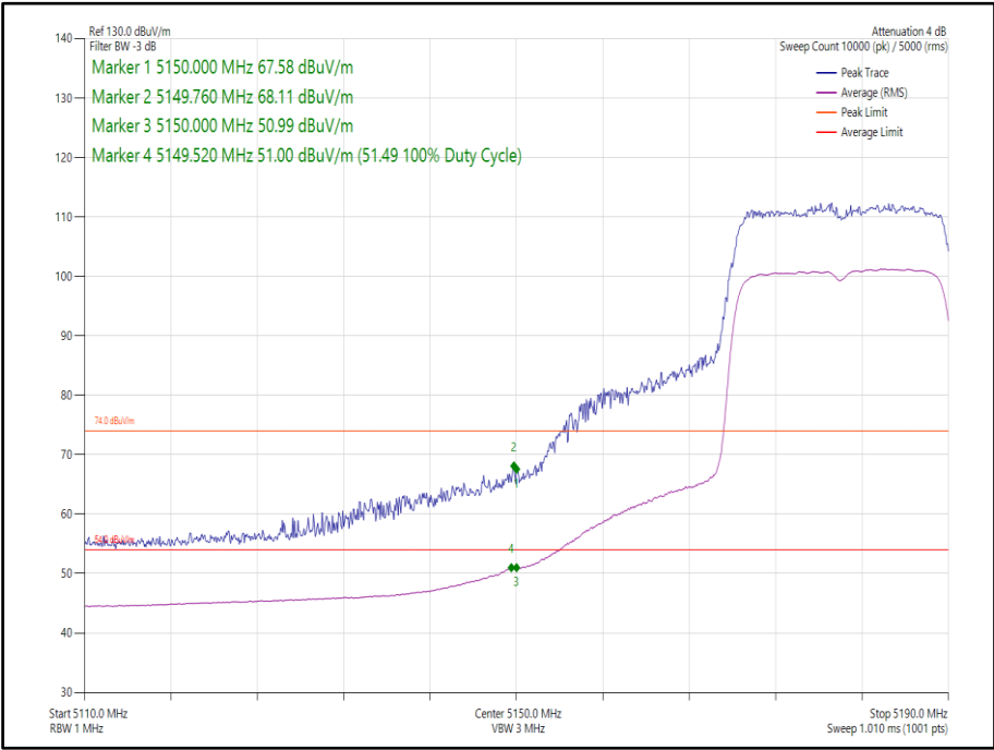
Figure 3 - 802.11ax HE20, Core 1, SU - 5180 MHz, Band Edge Frequency 5150 MHz
