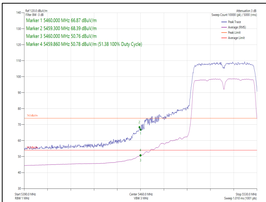
Figure 37 - 802.11n HT40, Core 1 - 5510 MHz Band Edge Frequency 5460 MHz
