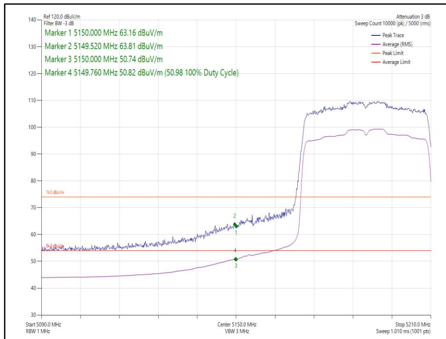
Figure 32 - 802.11ax HE40, Core 1, SU - 5190 MHz Band Edge Frequency 5150 MHz
