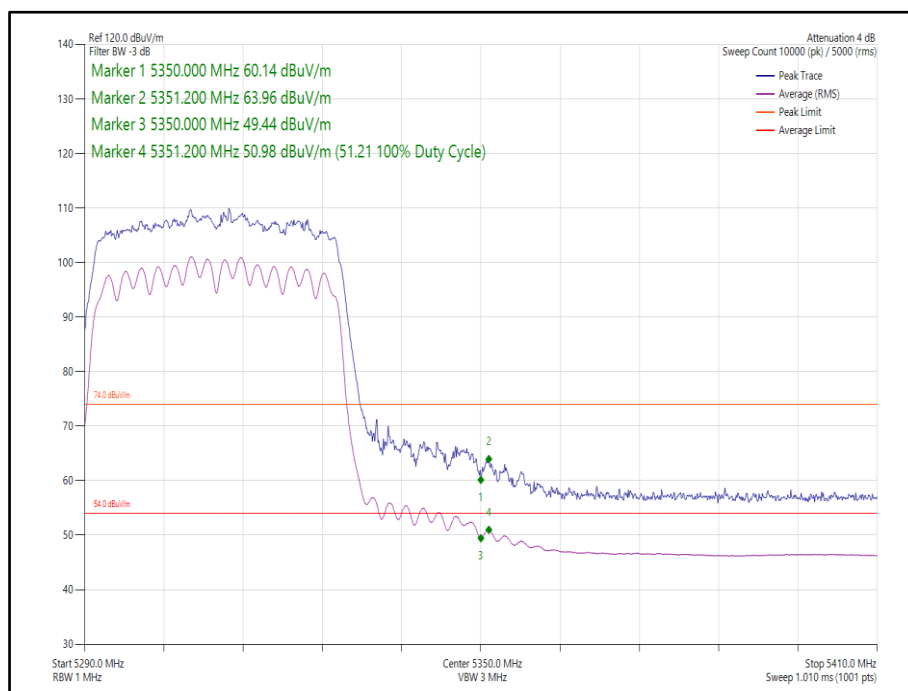
Figure 46 - 802.11n HT40 CDD, Cores 0-1 - 5310 MHz Band Edge Frequency 5350 MHz
