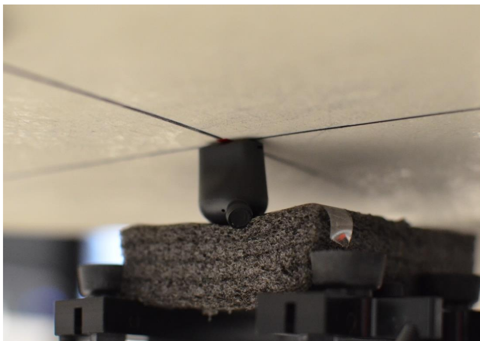
SAR Test Setup Photo 2: Body-Worn, Back Side, 0 mm
