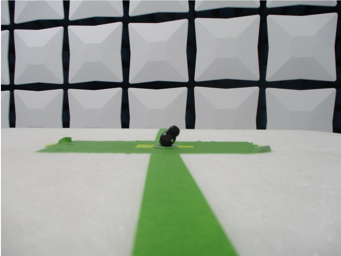
Figure 3: 1-18GHz Test Setup (Front View)
