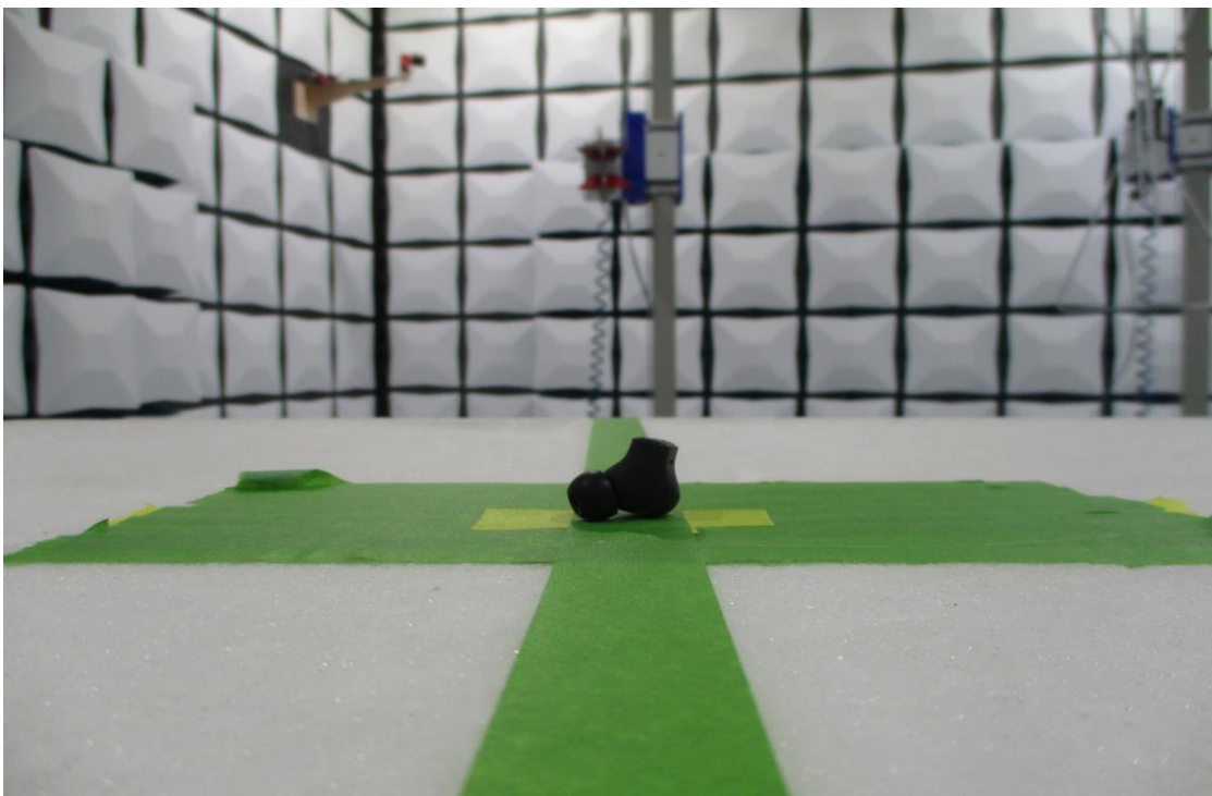
Figure 2: 1-18GHz Test Setup (Rear View)
