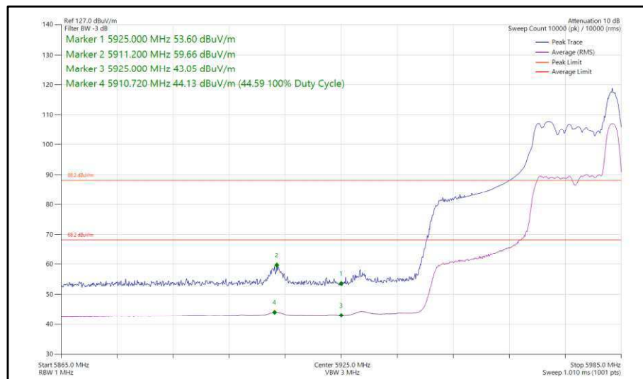
Figure 50 - 802.11ax, HE40, RU 26-17, SISO, Core 0 - 5965 MHz, Band Edge Frequency 5925 MHz
