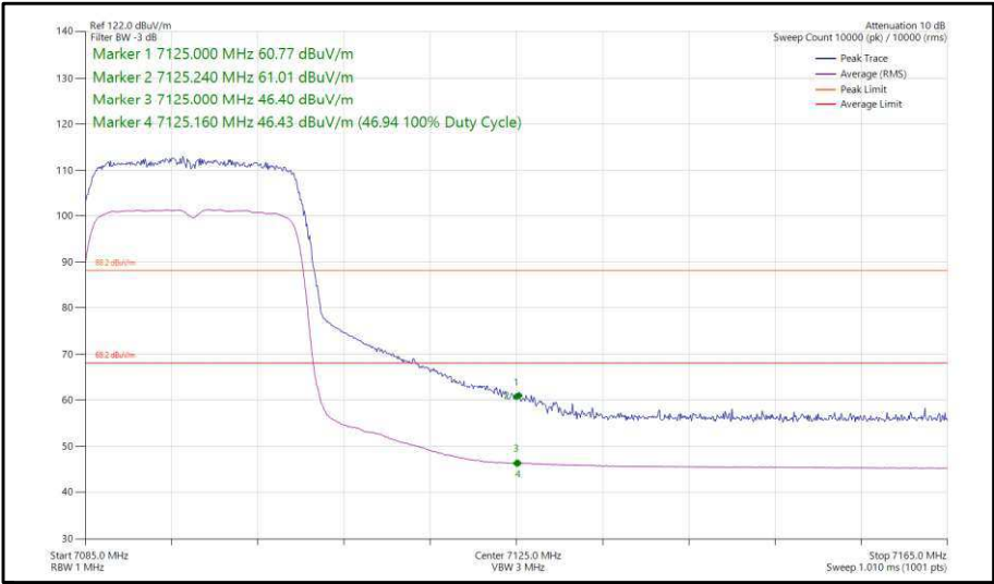
Figure 42 - 802.11ax, HE20, SU, SISO, Core 1 - 7095 MHz, Band Edge Frequency 7125 MHz
