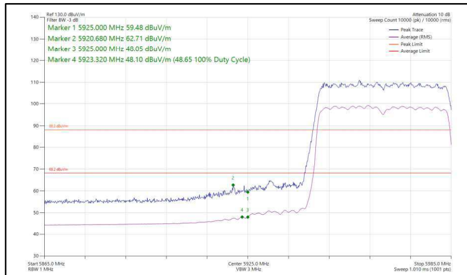
Figure 57 - 802.11ax, HE40, SU, CDD, Core 0-1 - 5965 MHz, Band Edge Frequency 5925 MHz
