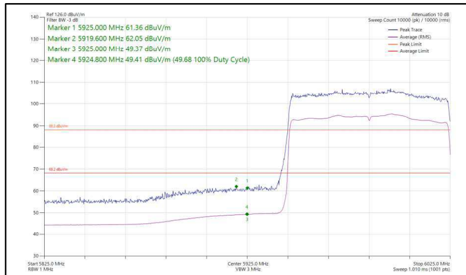
Figure 77 - 802.11ax, HE80, SU, TxBF, Core 0-1 - 5985 MHz, Band Edge Frequency 5925 MHz
