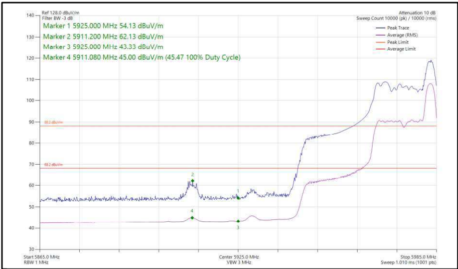
Figure 54 - 802.11ax, HE40, RU 26-17, SISO, Core 1 - 5965 MHz, Band Edge Frequency 5925 MHz
