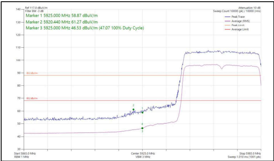
Figure 53 - 802.11ax, HE40, SU, SISO, Core 1 - 5965 MHz, Band Edge Frequency 5925 MHz
