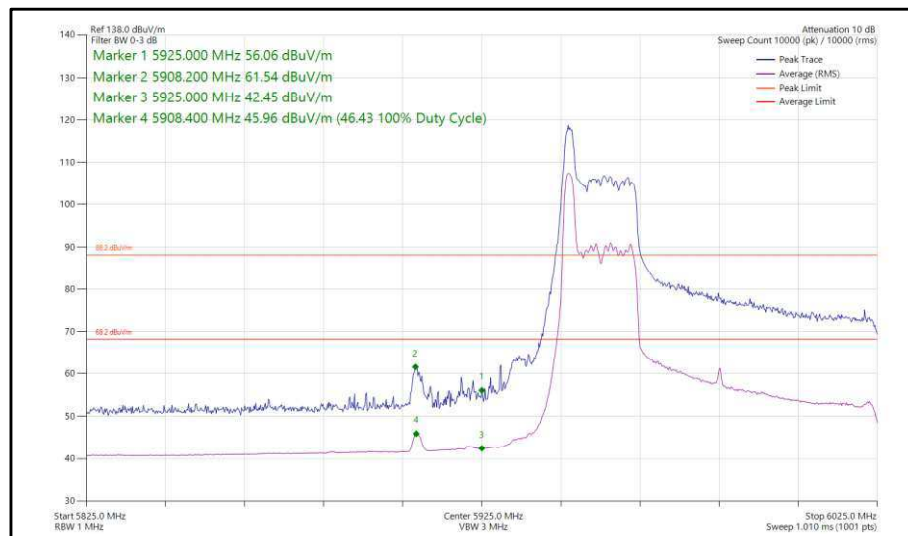
Figure 74 - 802.11ax, HE80, RU 26-0, SDM, Core 0-1 - 5985 MHz, Band Edge Frequency 5925 MHz
