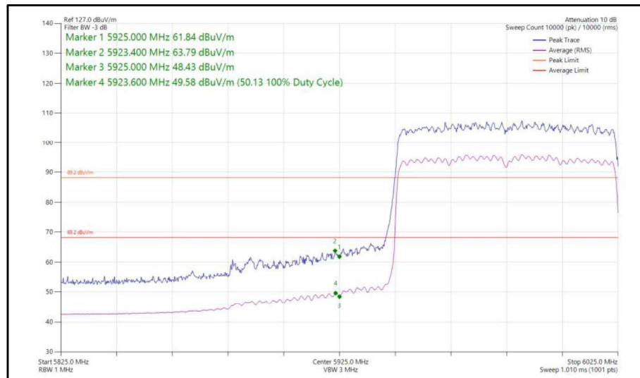
Figure 71 - 802.11ax, HE80, SU, CDD, Core 0-1 - 5985 MHz, Band Edge Frequency 5925 MHz
