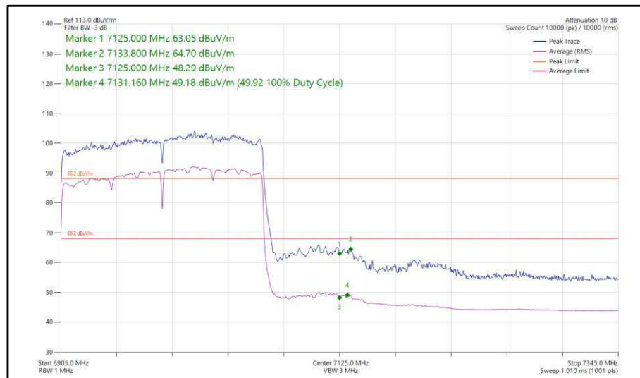
Figure 85 - 802.11ax, HE160, SU, SISO, Core 1 - 6985 MHz, Band Edge Frequency 7125 MHz
