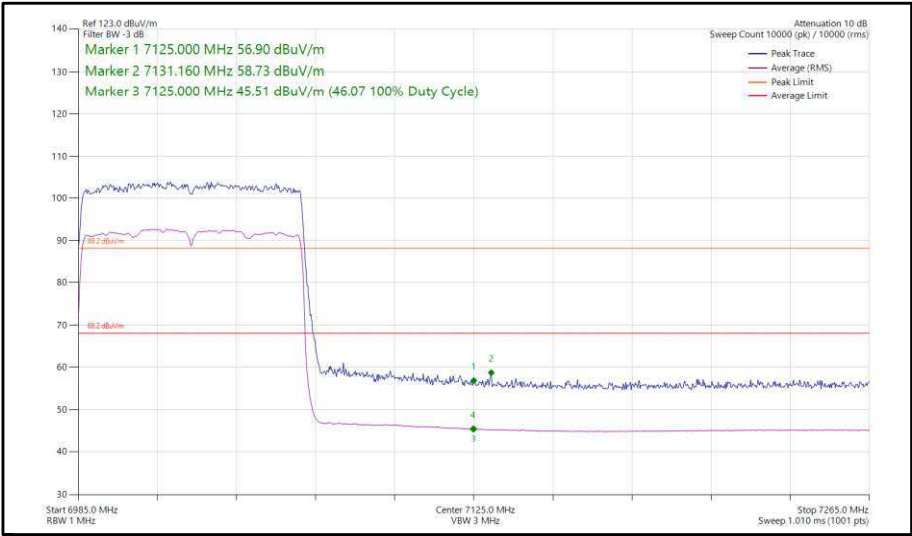
Figure 65 - 802.11ax, HE80, SU, SISO, Core 0 - 7025 MHz, Band Edge Frequency 7125 MHz
