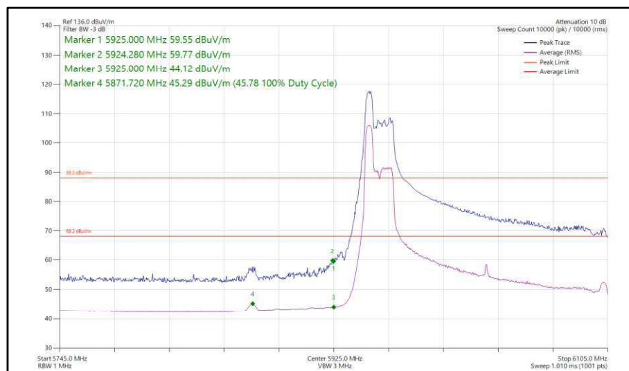
Figure 84 - 802.11ax, HE160, RU 52-37, SISO, Core 1 - 6025 MHz, Band Edge Frequency 5925 MHz
