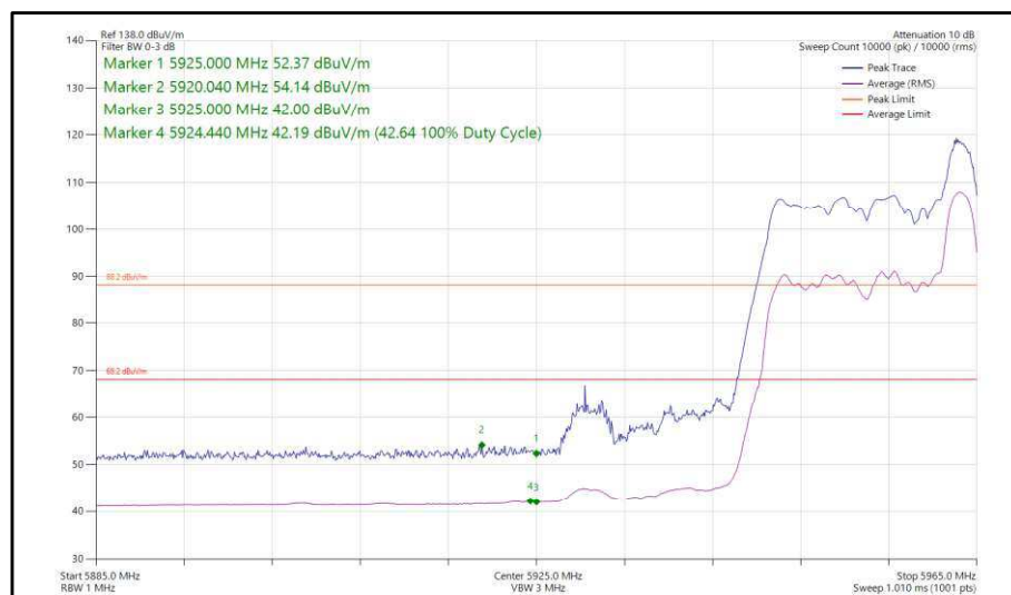
Figure 47 - 802.11ax, HE20, RU 26-8, SDM, Core 0-1 - 5955 MHz, Band Edge Frequency 5925 MHz
