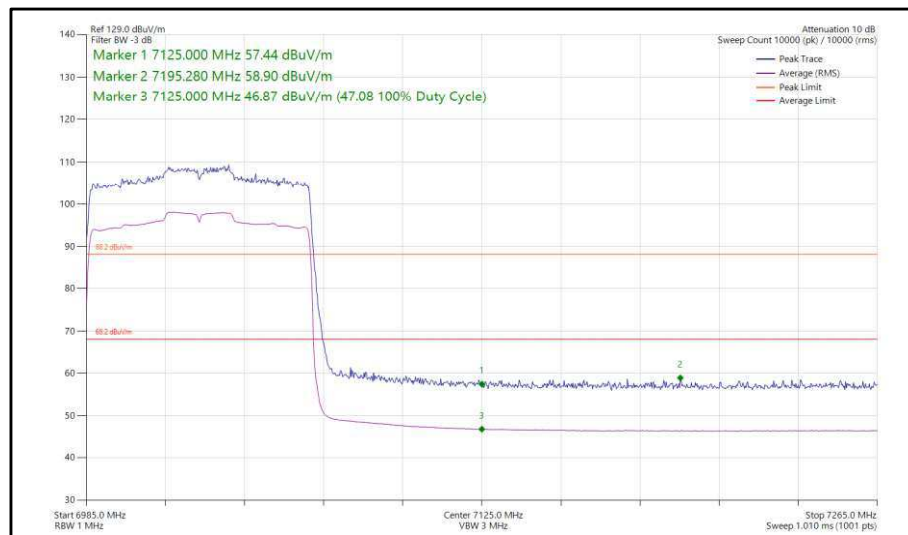
Figure 78 - 802.11ax, HE80, SU, TxBF, Core 0-1 - 7025 MHz, Band Edge Frequency 7125 MHz
