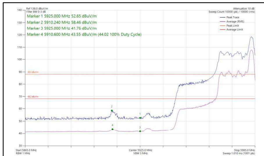
Figure 60 - 802.11ax, HE40, RU 26-17, SDM, Core 0-1 - 5965 MHz, Band Edge Frequency 5925 MHz
