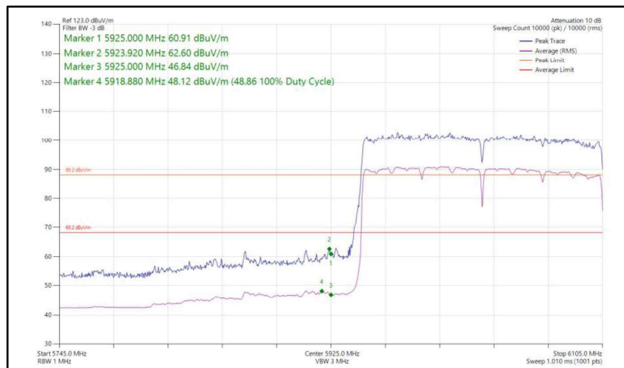
Figure 83 - 802.11ax, HE160, SU, SISO, Core 1 - 6025 MHz, Band Edge Frequency 5925 MHz
