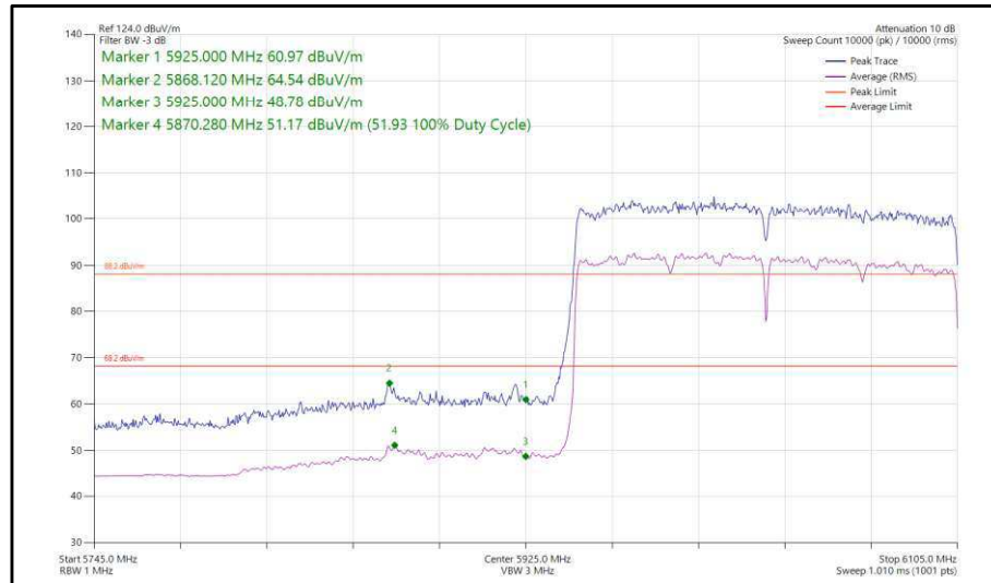
Figure 87 - 802.11ax, HE160, SU, CDD, Core 0-1 - 6025 MHz, Band Edge Frequency 5925 MHz
