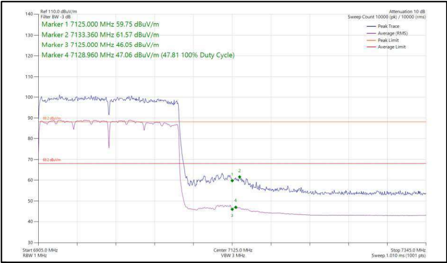
Figure 81 - 802.11ax, HE160, SU, SISO, Core 0 - 6985 MHz, Band Edge Frequency 7125 MHz
