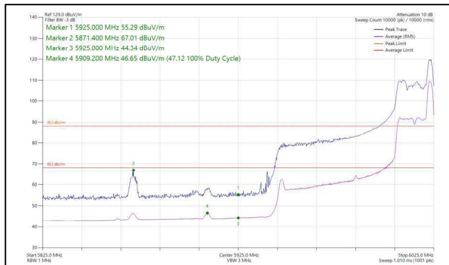
Figure 68 - 802.11ax, HE80, RU 26-36, SISO, Core 1 - 5985 MHz, Band Edge Frequency 5925 MHz
