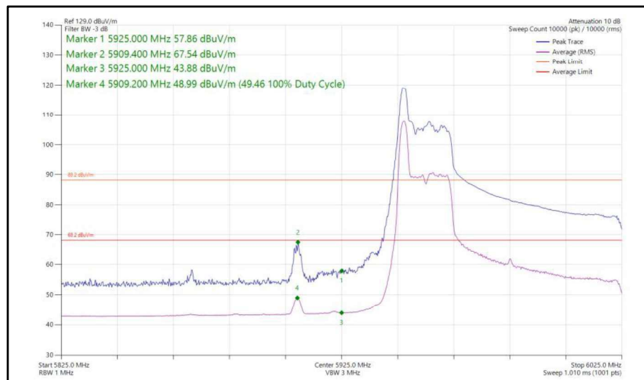
Figure 64 - 802.11ax, HE80, RU 26-0, SISO, Core 0 - 5985 MHz, Band Edge Frequency 5925 MHz
