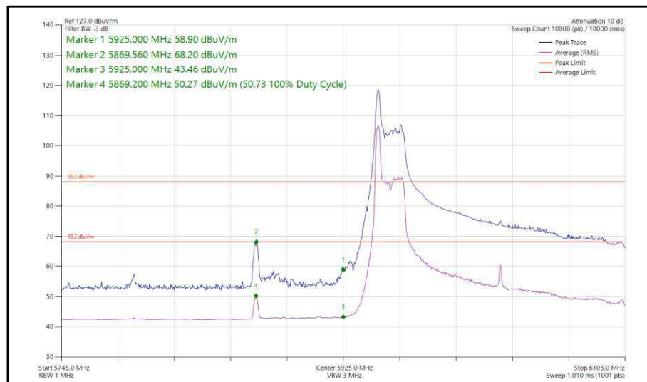
Figure 80 - 802.11ax, HE160, RU 26-0, SISO, Core 0 - 6025 MHz, Band Edge Frequency 5925 MHz
