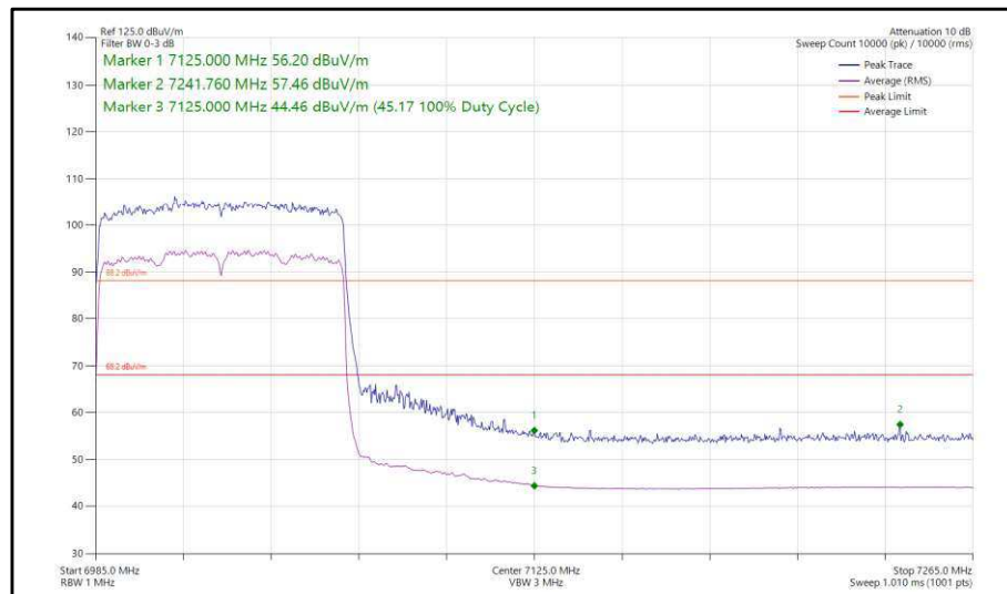
Figure 75 - 802.11ax, HE80, SU, SDM, Core 0-1 - 7025 MHz, Band Edge Frequency 7125 MHz
