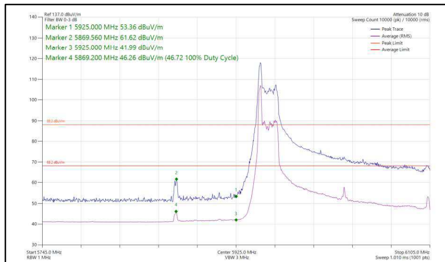
Figure 90 - 802.11ax, HE160, RU 26-0, SDM, Core 0-1 - 6025 MHz, Band Edge Frequency 5925 MHz
