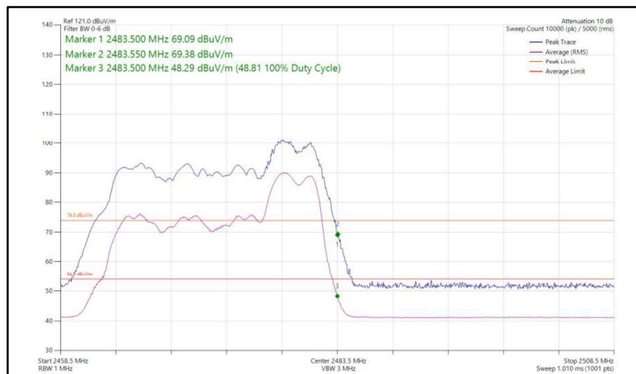
Figure 52 - 802.11ax, HE20, RU 52-40, CDD, Core 0-1 - 2472 MHz, Band Edge Frequency 2483.5 MHz
