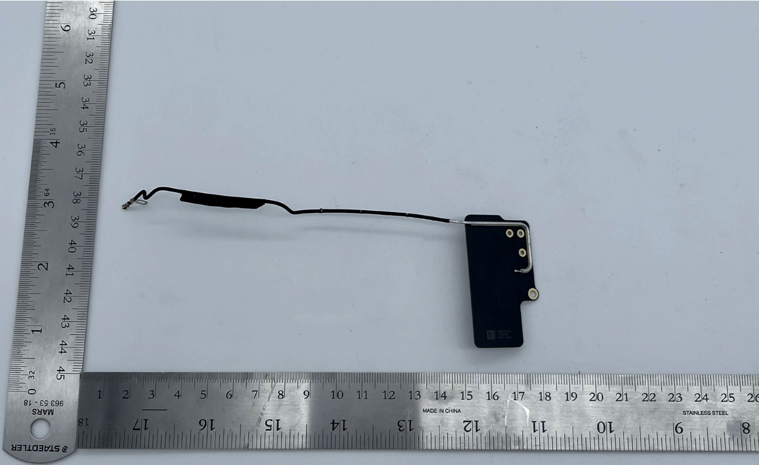
A2874 Antenna WF1 - Back
