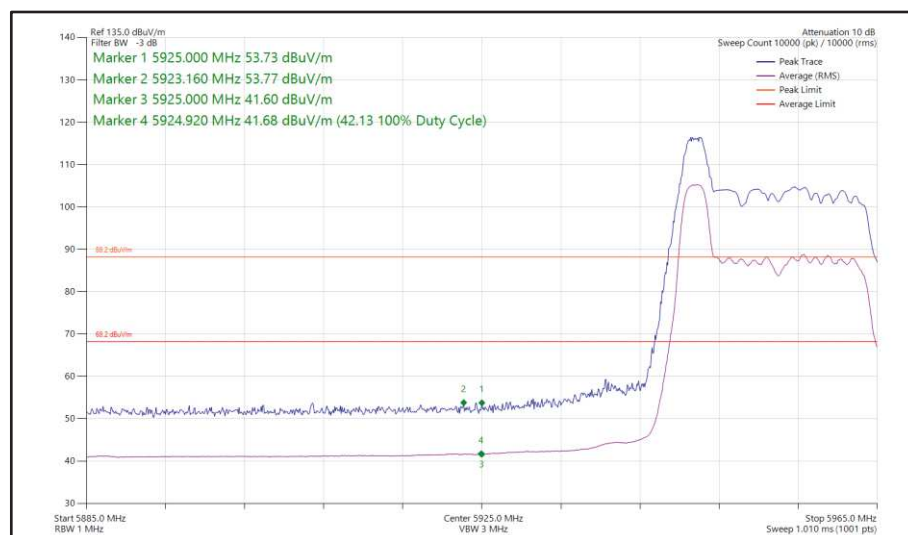
Figure 33 - 802.11ax, HE20, RU 26-0, SISO, Core 0 - 5955 MHz, Band Edge Frequency 5925 MHz
