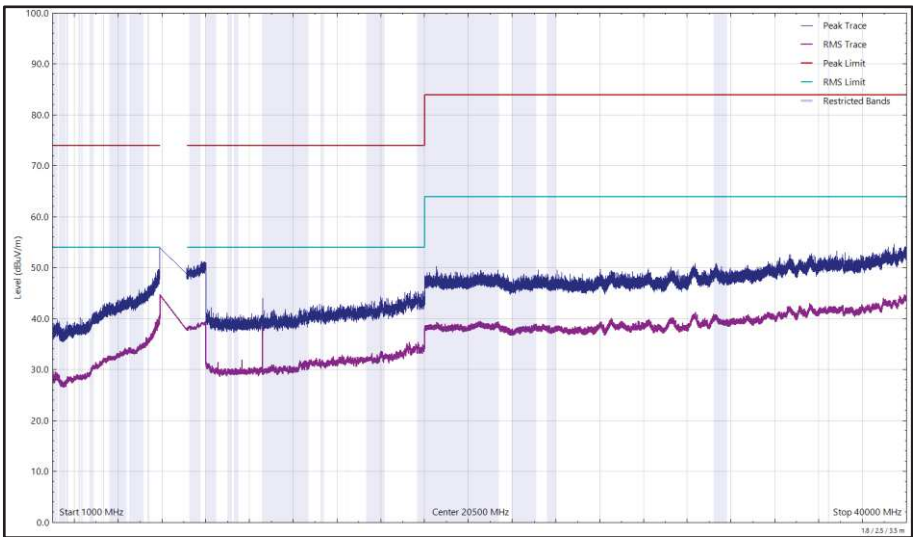
Figure 113 - U-NII-5 - 6415 MHz (CH93), HE20, SU, CDD, Core 0 + Core 1, 1 GHz to 40 GHz, Vertical
