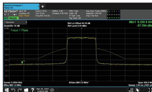
Figure 129 - B (Core 0) 802.11ax HE80 SU 6385 MHz (CH87)
