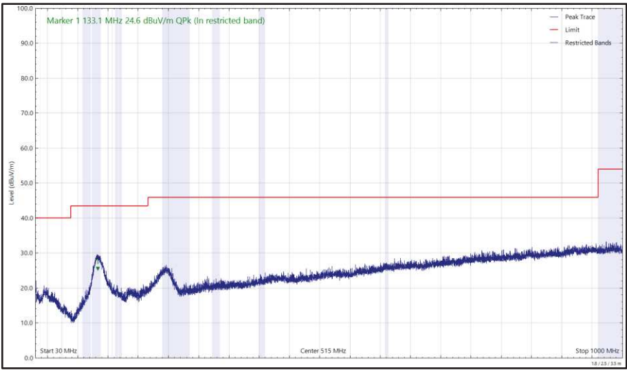
Figure 94 - U-NII-5 - 6175 MHz (CH45), HE20, SU, CDD, Core 0 + Core 1, 30 MHz to 1 GHz, Horizontal (Peak)
