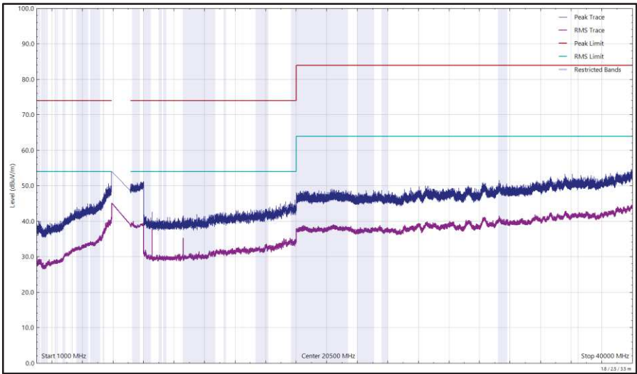
Figure 112 - U-NII-5 - 6415 MHz (CH93), HE20, SU, CDD, Core 0 + Core 1, 1 GHz to 40 GHz, Horizontal
