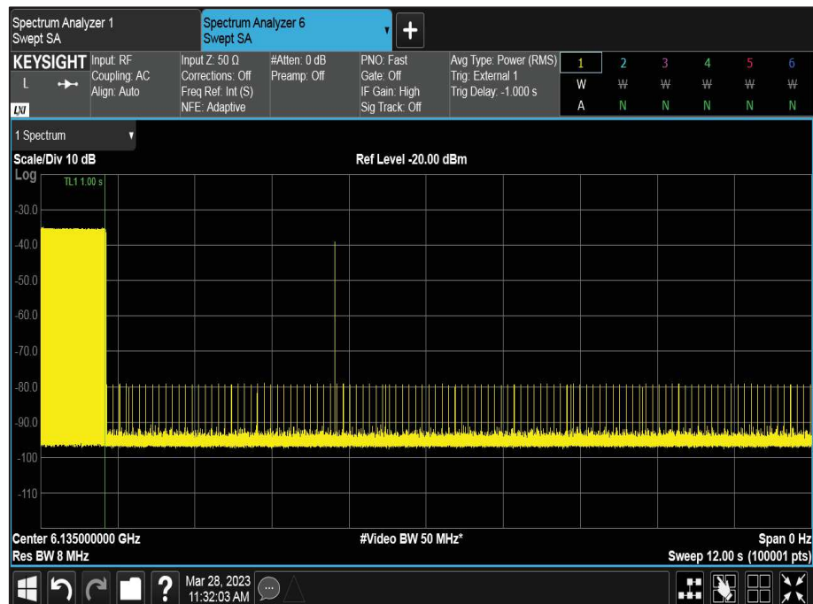
Figure 152 - U-NII-5, Minimum Bandwidth (AWGN Low)
