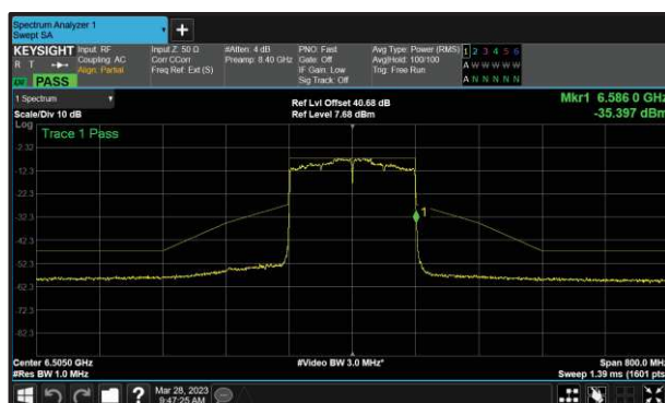
Figure 130 - B (Core 0) 802.11ax HE160 SU 6505 MHz (CH111)
