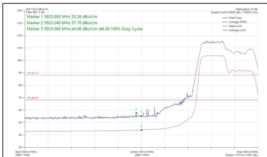
Figure 47 - 802.11ax, HE20, RU 106-53, SDM, Core 0-1 - 5955 MHz, Band Edge Frequency 5925 MHz
