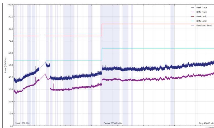
Figure 122 - U-NII-8 - 6895 MHz (CH189), HE20, SU, CDD, Core 0 + Core 1, 1 GHz to 40 GHz, Horizontal
