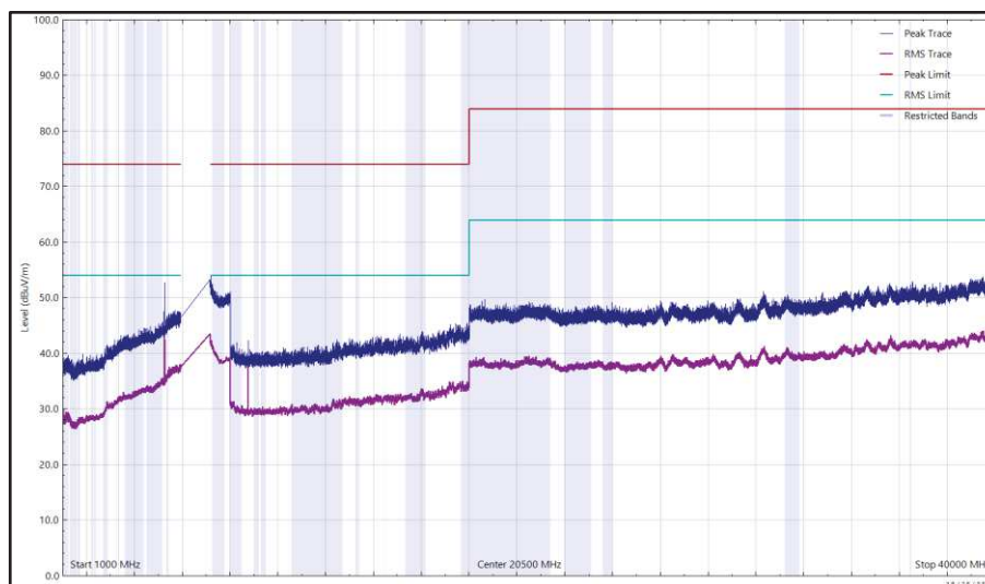
Figure 107 - U-NII-8 - 6995 MHz (CH209), HE20, SU, CDD, Core 0 + Core 1, 1 GHz to 40 GHz, Horizontal
