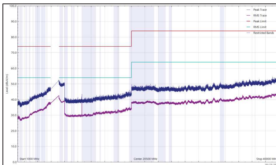
Figure 120 - U-NII-7 - 6855 MHz (CH181), HE20, SU, CDD, Core 0 + Core 1, 1 GHz to 40 GHz, Horizontal
