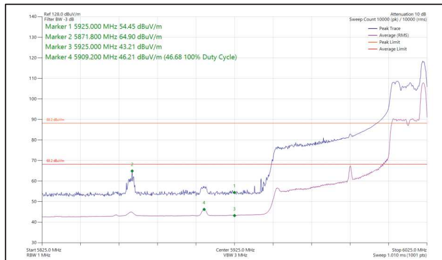
Figure 64 - 802.11ax, HE80, RU 26-36, SISO, Core 0 - 5985 MHz, Band Edge Frequency 5925 MHz
