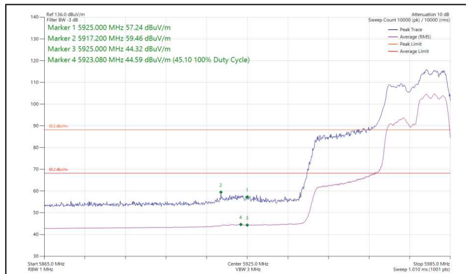
Figure 58 - 802.11ax, HE40, RU 106-56, CDD, Core 0-1 - 5965 MHz, Band Edge Frequency 5925 MHz
