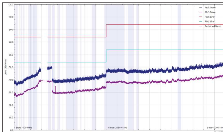
Figure 99 - U-NII-6 - 6475 MHz (CH105), HE20, SU, CDD, Core 0 + Core 1, 1 GHz to 40 GHz, Horizontal
