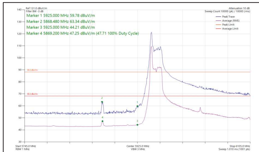
Figure 84 - 802.11ax, HE160, RU 26-0, SISO, Core 1 - 6025 MHz, Band Edge Frequency 5925 MHz
