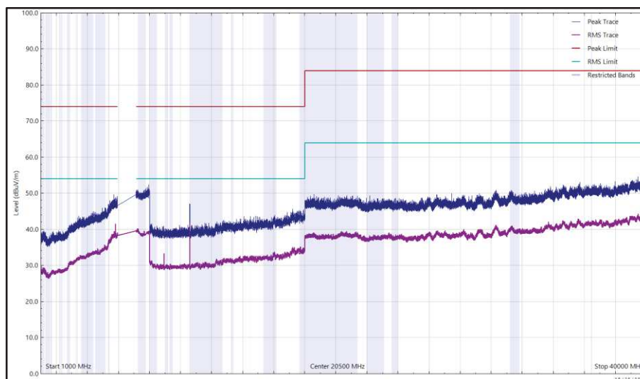
Figure 103 - U-NII-7 - 6695 MHz (CH149), HE20, SU, CDD, Core 0 + Core 1, 1 GHz to 40 GHz, Horizontal
