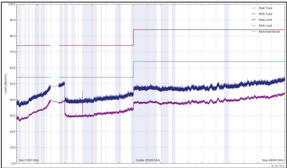
Figure 115 - U-NII-6 - 6435 MHz (CH97), HE20, SU, CDD, Core 0 + Core 1, 1 GHz to 40 GHz, Vertical
