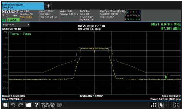
Figure 126 - B (Core 0) 802.11a 6875 MHz (CH185)
