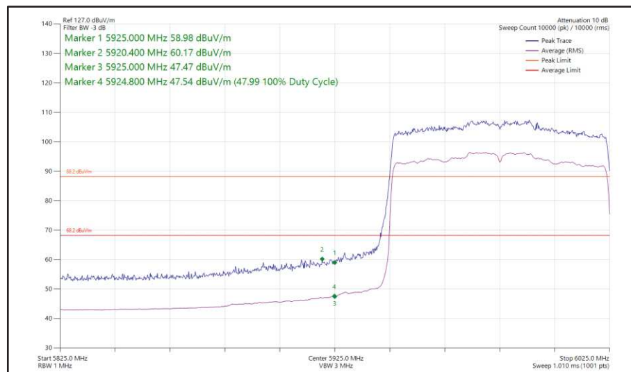
Figure 73 - 802.11ax, HE80, SU, SDM, Core 0-1 - 5985 MHz, Band Edge Frequency 5925 MHz
