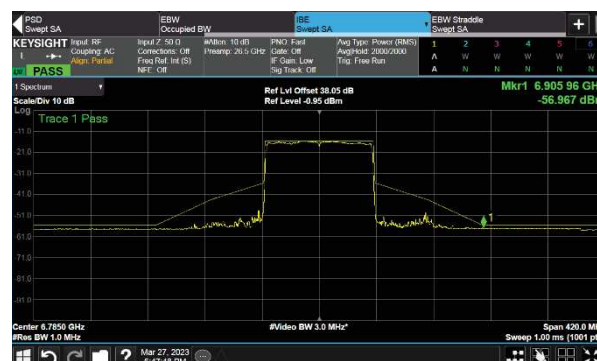
Figure 148 - B (Core 1) 802.11ax HE80 SU 6785 MHz (CH167)
