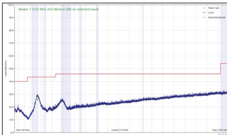
Figure 98 - U-NII-6 - 6475 MHz (CH105), HE20, SU, CDD, Core 0 + Core 1, 30 MHz to 1 GHz, Horizontal (Peak)
