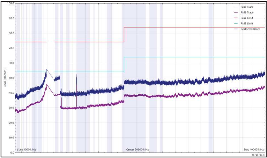
Figure 95 - U-NII-5 - 6175 MHz (CH45), HE20, SU, CDD, Core 0 + Core 1, 1 GHz to 40 GHz, Horizontal
