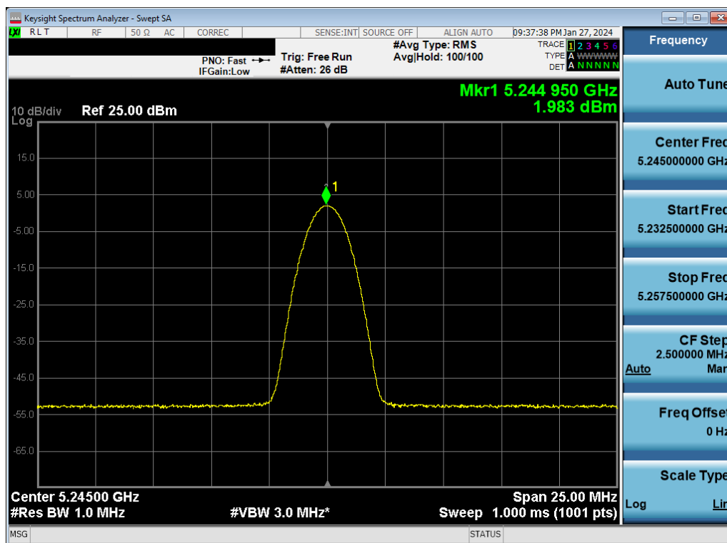
Plot 7-81. ISED PSD TxBF Antenna WF2a (BDR GFSK, ePA- 5245MHz)
