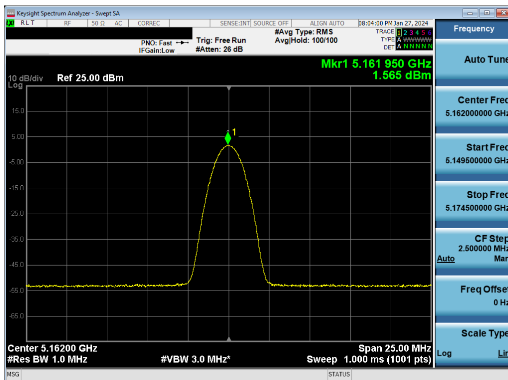
Plot 7-82. ISED PSD TxBF Antenna WF7a (BDR GFSK, iPA – 5162MHz)
