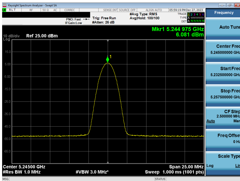
Plot 7-24. FCC/ISED PSD Antenna WF7a (BDR GFSK, iPA– 5245MHz)
