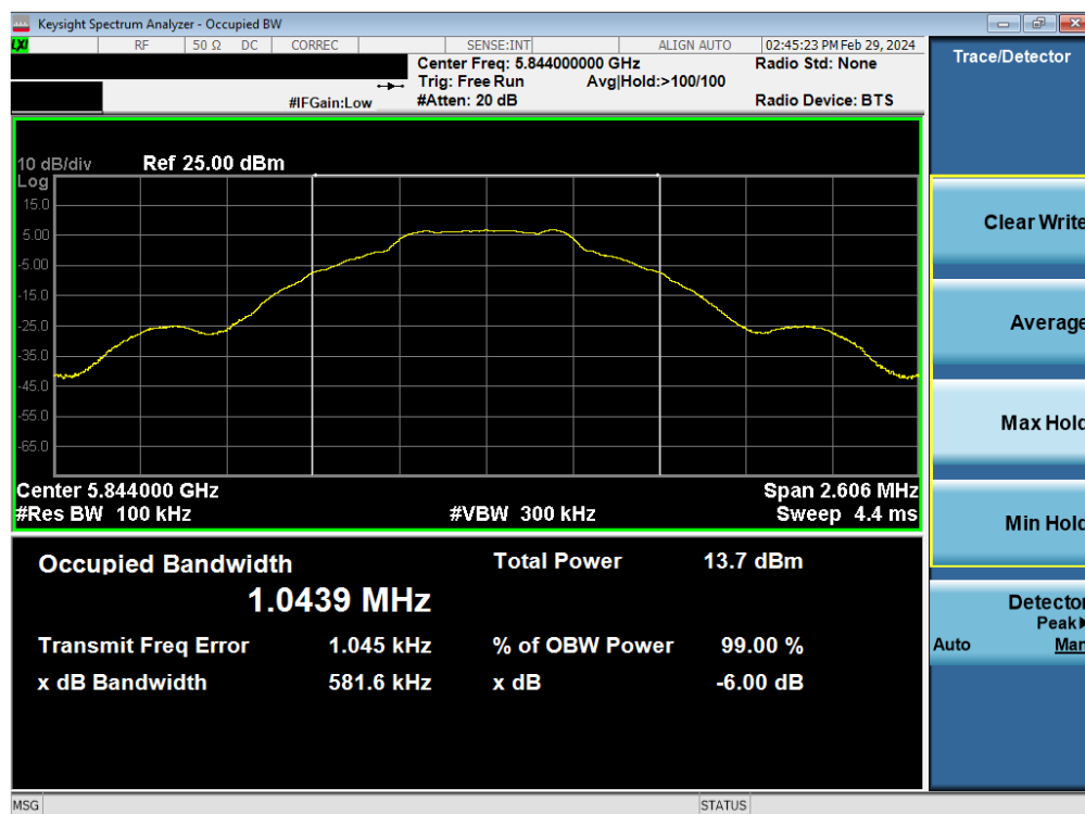
Plot 7-15. 6dB BW & 99% OBW Antenna WF2a (BDR GFSK, ePA 5844MHz)
