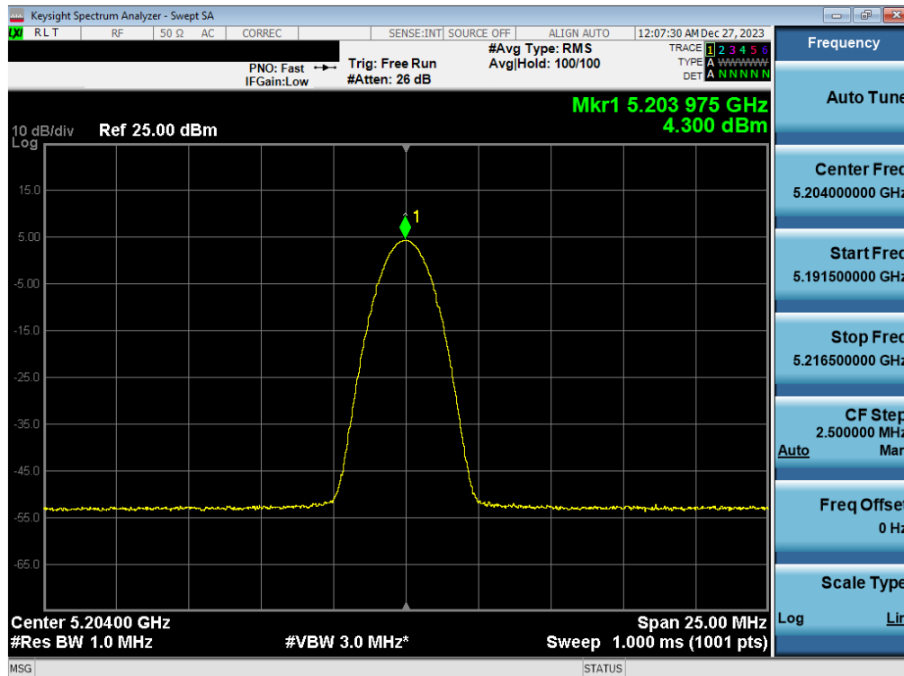
Plot 7-38. FCC/ISED PSD Antenna WF2a (BDR GFSK, iPA – 5204MHz)
