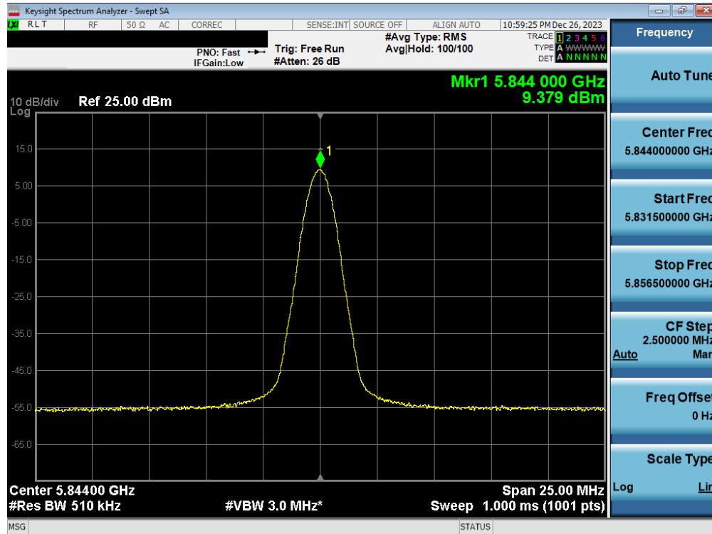
Plot 7-60. PSD Antenna WF7b (BDR GFSK, ePA 5844MHz)
