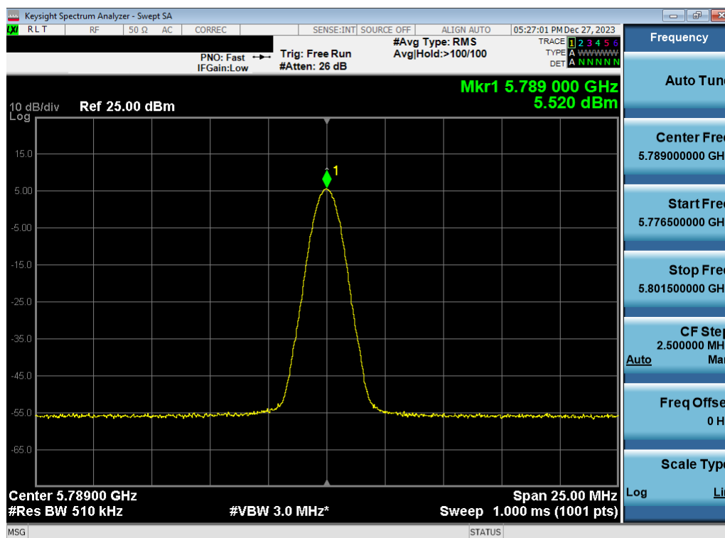
Plot 7-32. PSD Antenna WF7a (BDR GFSK, iPA 5789MHz)
