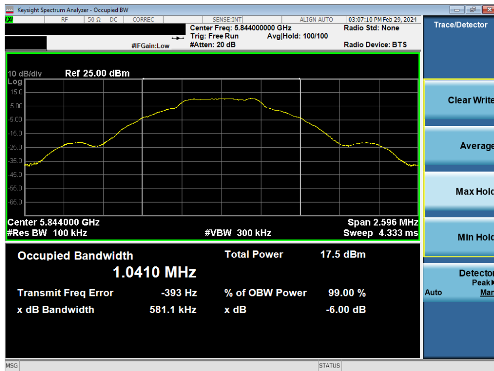
Plot 7-18. 6dB BW & 99% OBW Antenna WF7b (BDR GFSK, ePA 5844MHz)
