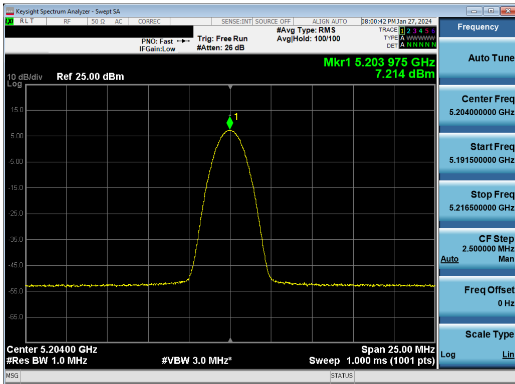
Plot 7-26. ISED PSD Antenna WF7a (BDR GFSK, ePA – 5204MHz)
