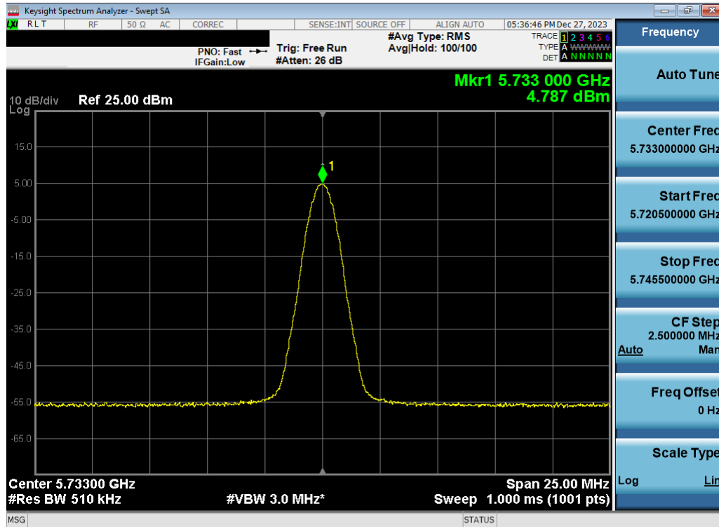
Plot 7-94. PSD TxBF Antenna WF7a (BDR GFSK, iPA 5733MHz)
