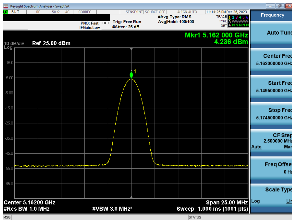
7-52. FCC/ISED PSD Antenna WF7b (BDR GFSK, iPA - 5162MHz)
