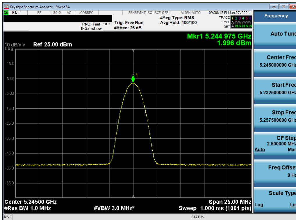
Plot 7-87. ISED PSD TxBF Antenna WF2a (BDR GFSK, iPA- 5245MHz)
