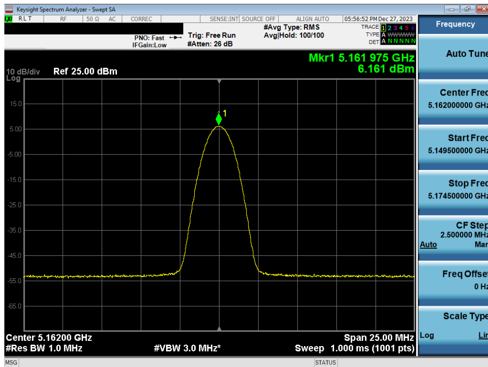
Plot 7-22. FCC/ISED PSD Antenna WF7a (BDR GFSK, iPA – 5162MHz)
