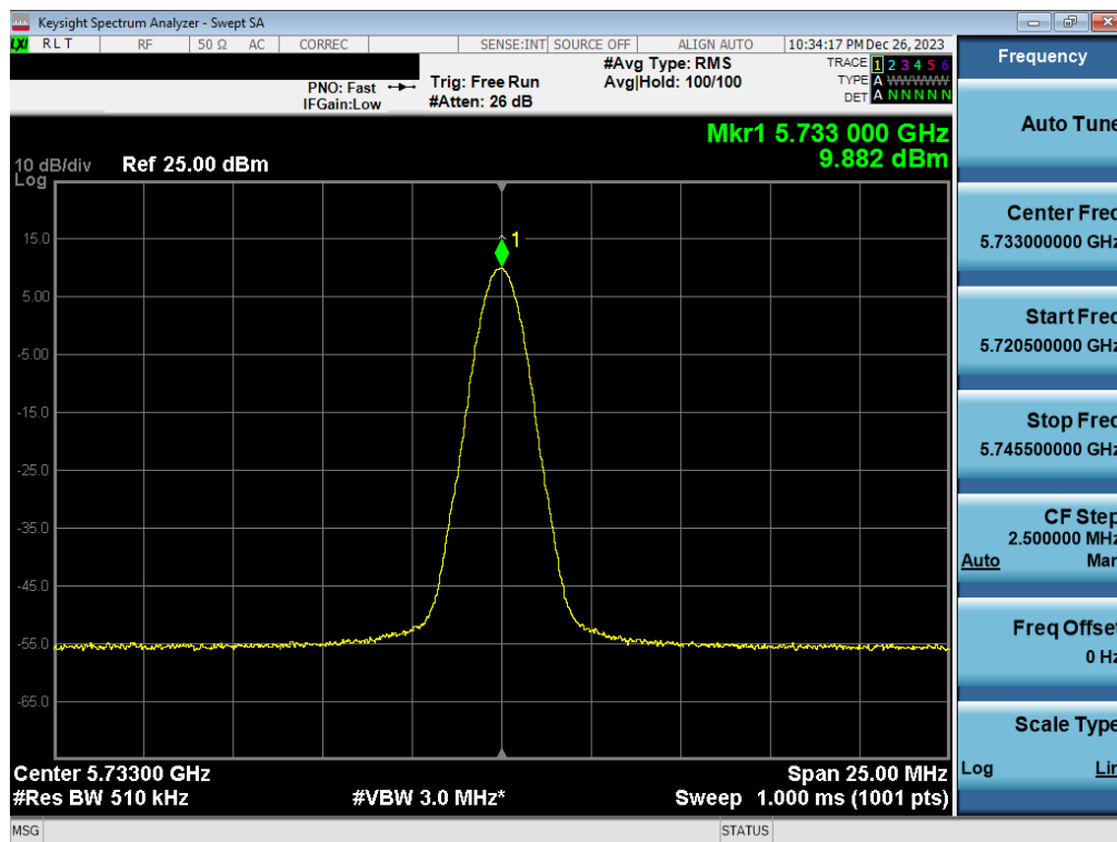
Plot 7-89. PSD TxBF Antenna WF2a (BDR GFSK, ePA 5733MHz)
