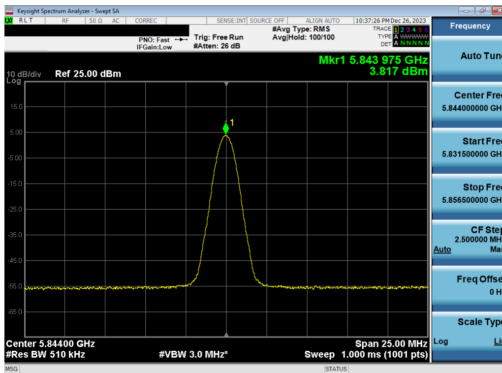
Plot 7-99. PSD TxBF Antenna WF2a (BDR GFSK, iPA 5844MHz)
