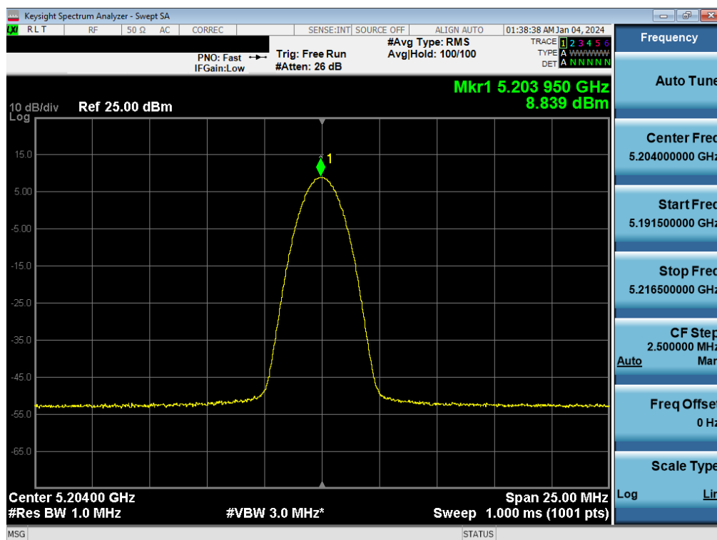
Plot 7-20. FCC PSD Antenna WF7a (BDR GFSK, ePA – 5204MHz)
