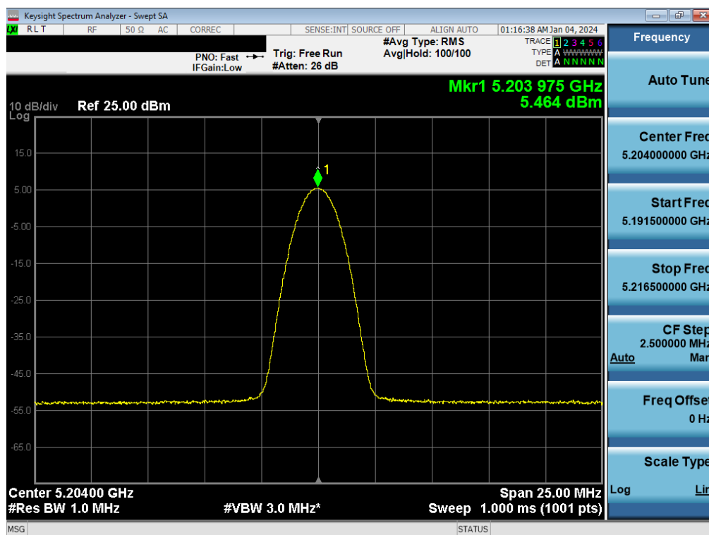
Plot 7-67. FCC PSD TxBF Antenna WF2a (BDR GFSK, ePA – 5204MHz)
