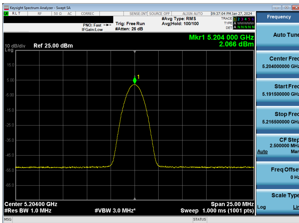
Plot 7-85. ISED PSD TxBF Antenna WF2a (BDR GFSK, iPA – 5204MHz)
