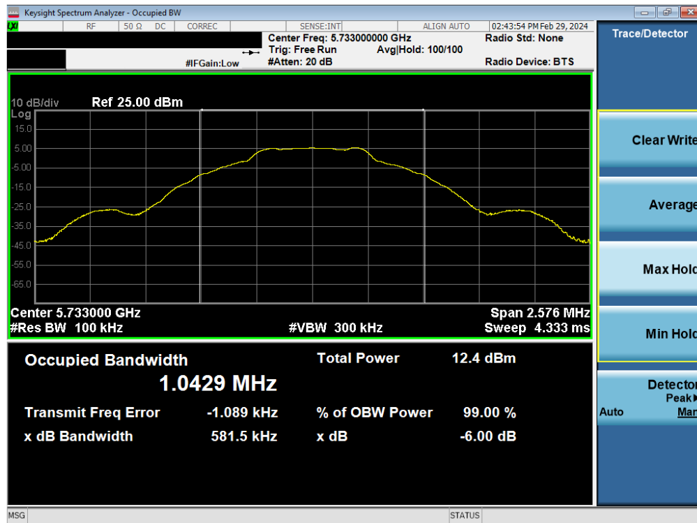
Plot 7-13. 6dB BW & 99% OBW Antenna WF2a (BDR GFSK, ePA 5733MHz)
