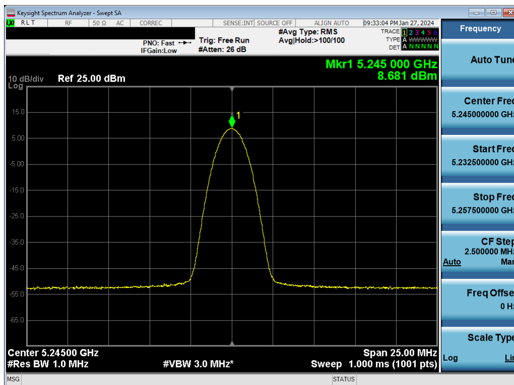
Plot 7-42. ISED PSD Antenna WF2a (BDR GFSK, ePA– 5245MHz)
