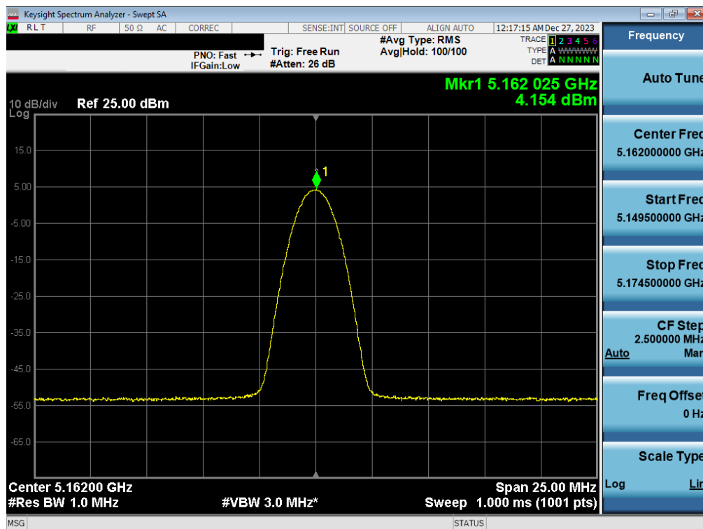
Plot 7-71. FCC PSD TxBF Antenna WF2a (BDR GFSK, iPA – 5162MHz)
