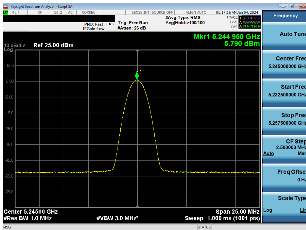
Plot 7-69. FCC PSD TxBF Antenna WF2a (BDR GFSK, ePA- 5245MHz)
