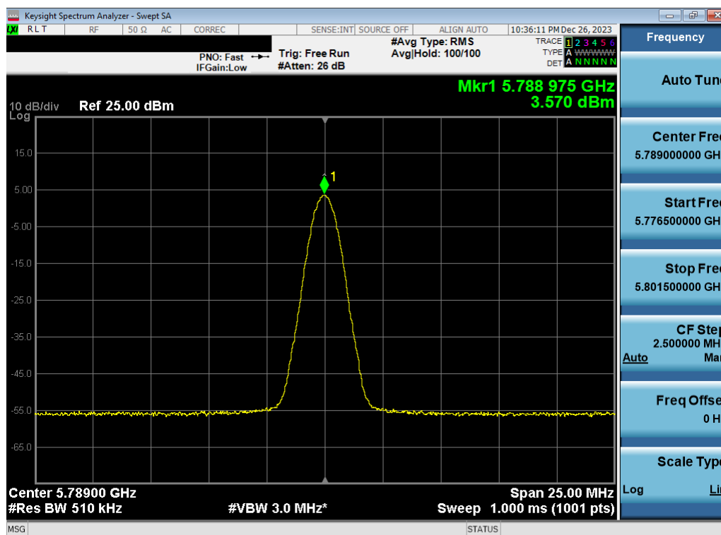
Plot 7-97. PSD TxBF Antenna WF2a (BDR GFSK, iPA 5789MHz)
