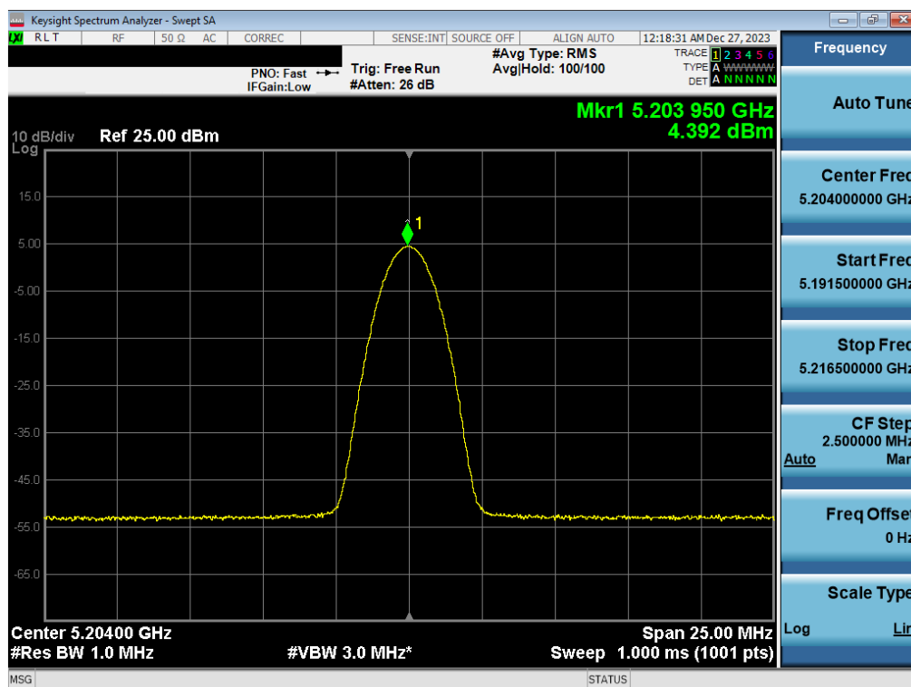
Plot 7-73. FCC PSD TxBF Antenna WF2a (BDR GFSK, iPA – 5204MHz)
