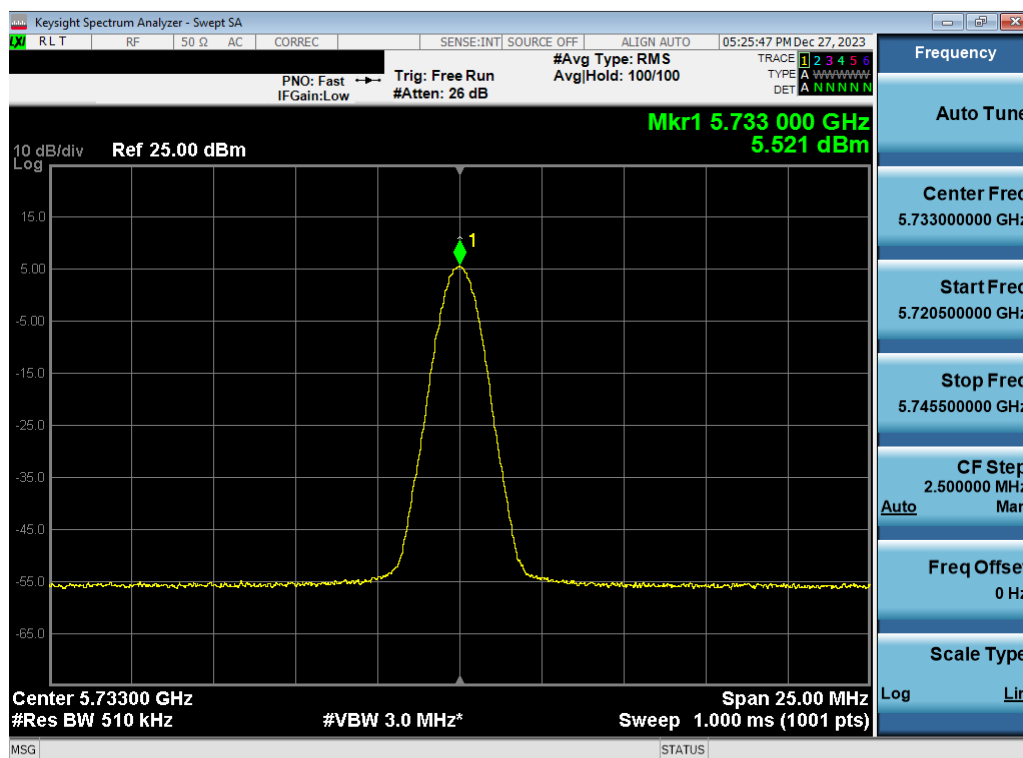
Plot 7-31. PSD Antenna WF7a (BDR GFSK, iPA 5733MHz)
