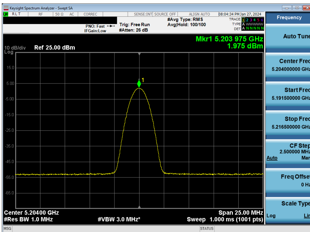
Plot 7-78. ISED PSD TxBF Antenna WF7a (BDR GFSK, ePA – 5204MHz)
