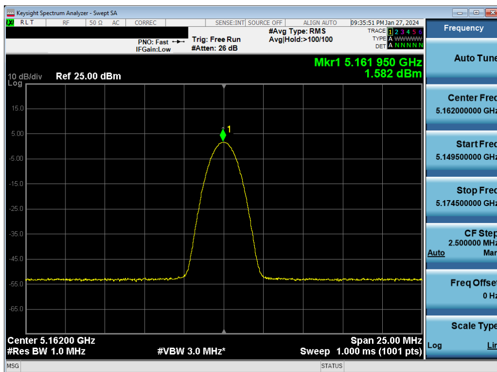
Plot 7-83. ISED PSD TxBF Antenna WF2a (BDR GFSK, iPA – 5162MHz)
