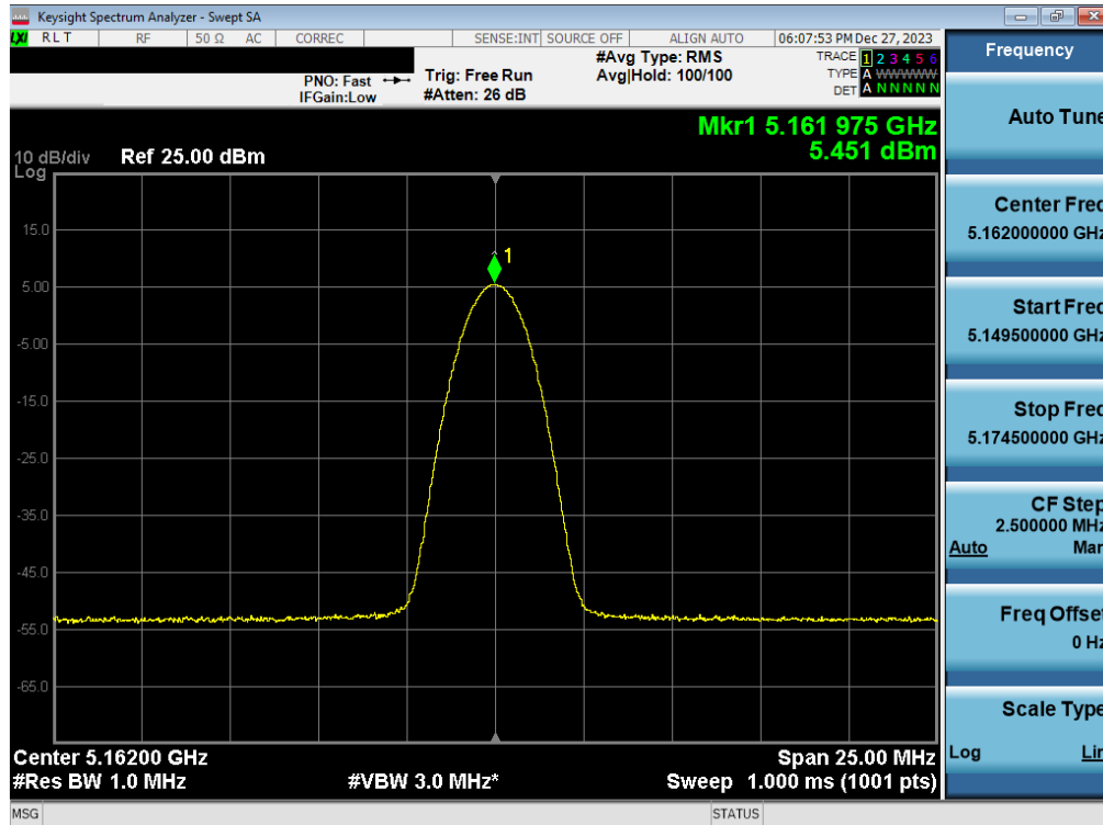
Plot 7-70. FCC PSD TxBF Antenna WF7a (BDR GFSK, iPA – 5162MHz)
