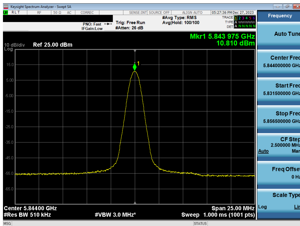
Plot 7-30. PSD Antenna WF7a (BDR GFSK, ePA 5844MHz)
