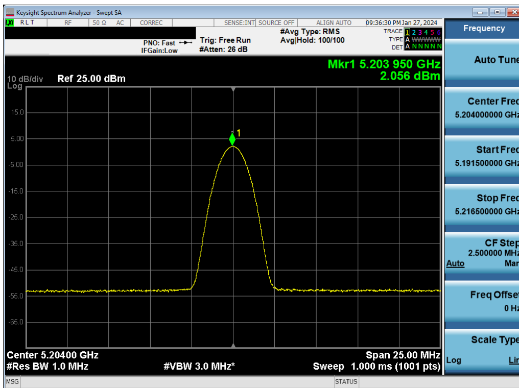
Plot 7-79. ISED PSD TxBF Antenna WF2a (BDR GFSK, ePA – 5204MHz)
