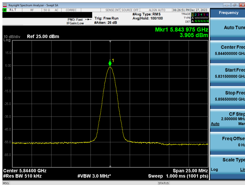
Plot 7-63. PSD Antenna WF7b (BDR GFSK, iPA 5844MHz)
