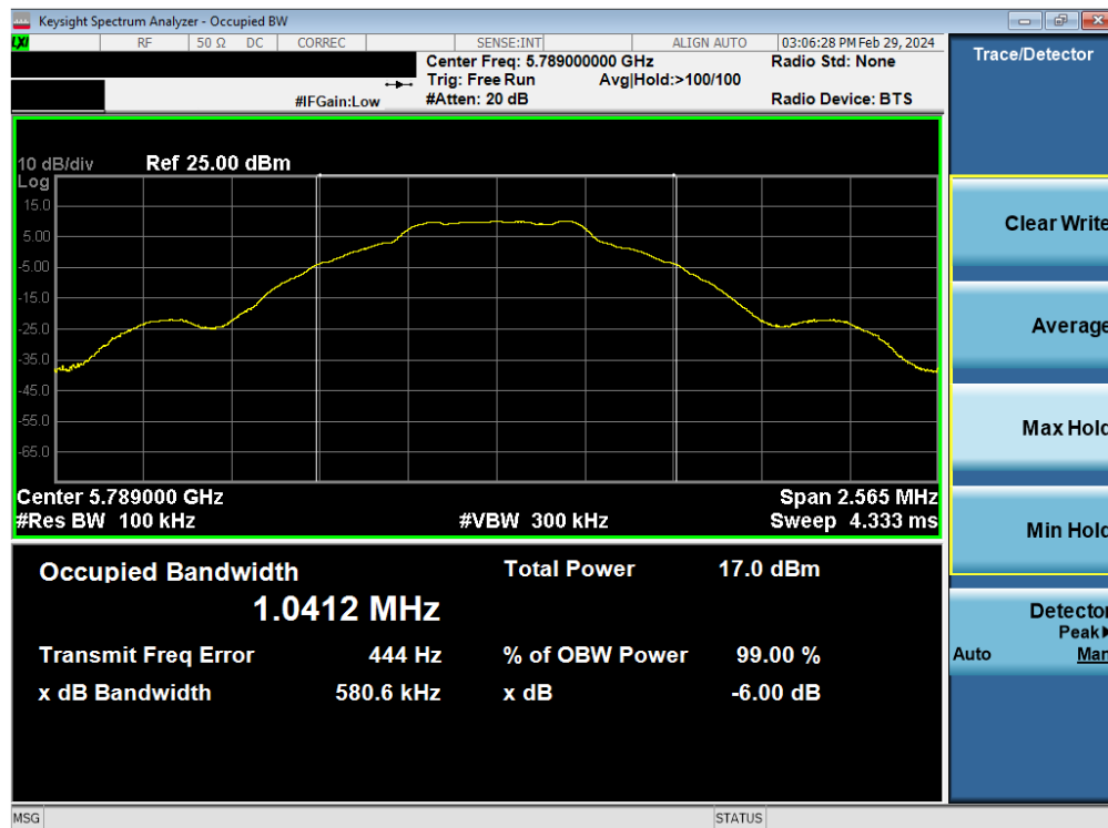
Plot 7-17. 6dB BW & 99% OBW Antenna WF7b (BDR GFSK, ePA 5789MHz)
