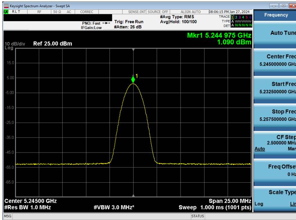
Plot 7-86. ISED PSD TxBF Antenna WF7a (BDR GFSK, iPA- 5245MHz)
