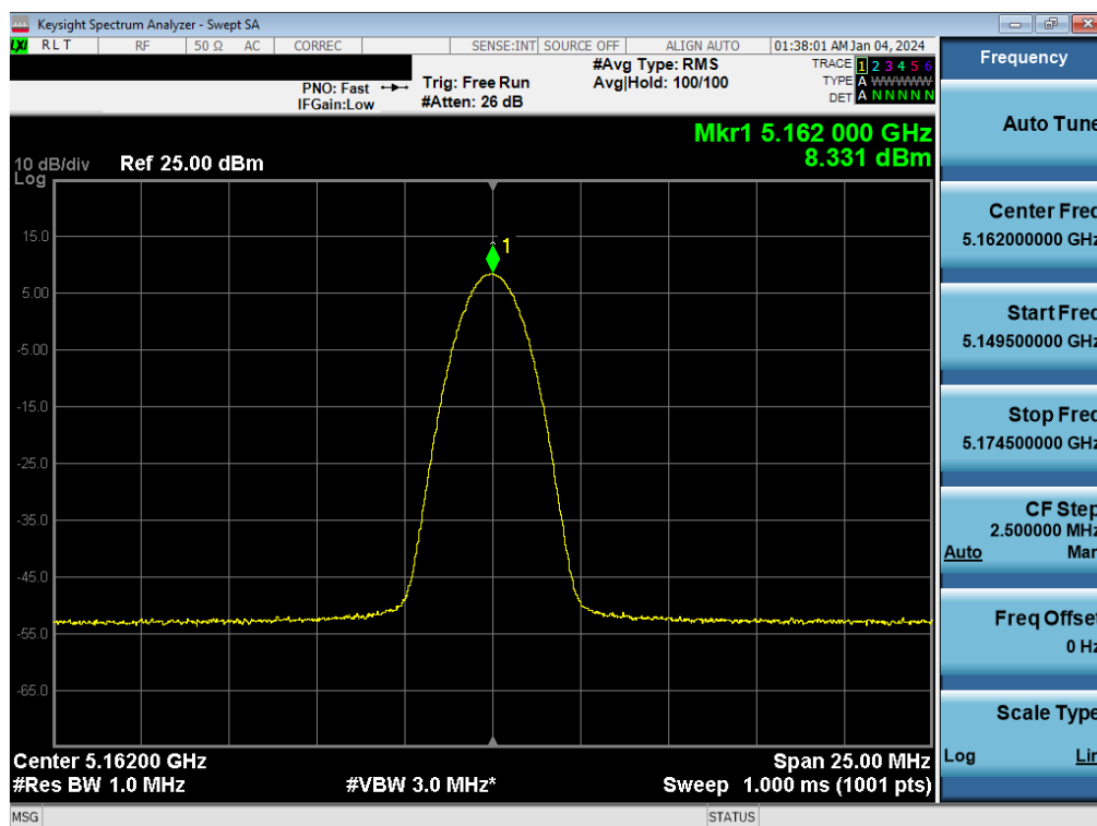
Plot 7-19. FCC PSD Antenna WF7a (BDR GFSK, ePA – 5162MHz)
