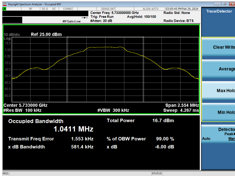
Plot 7-16. 6dB BW & 99% OBW Antenna WF7b (BDR GFSK, ePA 5733MHz)
