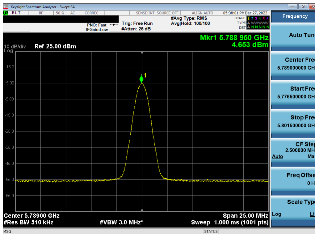
Plot 7-96. PSD TxBF Antenna WF7a (BDR GFSK, iPA 5789MHz)
