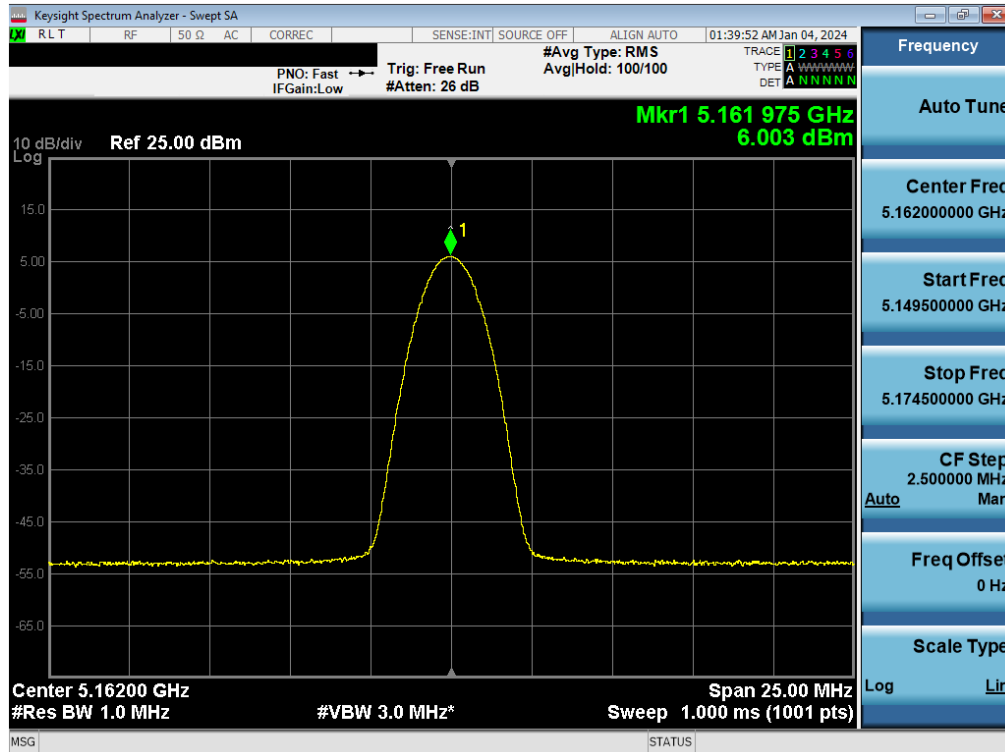
Plot 7-64. FCC PSD TxBF Antenna WF7a (BDR GFSK, ePA – 5162MHz)
