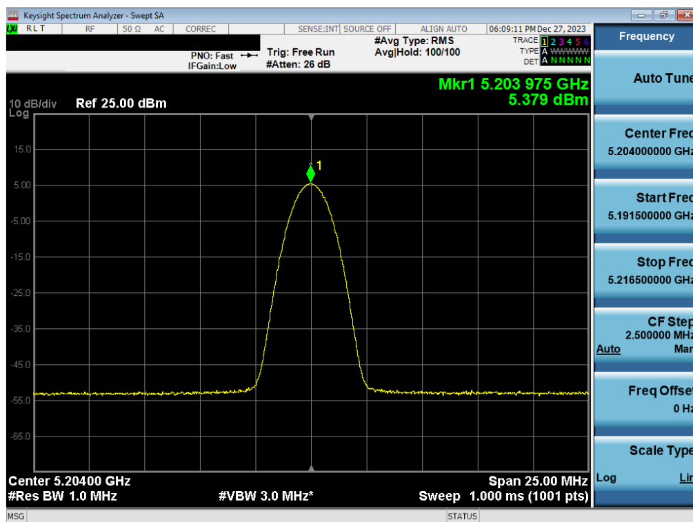
Plot 7-72. FCC PSD TxBF Antenna WF7a (BDR GFSK, iPA – 5204MHz)
