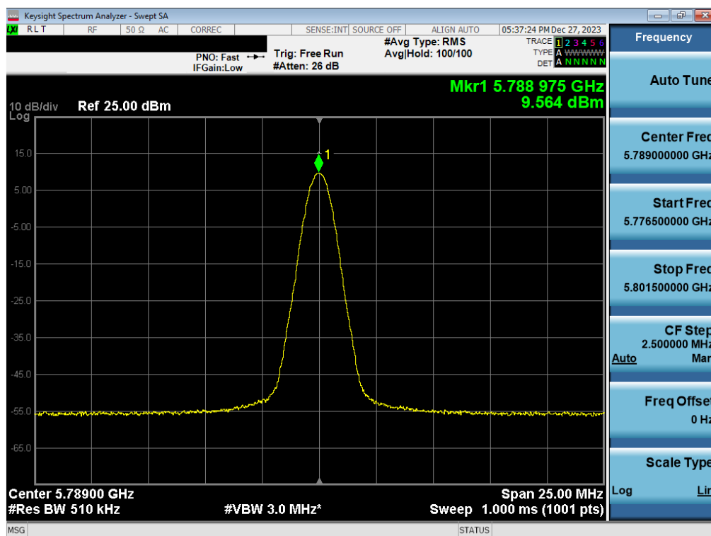
Plot 7-90. PSD TxBF Antenna WF7a (BDR GFSK, ePA 5789MHz)
