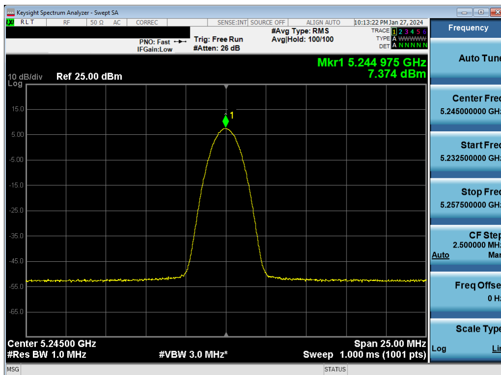
Plot 7-57. ISED PSD Antenna WF7b (BDR GFSK, ePA– 5245MHz)
