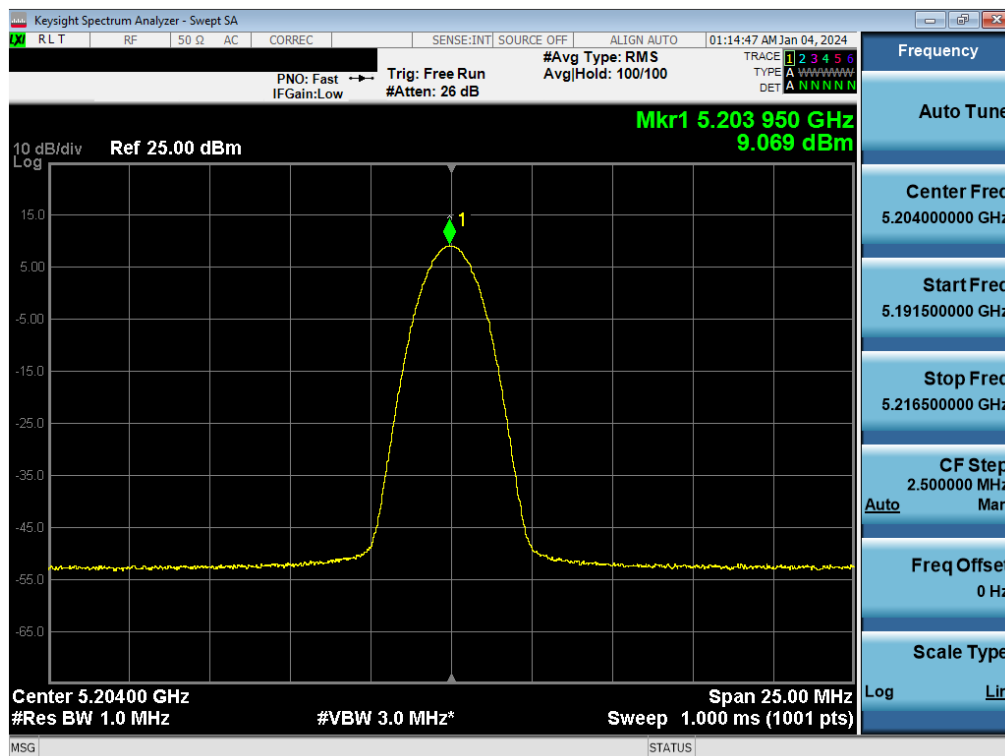
Plot 7-35. FCC PSD Antenna WF2a (BDR GFSK, ePA – 5204MHz)
