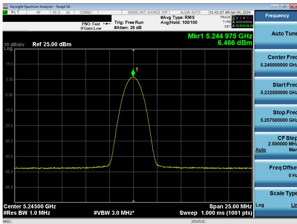
Plot 7-68. FCC PSD TxBF Antenna WF7a (BDR GFSK, ePA- 5245MHz)
