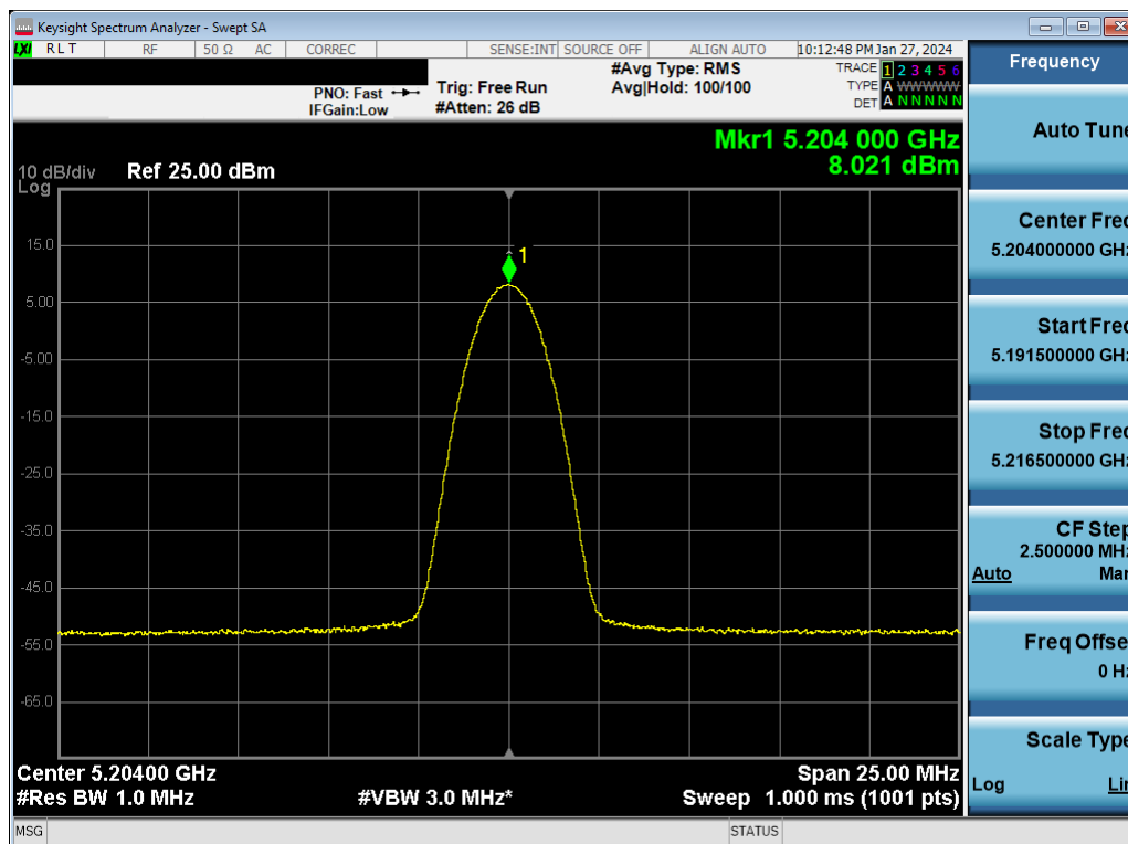
Plot 7-56. ISED PSD Antenna WF7b (BDR GFSK, ePA – 5204MHz)
