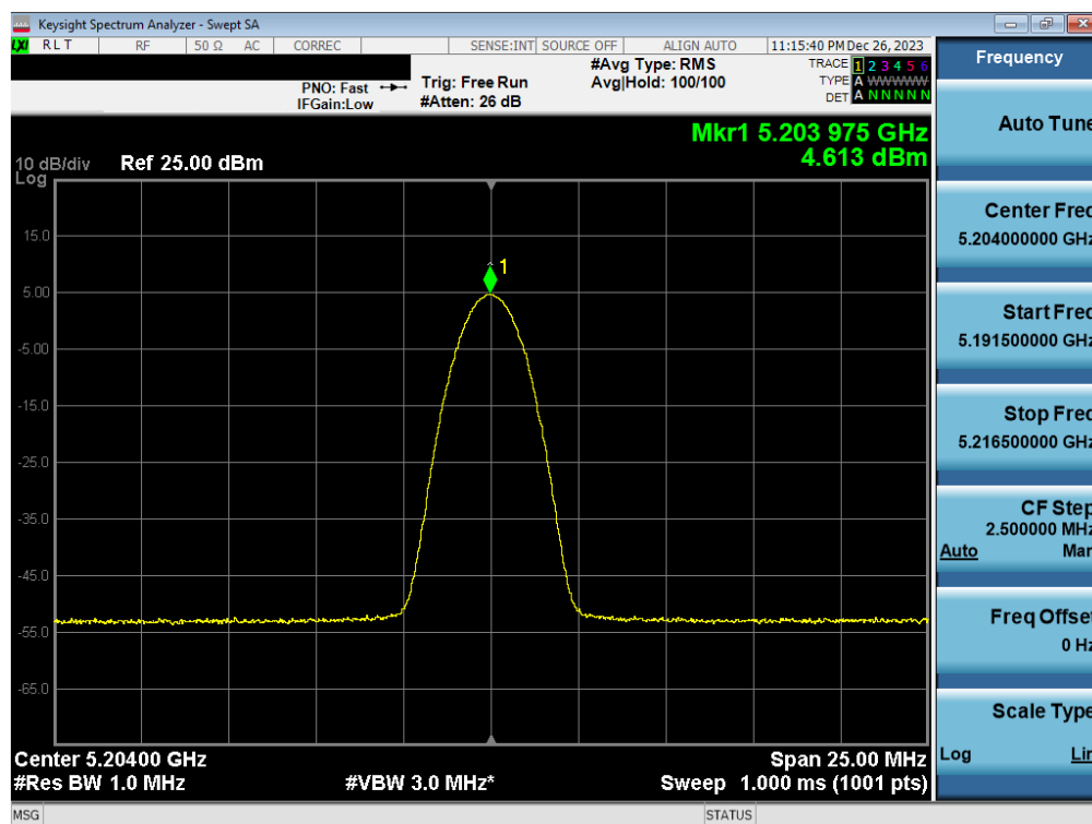
Plot 7-53. FCC/ISED PSD Antenna WF7b (BDR GFSK, iPA – 5204MHz)
