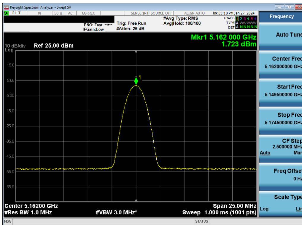
Plot 7-77. ISED PSD TxBF Antenna WF2a (BDR GFSK, ePA – 5162MHz)
