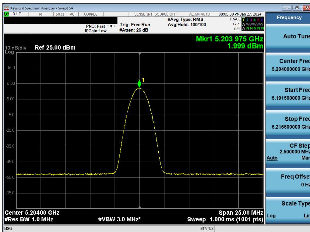
Plot 7-84. ISED PSD TxBF Antenna WF7a (BDR GFSK, iPA – 5204MHz)
