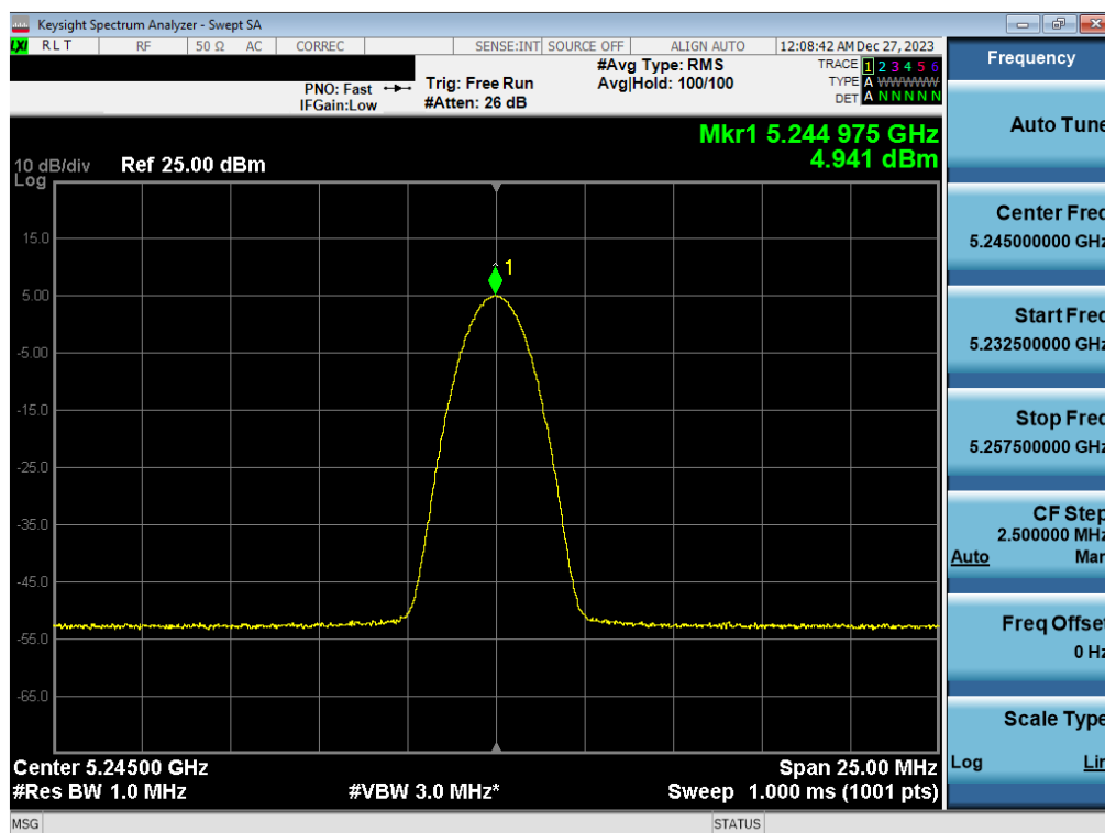
Plot 7-39. FCC/ISED PSD Antenna WF2a (BDR GFSK, iPA– 5245MHz)
