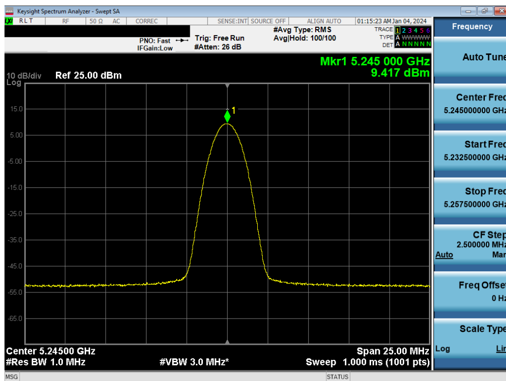
Plot 7-36. FCC PSD Antenna WF2a (BDR GFSK, ePA– 5245MHz)
