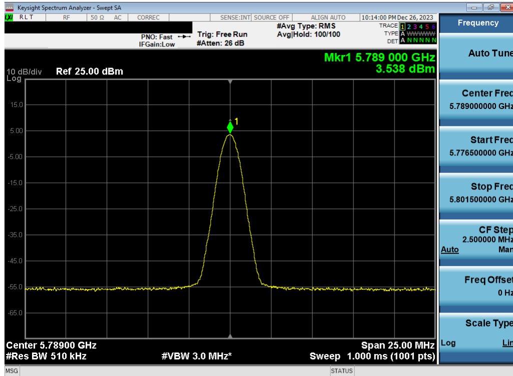
Plot 7-47. PSD Antenna WF2a (BDR GFSK, iPA 5789MHz)
