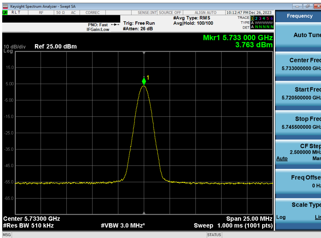
Plot 7-46. PSD Antenna WF2a (BDR GFSK, iPA 5733MHz)
