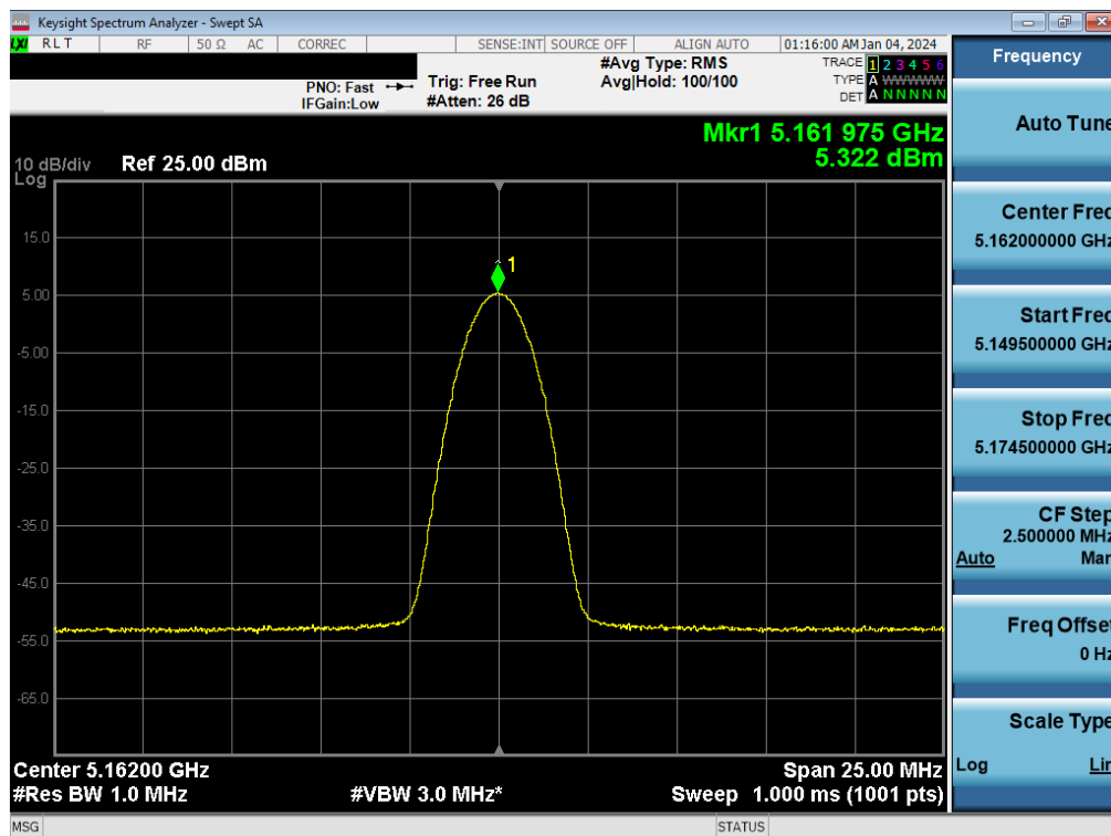
Plot 7-65. FCC PSD TxBF Antenna WF2a (BDR GFSK, ePA – 5162MHz)
