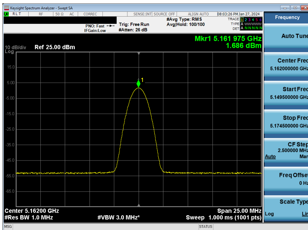
Plot 7-76. ISED PSD TxBF Antenna WF7a (BDR GFSK, ePA – 5162MHz)
