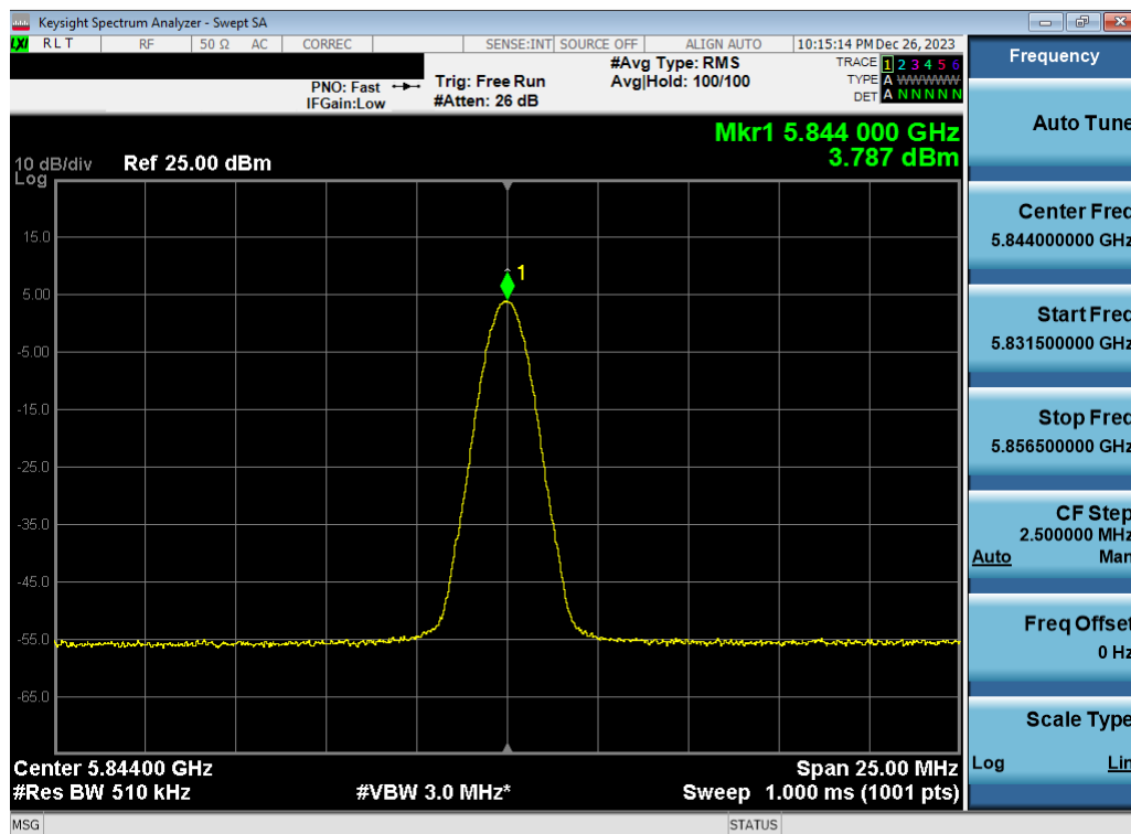
Plot 7-48. PSD Antenna WF2a (BDR GFSK, iPA 5844MHz)
