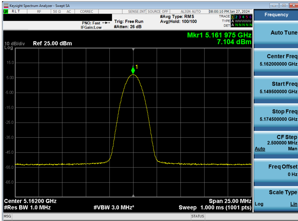
Plot 7-25. ISED PSD Antenna WF7a (BDR GFSK, ePA – 5162MHz)
