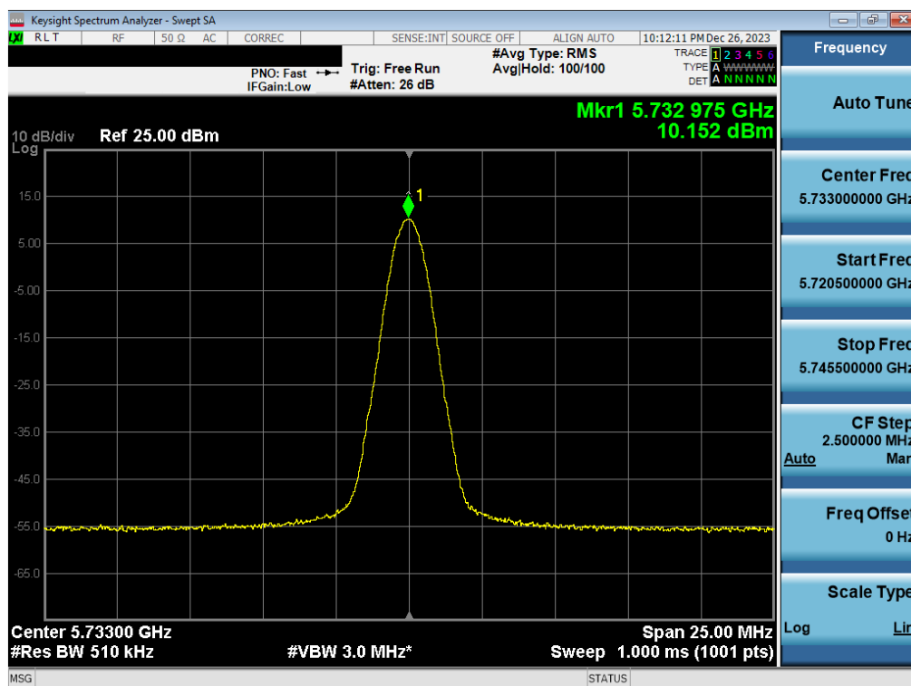
Plot 7-43. PSD Antenna WF2a (BDR GFSK, ePA 5733MHz)
