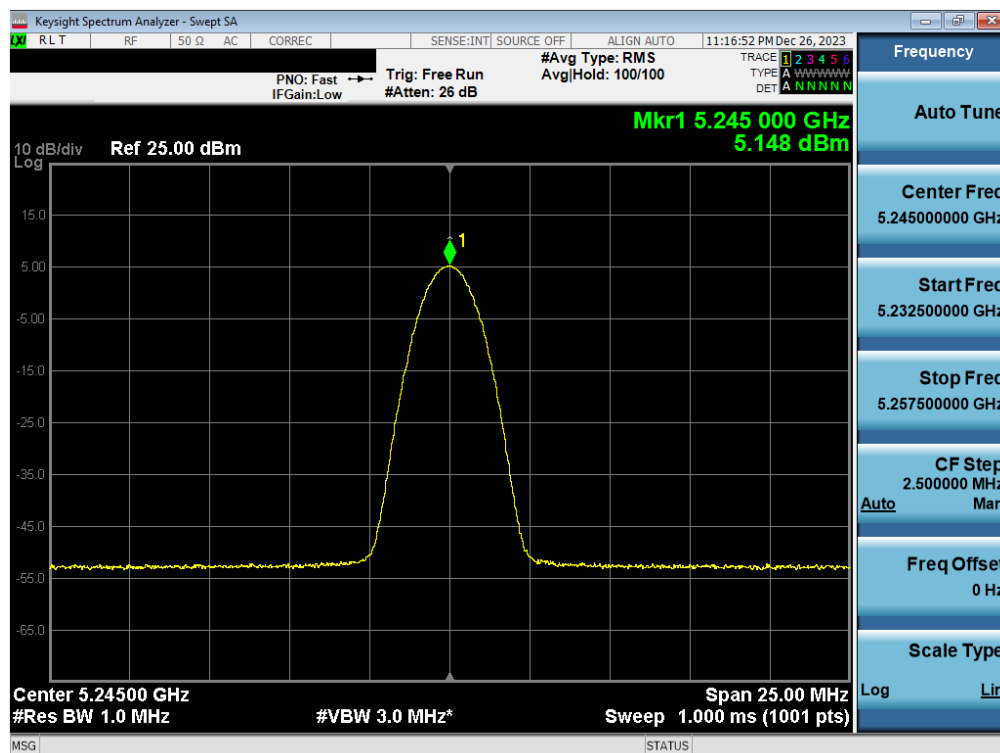
Plot 7-54. FCC/ISED PSD Antenna WF7b (BDR GFSK, iPA– 5245MHz)
