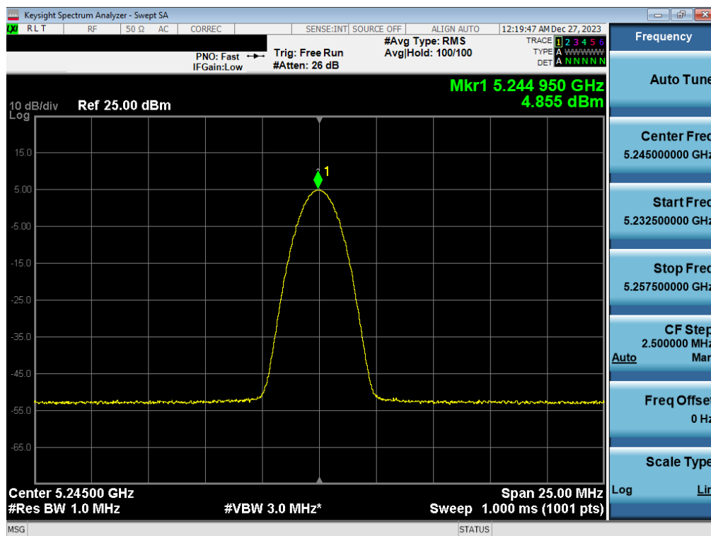
Plot 7-75. FCC PSD TxBF Antenna WF2a (BDR GFSK, iPA- 5245MHz)
