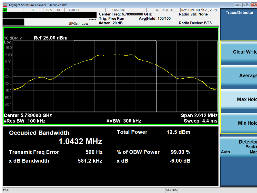
Plot 7-14. 6dB BW & 99% OBW Antenna WF2a (BDR GFSK, ePA 5789MHz)
