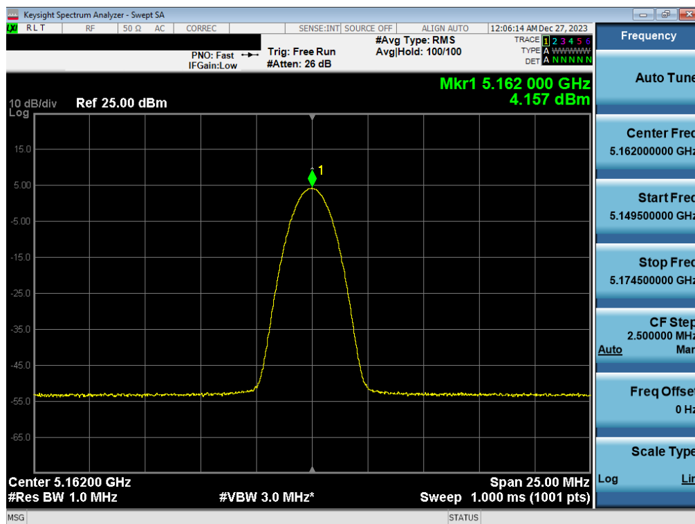
Plot 7-37. FCC/ISED PSD Antenna WF2a (BDR GFSK, iPA – 5162MHz)
