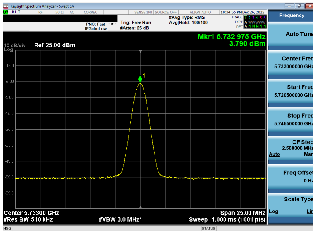
Plot 7-95. PSD TxBF Antenna WF2a (BDR GFSK, iPA 5733MHz)
