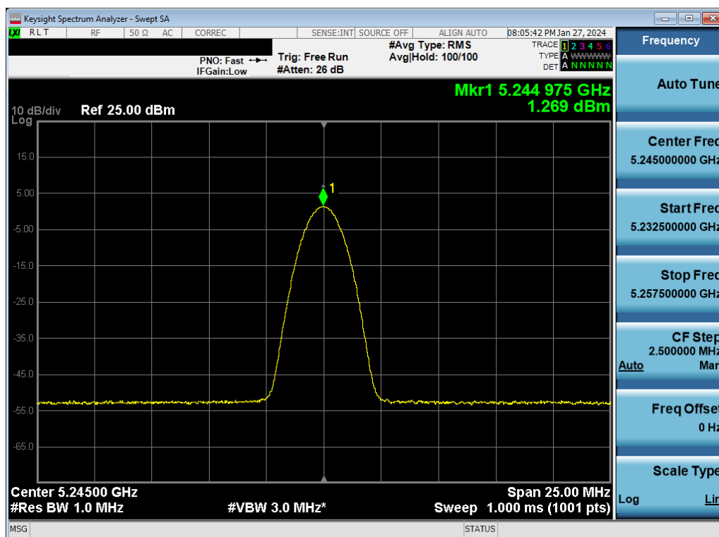
Plot 7-80. ISED PSD TxBF Antenna WF7a (BDR GFSK, ePA- 5245MHz)
