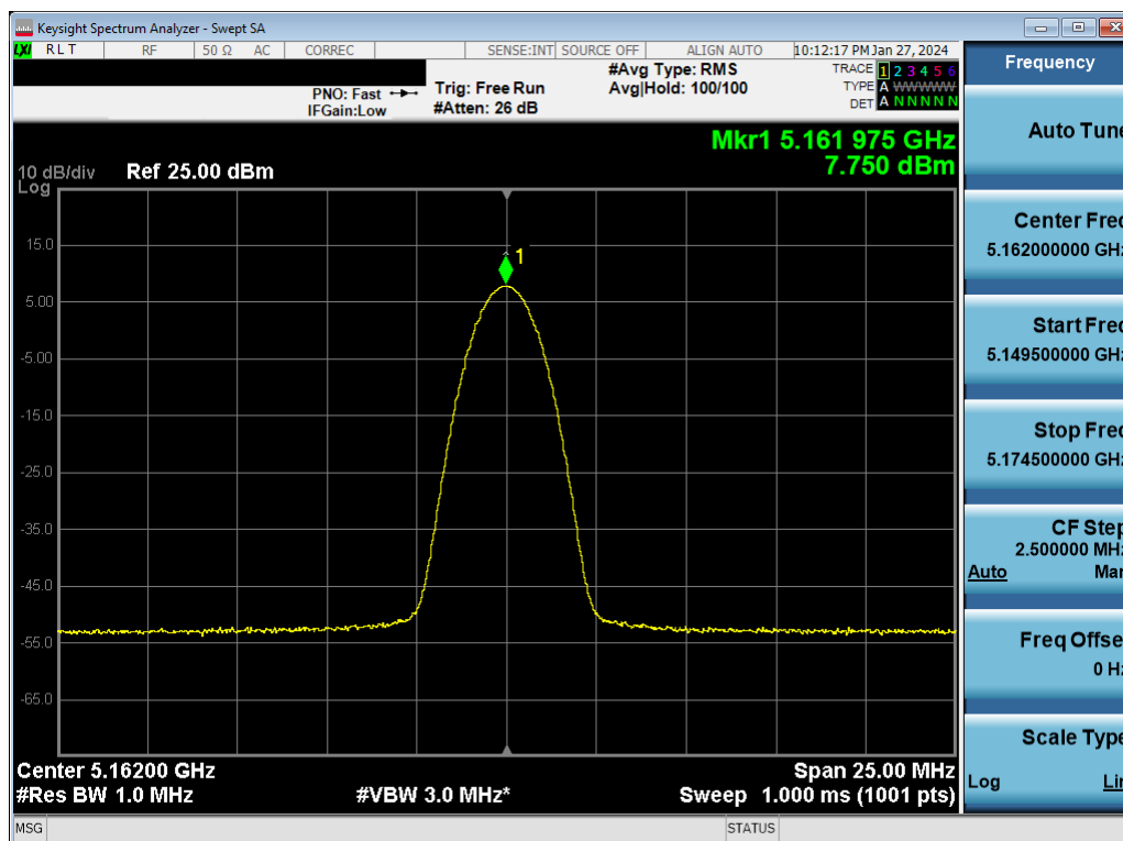
Plot 7-55. ISED PSD Antenna WF7b (BDR GFSK, ePA – 5162MHz)
