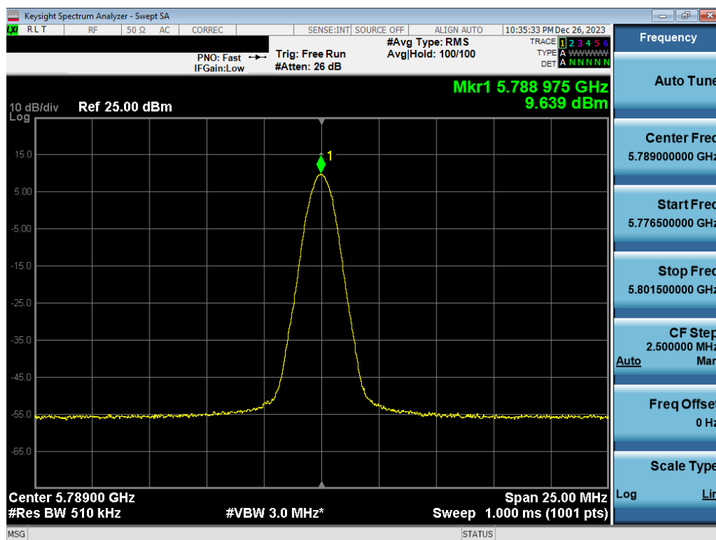
Plot 7-91. PSD TxBF Antenna WF2a (BDR GFSK, ePA 5789MHz)
