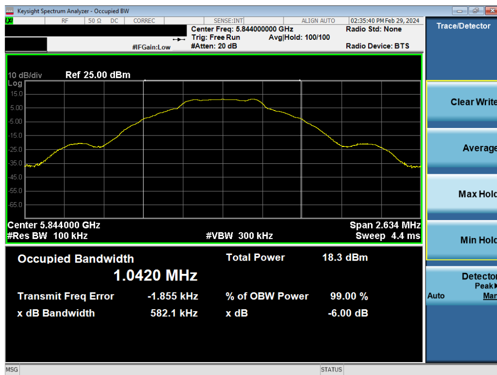
Plot 7-12. 6dB BW & 99% OBW Antenna WF7a (BDR GFSK, ePA 5844MHz)
