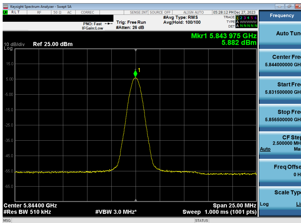
Plot 7-33. PSD Antenna WF7a (BDR GFSK, iPa 5844MHz)
