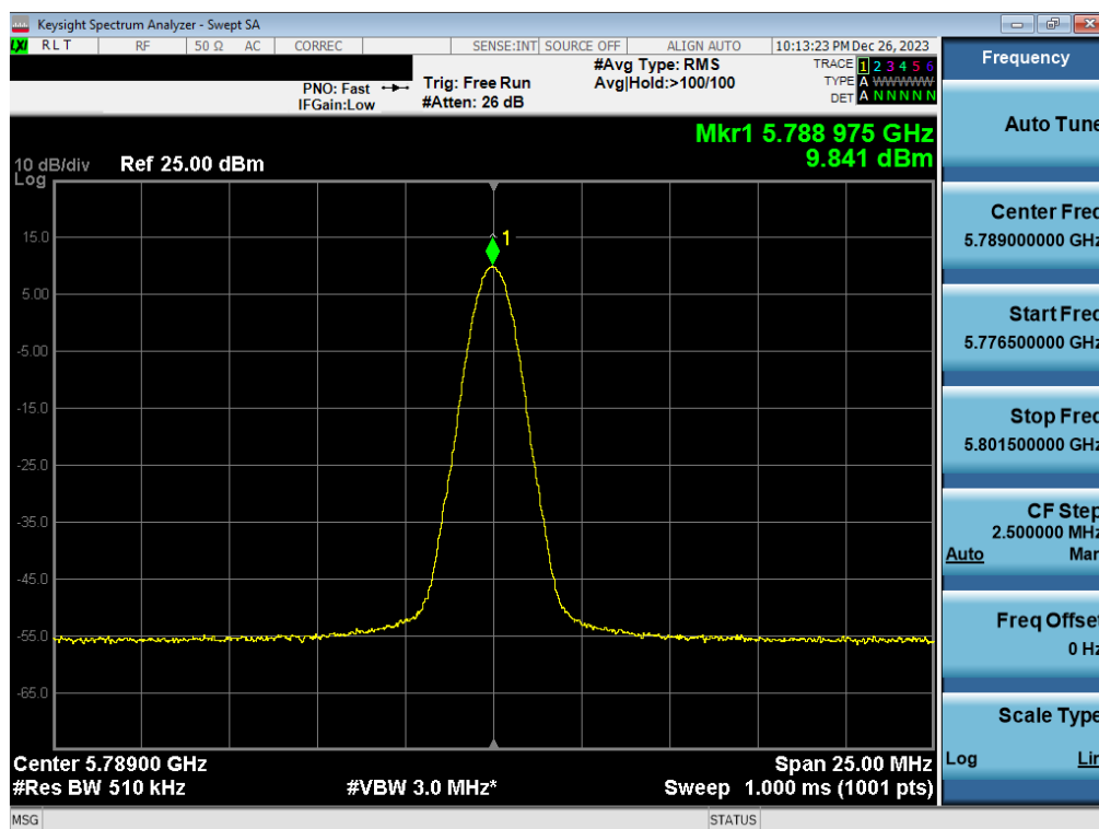
Plot 7-44. PSD Antenna WF2a (BDR GFSK, ePA 5789MHz)
