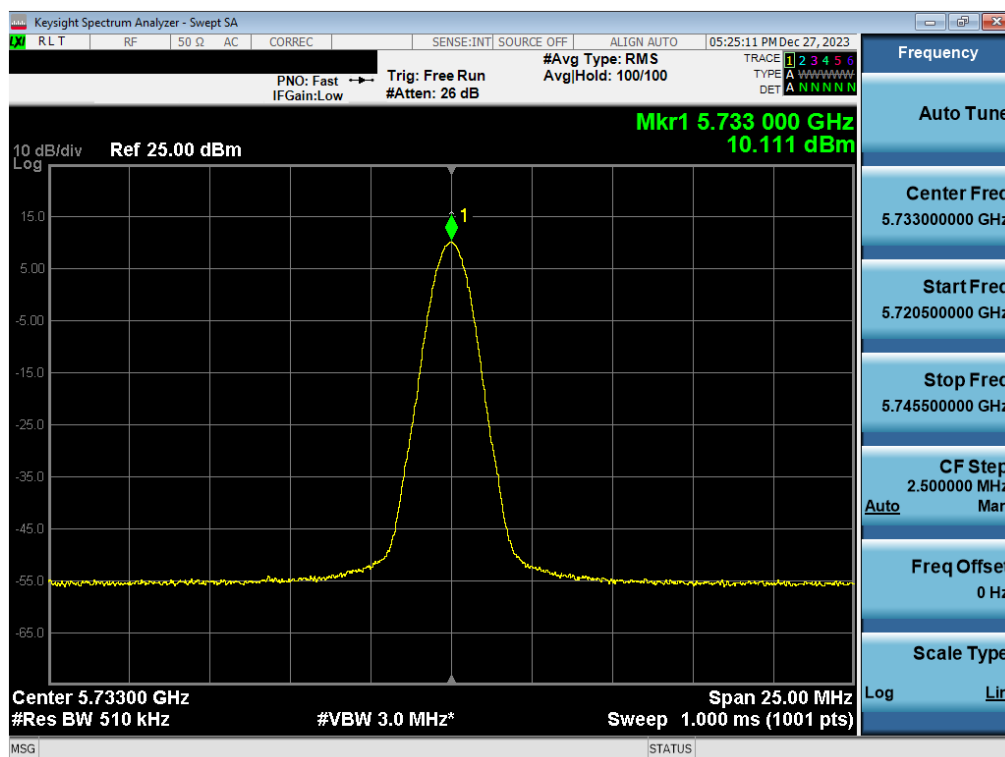
Plot 7-28. PSD Antenna WF7a (BDR GFSK, ePA 5733MHz)
