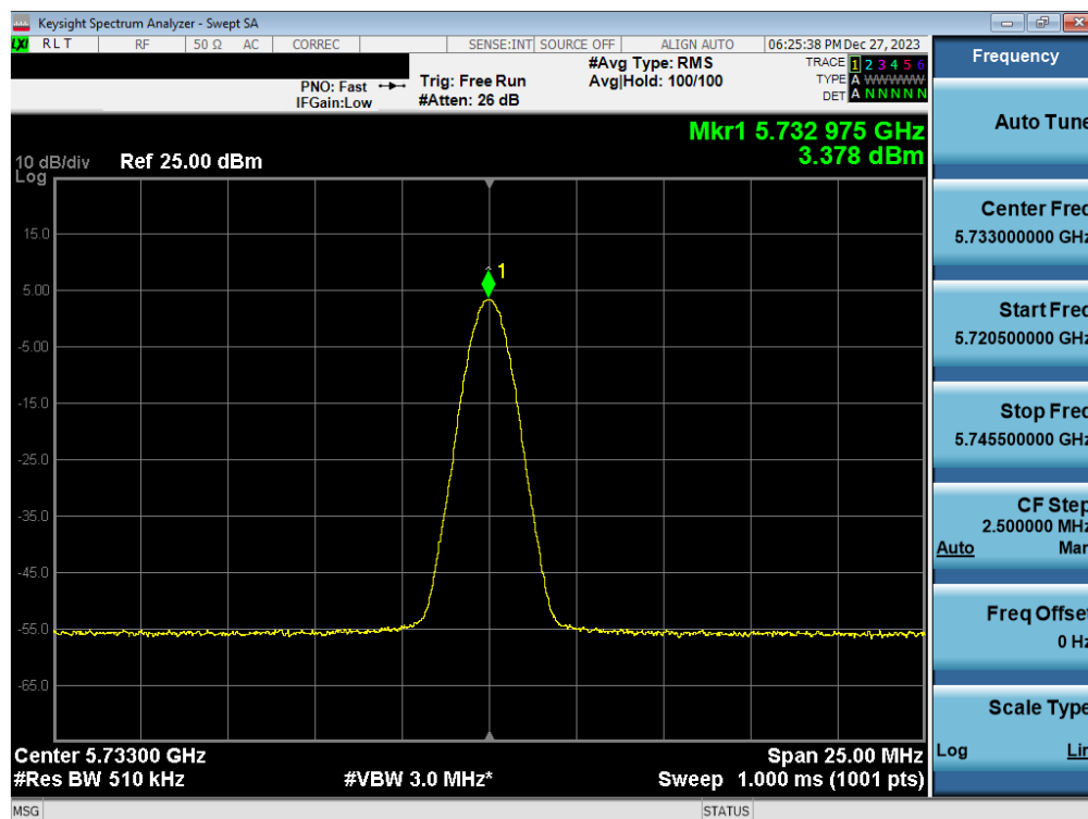
Plot 7-61. PSD Antenna WF7b (BDR GFSK, iPA 5733MHz)
