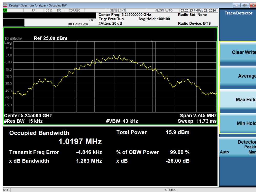
Plot 7-9. 26dB BW & 99% OBW Antenna WF7b (BDR GFSK- 5245MHz)
