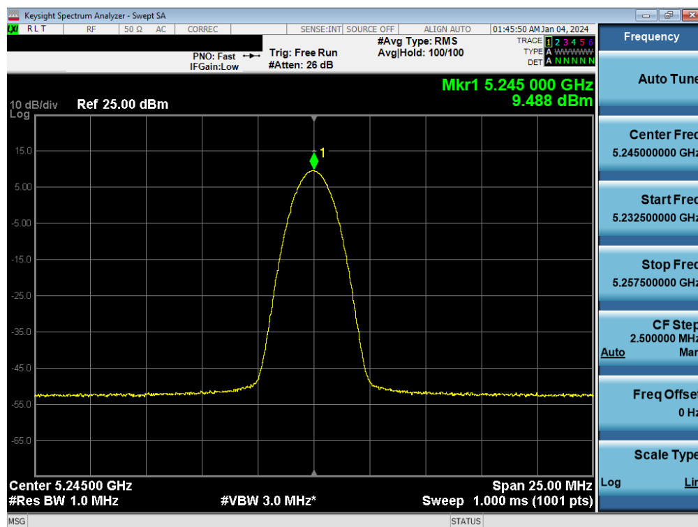
Plot 7-51. FCC PSD Antenna WF7b (BDR GFSK, ePA- 5245MHz)
