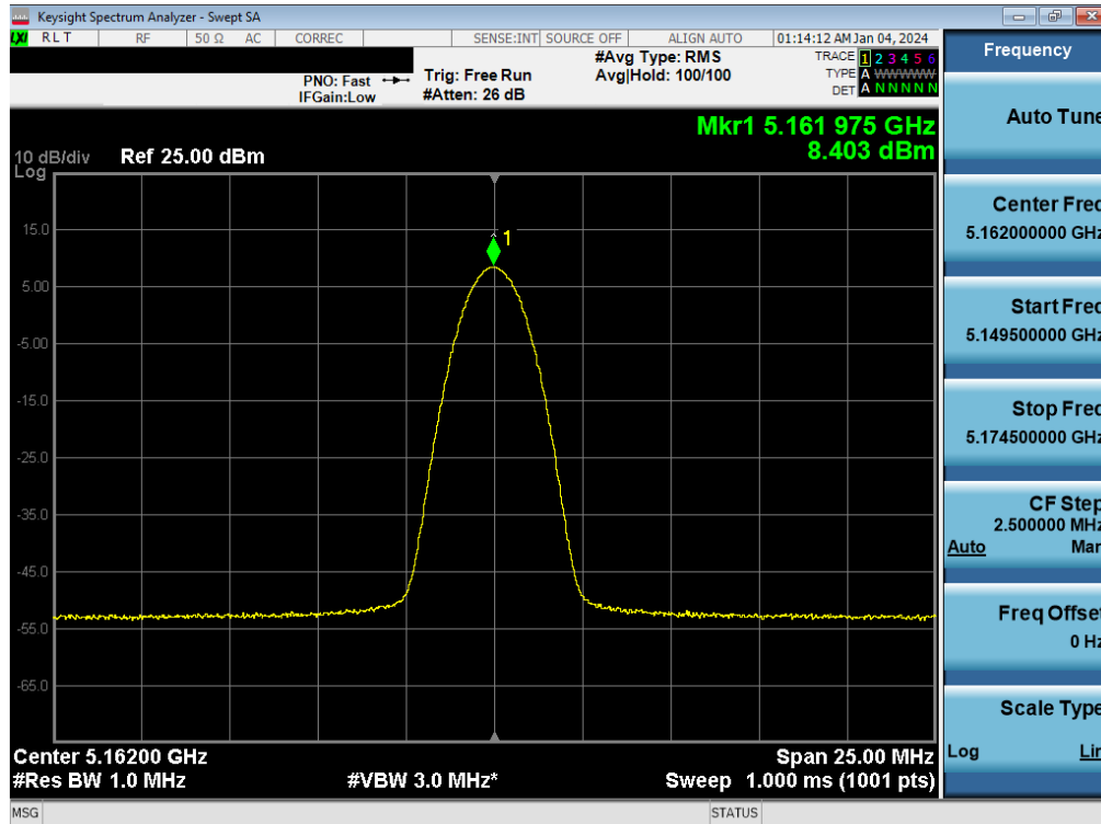
Plot 7-34. FCC PSD Antenna WF2a (BDR GFSK, ePA – 5162MHz)
