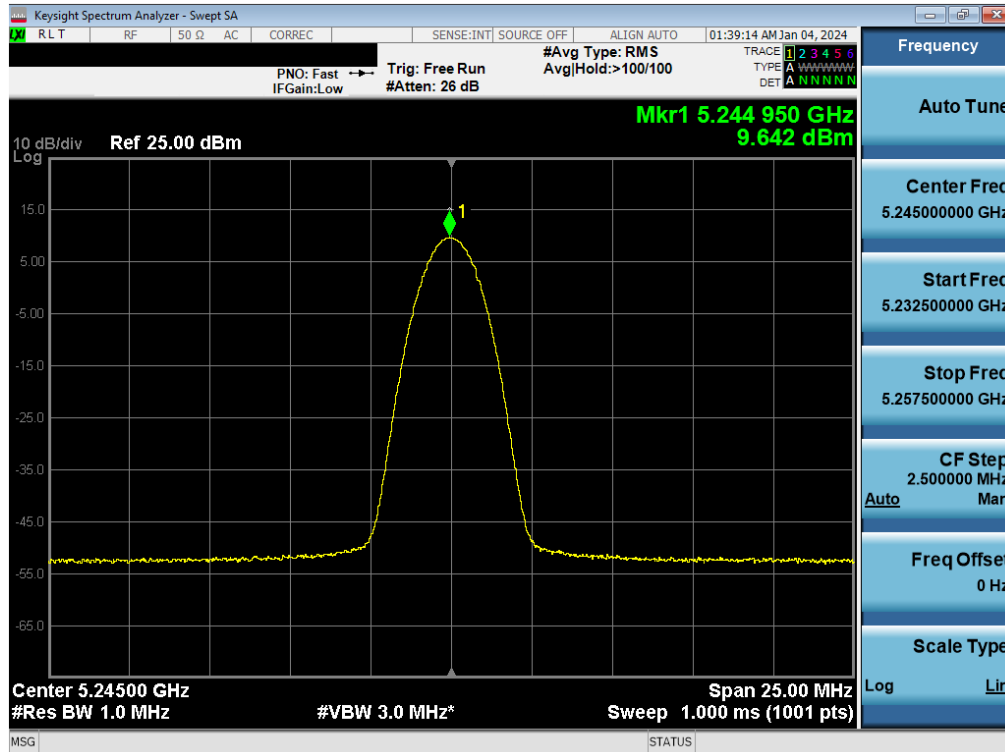
Plot 7-21. FCC PSD Antenna WF7a (BDR GFSK, ePA– 5245MHz)
