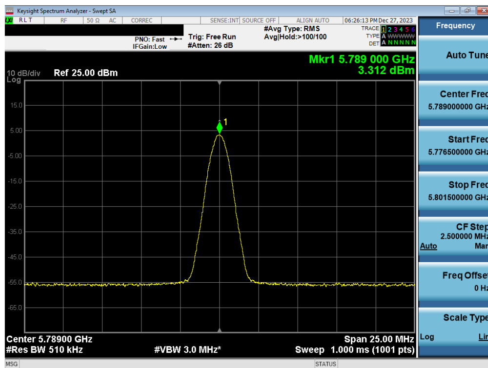
Plot 7-62. PSD Antenna WF7b (BDR GFSK, iPA 5789MHz)
