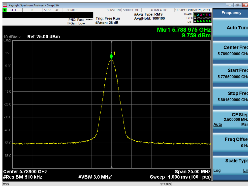
Plot 7-59. PSD Antenna WF7b (BDR GFSK, ePA 5789MHz)
