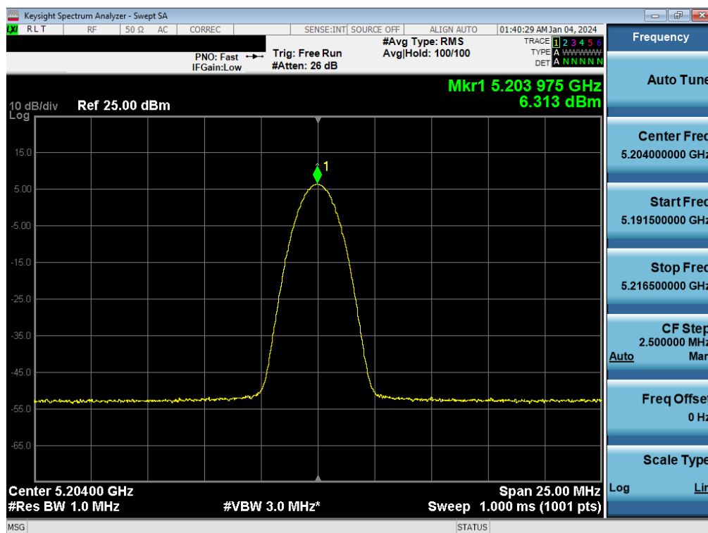
Plot 7-66. FCC PSD TxBF Antenna WF7a (BDR GFSK, ePA – 5204MHz)
