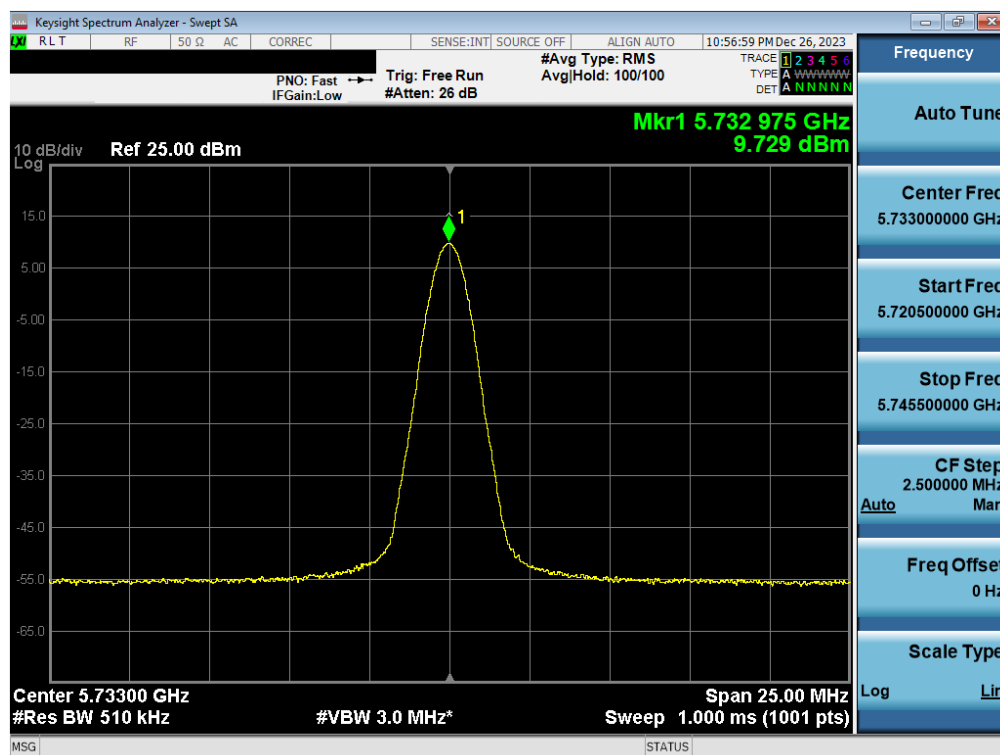
Plot 7-58. PSD Antenna WF7b (BDR GFSK, ePA 5733MHz)
