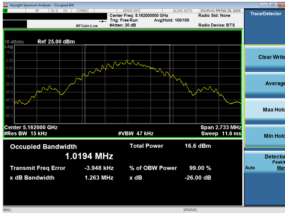
Plot 7-1. 26dB BW & 99% OBW Antenna WF7a (BDR GFSK, ePA– 5162MHz)
