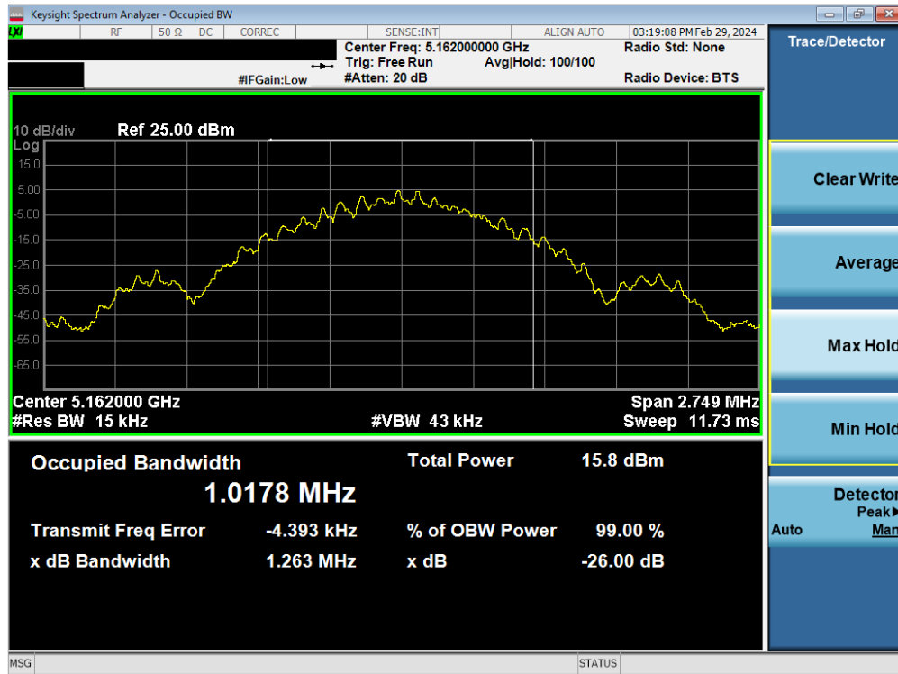
Plot 7-7. 26dB BW & 99% OBW Antenna WF7b (BDR GFSK, ePA- 5162MHz)
