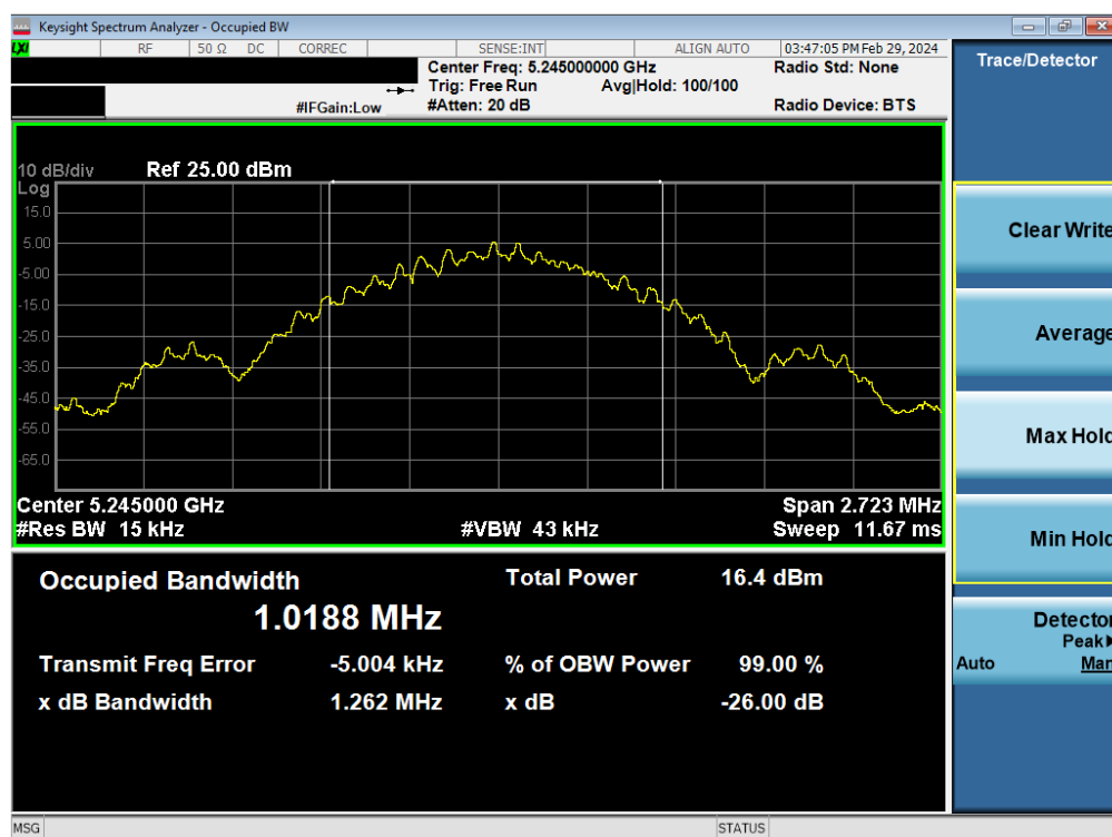
Plot 7-3. 26dB BW & 99% OBW Antenna WF7a (BDR GFSK- 5245MHz)
