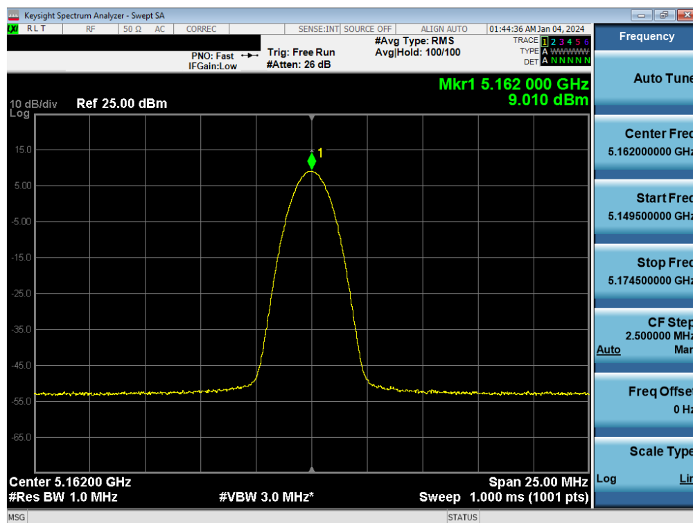
Plot 7-49. FCC PSD Antenna WF7b (BDR GFSK, ePA – 5162MHz)
