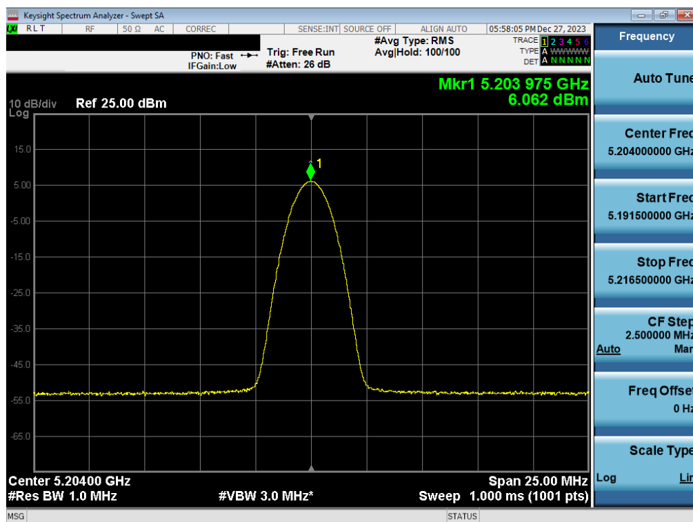
Plot 7-23. FCC/ISED PSD Antenna WF7a (BDR GFSK, iPA – 5204MHz)
