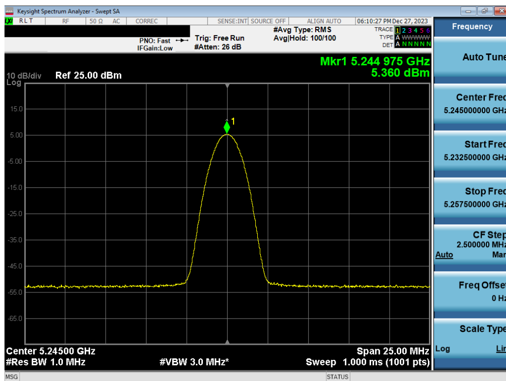
Plot 7-74. FCC PSD TxBF Antenna WF7a (BDR GFSK, iPA- 5245MHz)
