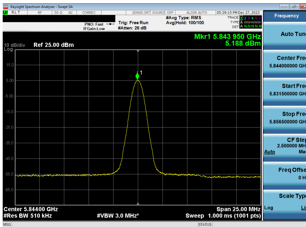
Plot 7-98. PSD TxBF Antenna WF7a (BDR GFSK, iPA 5844MHz)
