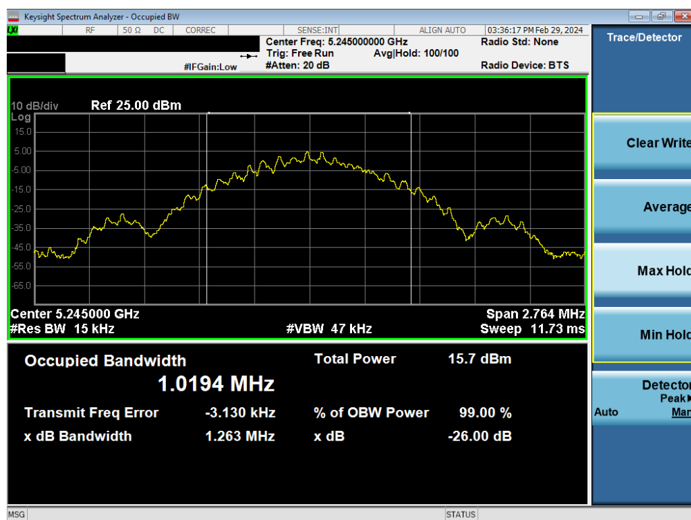
Plot 7-6. 26dB BW & 99% OBW Antenna WF2a (BDR GFSK– 5245MHz)
