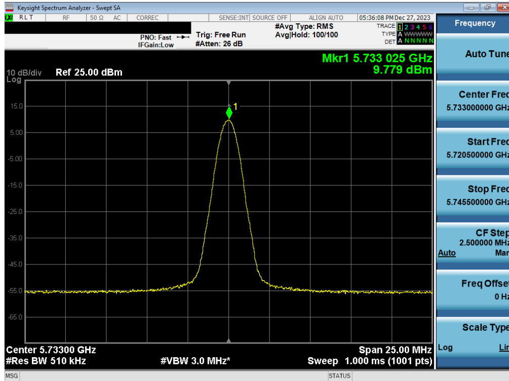
Plot 7-88. PSD TxBF Antenna WF7a (BDR GFSK, ePA 5733MHz)
