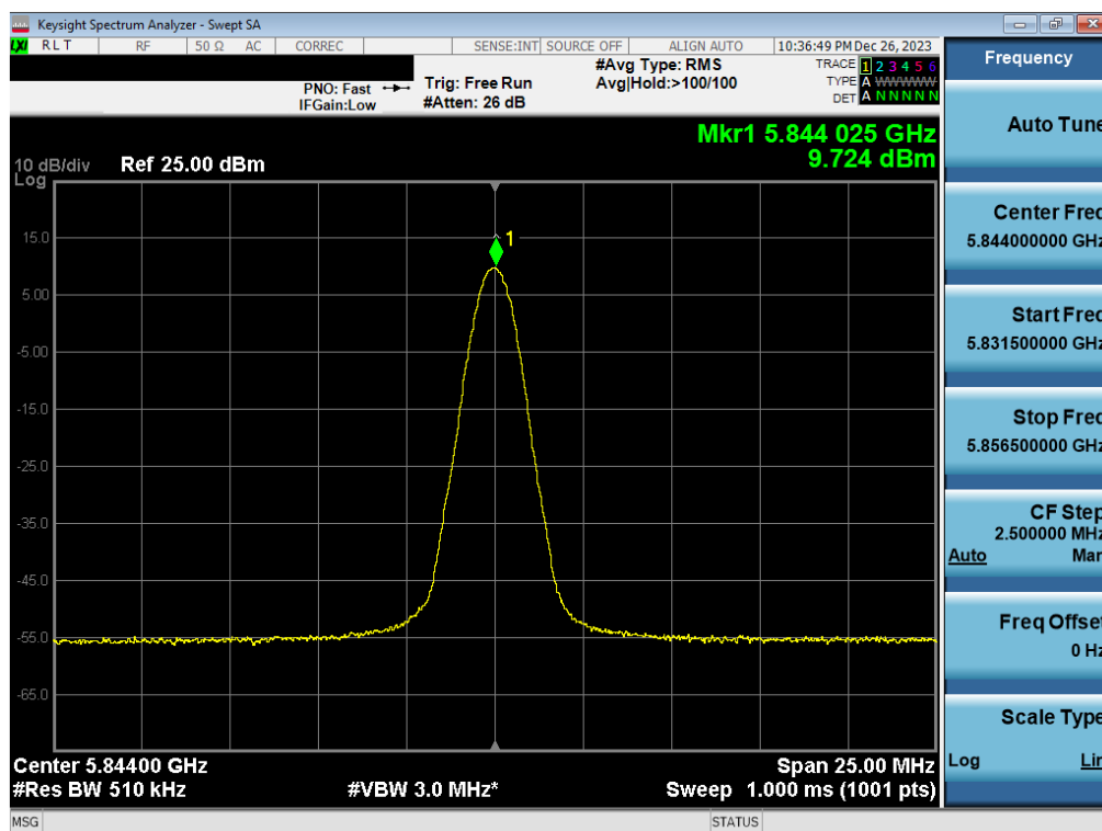
Plot 7-93. PSD TxBF Antenna WF2a (BDR GFSK, ePA 5844MHz)
