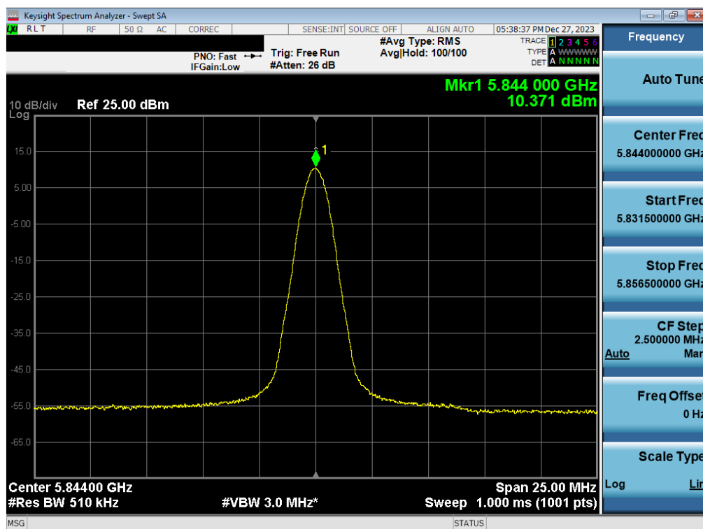
Plot 7-92. PSD TxBF Antenna WF7a (BDR GFSK, ePA 5844MHz)
