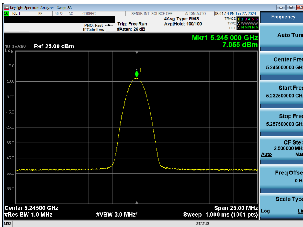
Plot 7-27. ISED PSD Antenna WF7a (BDR GFSK, ePA– 5245MHz)
