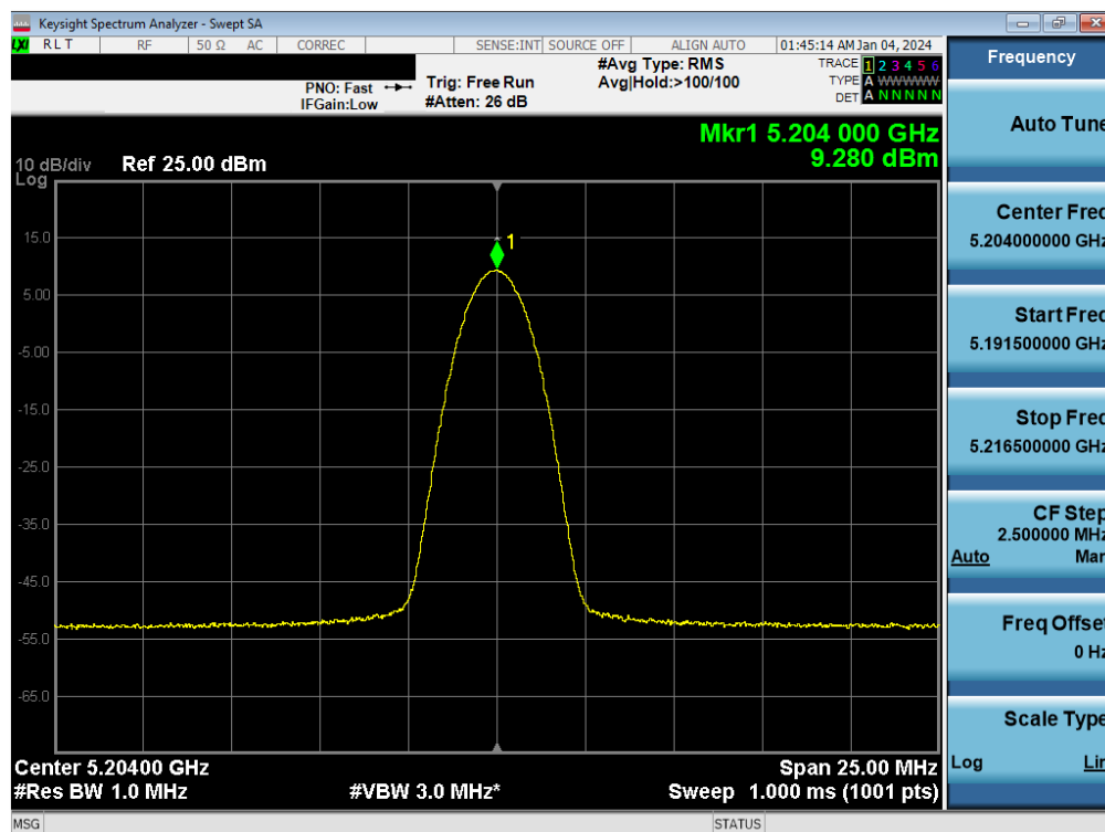
Plot 7-50. FCC PSD Antenna WF7b (BDR GFSK, ePA – 5204MHz)
