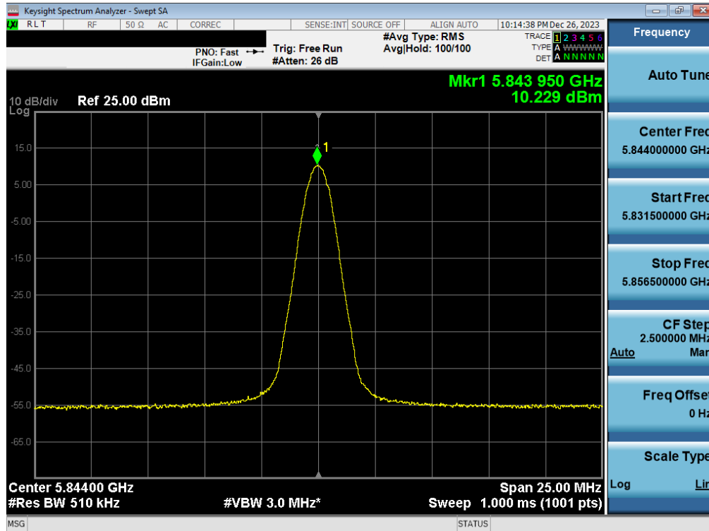
Plot 7-45. PSD Antenna WF2a (BDR GFSK, ePA 5844MHz)
