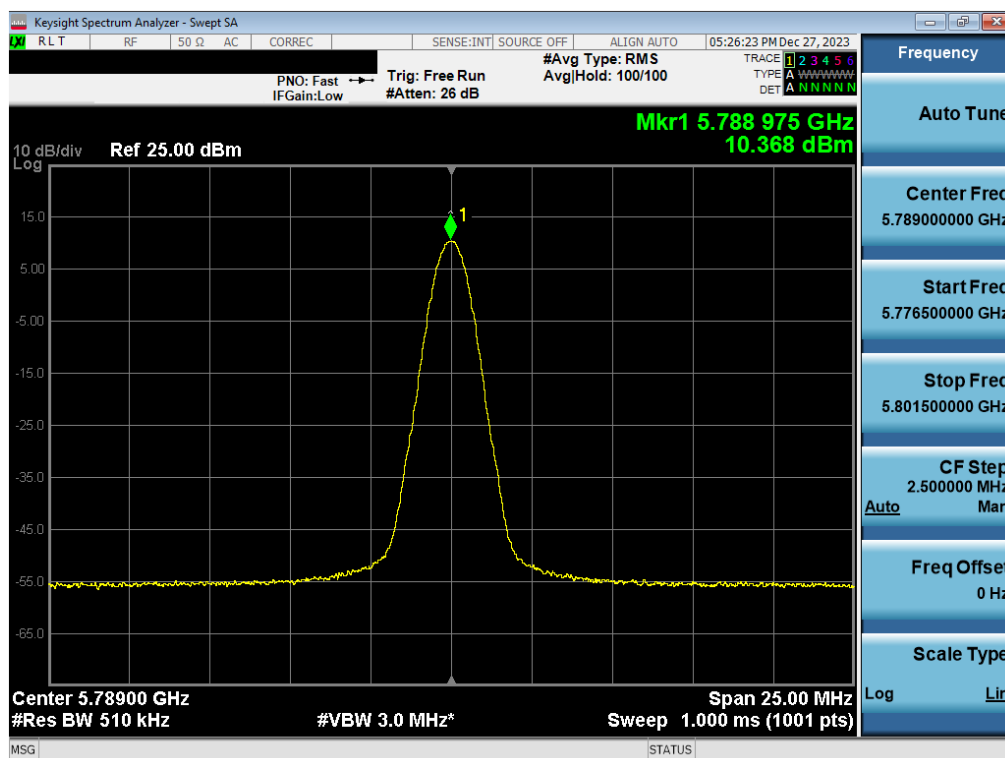
Plot 7-29. PSD Antenna WF7a (BDR GFSK, ePA 5789MHz)
