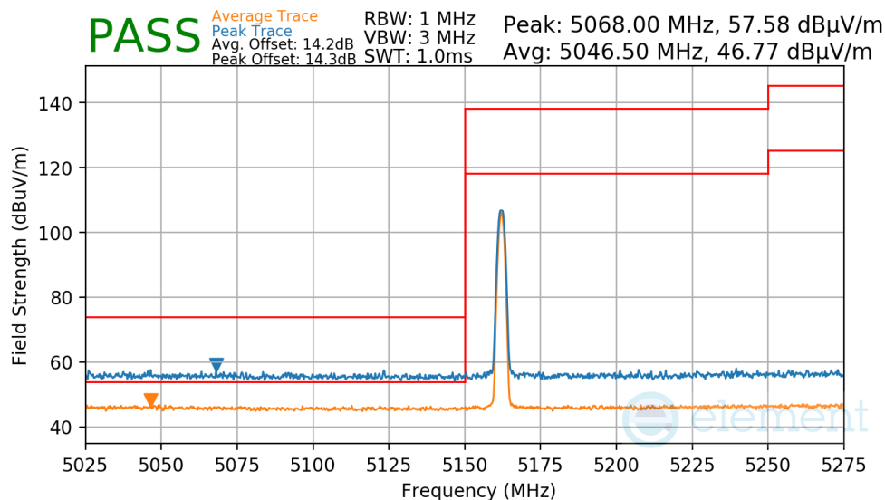
Plot 7-132. Radiated Lower Band Edge Measurement Antenna WF7b
