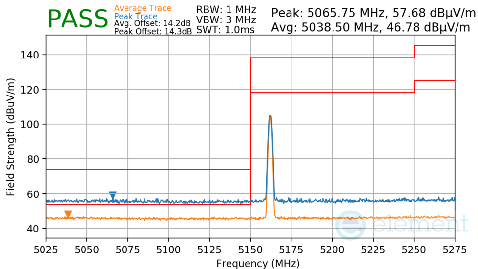
Plot 7-129. Radiated Lower Band Edge Measurement Antenna WF2a
