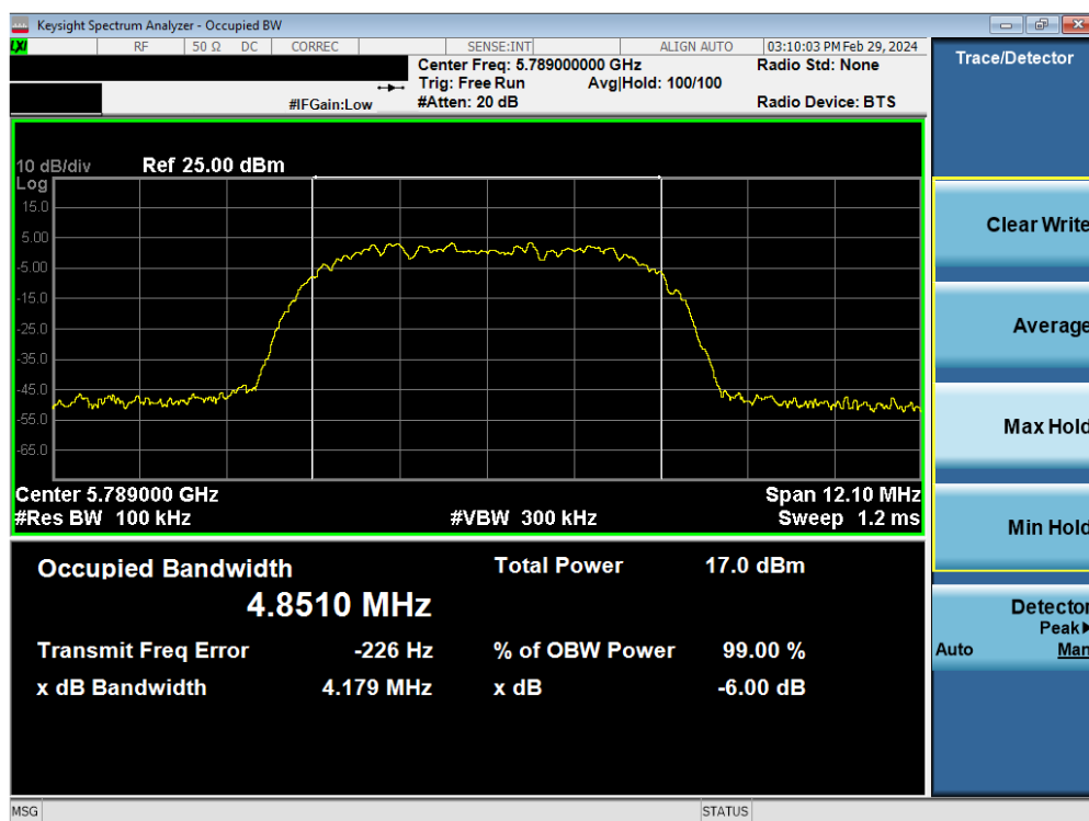
Plot 7-35. 6dB BW & 99% OBW Antenna WF7b (HDR8, ePA, 5789MHz)
