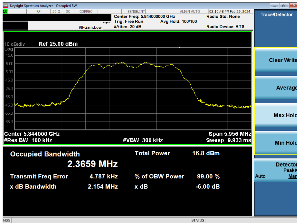
Plot 7-33. 6dB BW & 99% OBW Antenna WF7b (HDR4, ePA, 5844MHz)
