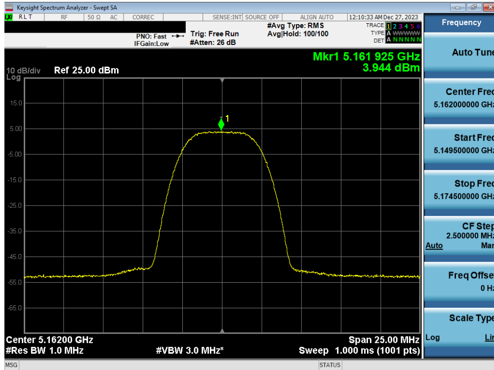
Plot 7-70. FCC/ISED PSD Antenna WF2a (HDR8, ePA – 5162MHz)
