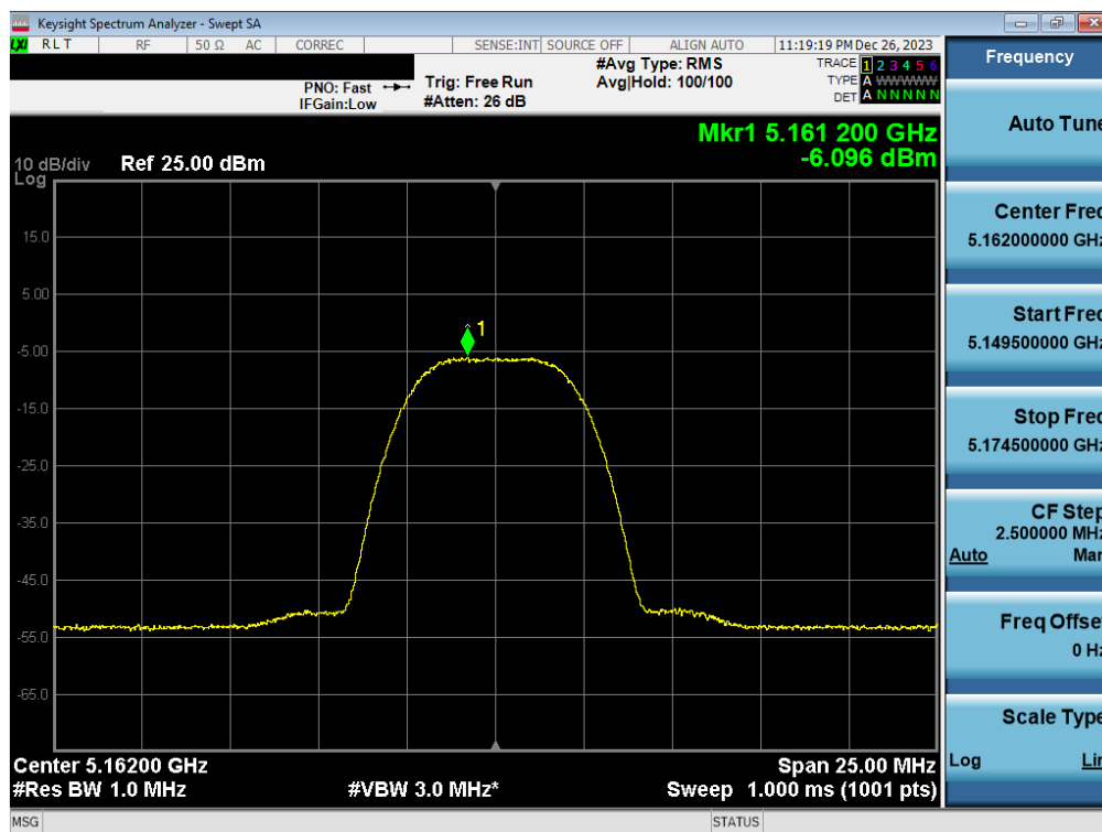
Plot 7-100. FCC/ISED PSD Antenna WF7b (HDR8, iPA - 5162MHz)
