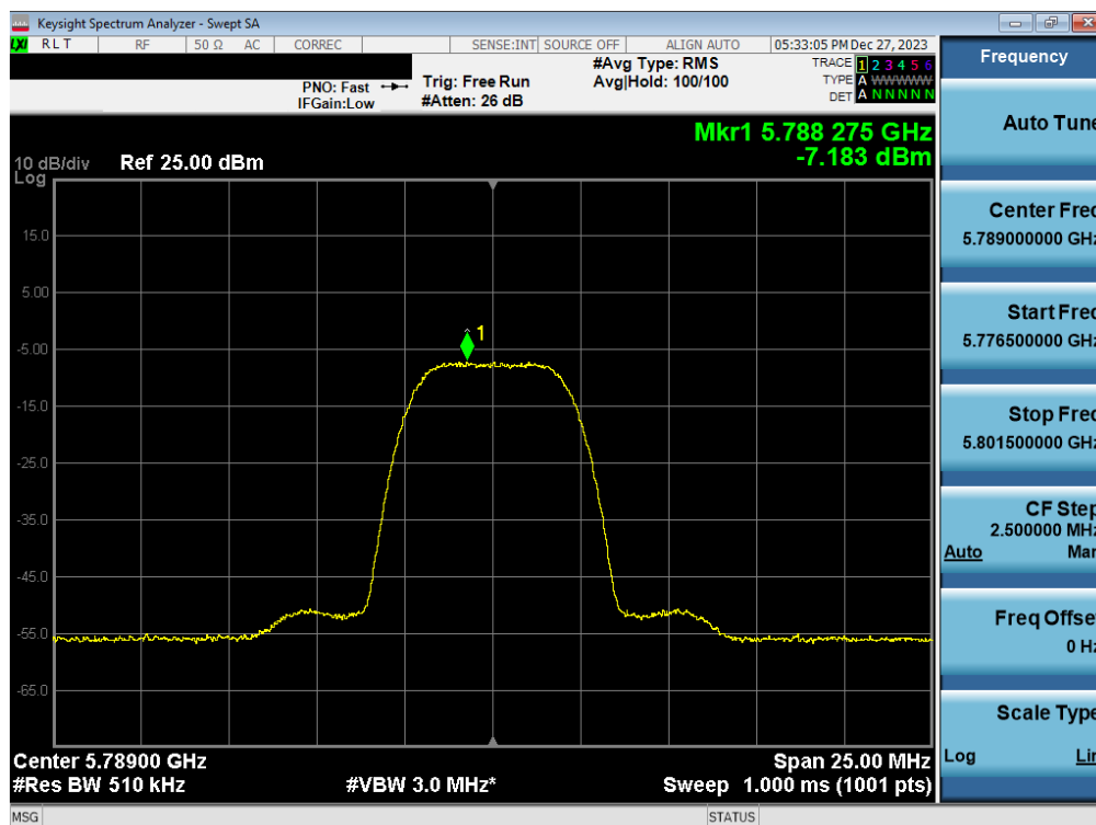
Plot 7-62. PSD Antenna WF7a (HDR8, iPA 5789MHz)
