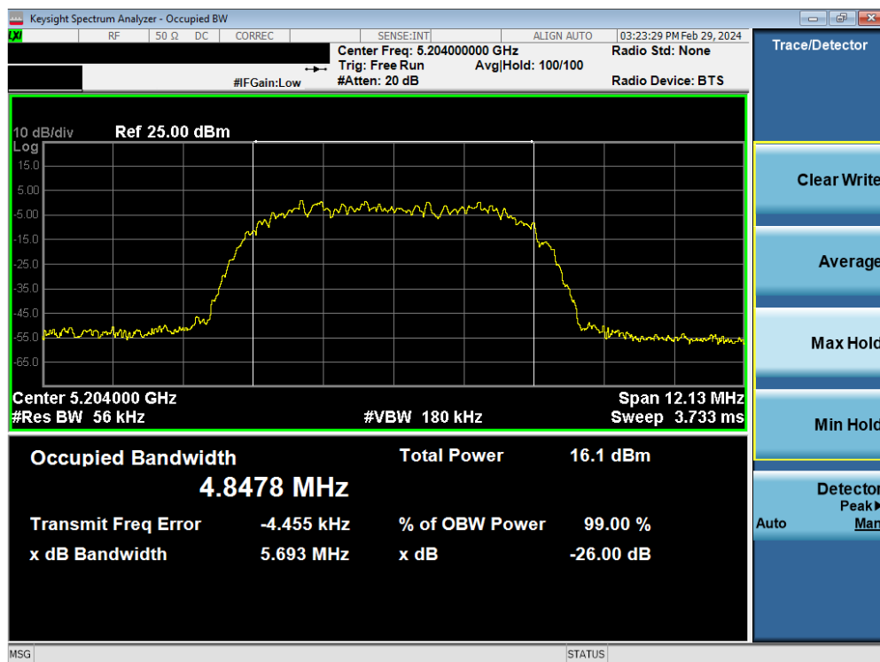
Plot 7-17. 26dB BW & 99% OBW Antenna WF7b (HDR8, ePA- 5204MHz)
