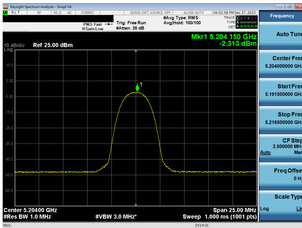
Plot 7-41. FCC/ISED PSD Antenna WF7a (HDR4, iPA – 5204MHz)
