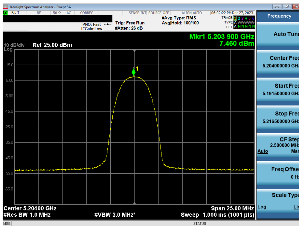
Plot 7-38. FCC PSD Antenna WF7a (HDR4, ePA – 5204MHz)
