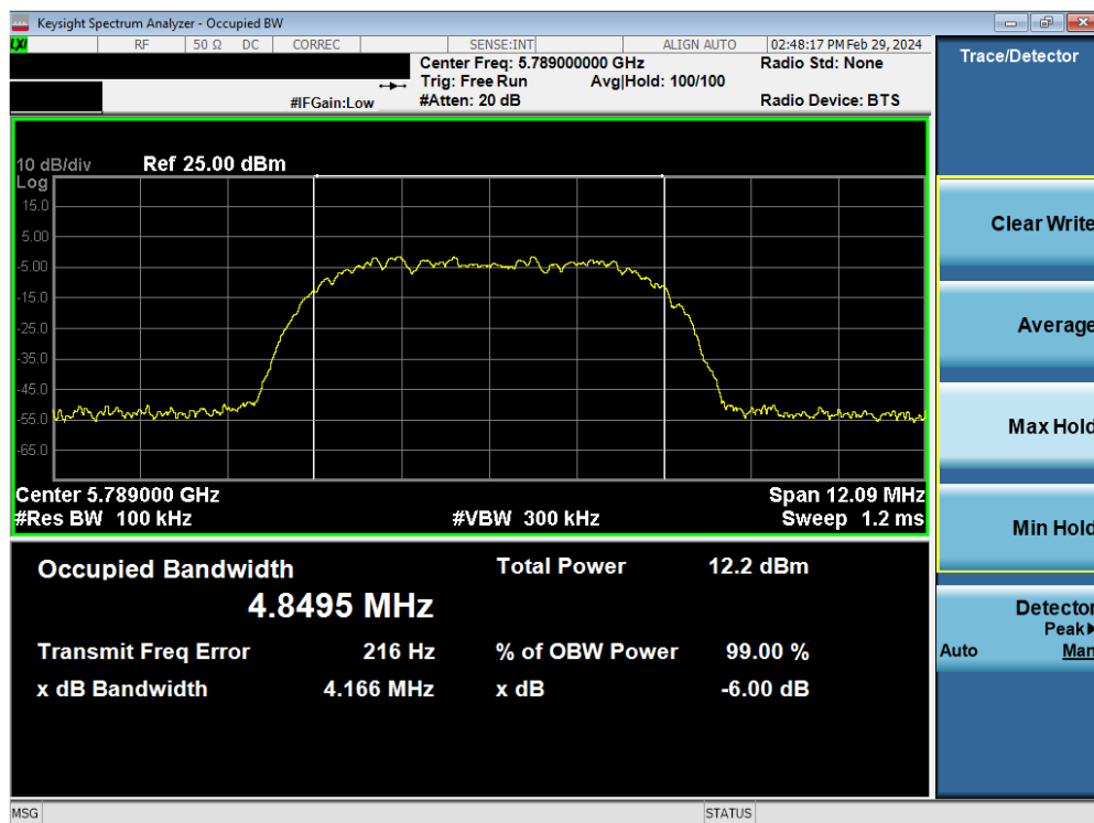
Plot 7-29. 6dB BW & 99% OBW Antenna WF2a (HDR8, ePA, 5789MHz)
