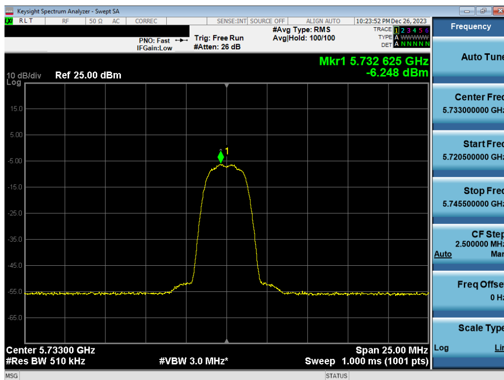
Plot 7-82. PSD Antenna WF2a (HDR4, iPA 5733MHz)
