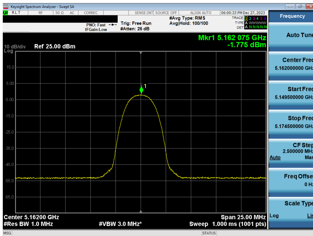
Plot 7-40. FCC/ISED PSD Antenna WF7a (HDR4, iPA - 5162MHz)
