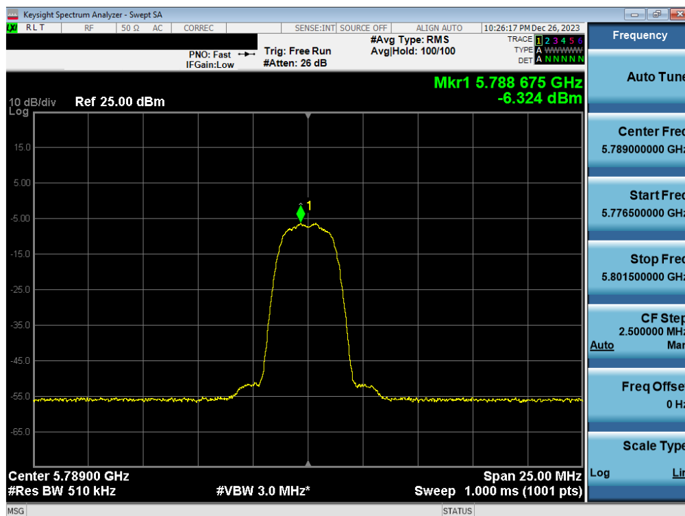
Plot 7-83. PSD Antenna WF2a (HDR4, iPA 5789MHz)
