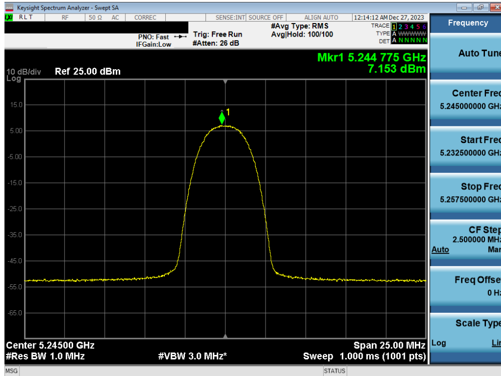
Plot 7-66. FCC PSD Antenna WF2a (HDR4, ePA- 5245MHz)
