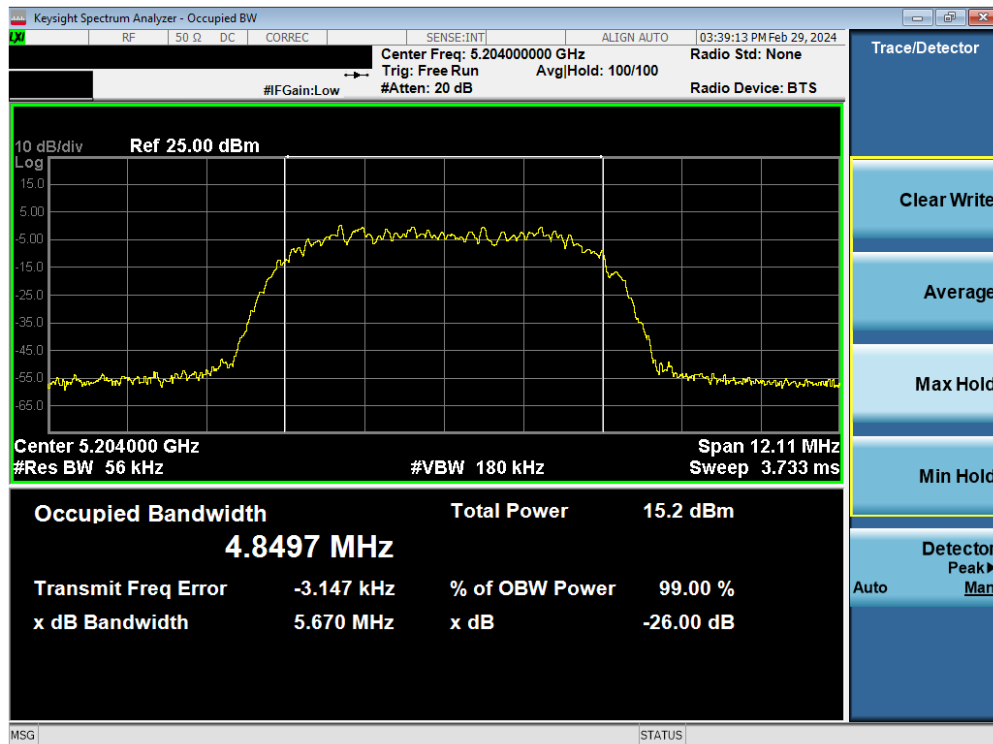
Plot 7-11. 26dB BW & 99% OBW Antenna WF2a (HDR8, ePA- 5204MHz)
