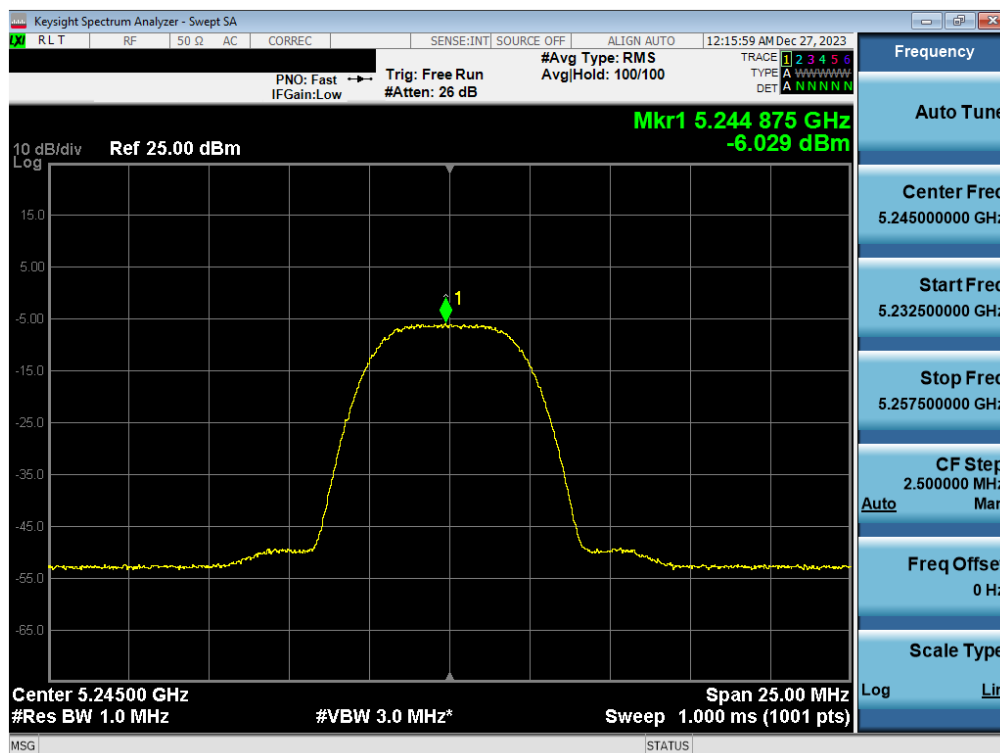
Plot 7-75. FCC/ISED PSD Antenna WF2a (HDR8, iPA– 5245MHz)
