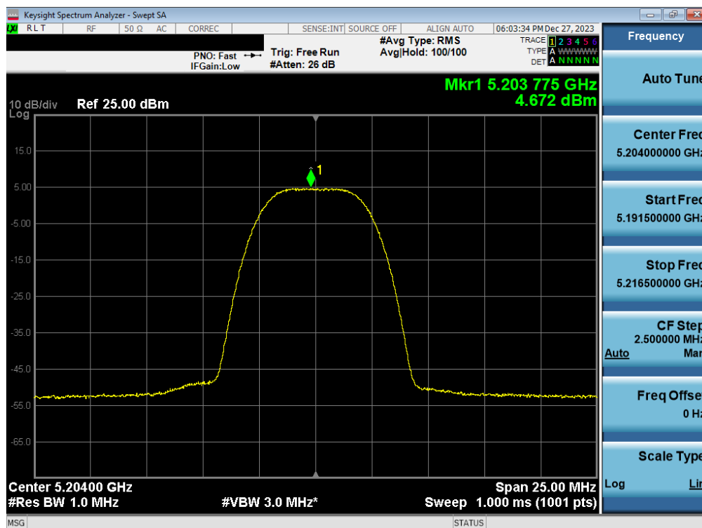
Plot 7-44. FCC/ISED PSD Antenna WF7a (HDR8, ePA – 5204MHz)
