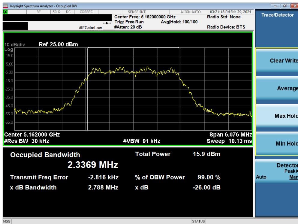
Plot 7-13. 26dB BW & 99% OBW Antenna WF7b (HDR4, ePA– 5162MHz)
