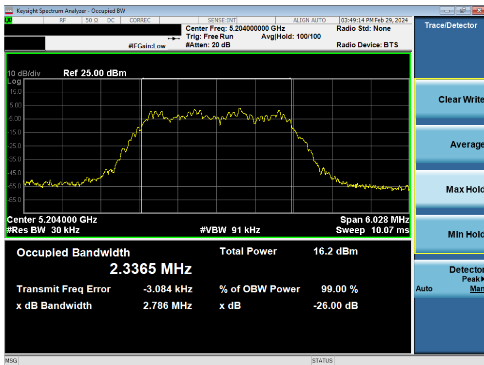
Plot 7-2. 26dB BW & 99% OBW Antenna WF7a (HDR4, ePA- 5204MHz)
