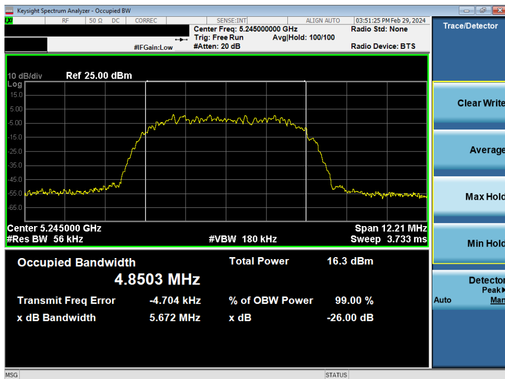
Plot 7-6. 26dB BW & 99% OBW Antenna WF7a (HDR8, ePA – 5245MHz)
