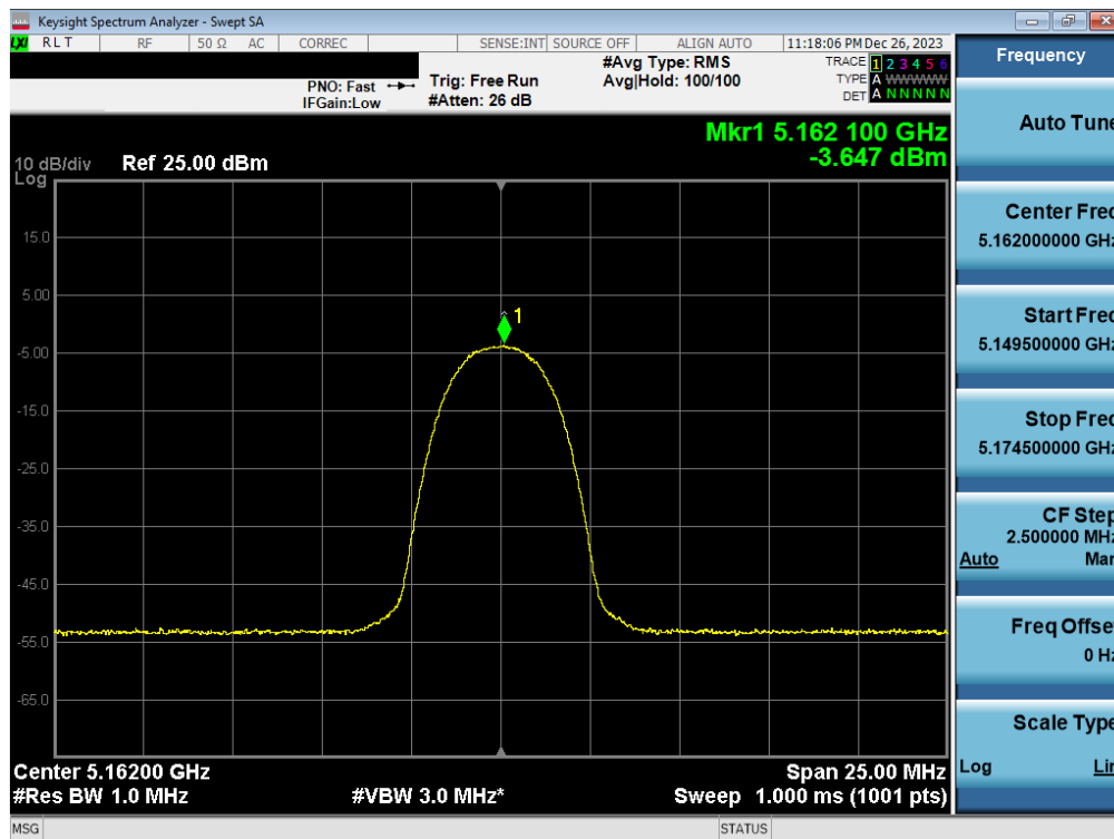
Plot 7-94. FCC/ISED PSD Antenna WF7b (HDR4, iPA - 5162MHz)
