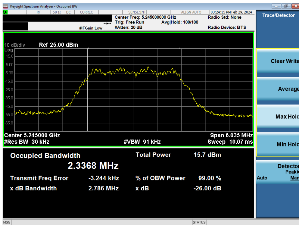
Plot 7-15. 26dB BW & 99% OBW Antenna WF7b (HDR4, ePA- 5245MHz)
