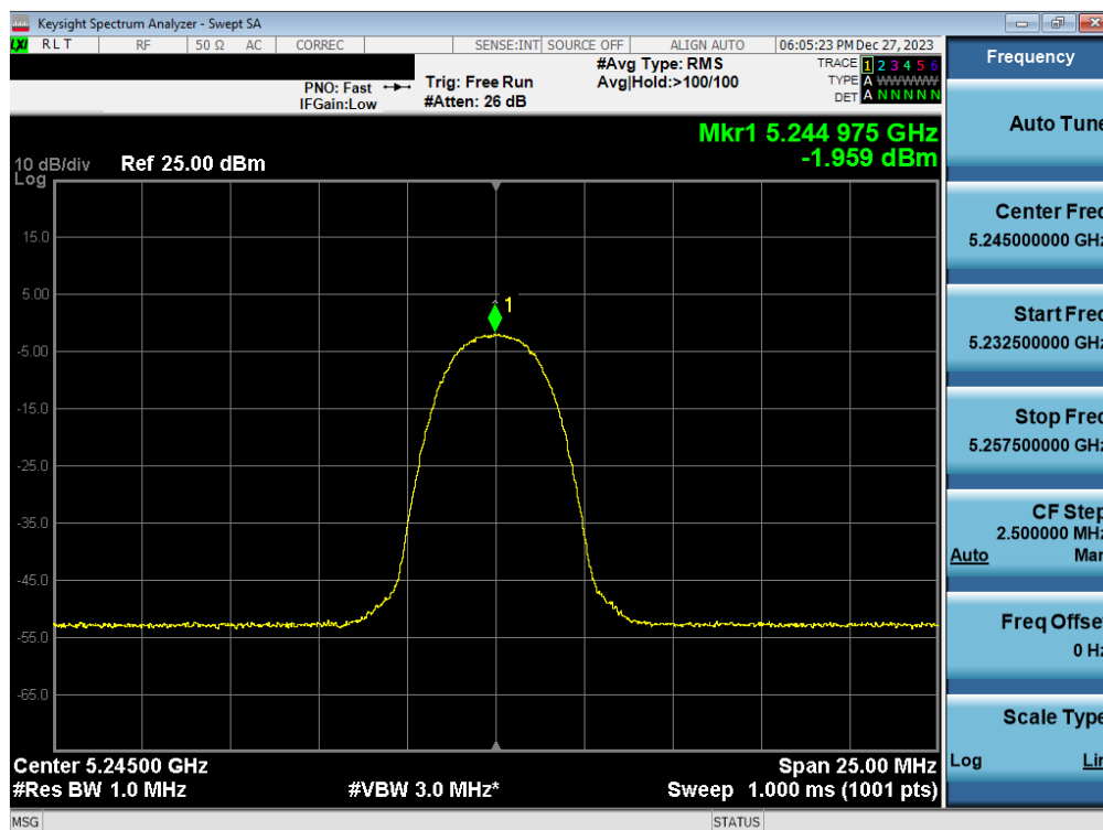
Plot 7-42. FCC/ISED PSD Antenna WF7a (HDR4, iPA– 5245MHz)
