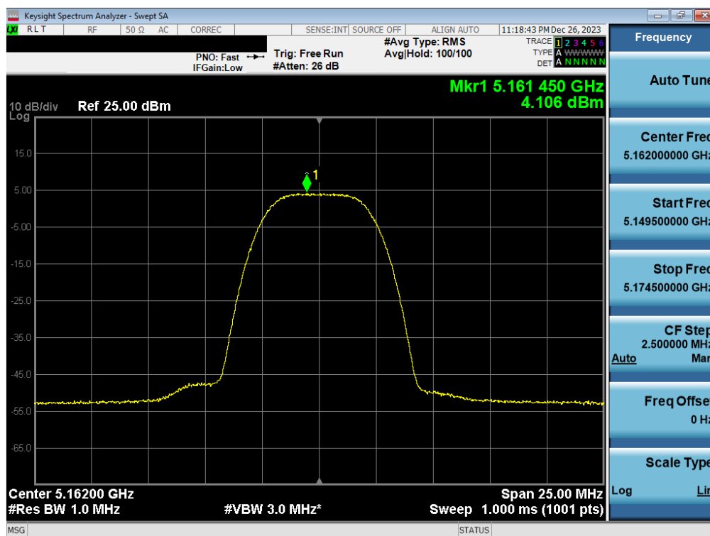
Plot 7-97. FCC/ISED PSD Antenna WF7b (HDR8, ePA – 5162MHz)
