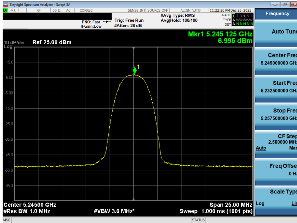
Plot 7-93. FCC PSD Antenna WF7b (HDR4, ePA- 5245MHz)
