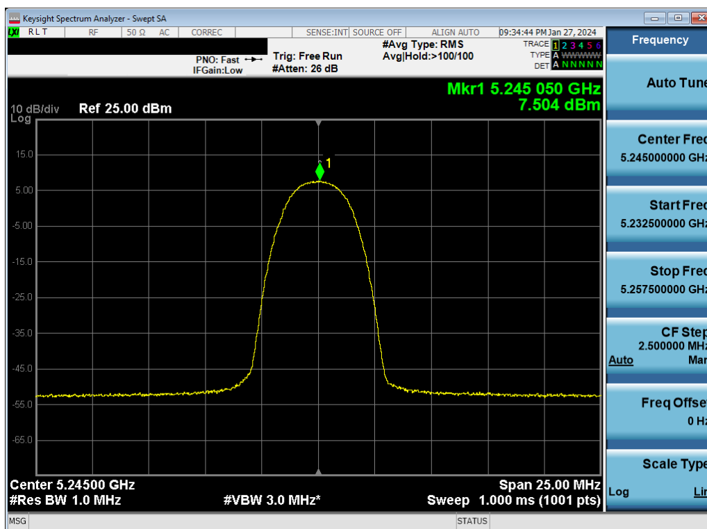
Plot 7-78. ISED PSD Antenna WF2a (HDR4, ePA– 5245MHz)
