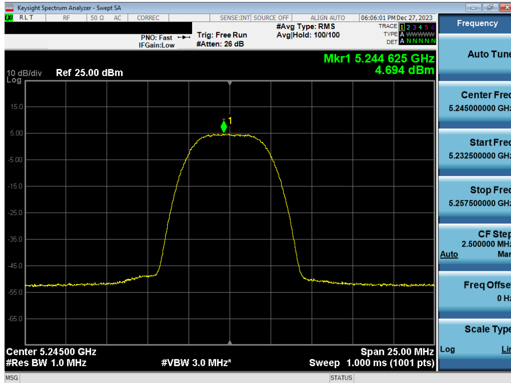
Plot 7-45. FCC/ISED PSD Antenna WF7a (HDR8, ePA– 5245MHz)
