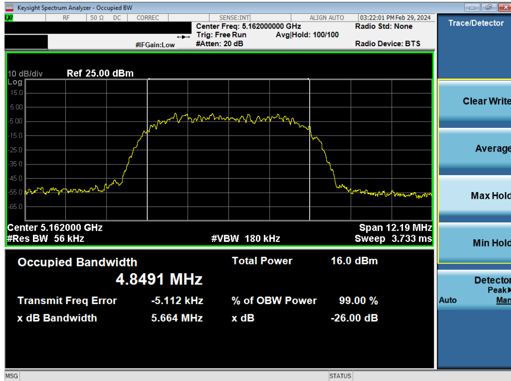
Plot 7-16. 26dB BW & 99% OBW Antenna WF7b (HDR8, ePA- 5162MHz)
