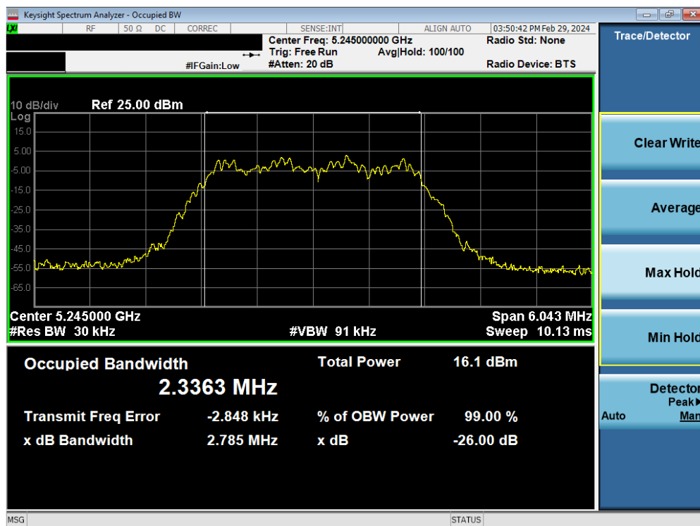
Plot 7-3. 26dB BW & 99% OBW Antenna WF7a (HDR4, ePA - 5245MHz)
