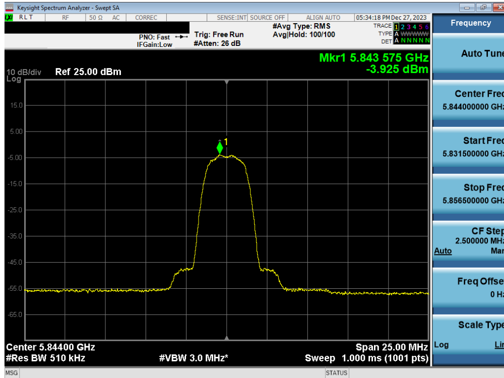
Plot 7-57. PSD Antenna WF7a (HDR4, iPA 5844MHz)
