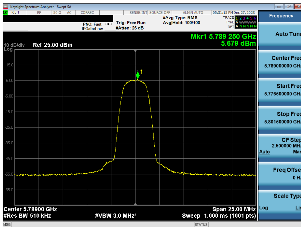
Plot 7-53. PSD Antenna WF7a (HDR4, ePA 5789MHz)
