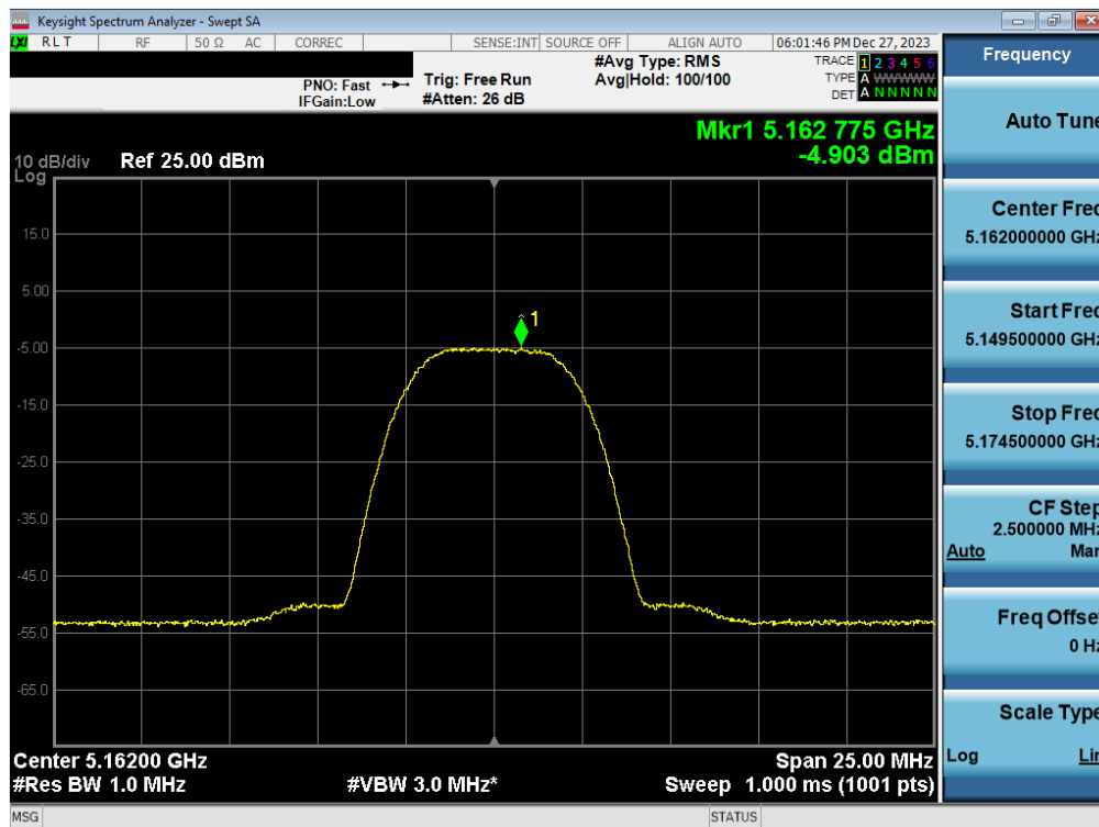
Plot 7-46. FCC/ISED PSD Antenna WF7a (HDR8, iPA – 5162MHz)
