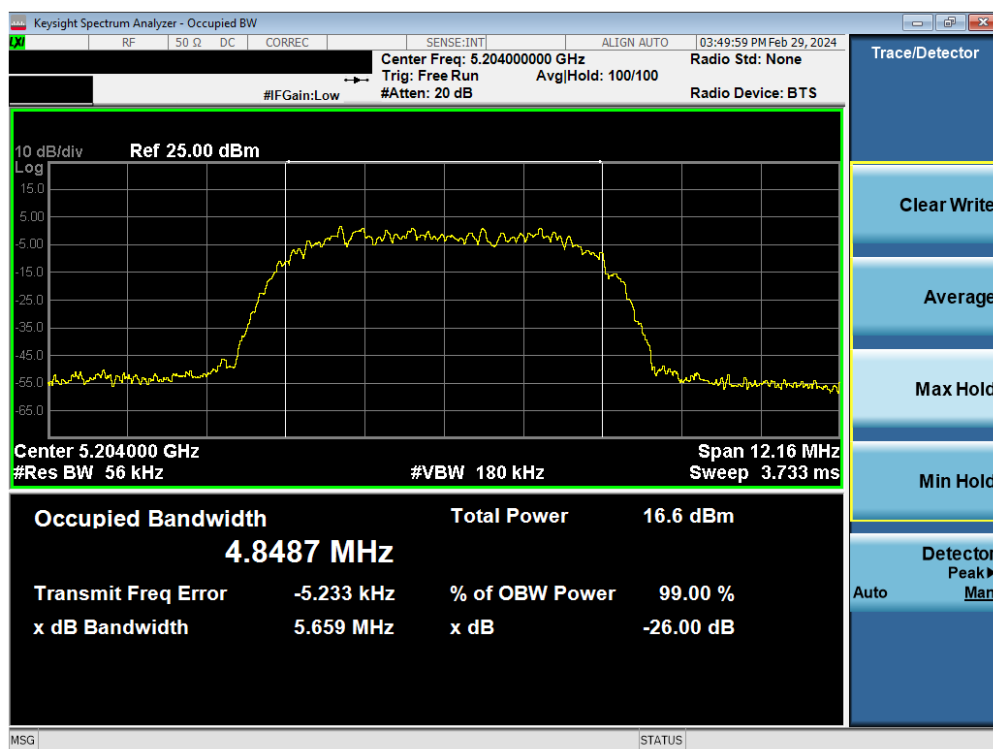
Plot 7-5. 26dB BW & 99% OBW Antenna WF7a (HDR8, ePA- 5204MHz)
