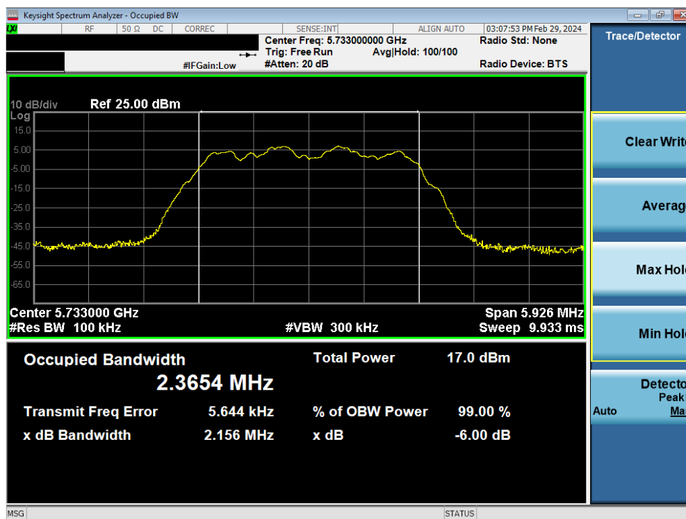
Plot 7-31. 6dB BW & 99% OBW Antenna WF7b (HDR4, ePA, 5733MHz)
