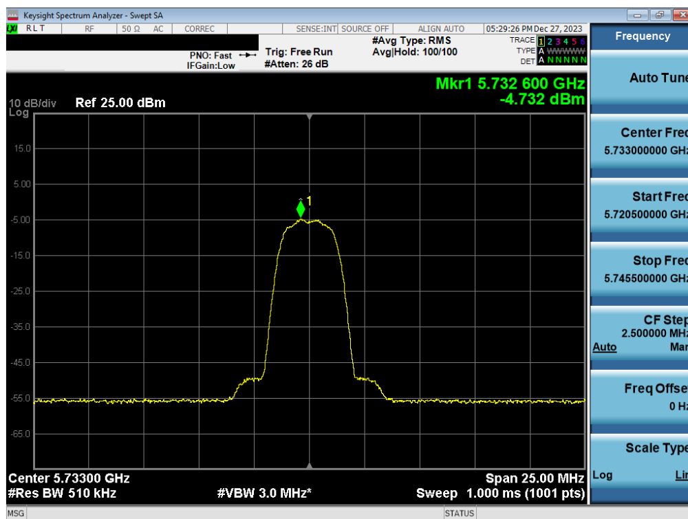
Plot 7-55. PSD Antenna WF7a (HDR4, iPA 5733MHz)
