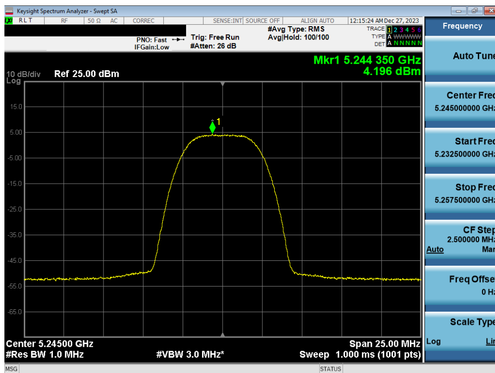
Plot 7-72. FCC/ISED PSD Antenna WF2a (HDR8, ePA- 5245MHz)
