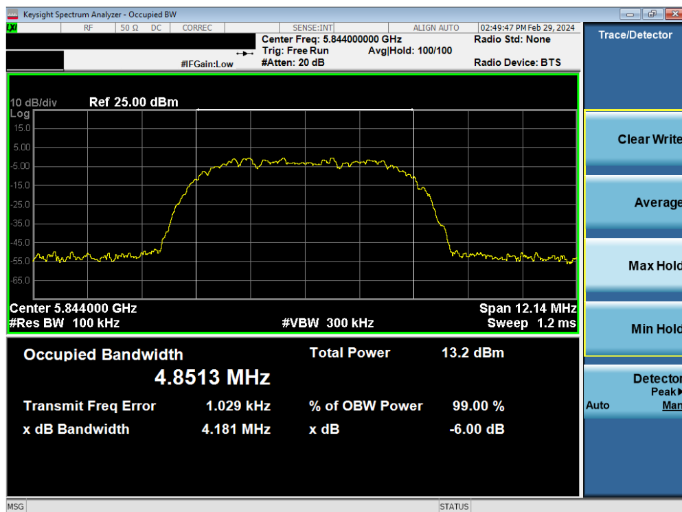
Plot 7-30. 6dB BW & 99% OBW Antenna WF2a (HDR8, ePA, 5844MHz)
