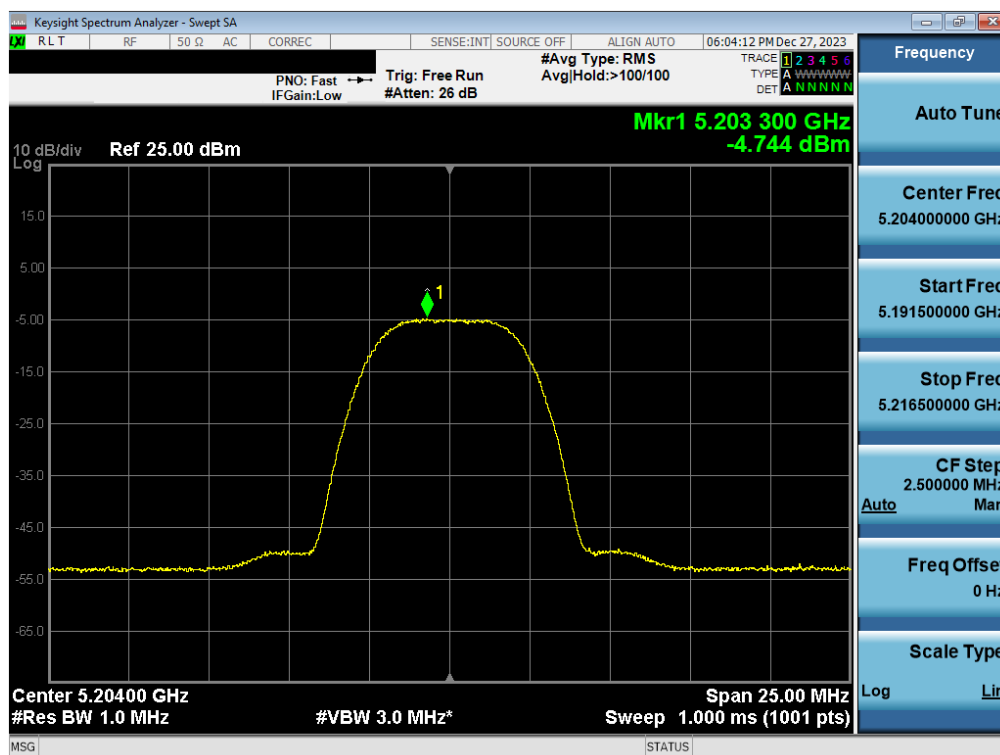
Plot 7-47. FCC/ISED PSD Antenna WF7a (HDR8, iPA – 5204MHz)
