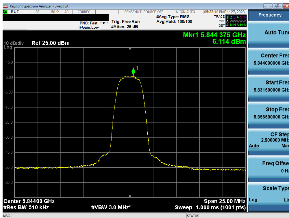
Plot 7-54. PSD Antenna WF7a (HDR4, ePA 5844MHz)
