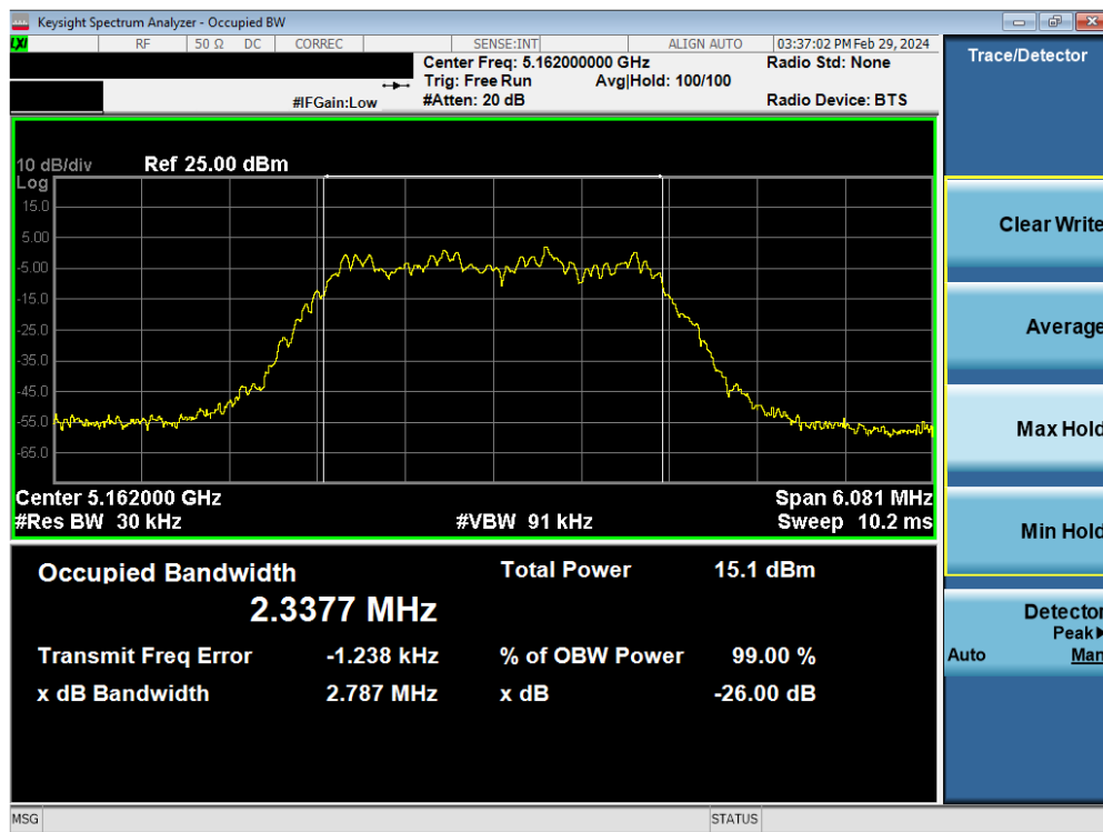
Plot 7-7. 26dB BW & 99% OBW Antenna WF2a (HDR4, ePA– 5162MHz)
