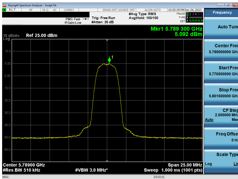
Plot 7-80. PSD Antenna WF2a (HDR4, ePA 5789MHz)
