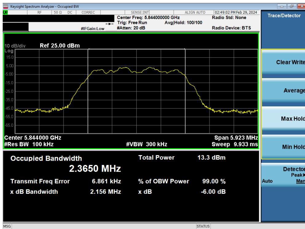
Plot 7-27. 6dB BW & 99% OBW Antenna WF2a (HDR4, ePA, 5844MHz)
