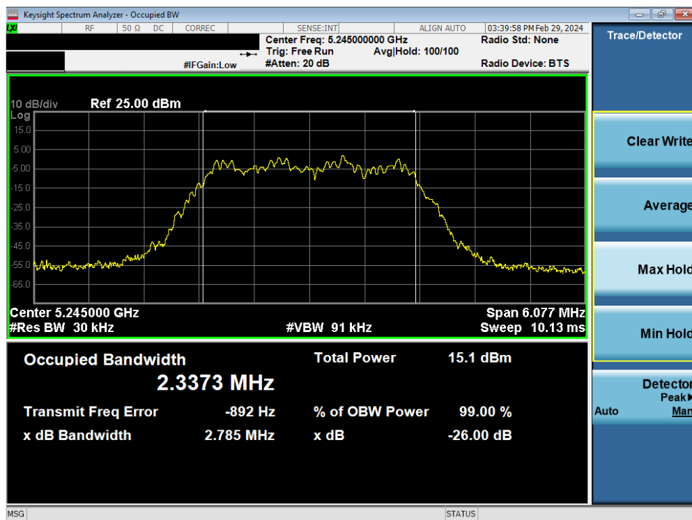
Plot 7-9. 26dB BW & 99% OBW Antenna WF2a (HDR4, ePA- 5245MHz)
