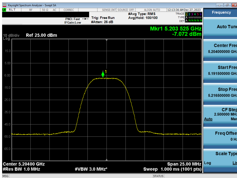
Plot 7-74. FCC/ISED PSD Antenna WF2a (HDR8, iPA – 5204MHz)
