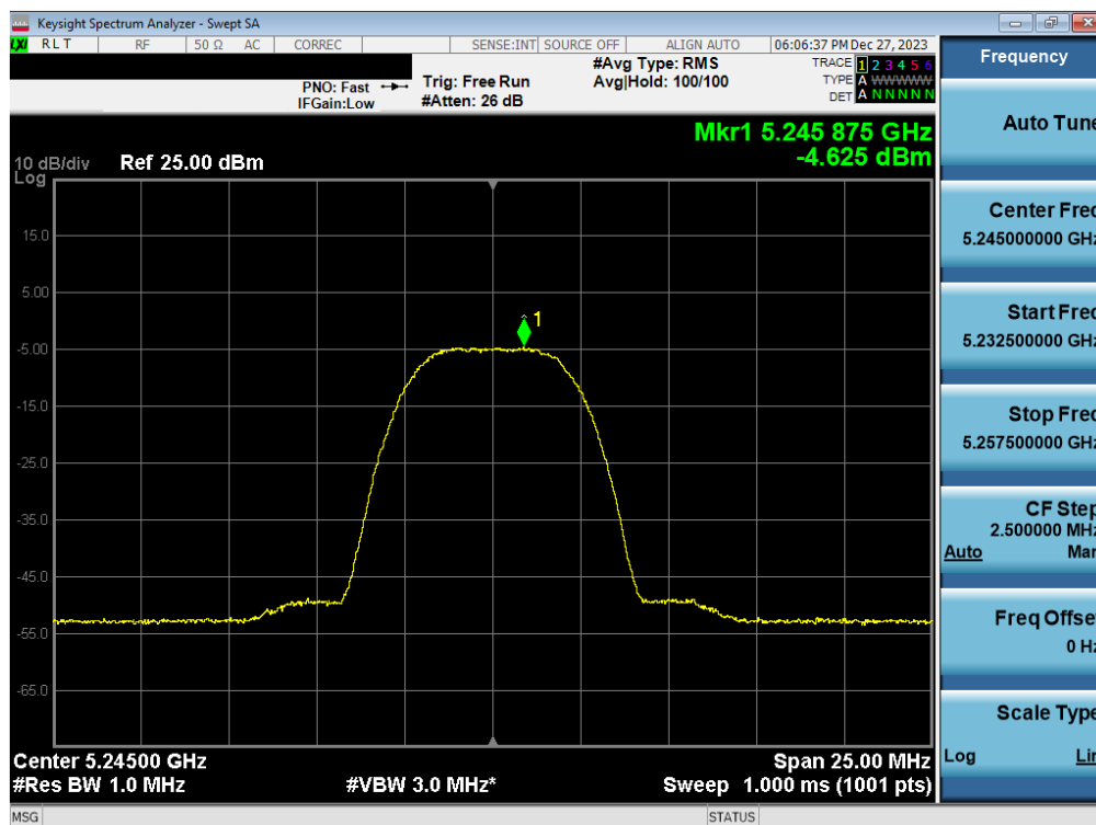
Plot 7-48. FCC/ISED PSD Antenna WF7a (HDR8, iPA– 5245MHz)
