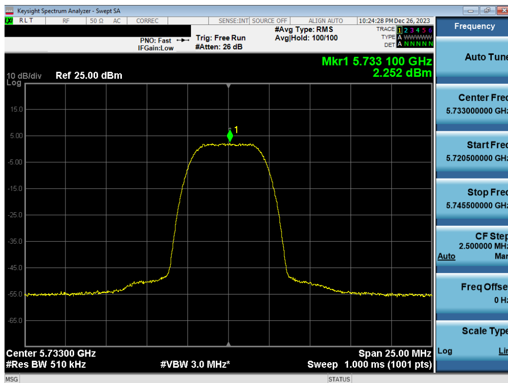
Plot 7-85. PSD Antenna WF2a (HDR8, ePA 5733MHz)
