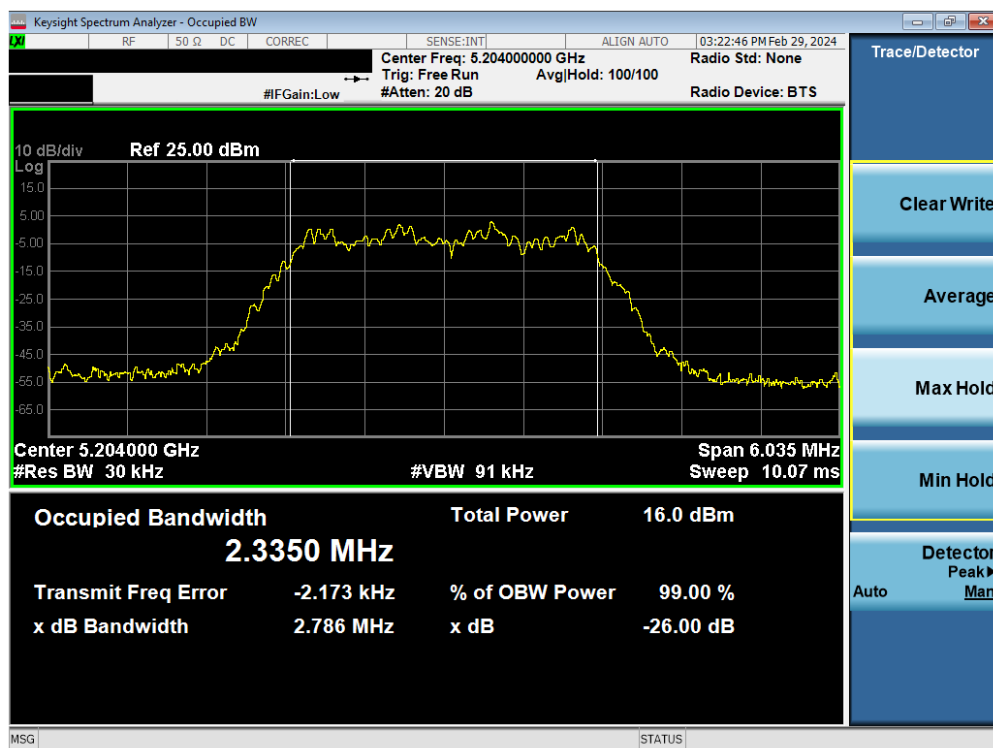
Plot 7-14. 26dB BW & 99% OBW Antenna WF7b (HDR4, ePA- 5204MHz)
