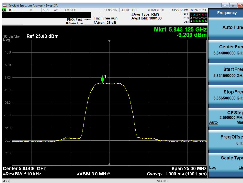
Plot 7-90. PSD Antenna WF2a (HDR8, iPA 5844MHz)
