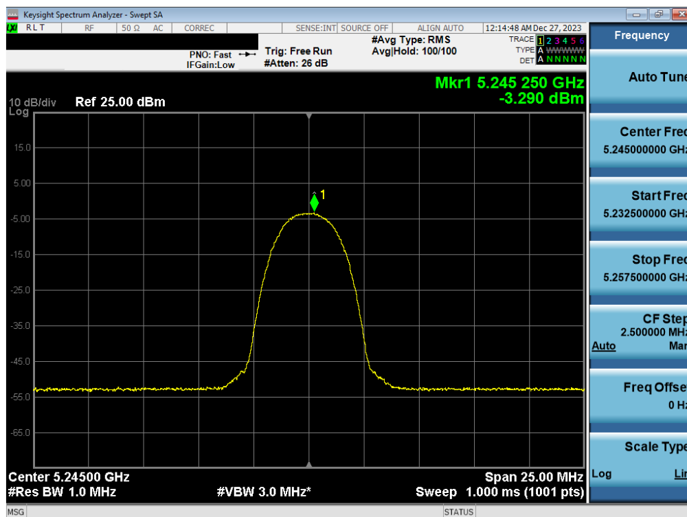
Plot 7-69. FCC/ISED PSD Antenna WF2a (HDR4, iPA– 5245MHz)
