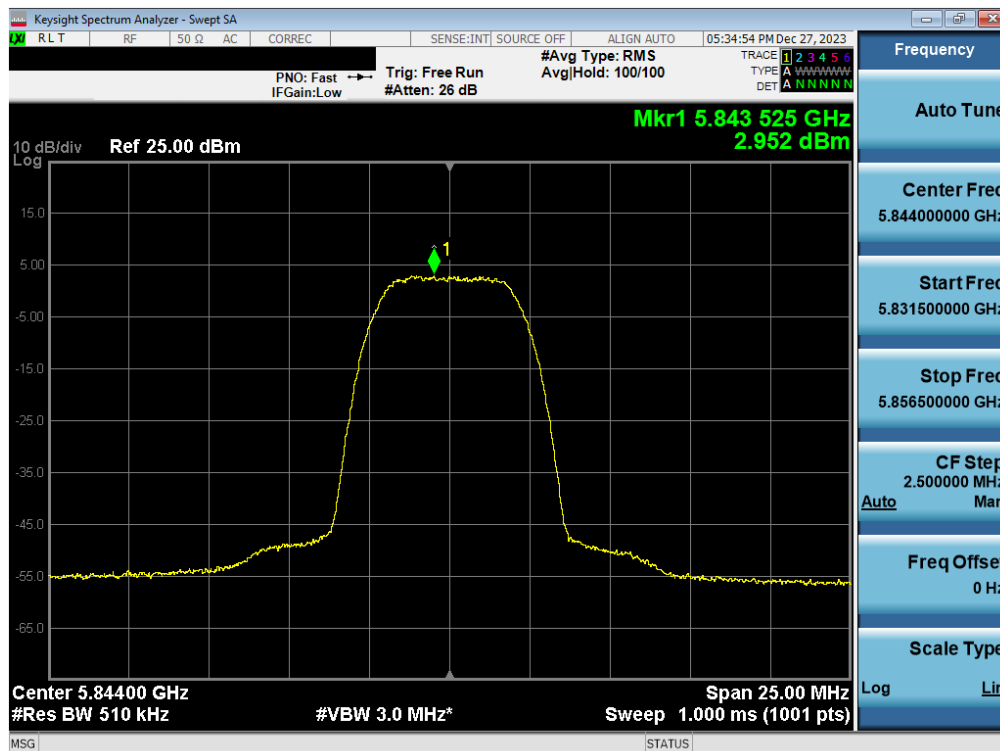
Plot 7-60. PSD Antenna WF7a (HDR8, ePA 5844MHz)
