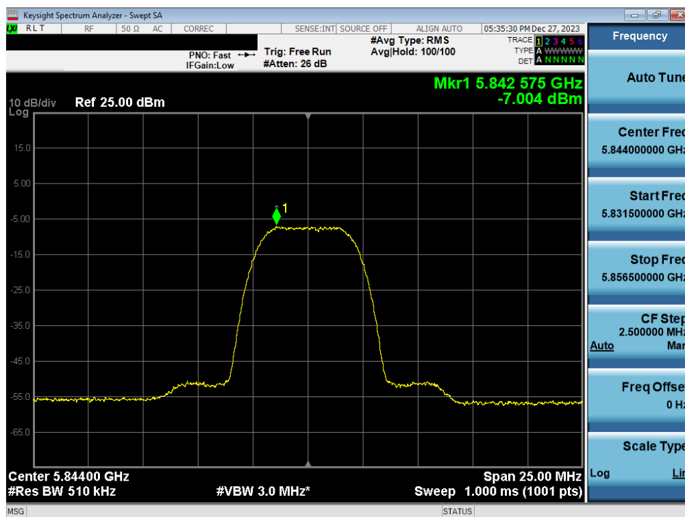
Plot 7-63. PSD Antenna WF7a (HDR8, iPA 5844MHz)
