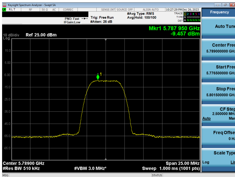
Plot 7-89. PSD Antenna WF2a (HDR8, iPA 5789MHz)
