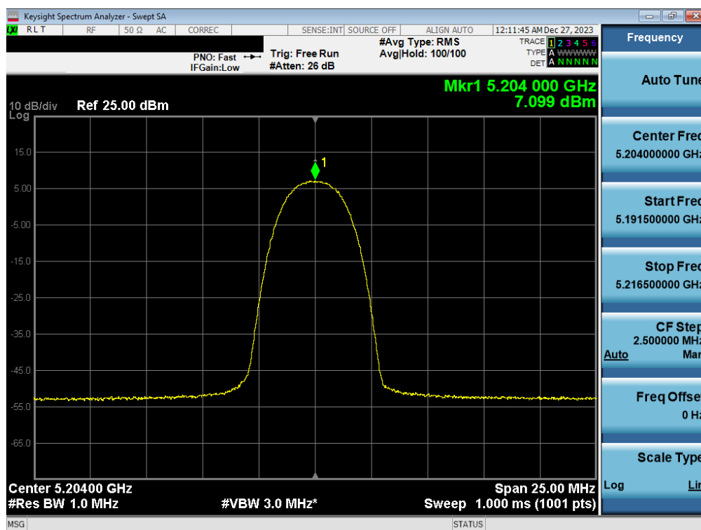
Plot 7-65. FCC PSD Antenna WF2a (HDR4, ePA – 5204MHz)
