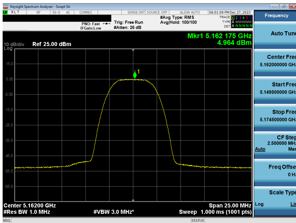
Plot 7-43. FCC/ISED PSD Antenna WF7a (HDR8, ePA – 5162MHz)
