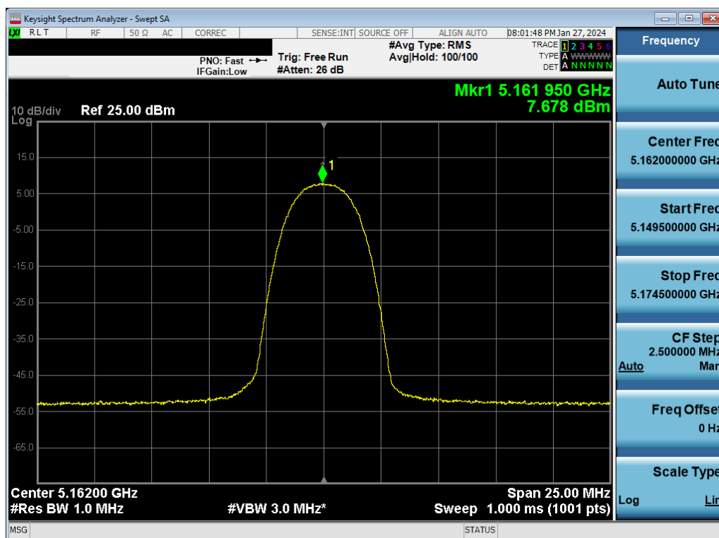
Plot 7-49. ISED PSD Antenna WF7a (HDR4, ePA – 5162MHz)
