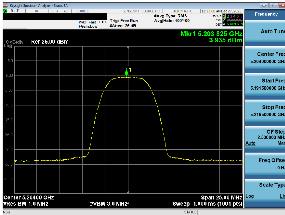
Plot 7-71. FCC/ISED PSD Antenna WF2a (HDR8, ePA – 5204MHz)
