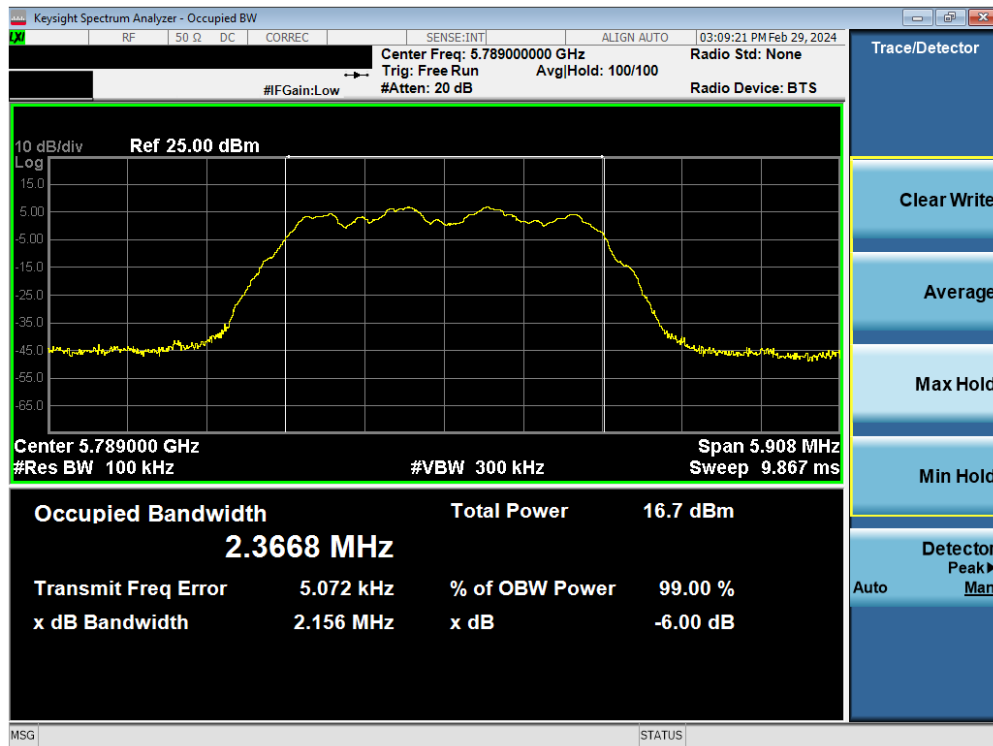
Plot 7-32. 6dB BW & 99% OBW Antenna WF7b (HDR4, ePA, 5789MHz)
