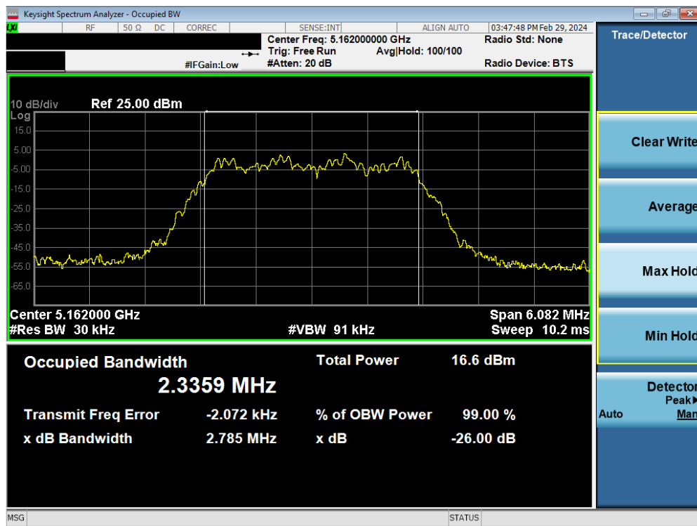
Plot 7-1. 26dB BW & 99% OBW Antenna WF7a (HDR4, ePA– 5162MHz)
