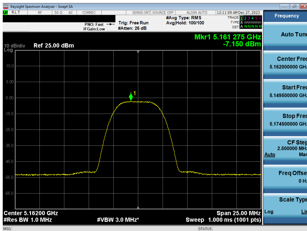
Plot 7-73. FCC/ISED PSD Antenna WF2a (HDR8, iPA - 5162MHz)
