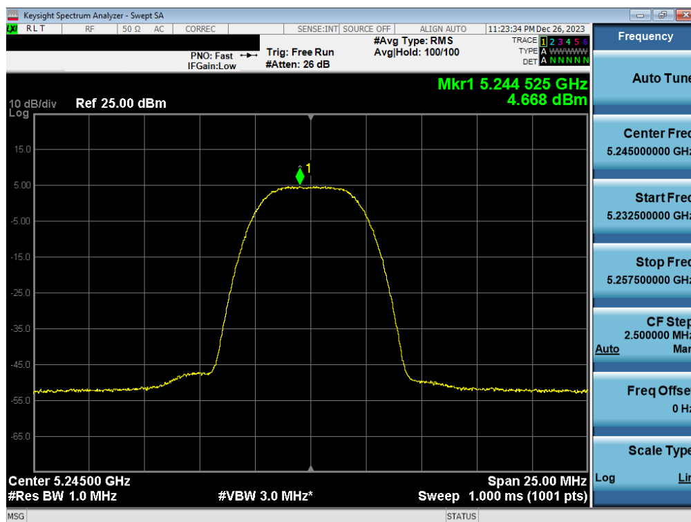
Plot 7-99. FCC/ISED PSD Antenna WF7b (HDR8, ePA-5245MHz)
