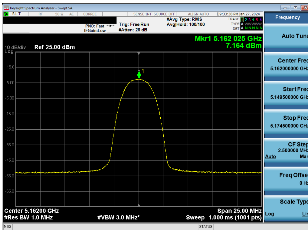
Plot 7-76. ISED PSD Antenna WF2a (HDR4, ePA – 5162MHz)
