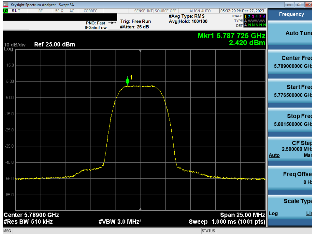
Plot 7-59. PSD Antenna WF7a (HDR8, ePA 5789MHz)
