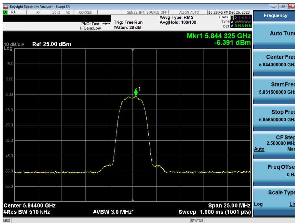
Plot 7-84. PSD Antenna WF2a (HDR4, iPA 5844MHz)
