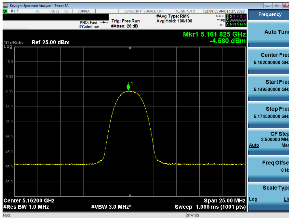
Plot 7-67. FCC/ISED PSD Antenna WF2a (HDR4, iPA - 5162MHz)
