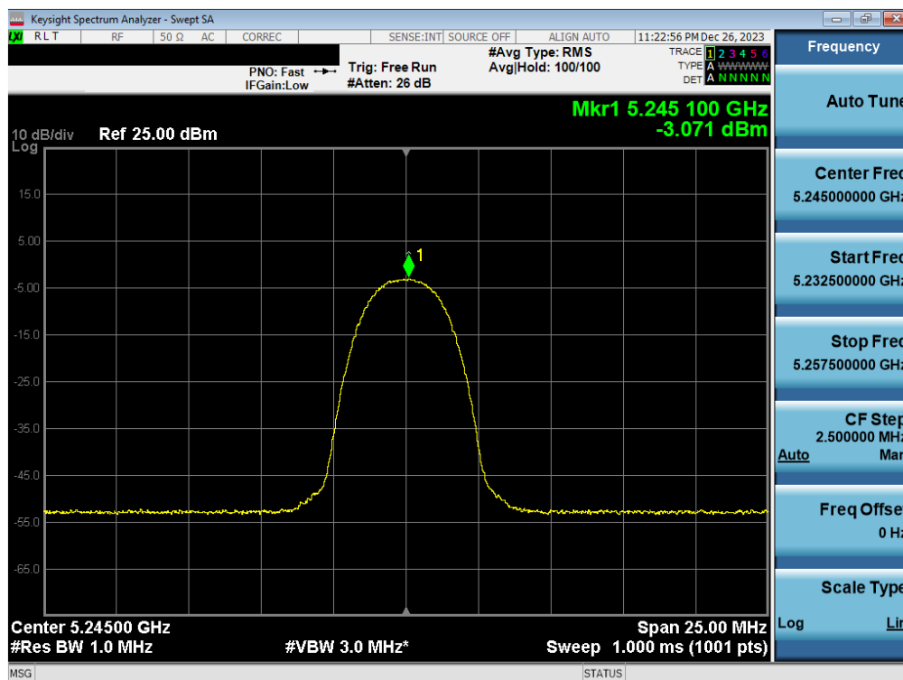
Plot 7-96. FCC/ISED PSD Antenna WF7b (HDR4, iPA– 5245MHz)
