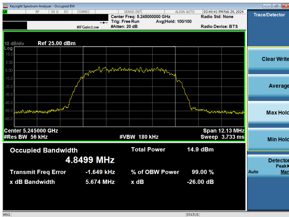
Plot 7-12. 26dB BW & 99% OBW Antenna WF2a (HDR8, ePA– 5245MHz)
