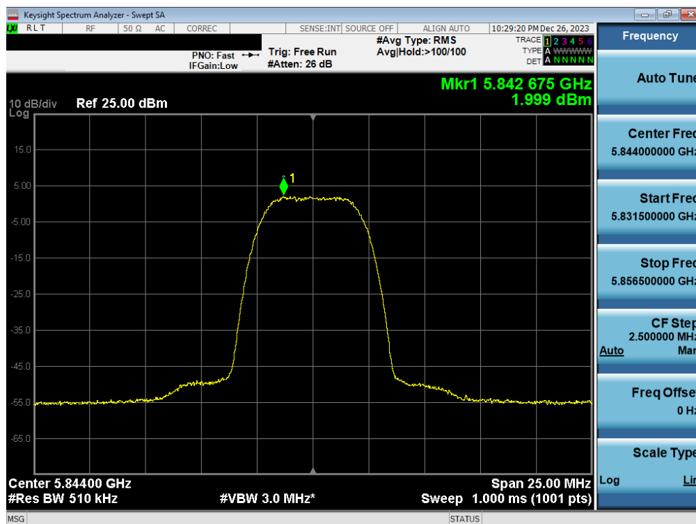
Plot 7-87. PSD Antenna WF2a (HDR8, ePA 5844MHz)
