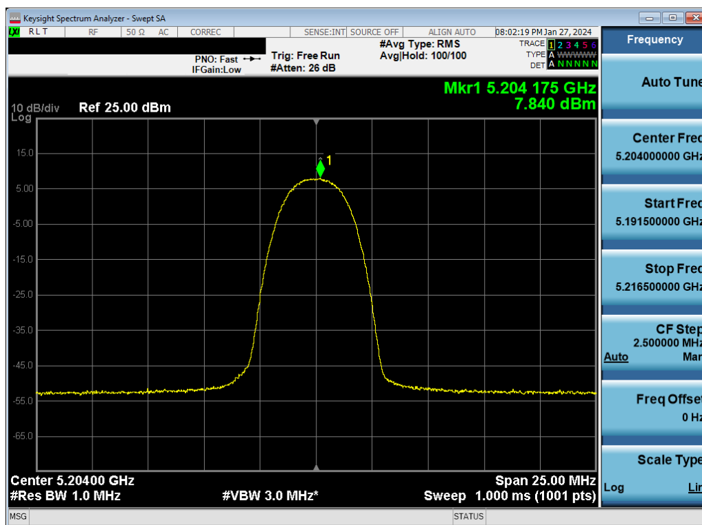
Plot 7-50. ISED PSD Antenna WF7a (HDR4, ePA – 5204MHz)
