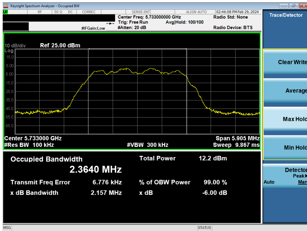
Plot 7-25. 6dB BW & 99% OBW Antenna WF2a (HDR4, ePA, 5733MHz)
