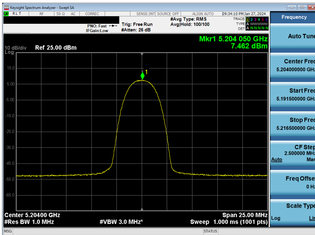
Plot 7-77. ISED PSD Antenna WF2a (HDR4, ePA – 5204MHz)
