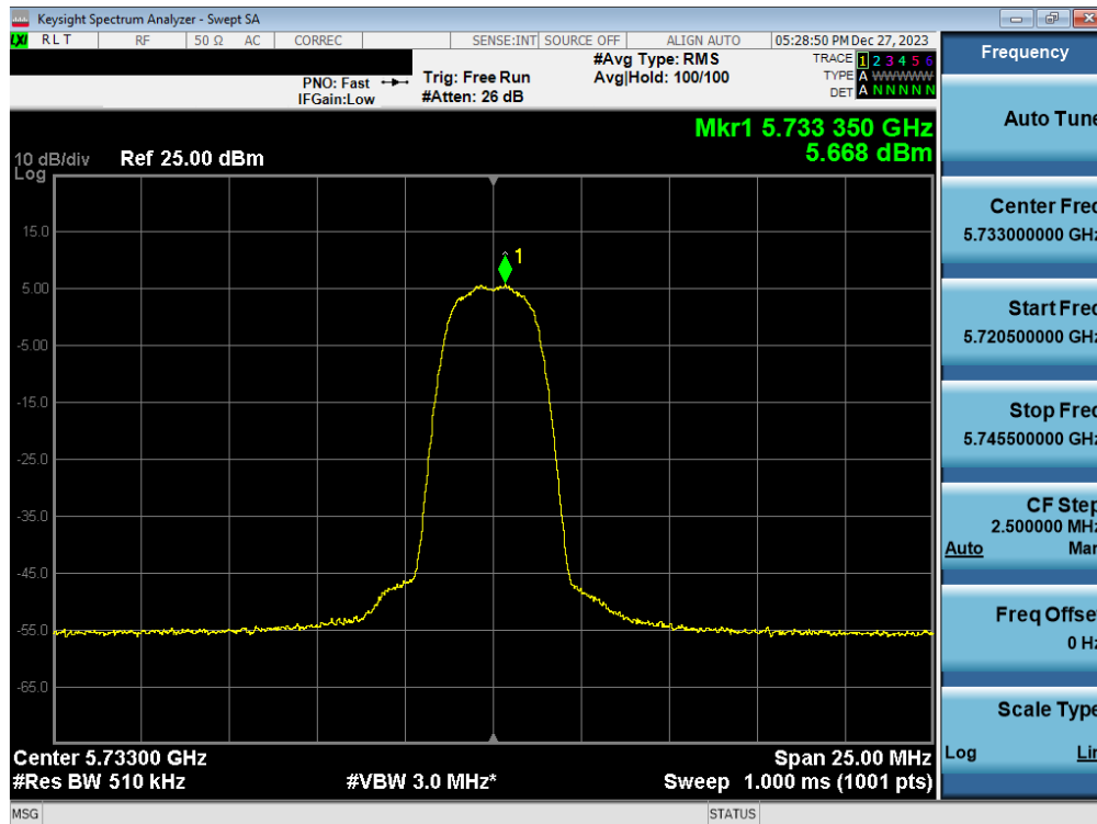
Plot 7-52. PSD Antenna WF7a (HDR4, ePA 5733MHz)
