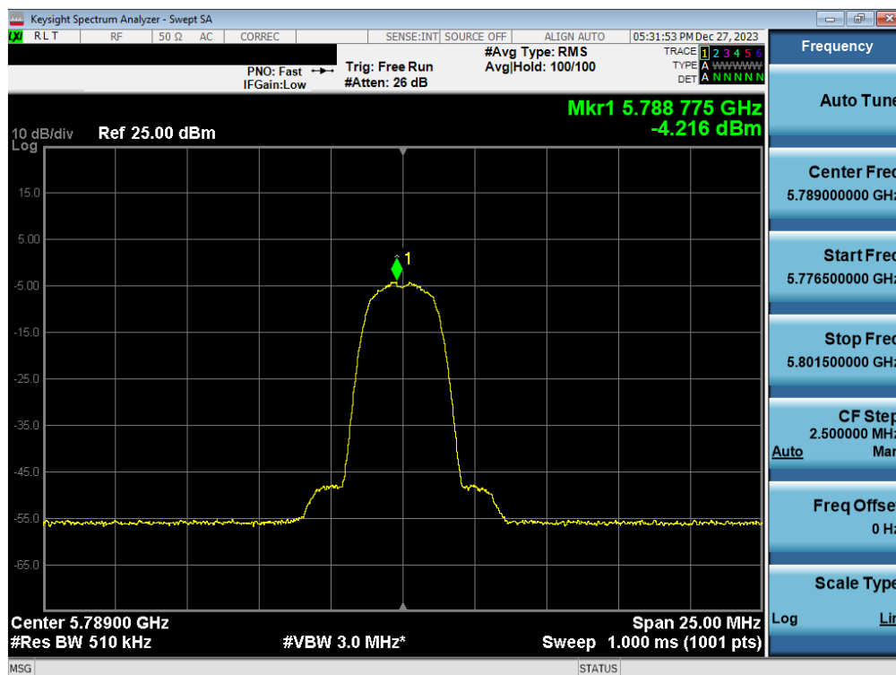
Plot 7-56. PSD Antenna WF7a (HDR4, iPA 5789MHz)
