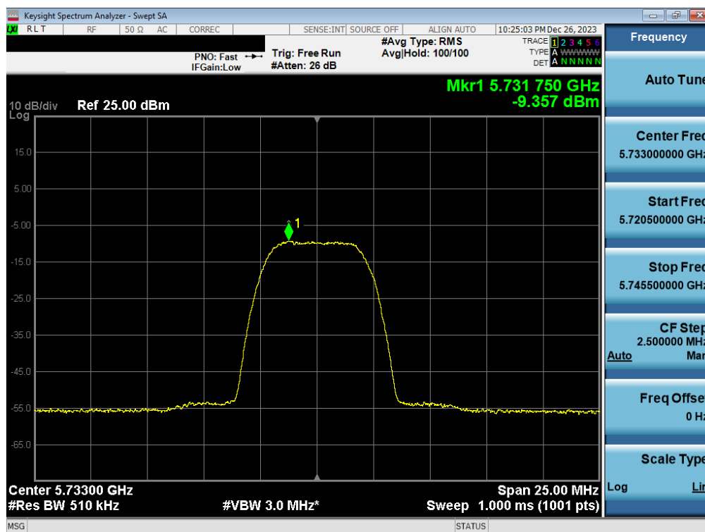
Plot 7-88. PSD Antenna WF2a (HDR8, iPA 5733MHz)
