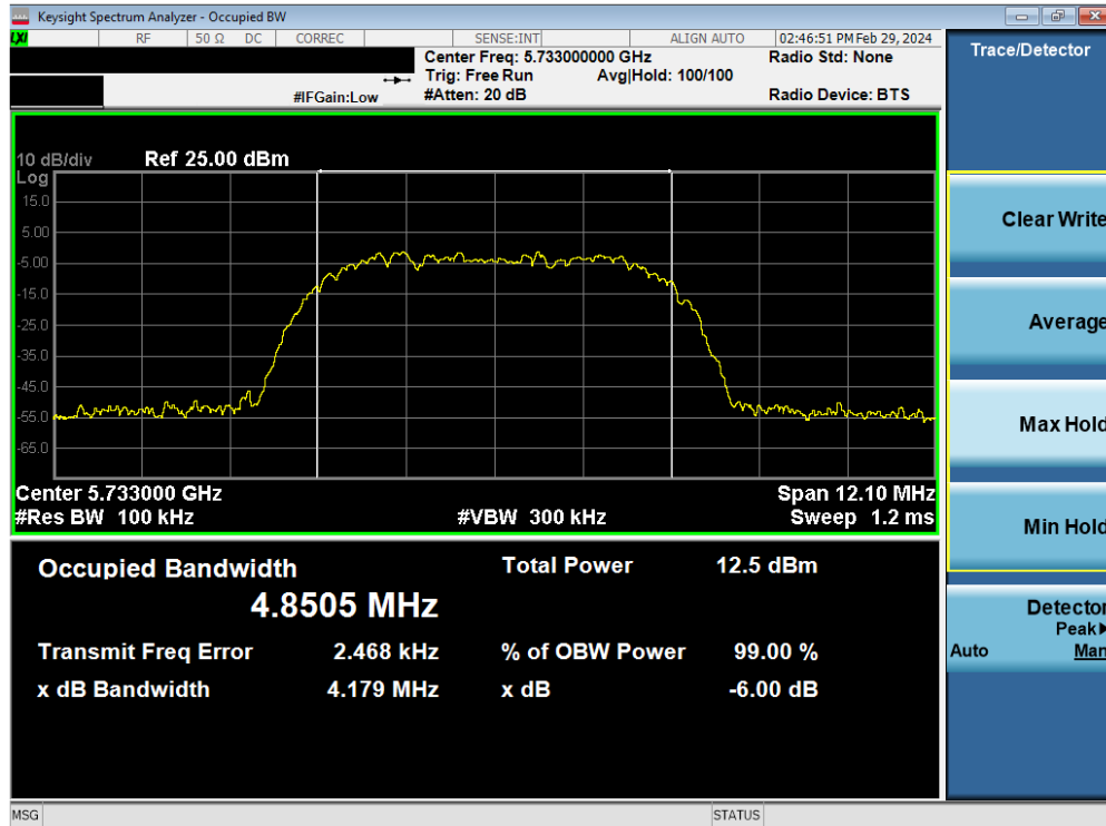
Plot 7-28. 6dB BW & 99% OBW Antenna WF2a (HDR8, ePA, 5733MHz)
