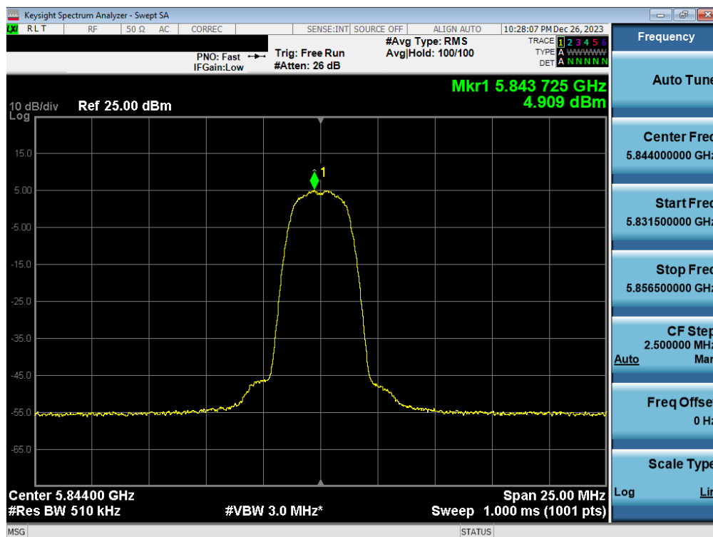
Plot 7-81. PSD Antenna WF2a (HDR4, ePA 5844MHz)
