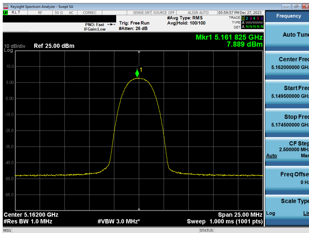
Plot 7-37. FCC PSD Antenna WF7a (HDR4, ePA – 5162MHz)
