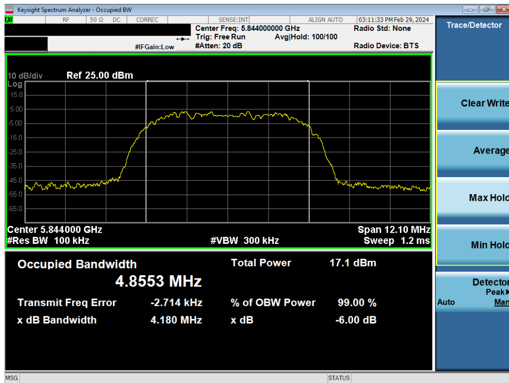
Plot 7-36. 6dB BW & 99% OBW Antenna WF7b (HDR8, ePA, 5844MHz)
