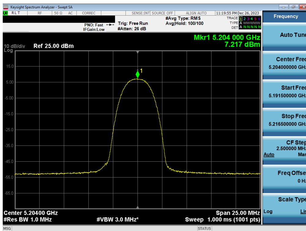
Plot 7-92. FCC PSD Antenna WF7b (HDR4, ePA – 5204MHz)
