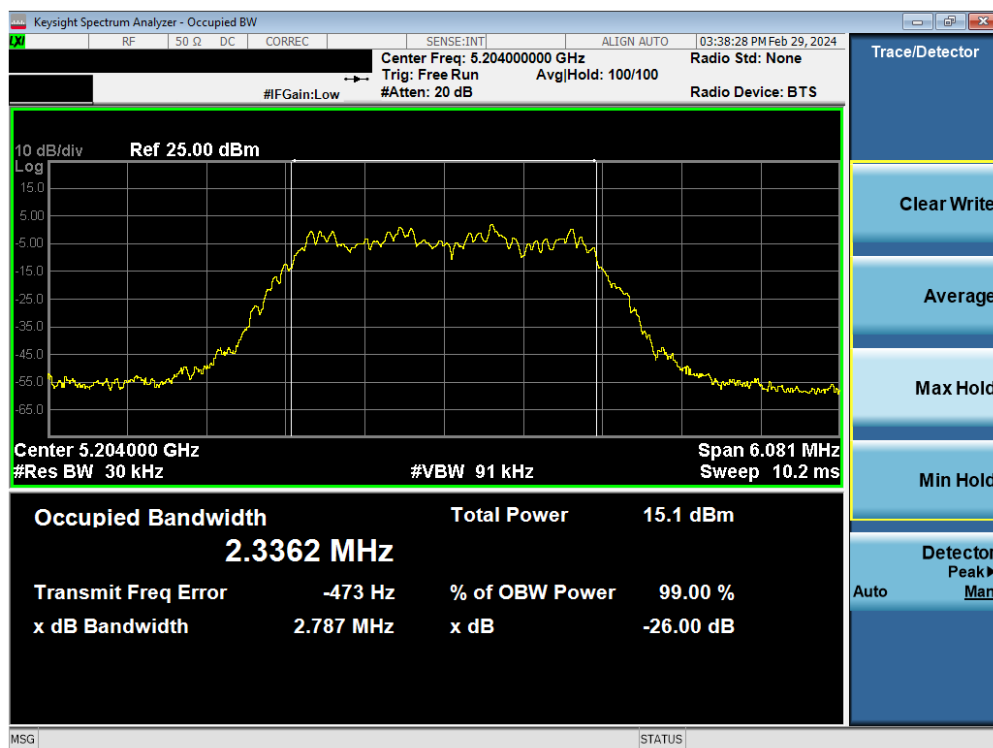
Plot 7-8. 26dB BW & 99% OBW Antenna WF2a (HDR4, ePA- 5204MHz)
