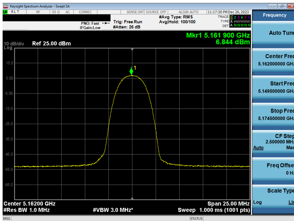
Plot 7-91. FCC PSD Antenna WF7b (HDR4, ePA – 5162MHz)
