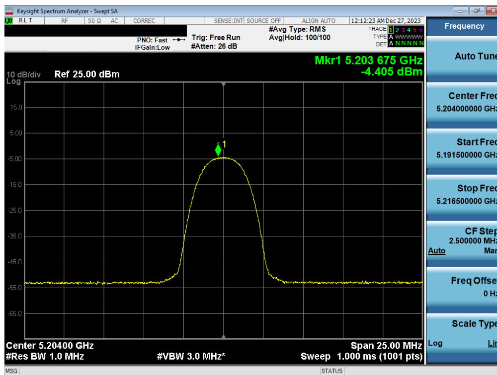
Plot 7-68. FCC/ISED PSD Antenna WF2a (HDR4, iPA – 5204MHz)
