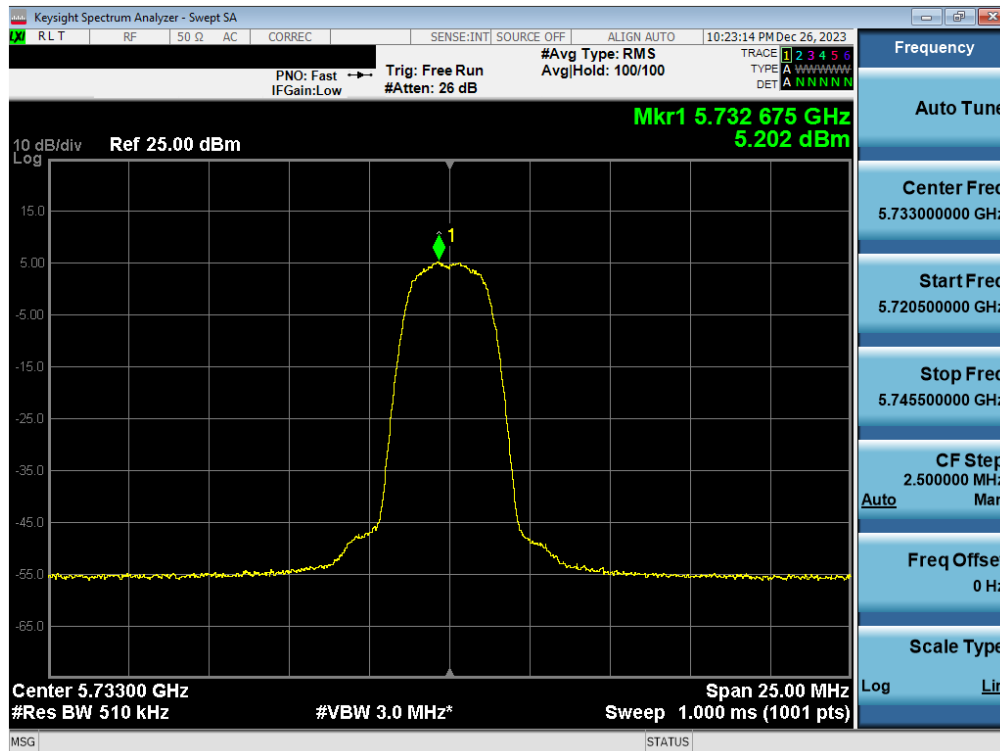
Plot 7-79. PSD Antenna WF2a (HDR4, ePA 5733MHz)
