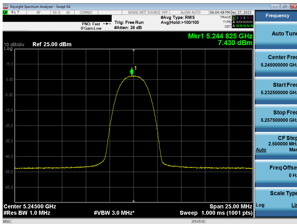
Plot 7-39. FCC PSD Antenna WF7a (HDR4, ePA- 5245MHz)
