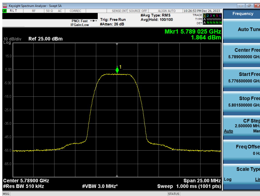
Plot 7-86. PSD Antenna WF2a (HDR8, ePA 5789MHz)
