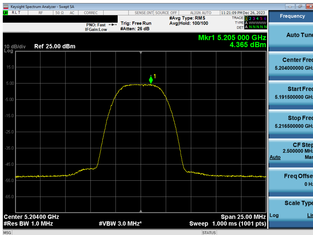
Plot 7-98. FCC/ISED PSD Antenna WF7b (HDR8, ePA – 5204MHz)
