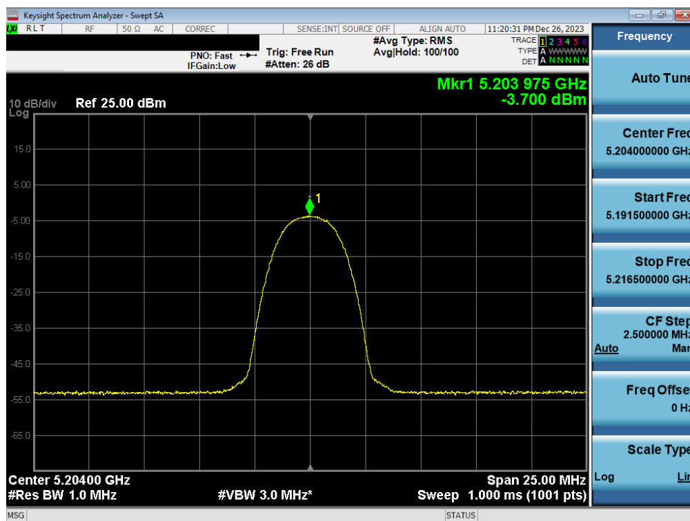
Plot 7-95. FCC/ISED PSD Antenna WF7b (HDR4, iPA – 5204MHz)
