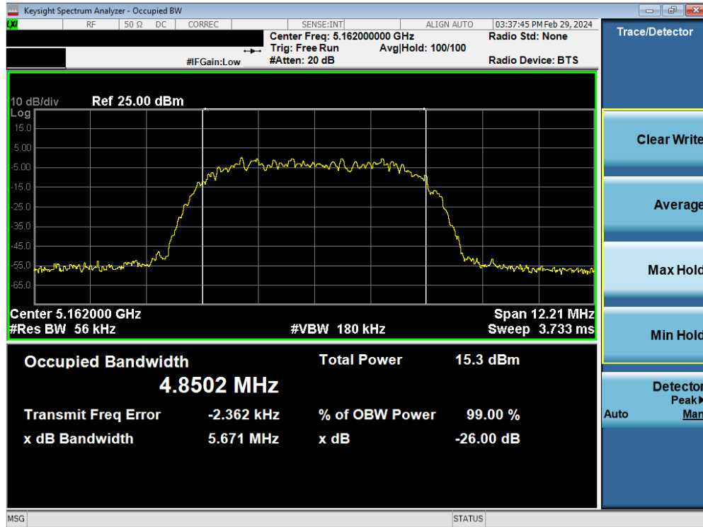
Plot 7-10. 26dB BW & 99% OBW Antenna WF2a (HDR8, ePA- 5162MHz)
