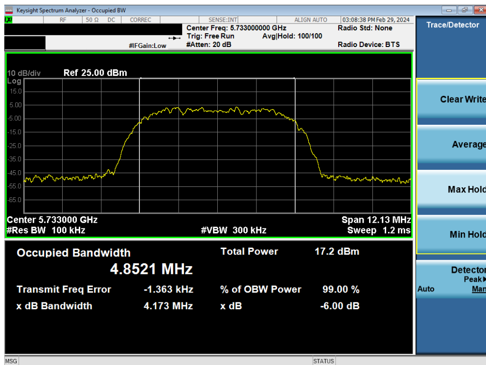
Plot 7-34. 6dB BW & 99% OBW Antenna WF7b (HDR8, ePA, 5733MHz)
