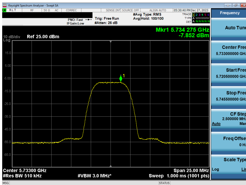
Plot 7-61. PSD Antenna WF7a (HDR8, iPA 5733MHz)
