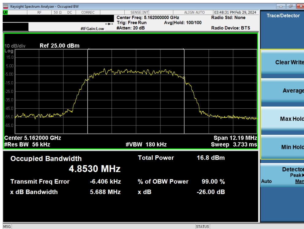
Plot 7-4. 26dB BW & 99% OBW Antenna WF7a (HDR8, ePA- 5162MHz)
