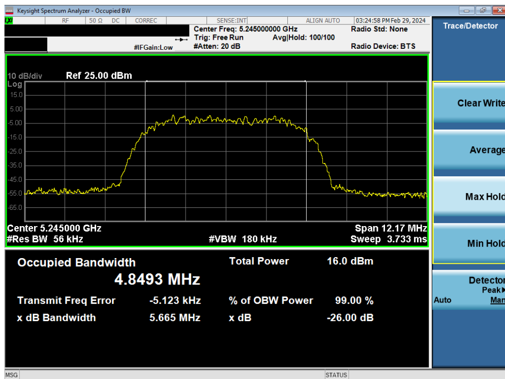
Plot 7-18. 26dB BW & 99% OBW Antenna WF7b (HDR8, ePA- 5245MHz)
