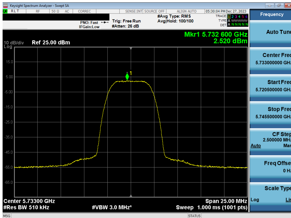
Plot 7-58. PSD Antenna WF7a (HDR8, ePA 5733MHz)
