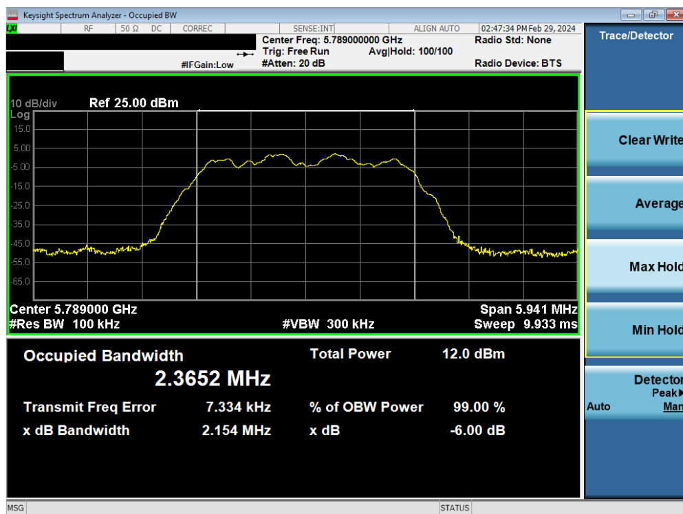
Plot 7-26. 6dB BW & 99% OBW Antenna WF2a (HDR4, ePA, 5789MHz)
