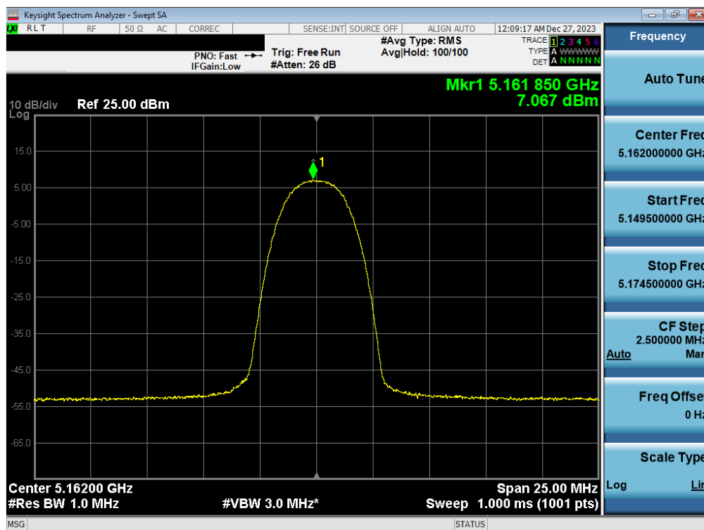
Plot 7-64. FCC PSD Antenna WF2a (HDR4, ePA – 5162MHz)
