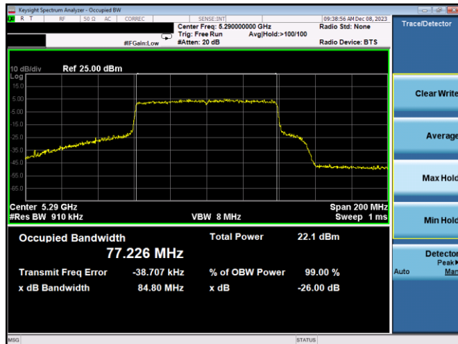
Plot 7-14. 26dB BW & 99% OBW Antenna WF7a (80MHz BW 802.11ax(SU) – Ch. 58, MCS2)
