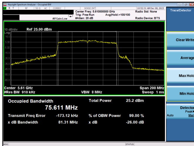
Plot 7-41. 26dB BW & 99% OBW Antenna WF7a (80MHz BW 802.11ac – Ch. 122, MCS4)
