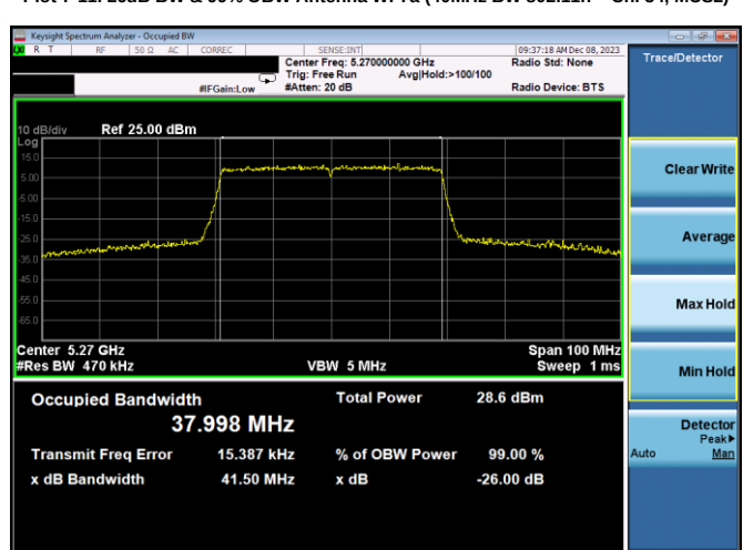
Plot 7-12. 26dB BW & 99% OBW Antenna WF7a (40MHz BW 802.11ax(SU) – Ch. 54, MCS2)
