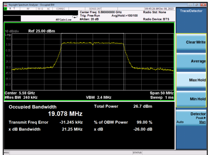
Plot 7-16. 26dB BW & 99% OBW Antenna WF7a (20MHz BW 802.11ax(SU) – Ch. 116, MCS2)
