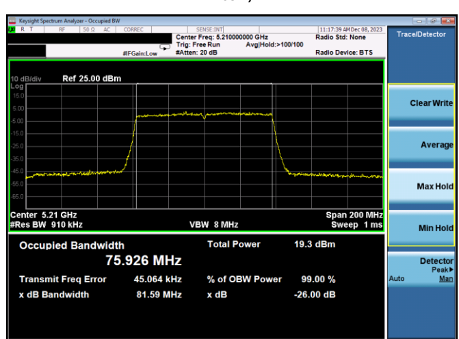
Plot 7-49. 26dB BW & 99% OBW Antenna WF7a (80MHz BW 802.11ac – Ch. 42, MCS9)
