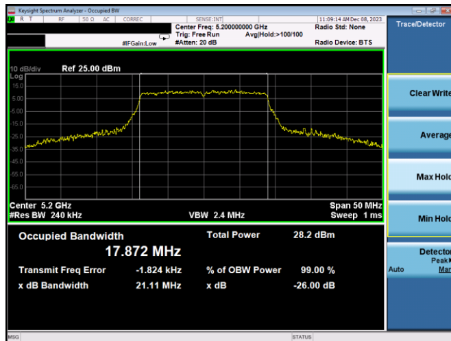
Plot 7-45. 26dB BW & 99% OBW Antenna WF7a (20MHz BW 802.11n – Ch. 40, MCS7)
