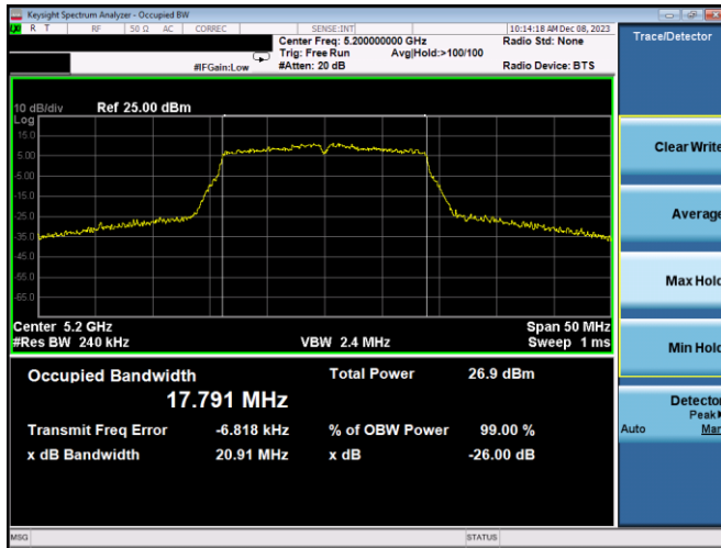
Plot 7-23. 26dB BW & 99% OBW Antenna WF7a (20MHz BW 802.11n – Ch. 40, MCS4)
