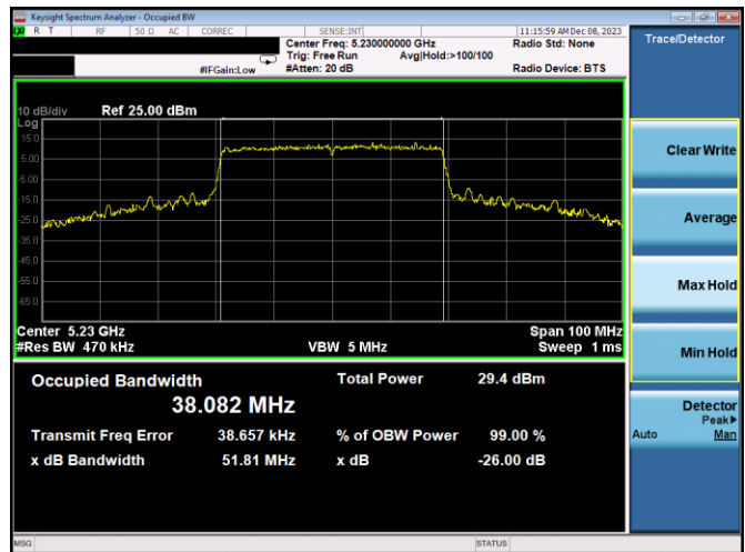
Plot 7-48. 26dB BW & 99% OBW Antenna WF7a (40MHz BW 802.11ax(SU) – Ch. 46, MCS11)
