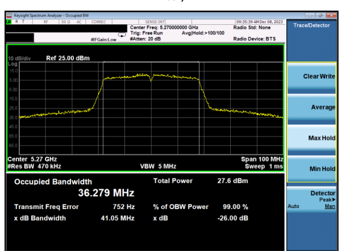
Plot 7-11. 26dB BW & 99% OBW Antenna WF7a (40MHz BW 802.11n – Ch. 54, MCS2)
