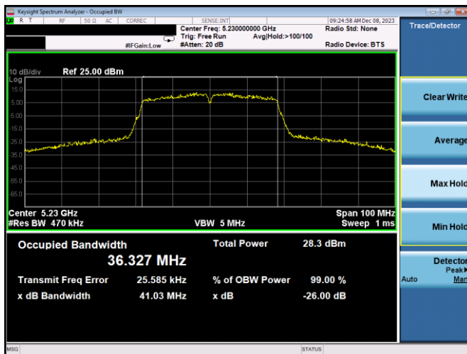
Plot 7-3. 26dB BW & 99% OBW Antenna WF7a (40MHz BW 802.11n – Ch. 46, MCS2)
