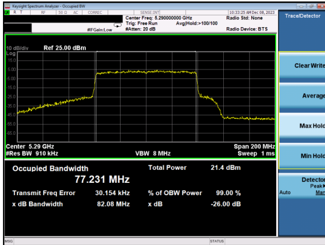
Plot 7-36. 26dB BW & 99% OBW Antenna WF7a (80MHz BW 802.11ax(SU) – Ch. 58, MCS4)
