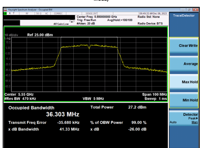
Plot 7-17. 26dB BW & 99% OBW Antenna WF7a (40MHz BW 802.11n – Ch. 110, MCS2)
