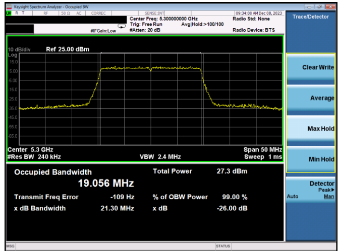
Plot 7-10. 26dB BW & 99% OBW Antenna WF7a (20MHz BW 802.11ax(SU) – Ch. 60, MCS2)
