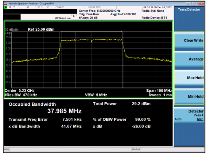
Plot 7-4. 26dB BW & 99% OBW Antenna WF7a (40MHz BW 802.11ax(SU) – Ch. 46, MCS2)
