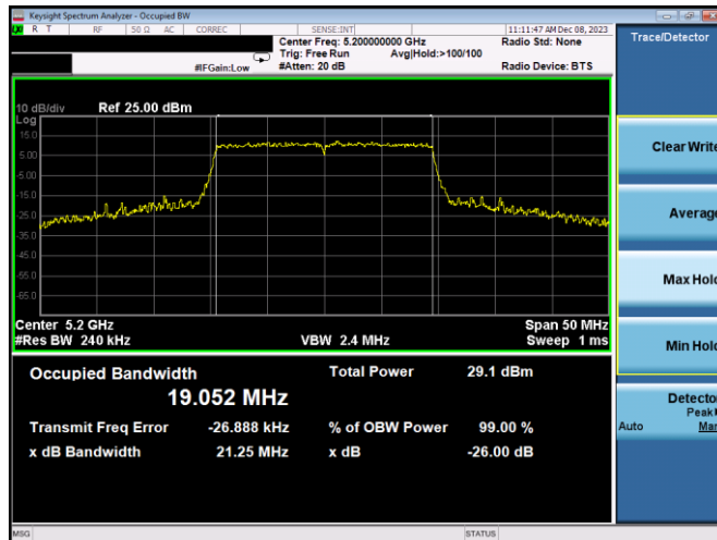
Plot 7-46. 26dB BW & 99% OBW Antenna WF7a (20MHz BW 802.11ax(SU) – Ch. 40, MCS11)
