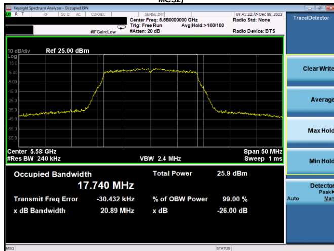
Plot 7-15. 26dB BW & 99% OBW Antenna WF7a (20MHz BW 802.11n – Ch. 116, MCS2)
