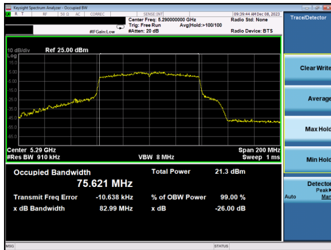
Plot 7-13. 26dB BW & 99% OBW Antenna WF7a (80MHz BW 802.11ac – Ch. 58, MCS2)
