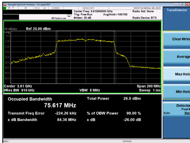
Plot 7-19. 26dB BW & 99% OBW Antenna WF7a (80MHz BW 802.11ac – Ch. 122, MCS2)
