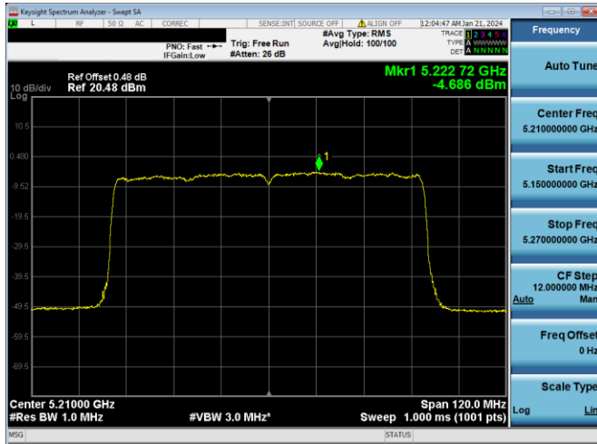
Plot 7-675. PSD CDD PRIMARY Antenna WF7a (80MHz BW 802.11ax(SU) - Ch. 42, MCS11)
