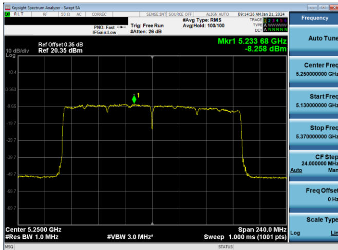
Plot 7-680. PSD CDD PRIMARY Antenna WF2a (160MHz BW 802.11ax(SU) - Ch. 50, MCS11)
