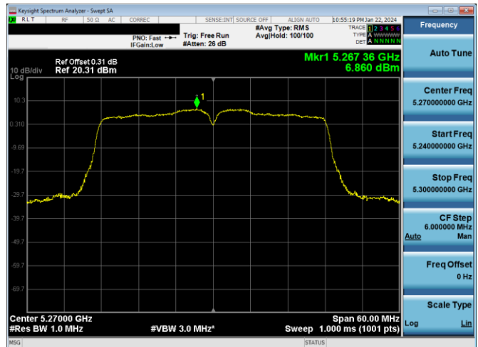
Plot 7-641. PSD CDD PRIMARY Antenna WF7a (40MHz BW 802.11n – Ch. 54, MCS12)
