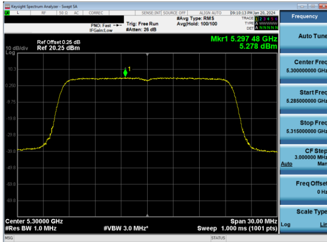
Plot 7-639. PSD CDD PRIMARY Antenna WF7a (20MHz BW 802.11ax(SU) – Ch. 60, MCS4)
