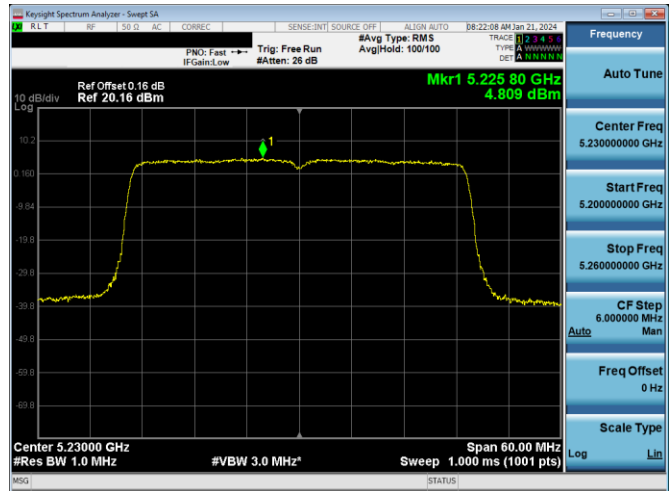
Plot 7-628. PSD CDD PRIMARY Antenna WF2a (40MHz BW 802.11ax(SU) – Ch. 46, MCS4)
