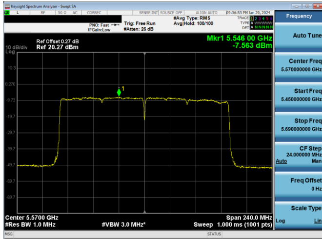
Plot 7-663. PSD CDD PRIMARY Antenna WF7a (160MHz BW 802.11ax(SU) - Ch. 114, MCS4)
