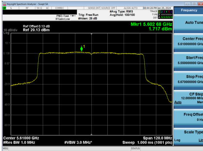
Plot 7-615. PSD CDD PRIMARY Antenna WF7a (80MHz BW 802.11ax(SU) – Ch. 122, MCS2)
