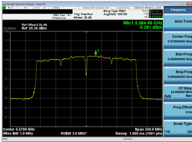
Plot 7-662. PSD CDD PRIMARY Antenna WF2a (160MHz BW 802.11ac - Ch. 114, MCS4)
