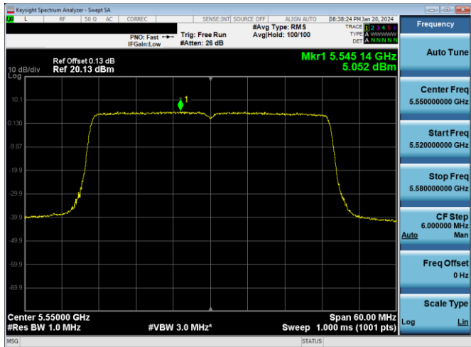
Plot 7-611. PSD CDD PRIMARY Antenna WF7a (40MHz BW 802.11ax(SU) – Ch. 110, MCS2)
