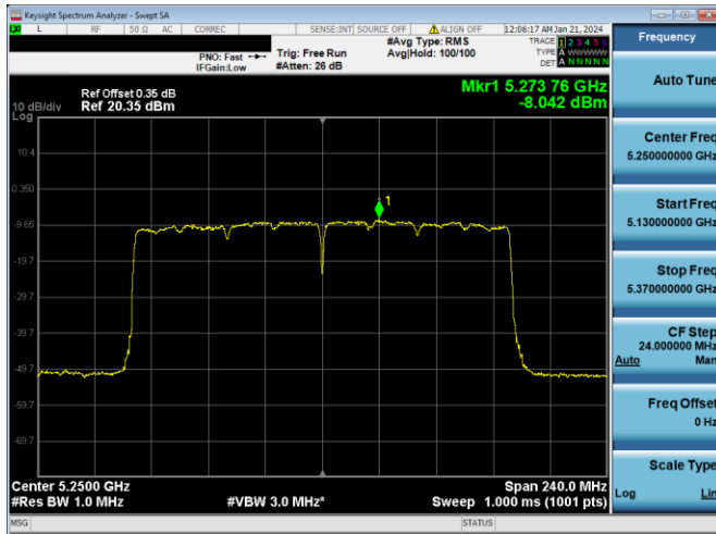
Plot 7-679. PSD CDD PRIMARY Antenna WF7a (160MHz BW 802.11ax(SU) - Ch. 50, MCS11)
