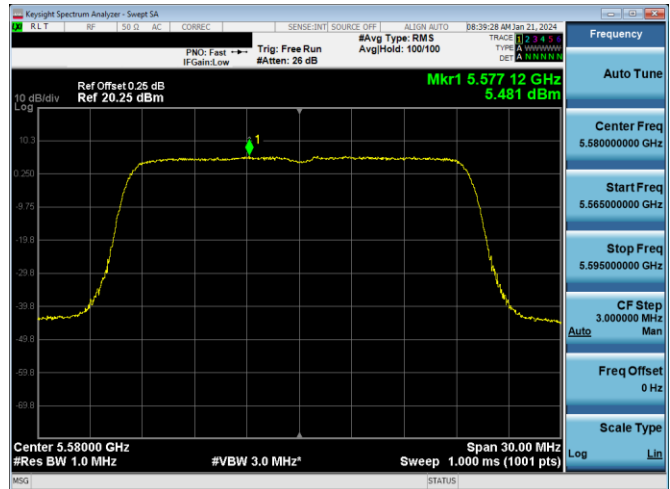
Plot 7-652. PSD CDD PRIMARY Antenna WF2a (20MHz BW 802.11ax(SU) - Ch. 116, MCS4)
