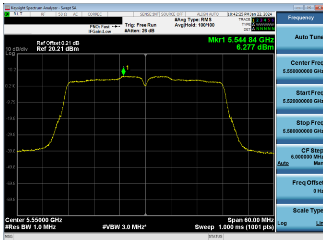
Plot 7-609. PSD CDD PRIMARY Antenna WF7a (40MHz BW 802.11n – Ch. 110, MCS10)
