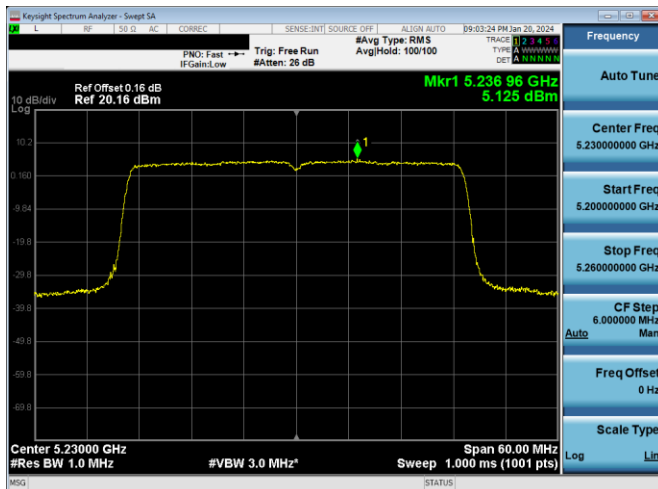
Plot 7-627. PSD CDD PRIMARY Antenna WF7a (40MHz BW 802.11ax(SU) – Ch. 46, MCS4)
