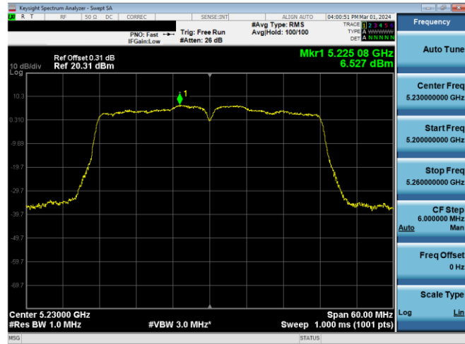
Plot 7-626. PSD CDD PRIMARY Antenna WF2a (40MHz BW 802.11n – Ch. 46, MCS12)
