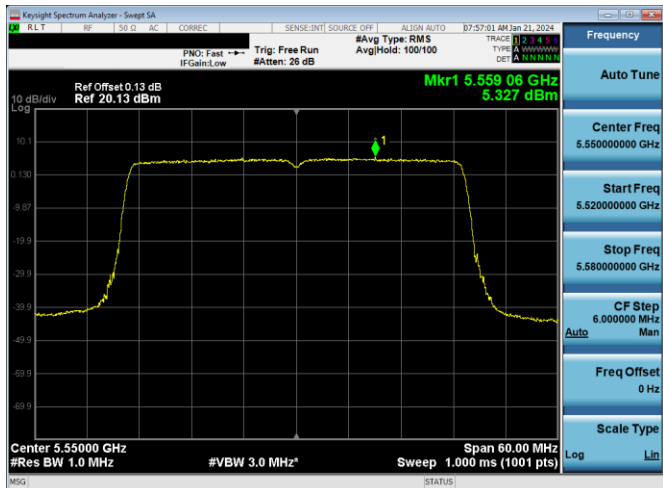
Plot 7-612. PSD CDD PRIMARY Antenna WF2a (40MHz BW 802.11ax(SU) – Ch. 110, MCS2)
