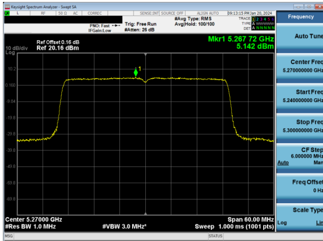
Plot 7-643. PSD CDD PRIMARY Antenna WF7a (40MHz BW 802.11ax(SU) – Ch. 54, MCS4)
