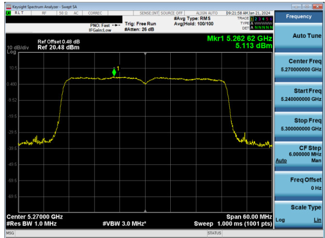
Plot 7-688. PSD CDD PRIMARY Antenna WF2a (40MHz BW 802.11ax(SU) – Ch. 54, MCS11)
