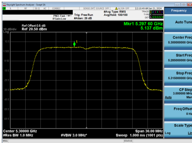
Plot 7-681. PSD CDD PRIMARY Antenna WF7a (20MHz BW 802.11n - Ch. 60, MCS15)
