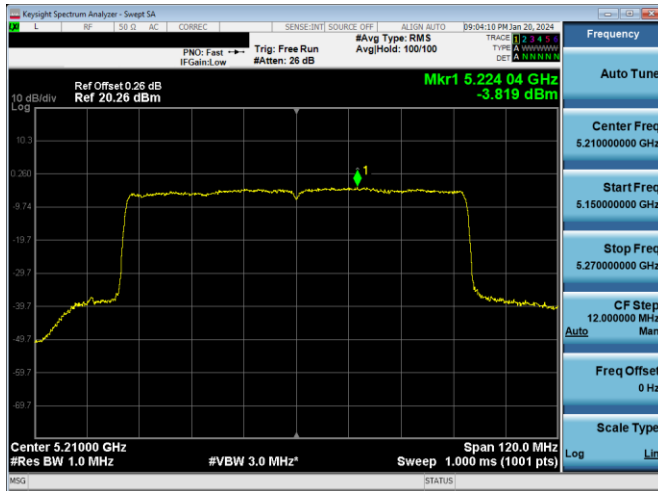
Plot 7-631. PSD CDD PRIMARY Antenna WF7a (80MHz BW 802.11ax(SU) – Ch. 42, MCS4)
