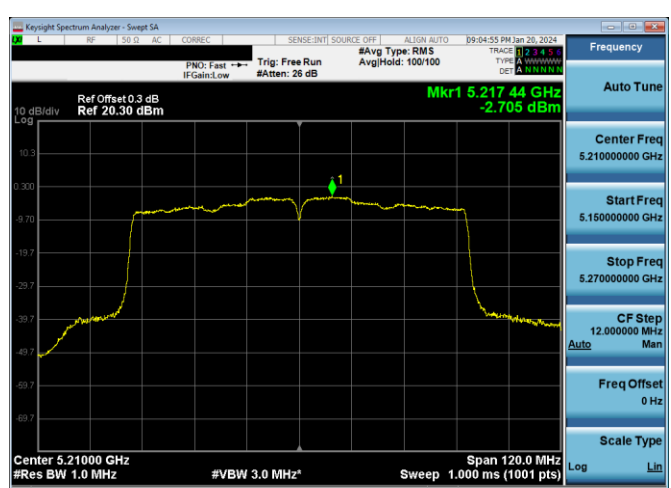
Plot 7-629. PSD CDD PRIMARY Antenna WF7a (80MHz BW 802.11ac – Ch. 42, MCS4)
