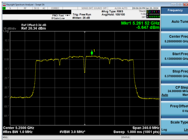
Plot 7-633. PSD CDD PRIMARY Antenna WF7a (160MHz BW 802.11ac – Ch. 50, MCS4)
