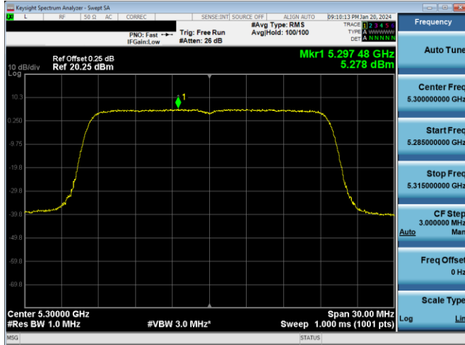
Plot 7-637. PSD CDD PRIMARY Antenna WF7a (20MHz BW 802.11n – Ch. 60, MCS12)
