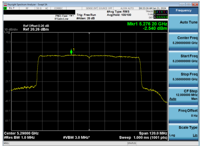
Plot 7-648. PSD CDD PRIMARY Antenna WF2a (80MHz BW 802.11ax(SU) – Ch. 58, MCS4)
