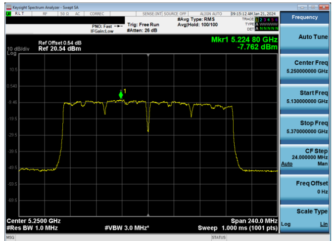
Plot 7-678. PSD CDD PRIMARY Antenna WF2a (160MHz BW 802.11ac - Ch. 50, MCS9)
