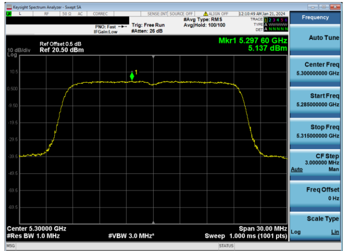
Plot 7-683. PSD CDD PRIMARY Antenna WF7a (20MHz BW 802.11ax(SU) - Ch. 60, MCS11)
