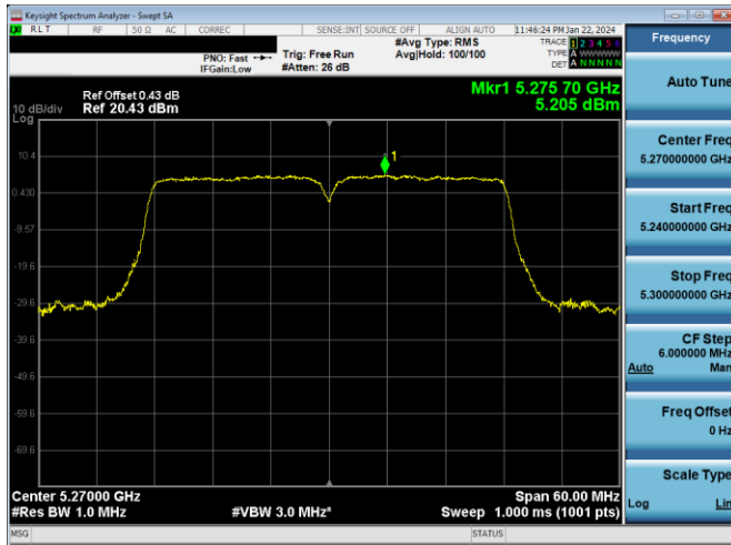
Plot 7-685. PSD CDD PRIMARY Antenna WF7a (40MHz BW 802.11n – Ch. 54, MCS15)
