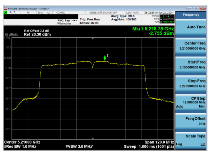
Plot 7-630. PSD CDD PRIMARY Antenna WF2a (80MHz BW 802.11ac – Ch. 42, MCS4)
