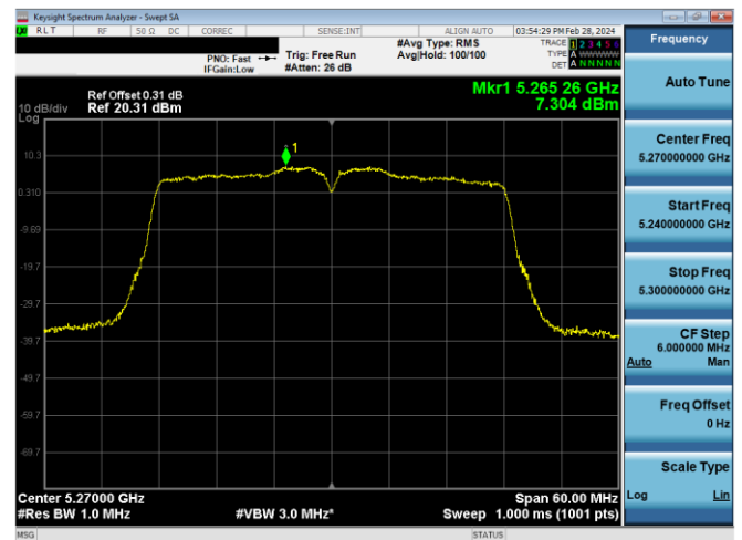
Plot 7-642. PSD CDD PRIMARY Antenna WF2a (40MHz BW 802.11n – Ch. 54, MCS12)
