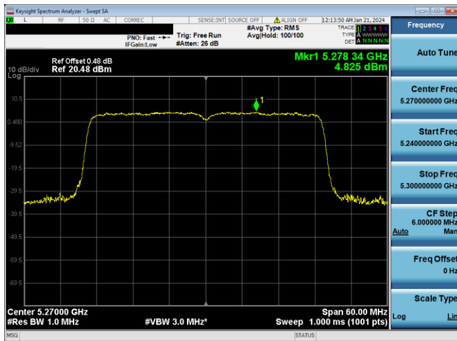
Plot 7-687. PSD CDD PRIMARY Antenna WF7a (40MHz BW 802.11ax(SU) – Ch. 54, MCS11)
