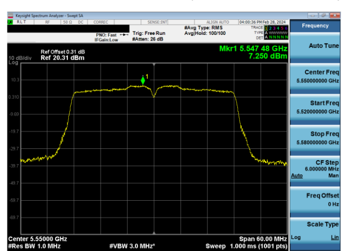
Plot 7-654. PSD CDD PRIMARY Antenna WF2a (40MHz BW 802.11n - Ch. 110, MCS12)
