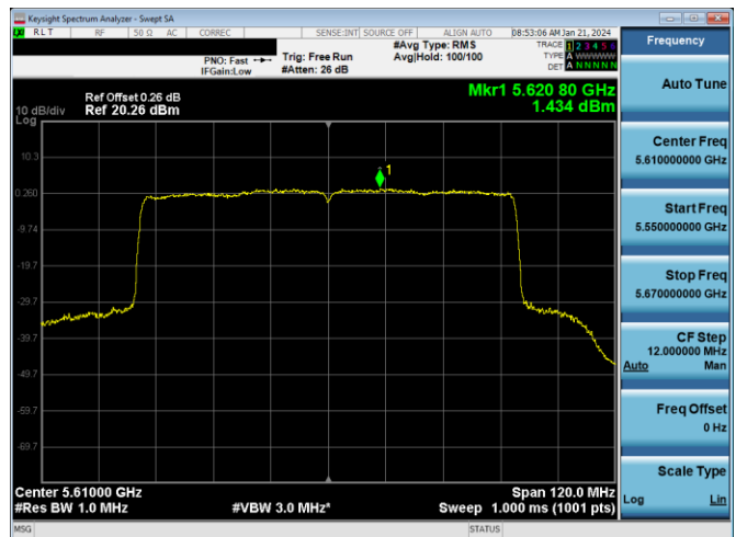
Plot 7-660. PSD CDD PRIMARY Antenna WF2a (80MHz BW 802.11ax(SU) – Ch. 122, MCS4)
