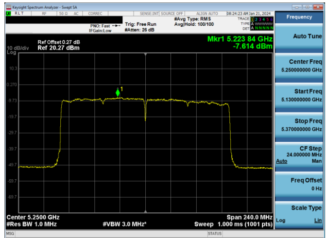
Plot 7-636. PSD CDD PRIMARY Antenna WF2a (160MHz BW 802.11ax(SU) – Ch. 50, MCS4)
