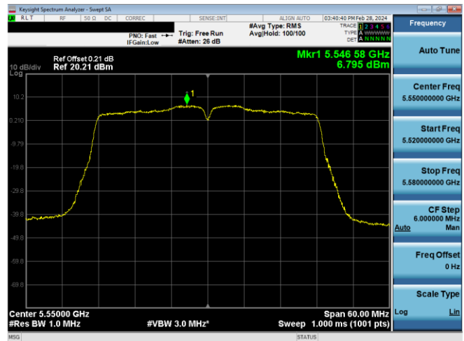
Plot 7-610. PSD CDD PRIMARY Antenna WF2a (40MHz BW 802.11n – Ch. 110, MCS10)
