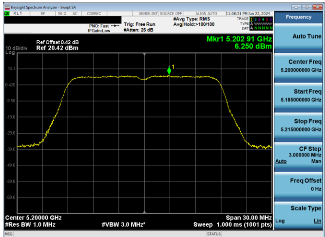
Plot 7-665. PSD CDD PRIMARY Antenna WF7a (20MHz BW 802.11n - Ch. 40, MCS15)
