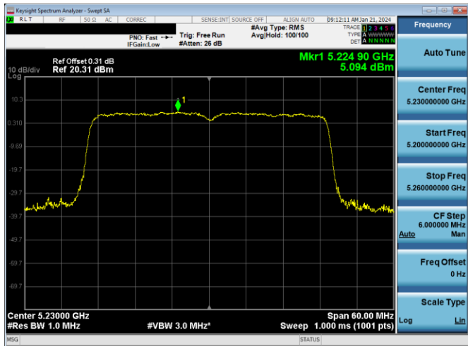
Plot 7-672. PSD CDD PRIMARY Antenna WF2a (40MHz BW 802.11ax(SU) – Ch. 46, MCS11)
