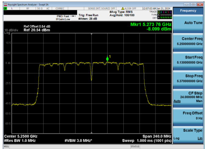
Plot 7-677. PSD CDD PRIMARY Antenna WF7a (160MHz BW 802.11ac - Ch. 50, MCS9)
