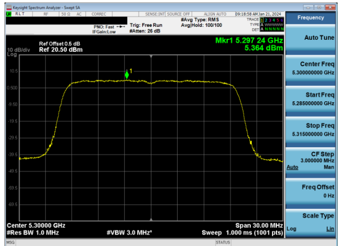
Plot 7-684. PSD CDD PRIMARY Antenna WF2a (20MHz BW 802.11ax(SU) - Ch. 60, MCS11)
