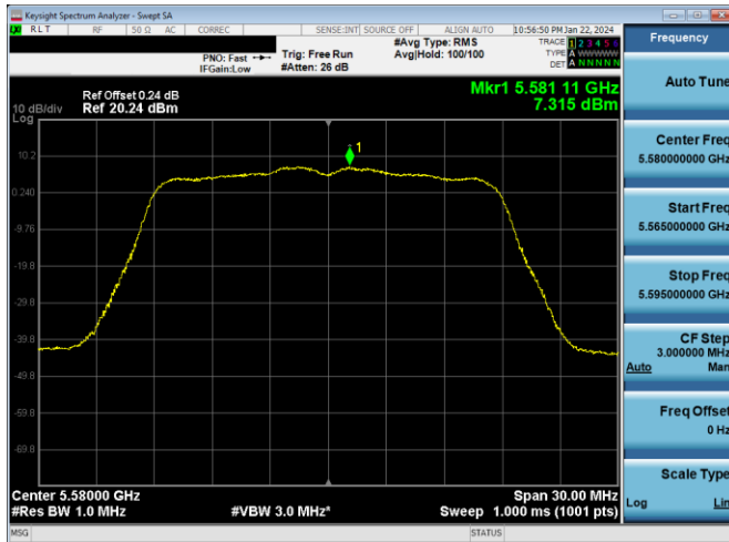
Plot 7-649. PSD CDD PRIMARY Antenna WF7a (20MHz BW 802.11n - Ch. 116, MCS12)
