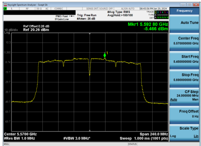
Plot 7-617. PSD CDD PRIMARY Antenna WF7a (160MHz BW 802.11ac – Ch. 114, MCS2)
