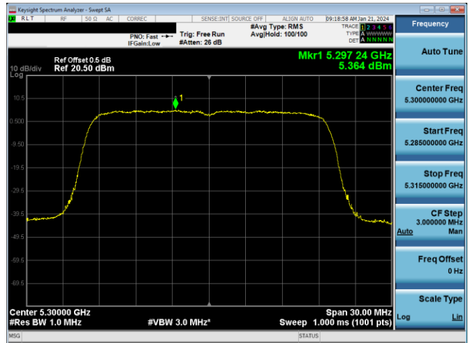
Plot 7-682. PSD CDD PRIMARY Antenna WF2a (20MHz BW 802.11n - Ch. 60, MCS15)
