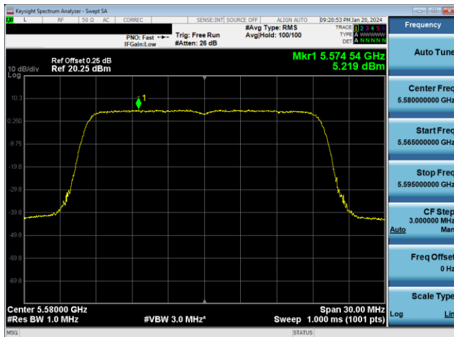
Plot 7-651. PSD CDD PRIMARY Antenna WF7a (20MHz BW 802.11ax(SU) - Ch. 116, MCS4)
