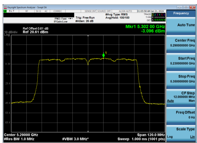
Plot 7-689. PSD CDD PRIMARY Antenna WF7a (80MHz BW 802.11ac – Ch. 58, MCS9)
