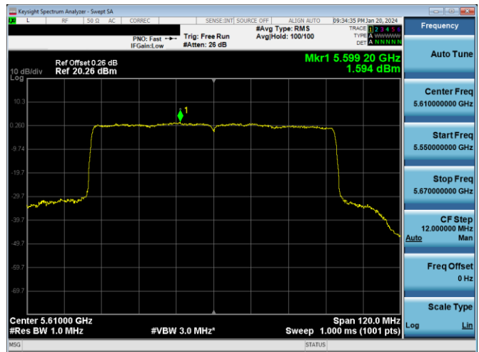
Plot 7-659. PSD CDD PRIMARY Antenna WF7a (80MHz BW 802.11ax(SU) – Ch. 122, MCS4)
