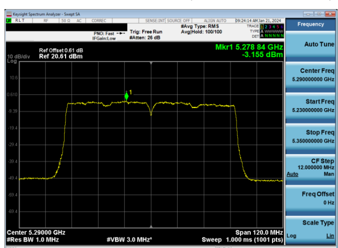
Plot 7-690. PSD CDD PRIMARY Antenna WF2a (80MHz BW 802.11ac – Ch. 58, MCS9)
