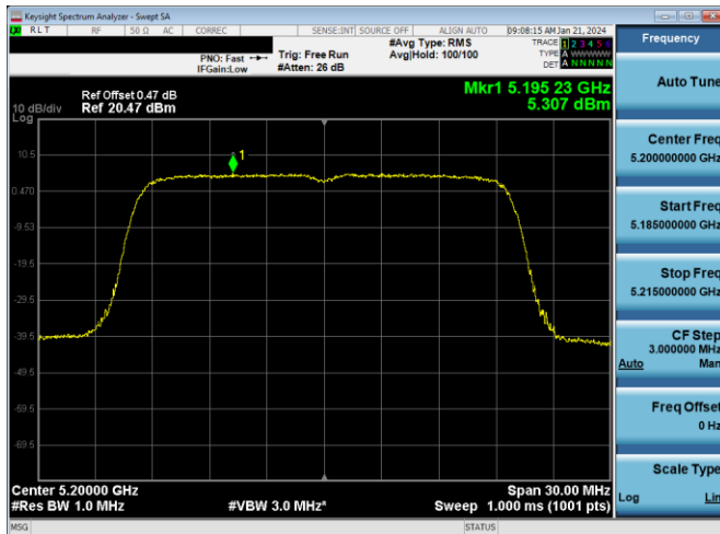
Plot 7-668. PSD CDD PRIMARY Antenna WF2a (20MHz BW 802.11ax(SU) – Ch. 40, MCS11)
