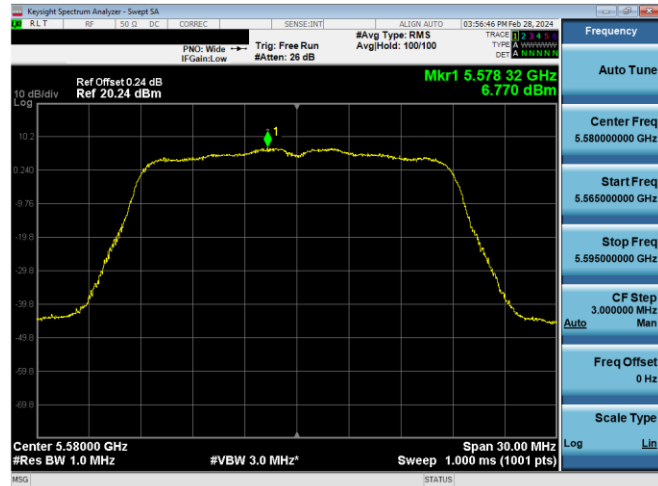
Plot 7-650. PSD CDD PRIMARY Antenna WF2a (20MHz BW 802.11n - Ch. 116, MCS12)
