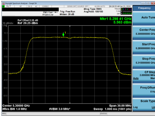
Plot 7-638. PSD CDD PRIMARY Antenna WF2a (20MHz BW 802.11n – Ch. 60, MCS12)
