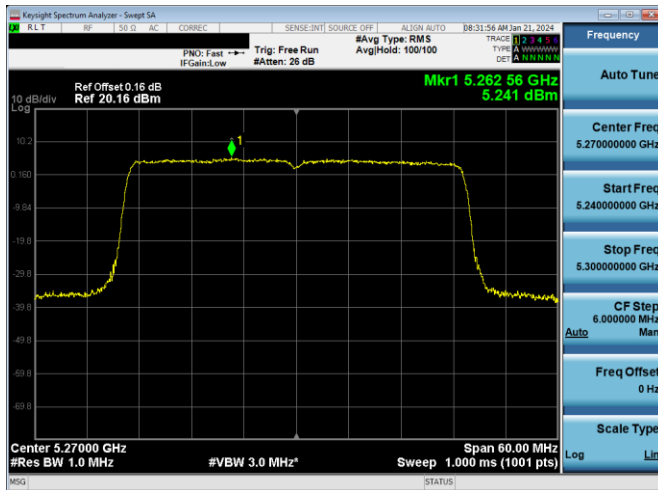
Plot 7-644. PSD CDD PRIMARY Antenna WF2a (40MHz BW 802.11ax(SU) – Ch. 54, MCS4)
