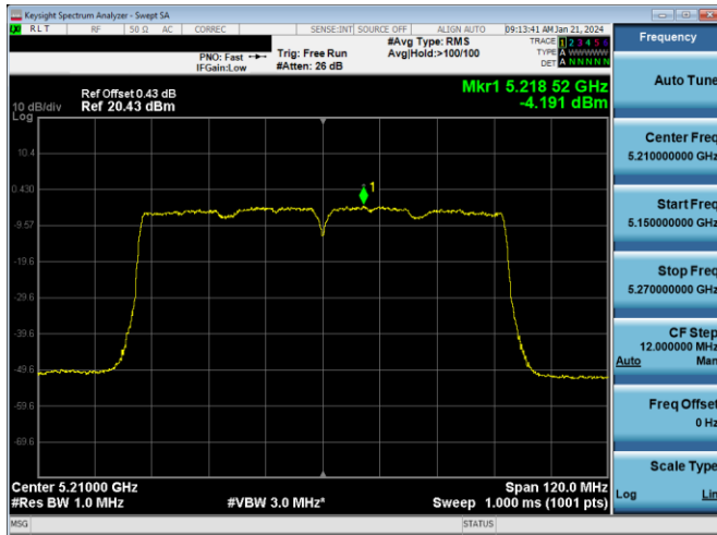
Plot 7-674. PSD CDD PRIMARY Antenna WF2a (80MHz BW 802.11ac - Ch. 42, MCS9)
