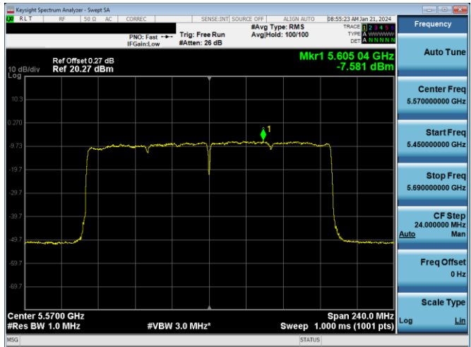
Plot 7-664. PSD CDD PRIMARY Antenna WF2a (160MHz BW 802.11ax(SU) - Ch. 114, MCS4)
