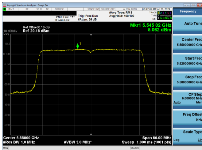
Plot 7-656. PSD CDD PRIMARY Antenna WF2a (40MHz BW 802.11ax(SU) – Ch. 110, MCS4)
