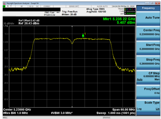
Plot 7-670. PSD CDD PRIMARY Antenna WF2a (40MHz BW 802.11n – Ch. 46, MCS15)
