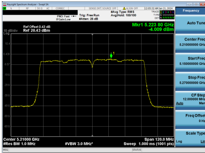
Plot 7-673. PSD CDD PRIMARY Antenna WF7a (80MHz BW 802.11ac - Ch. 42, MCS9)
