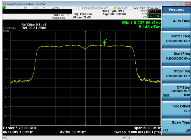
Plot 7-671. PSD CDD PRIMARY Antenna WF7a (40MHz BW 802.11ax(SU) – Ch. 46, MCS11)
