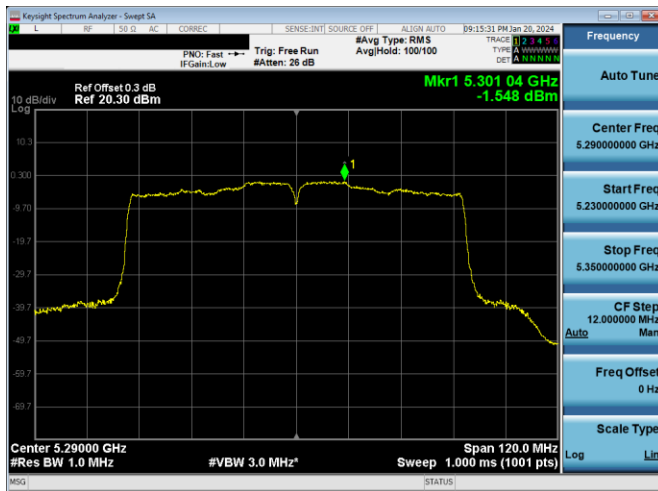
Plot 7-645. PSD CDD PRIMARY Antenna WF7a (80MHz BW 802.11ac – Ch. 58, MCS4)
