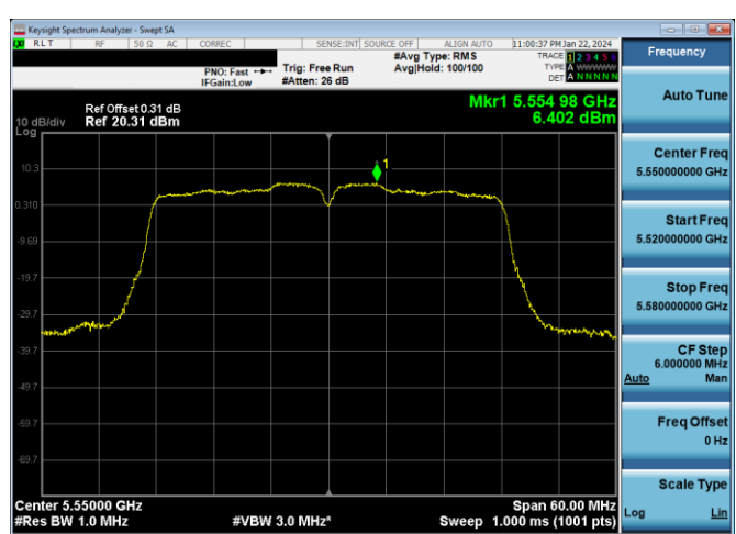
Plot 7-653. PSD CDD PRIMARY Antenna WF7a (40MHz BW 802.11n - Ch. 110, MCS12)
