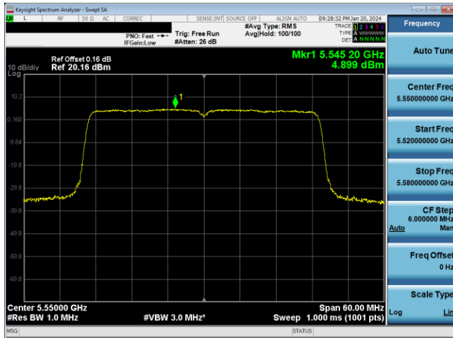
Plot 7-655. PSD CDD PRIMARY Antenna WF7a (40MHz BW 802.11ax(SU) – Ch. 110, MCS4)
