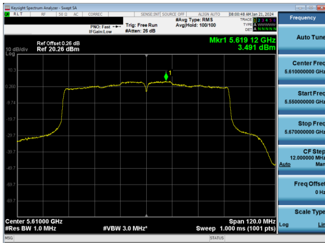
Plot 7-614. PSD CDD PRIMARY Antenna WF2a (80MHz BW 802.11ac – Ch. 122, MCS2)
