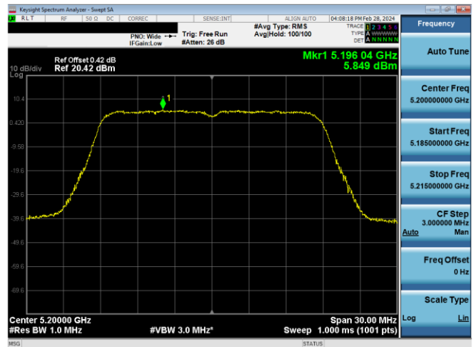
Plot 7-666. PSD CDD PRIMARY Antenna WF2a (20MHz BW 802.11n - Ch. 40, MCS15)
