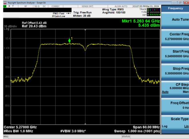
Plot 7-686. PSD CDD PRIMARY Antenna WF2a (40MHz BW 802.11n – Ch. 54, MCS15)
