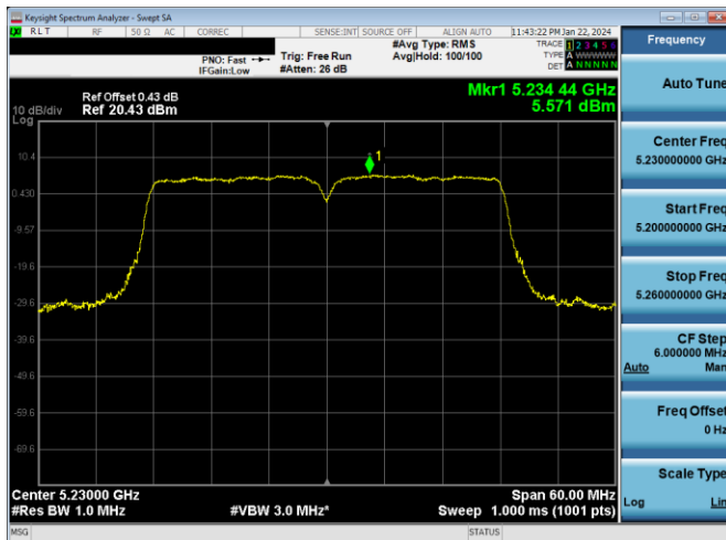
Plot 7-669. PSD CDD PRIMARY Antenna WF7a (40MHz BW 802.11n – Ch. 46, MCS15)
