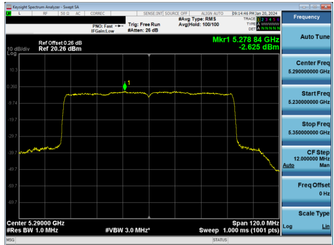
Plot 7-647. PSD CDD PRIMARY Antenna WF7a (80MHz BW 802.11ax(SU) – Ch. 58, MCS4)
