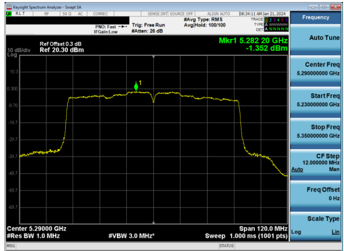
Plot 7-646. PSD CDD PRIMARY Antenna WF2a (80MHz BW 802.11ac – Ch. 58, MCS4)
