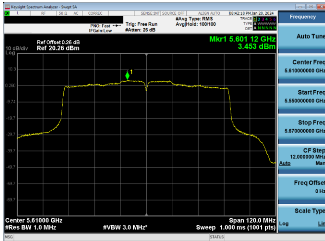
Plot 7-613. PSD CDD PRIMARY Antenna WF7a (80MHz BW 802.11ac – Ch. 122, MCS2)
