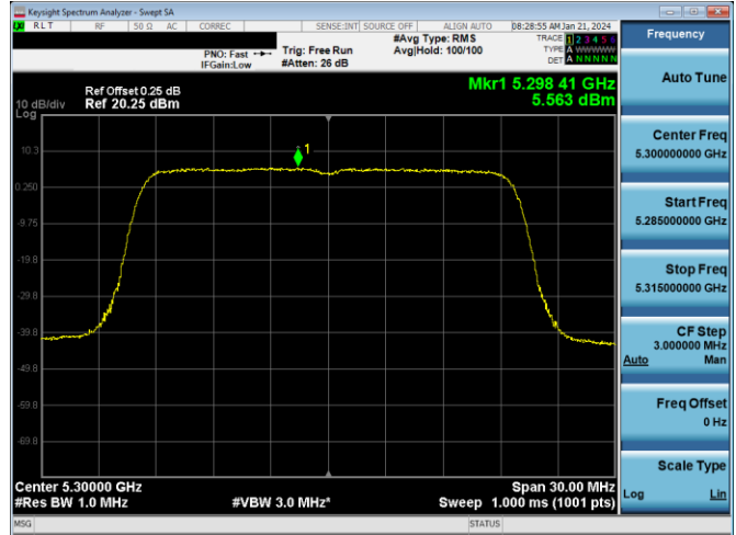
Plot 7-640. PSD CDD PRIMARY Antenna WF2a (20MHz BW 802.11ax(SU) – Ch. 60, MCS4)
