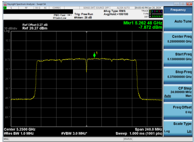
Plot 7-635. PSD CDD PRIMARY Antenna WF7a (160MHz BW 802.11ax(SU) – Ch. 50, MCS4)
