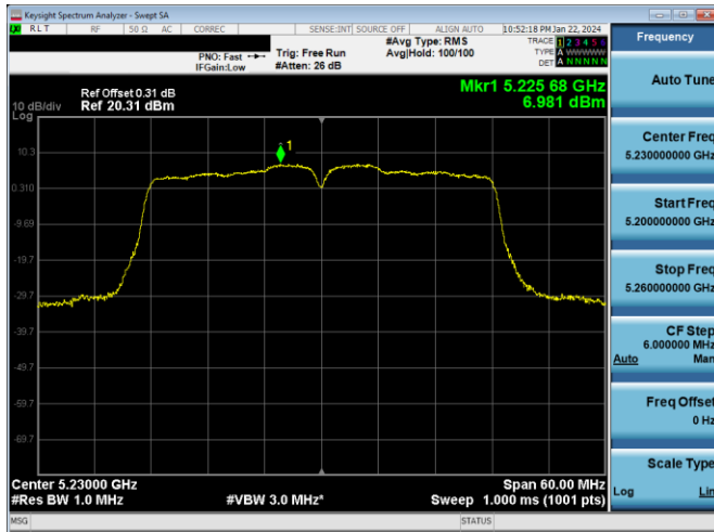
Plot 7-625. PSD CDD PRIMARY Antenna WF7a (40MHz BW 802.11n – Ch. 46, MCS12)
