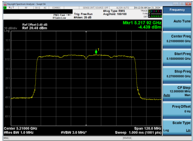
Plot 7-676. PSD CDD PRIMARY Antenna WF2a (80MHz BW 802.11ax(SU) - Ch. 42, MCS11)
