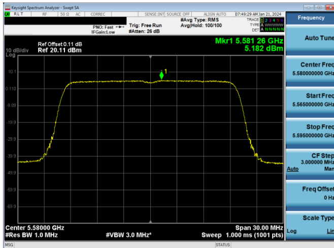
Plot 7-608. PSD CDD PRIMARY Antenna WF2a (20MHz BW 802.11ax(SU) – Ch. 116, MCS2)
