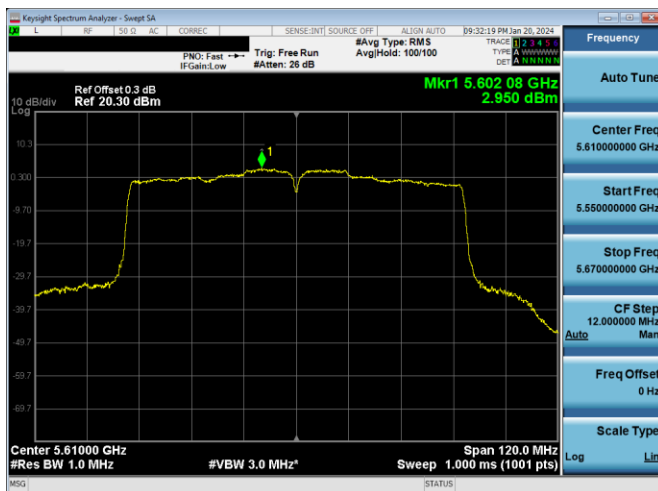
Plot 7-657. PSD CDD PRIMARY Antenna WF7a (80MHz BW 802.11ac – Ch. 122, MCS4)
