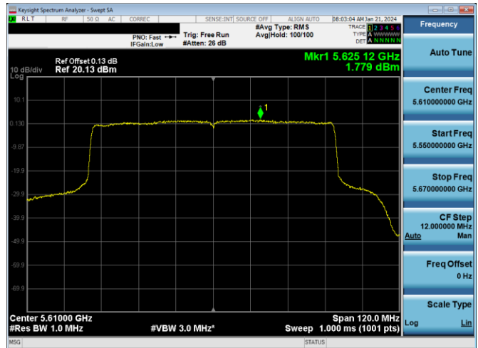
Plot 7-616. PSD CDD PRIMARY Antenna WF2a (80MHz BW 802.11ax(SU) – Ch. 122, MCS2)
