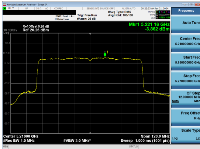
Plot 7-632. PSD CDD PRIMARY Antenna WF2a (80MHz BW 802.11ax(SU) – Ch. 42, MCS4)
