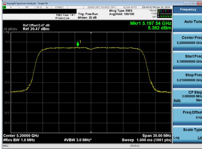
Plot 7-667. PSD CDD PRIMARY Antenna WF7a (20MHz BW 802.11ax(SU) – Ch. 40, MCS11)
