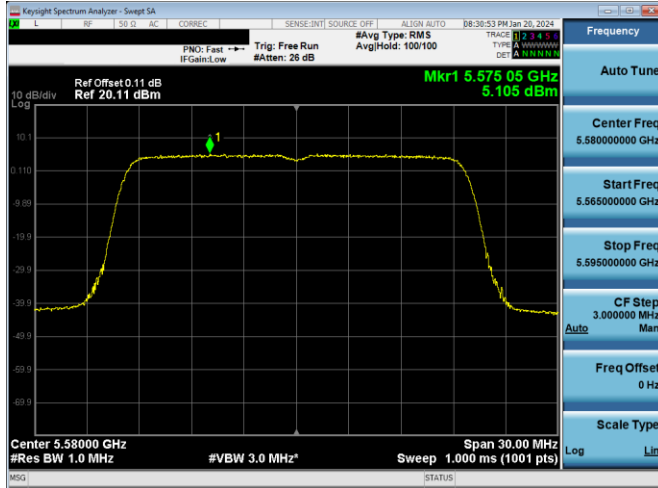
Plot 7-607. PSD CDD PRIMARY Antenna WF7a (20MHz BW 802.11ax(SU) – Ch. 116, MCS2)
