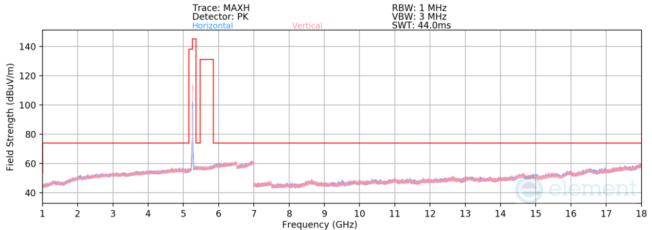
Plot 7-910. Radiated Spurious Emissions above 1GHz Antenna WF7a (802.11n – Ch. 52)
