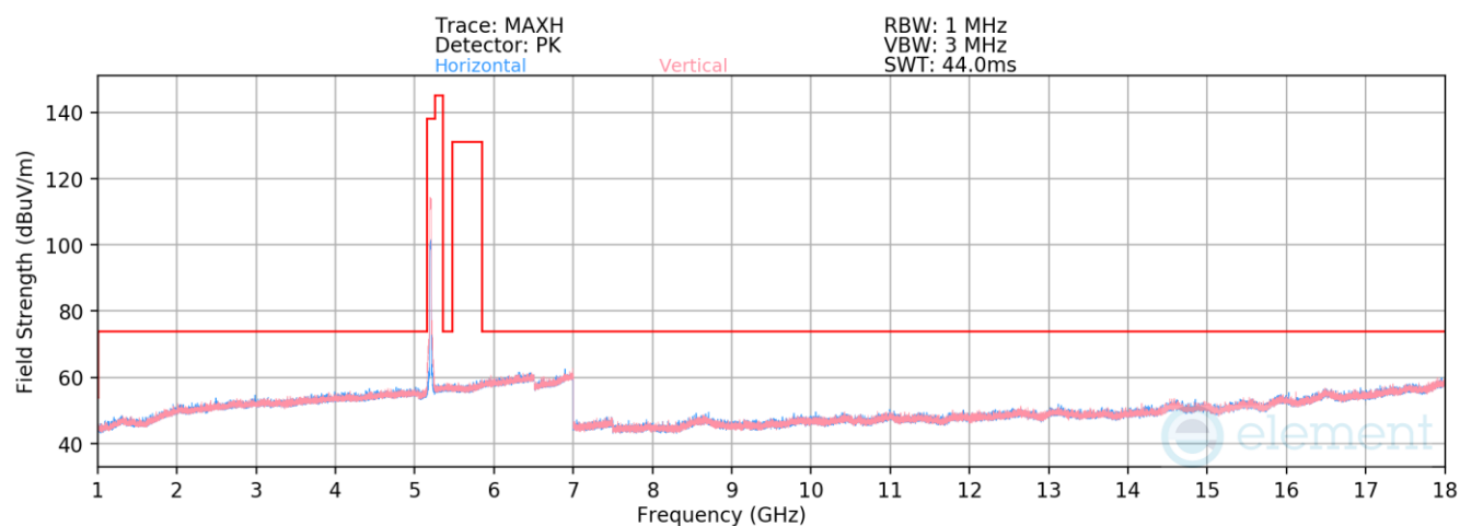
Plot 7-920. Radiated Spurious Emissions above 1GHz Antenna WF7a (802.11ax(SU) – Ch. 40)
