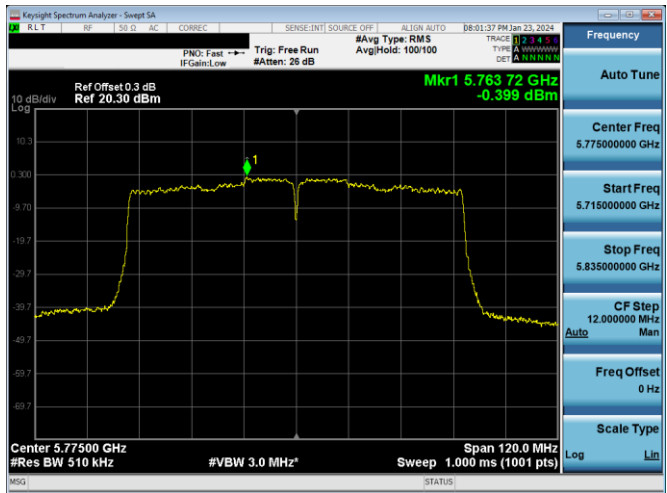
Plot 7-868. PSD CDD DIVERSITY Antenna WF2a (80MHz BW 802.11ac – Ch. 155, MCS4)
