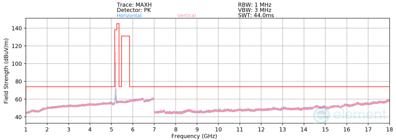
Plot 7-908. Radiated Spurious Emissions above 1GHz Antenna WF7a (802.11n – Ch. 40)
