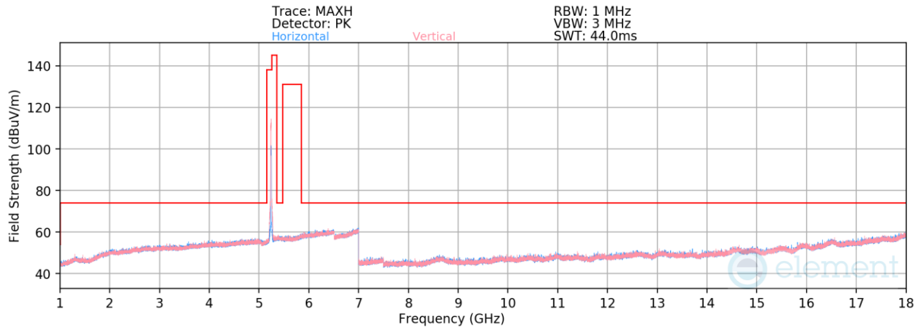
Plot 7-909. Radiated Spurious Emissions above 1GHz Antenna WF7a (802.11n – Ch. 48)
