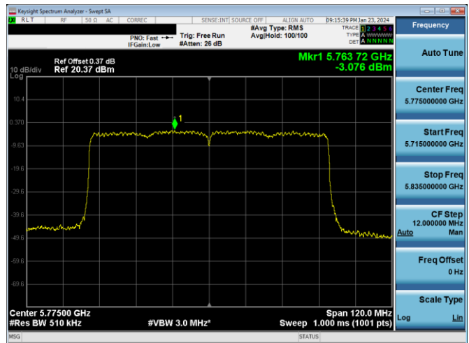
Plot 7-882. PSD CDD DIVERSITY Antenna WF2a (80MHz BW 802.11ax(SU) – Ch. 155, MCS11)
