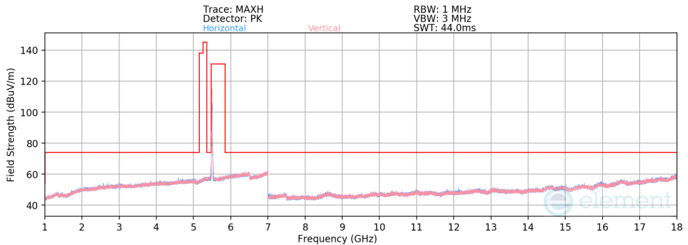
Plot 7-913. Radiated Spurious Emissions above 1GHz Antenna WF7a (802.11n – Ch. 100)
