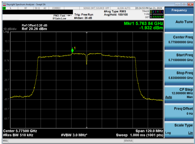
Plot 7-856. PSD CDD DIVERSITY Antenna WF2a (80MHz BW 802.11ac – Ch. 155, MCS2)
