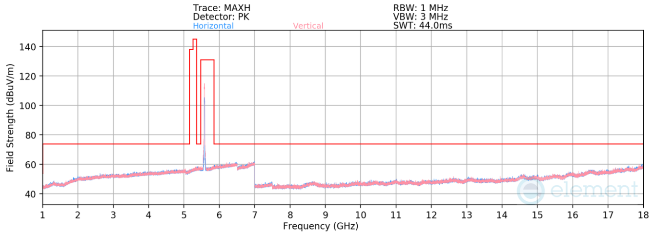
Plot 7-914. Radiated Spurious Emissions above 1GHz Antenna WF7a (802.11n – Ch. 116)
