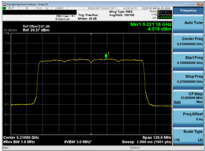
Plot 7-904. ISSED PSD CDD DIVERSITY Antenna WF2a (80MHz BW 11ax (SU) - Ch.42, MCS11)
