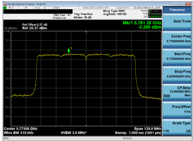
Plot 7-881. PSD CDD DIVERSITY Antenna WF7a (80MHz BW 802.11ax(SU) – Ch. 155, MCS11)
