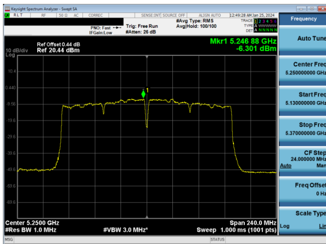
Plot 7-897. ISED PSD CDD DIVERSITY Antenna WF2a (160MHz BW 11ac – Ch.50, MCS4)
