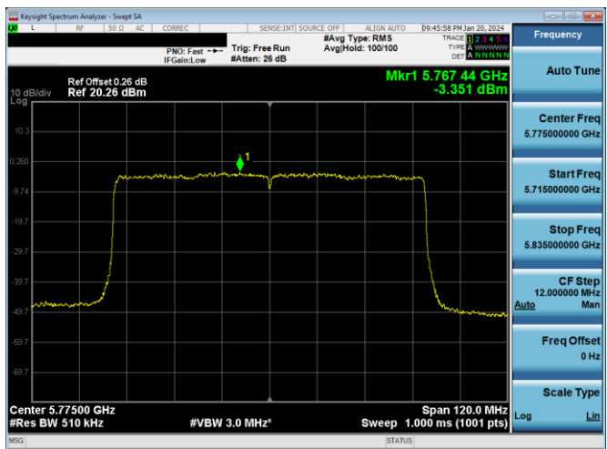
Plot 7-869. PSD CDD DIVERSITY Antenna WF7a (80MHz BW 802.11ax(SU) – Ch. 155, MCS4)
