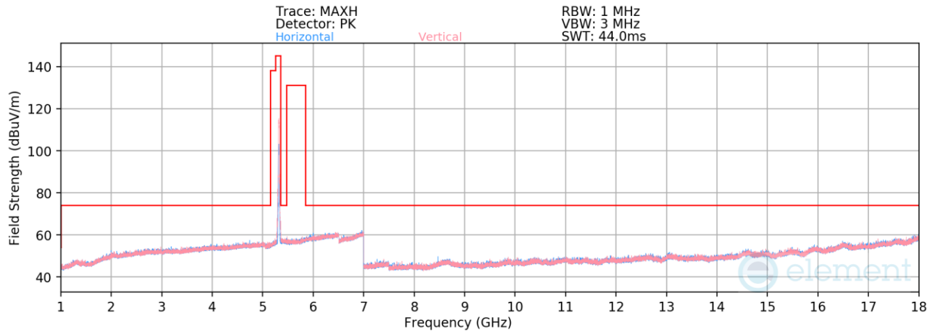
Plot 7-912. Radiated Spurious Emissions above 1GHz Antenna WF7a (802.11n – Ch. 64)
