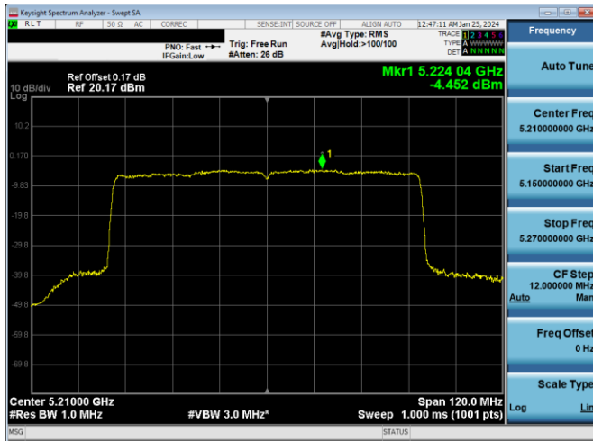
Plot 7-896. ISED PSD CDD DIVERSITY Antenna WF2a (80MHz BW 11ax (SU) – Ch.42, MCS4)
