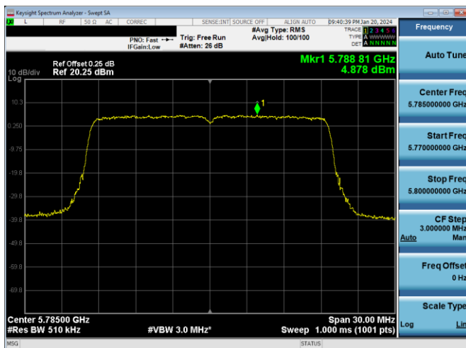
Plot 7-861. PSD CDD DIVERSITY Antenna WF7a (20MHz BW 802.11ax(SU) – Ch. 157, MCS4)
