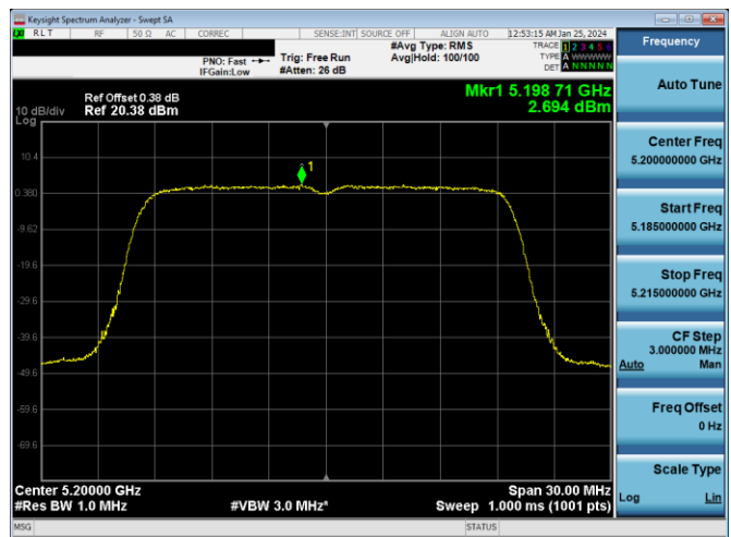
Plot 7-900. ISED PSD CDD DIVERSITY Antenna WF2a (20MHz BW 11ax(SU) – Ch.40, MCS11)
