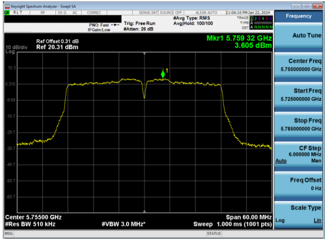
Plot 7-863. PSD CDD DIVERSITY Antenna WF7a (40MHz BW 802.11n – Ch. 151, MCS12)
