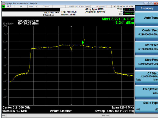
Plot 7-895. ISED PSD CDD DIVERSITY Antenna WF2a (80MHz BW 11ac – Ch.42, MCS4)
