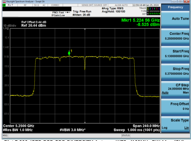
Plot 7-906. ISSED PSD CDD DIVERSITY Antenna WF2a (160MHz BW 11ax (SU) - Ch.50, MCS11)
