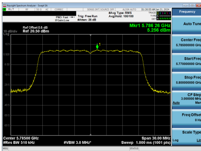
Plot 7-873. PSD CDD DIVERSITY Antenna WF7a (20MHz BW 802.11ax(SU) - Ch. 157, MCS11)
