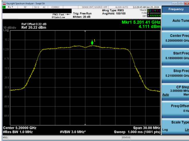
Plot 7-883. ISSED PSD SDM DIVERSITY Antenna WF2a (20MHz BW 11n – Ch.40, MCS10)
