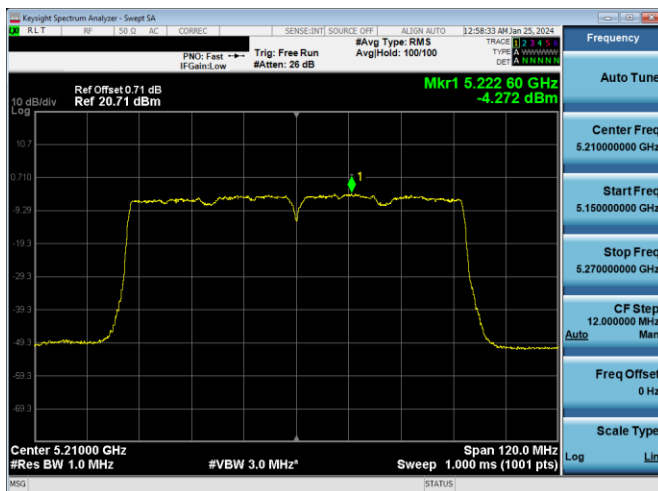
Plot 7-903. ISSED PSD CDD DIVERSITY Antenna WF2a (80MHz BW 11ac - Ch.42, MCS9)
