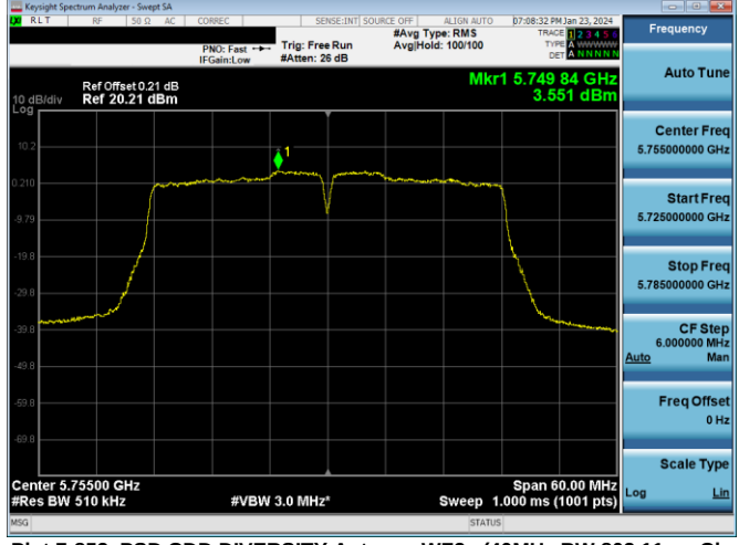
Plot 7-852. PSD CDD DIVERSITY Antenna WF2a (40MHz BW 802.11n - Ch. 151, MCS10)
