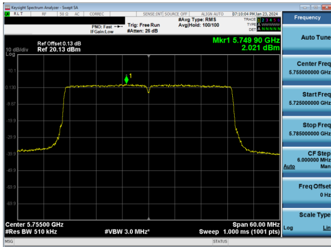
Plot 7-854. PSD CDD DIVERSITY Antenna WF2a (40MHz BW 802.11ax(SU) – Ch. 151, MCS2)
