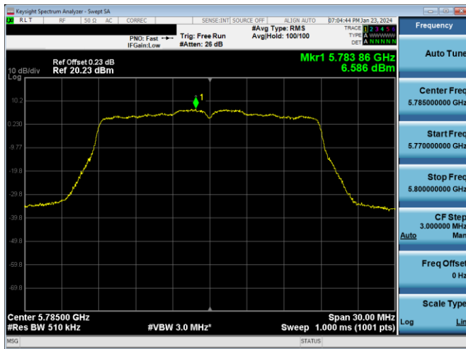
Plot 7-848. PSD CDD DIVERSITY Antenna WF2a (20MHz BW 802.11n - Ch. 157, MCS10)
