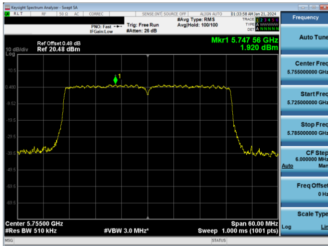
Plot 7-877. PSD CDD DIVERSITY Antenna WF7a (40MHz BW 802.11ax(SU) – Ch. 151, MCS11)
