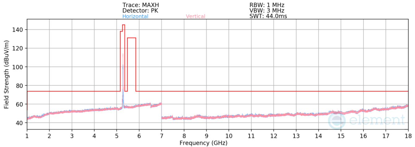
Plot 7-911. Radiated Spurious Emissions above 1GHz Antenna WF7a (802.11n – Ch. 56)
