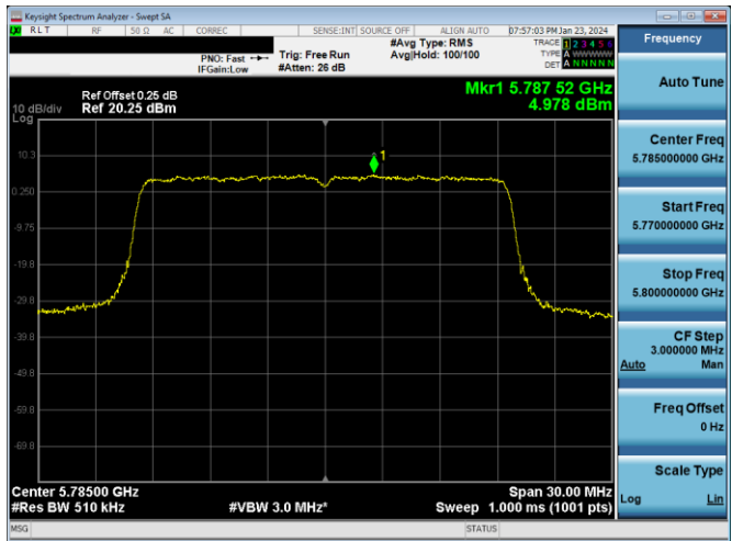
Plot 7-862. PSD CDD DIVERSITY Antenna WF2a (20MHz BW 802.11ax(SU) – Ch. 157, MCS4)
