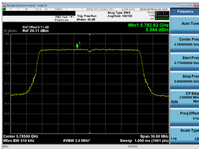
Plot 7-849. PSD CDD DIVERSITY Antenna WF7a (20MHz BW 802.11ax(SU) - Ch. 157, MCS2)
