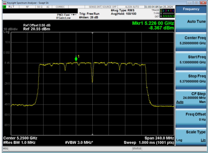
Plot 7-905. ISSED PSD CDD DIVERSITY Antenna WF2a (160MHz BW 11ac - Ch.50, MCS9)
