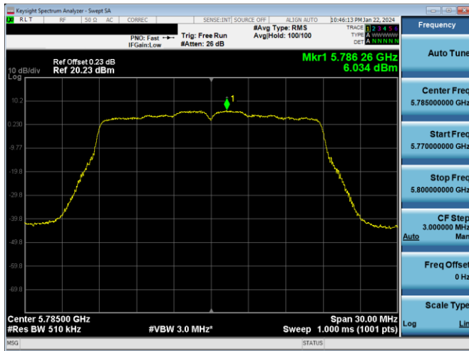
Plot 7-847. PSD CDD DIVERSITY Antenna WF7a (20MHz BW 802.11n - Ch. 157, MCS10)
