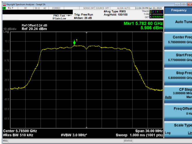
Plot 7-859. PSD CDD DIVERSITY Antenna WF7a (20MHz BW 802.11n – Ch. 157, MCS12)
