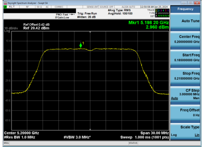
Plot 7-899. ISED PSD CDD DIVERSITY Antenna WF2a (20MHz BW 11n – Ch.40, MCS15)
