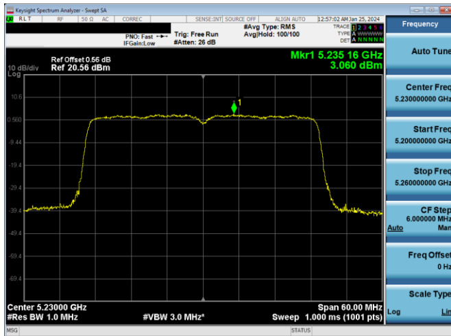
Plot 7-902. ISSED PSD SDM DIVERSITY Antenna WF2a (40MHz BW 11ax(SU) - Ch.46, MCS11)
