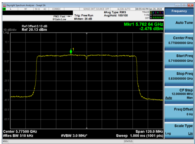
Plot 7-857. PSD CDD DIVERSITY Antenna WF7a (80MHz BW 802.11ax(SU) – Ch. 155, MCS2)
