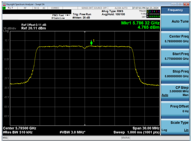
Plot 7-850. PSD CDD DIVERSITY Antenna WF2a (20MHz BW 802.11ax(SU) - Ch. 157, MCS2)
