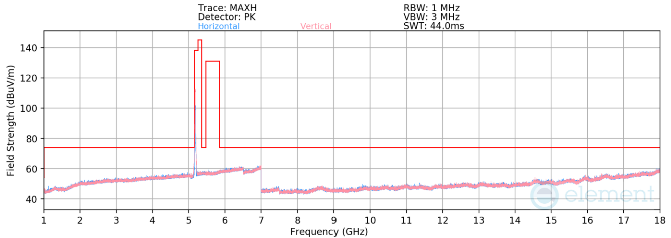
Plot 7-919. Radiated Spurious Emissions above 1GHz Antenna WF7a (802.11ax(SU) – Ch. 36)
