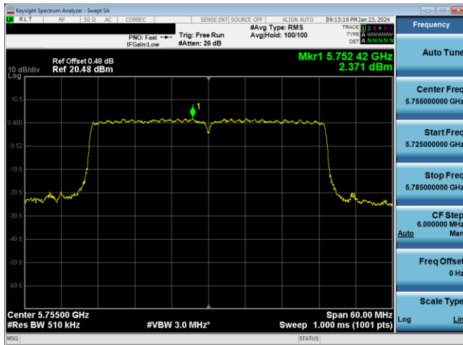
Plot 7-878. PSD CDD DIVERSITY Antenna WF2a (40MHz BW 802.11ax(SU) – Ch. 151, MCS11)
