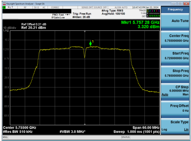
Plot 7-851. PSD CDD DIVERSITY Antenna WF7a (40MHz BW 802.11n - Ch. 151, MCS10)
