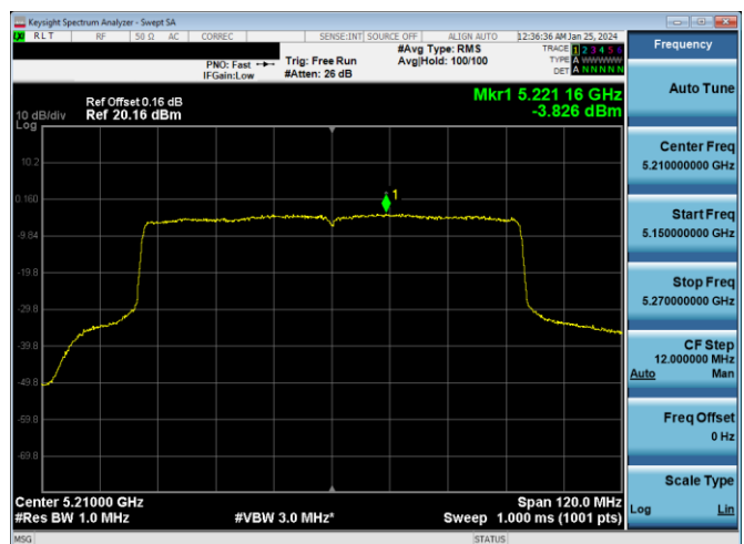
Plot 7-888. ISSED PSD CDD DIVERSITY Antenna WF2a (80MHz BW 11ax (SU) – Ch.42, MCS2)
