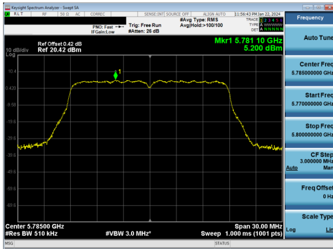
Plot 7-871. PSD CDD DIVERSITY Antenna WF7a (20MHz BW 802.11n - Ch. 157, MCS15)
