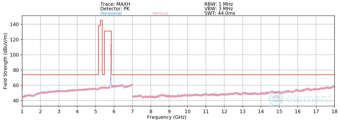
Plot 7-918. Radiated Spurious Emissions above 1GHz Antenna WF7a (802.11n – Ch. 165)
