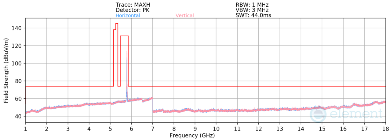
Plot 7-917. Radiated Spurious Emissions above 1GHz Antenna WF7a (802.11n – Ch. 157)
