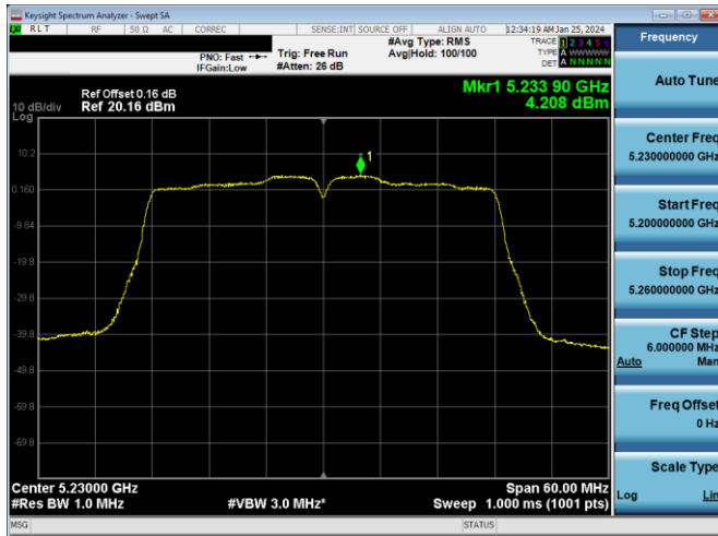
Plot 7-885. ISSED PSD SDM DIVERSITY Antenna WF2a (40MHz BW 11n – Ch.46, MCS10)
