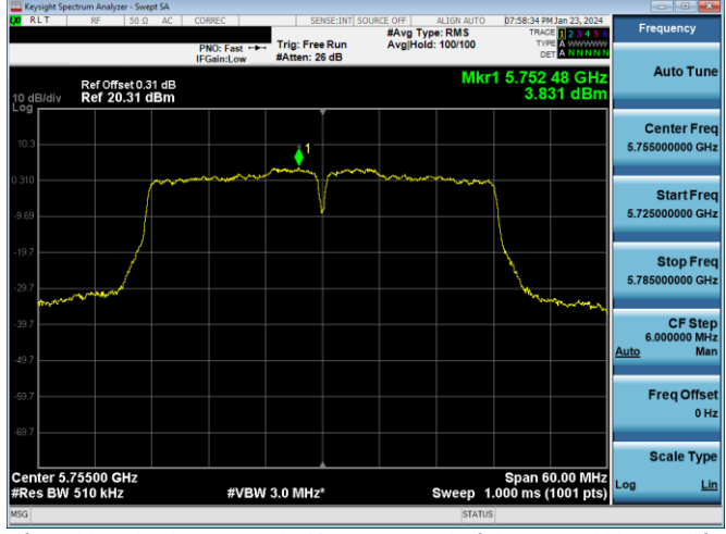
Plot 7-864. PSD CDD DIVERSITY Antenna WF2a (40MHz BW 802.11n – Ch. 151, MCS12)
