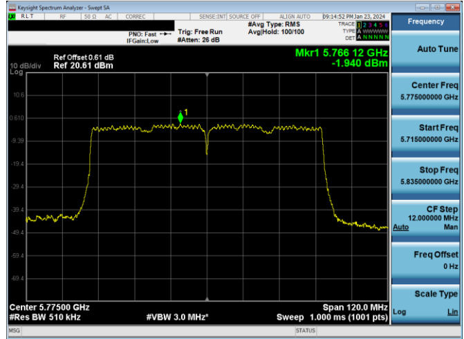
Plot 7-880. PSD CDD DIVERSITY Antenna WF2a (80MHz BW 802.11ac – Ch. 155, MCS9)
