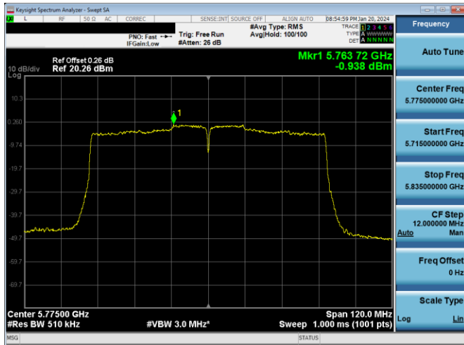
Plot 7-855. PSD CDD DIVERSITY Antenna WF7a (80MHz BW 802.11ac – Ch. 155, MCS2)
