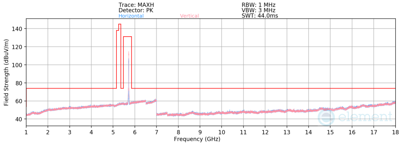
Plot 7-915. Radiated Spurious Emissions above 1GHz Antenna WF7a (802.11n – Ch. 144)
