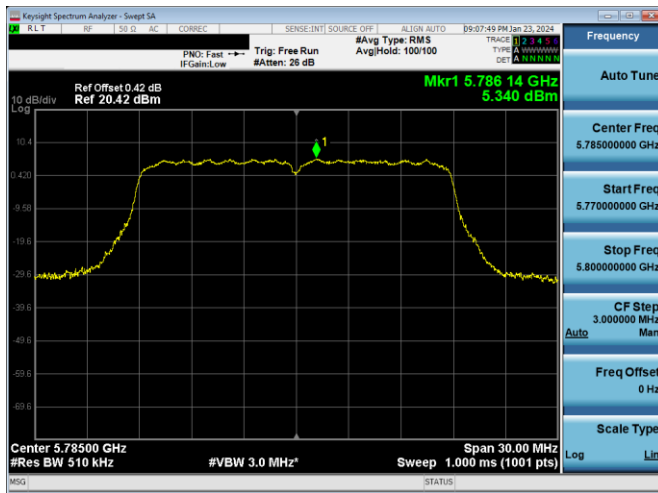
Plot 7-872. PSD CDD DIVERSITY Antenna WF2a (20MHz BW 802.11n - Ch. 157, MCS15)
