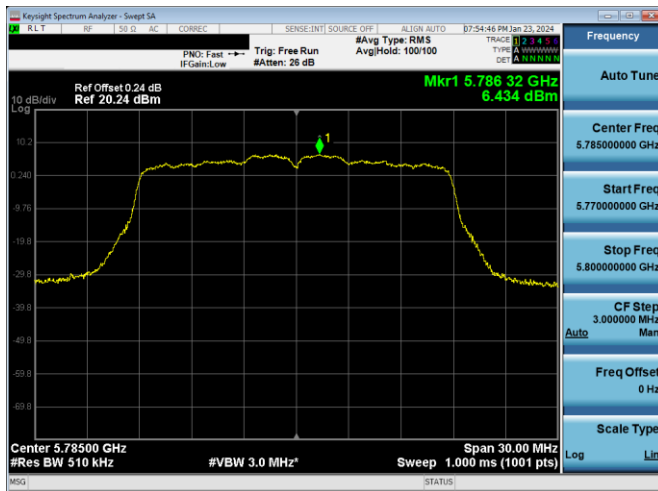
Plot 7-860. PSD CDD DIVERSITY Antenna WF2a (20MHz BW 802.11n – Ch. 157, MCS12)
