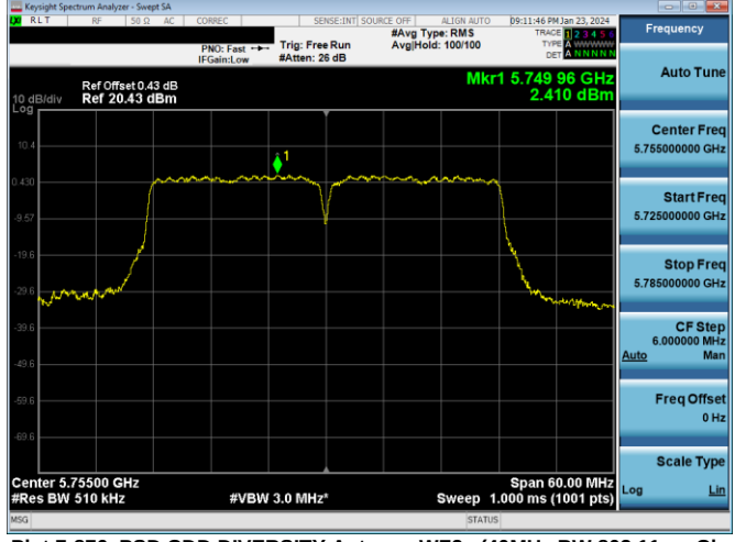
Plot 7-876. PSD CDD DIVERSITY Antenna WF2a (40MHz BW 802.11n - Ch. 151, MCS15)
