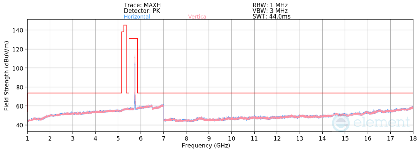
Plot 7-916. Radiated Spurious Emissions above 1GHz Antenna WF7a (802.11n – Ch. 149)
