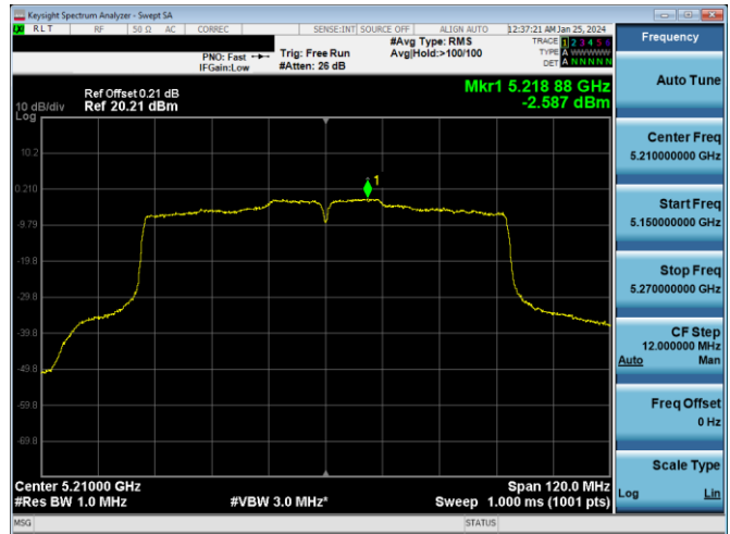
Plot 7-887. ISSED PSD CDD DIVERSITY Antenna WF2a (80MHz BW 11ac – Ch.42, MCS2)
