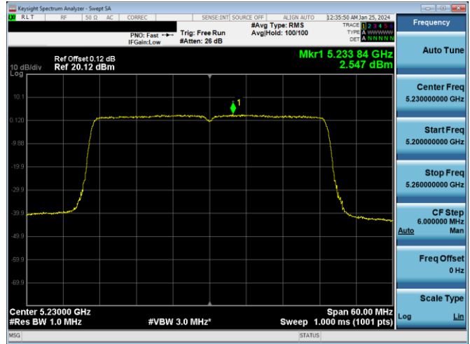
Plot 7-886. ISSED CDD DIVERSITY PSD Antenna WF2a (40MHz BW 11ax(SU) – Ch.46, MCS2)
