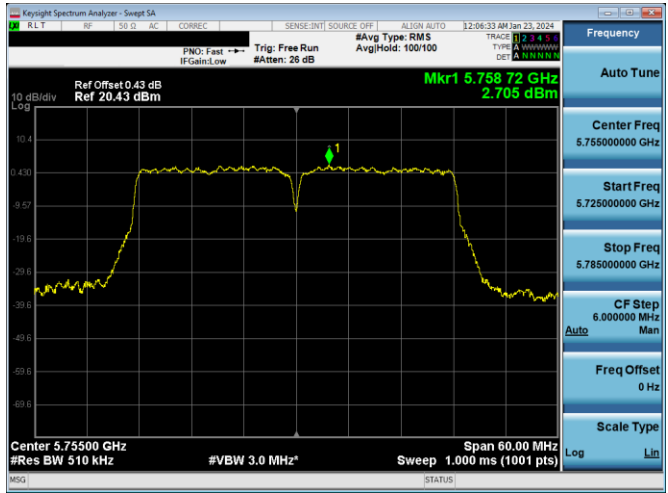
Plot 7-875. PSD CDD DIVERSITY Antenna WF7a (40MHz BW 802.11n - Ch. 151, MCS15)
