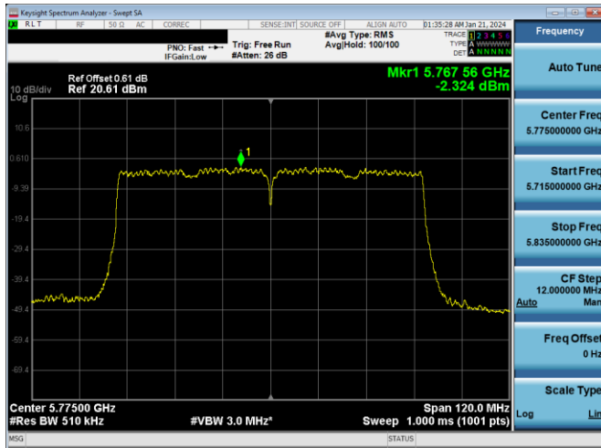
Plot 7-879. PSD CDD DIVERSITY Antenna WF7a (80MHz BW 802.11ac – Ch. 155, MCS9)
