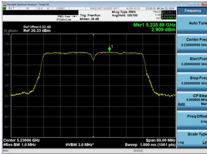
Plot 7-901. ISSED PSD SDM DIVERSITY Antenna WF2a (40MHz BW 11n - Ch.46, MCS15)
