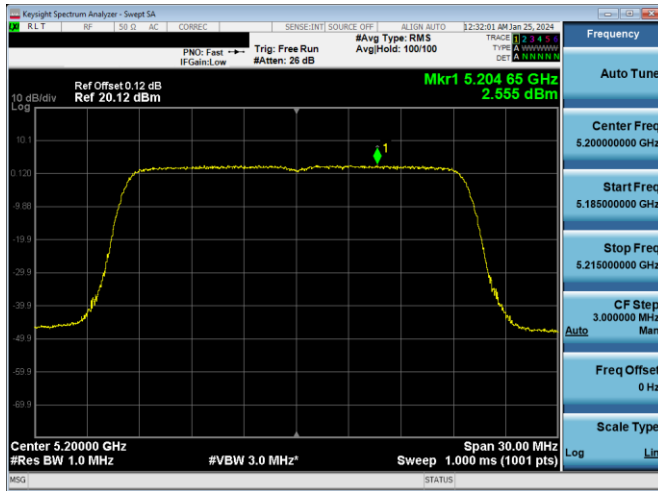
Plot 7-884. ISSED PSD SDM DIVERSITY Antenna WF2a (20MHz BW 11ax(SU) – Ch.40, MCS2)
