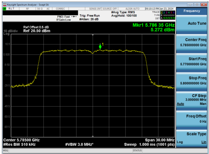
Plot 7-874. PSD CDD DIVERSITY Antenna WF2a (20MHz BW 802.11ax(SU) - Ch. 157, MCS11)
