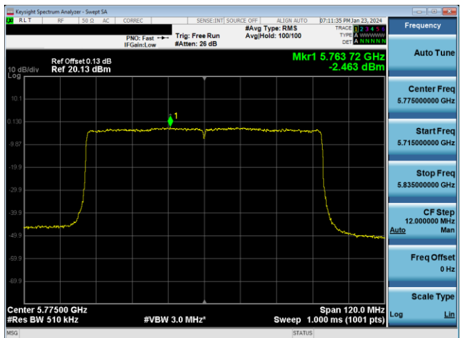
Plot 7-858. PSD CDD DIVERSITY Antenna WF2a (80MHz BW 802.11ax(SU) – Ch. 155, MCS2)
