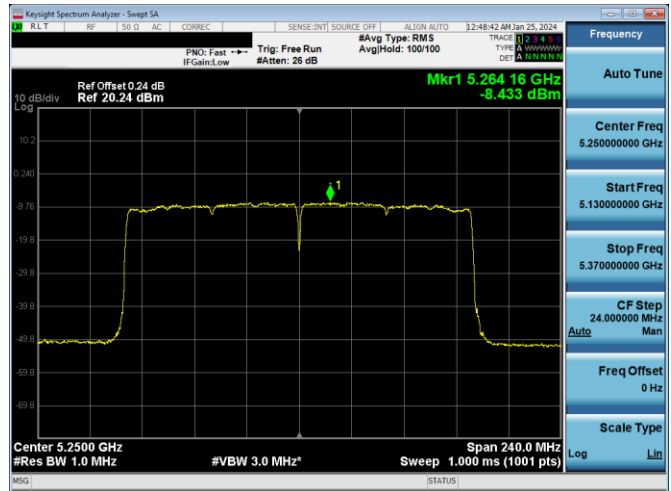
Plot 7-898. ISED CDD DIVERSITY SDM DIVERSITY Antenna WF2a (160MHz BW 11ax (SU) – Ch.50, MCS4)
