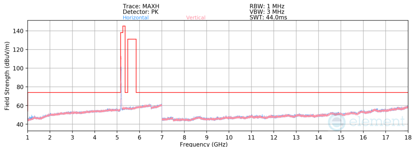
Plot 7-907. Radiated Spurious Emissions above 1GHz Antenna WF7a (802.11n – Ch. 36)
