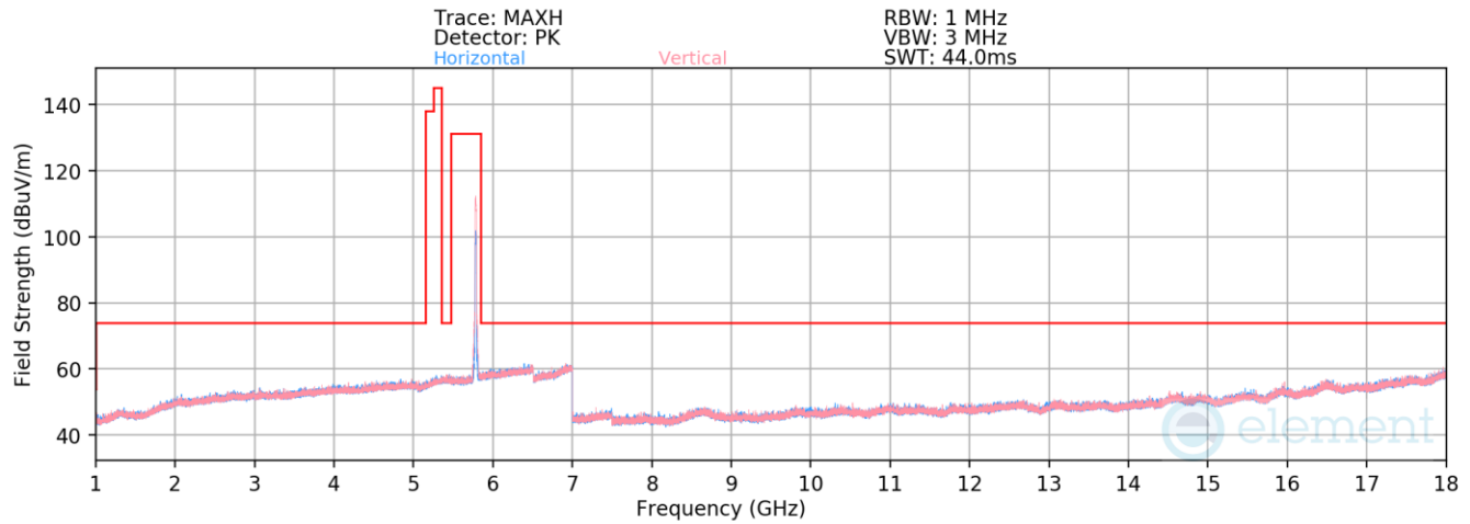
Plot 7-965. Radiated Spurious Emissions above 1GHz Antenna WF7b (802.11n – Ch. 157)
