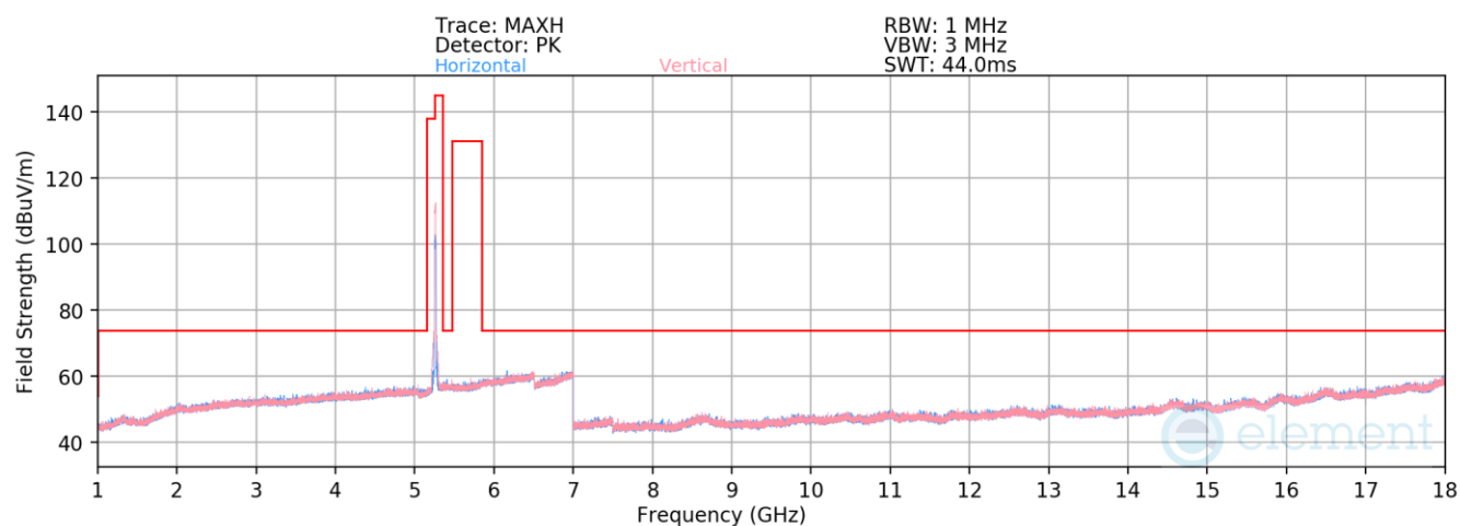
Plot 7-958. Radiated Spurious Emissions above 1GHz Antenna WF7b (802.11n – Ch. 52)
