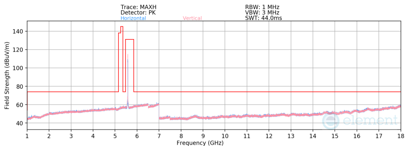
Plot 7-938. Radiated Spurious Emissions above 1GHz Antenna WF2a (802.11n – Ch. 116)
