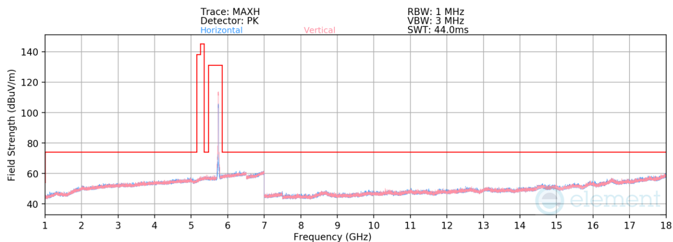
Plot 7-928. Radiated Spurious Emissions above 1GHz Antenna WF7a (802.11ax(SU) – Ch. 149)
