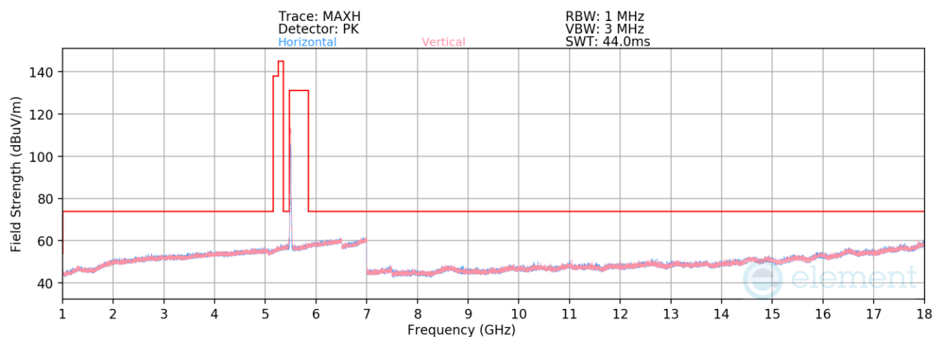
Plot 7-961. Radiated Spurious Emissions above 1GHz Antenna WF7b (802.11n – Ch. 100)
