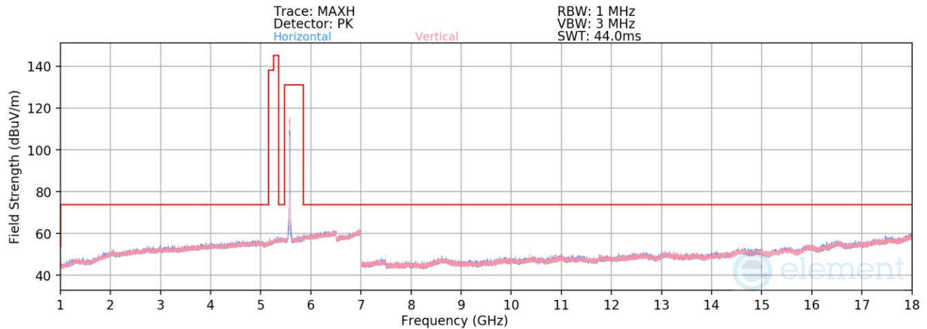
Plot 7-950. Radiated Spurious Emissions above 1GHz Antenna WF2a (802.11ax(SU) – Ch. 116)
