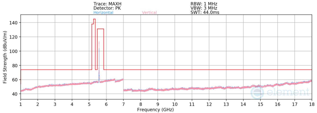
Plot 7-962. Radiated Spurious Emissions above 1GHz Antenna WF7b (802.11n – Ch. 116)
