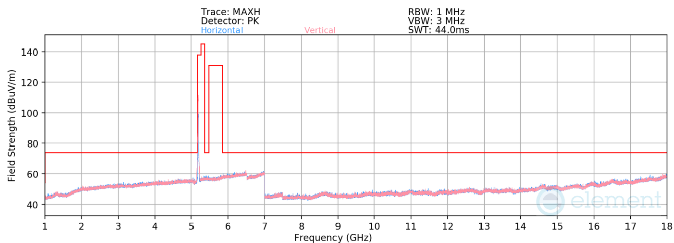
Plot 7-967. Radiated Spurious Emissions above 1GHz Antenna WF7b (802.11ax(SU) – Ch. 36)
