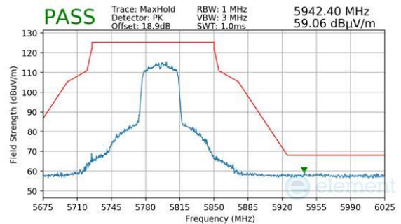
Plot 7-1120. ANTENNA WF7A (PK, CH.159, 802.11N, MCS2)
