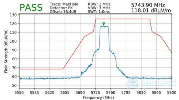
Plot 7-1098. ANTENNA WF7A (PK, CH.149, 802.11AX(SU), MCS4)
