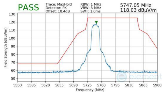
Plot 7-1068. ANTENNA WF7A (PK, CH.149, 802.11N, MCS2)
