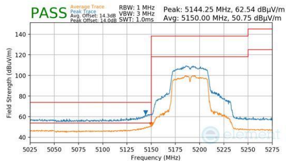
Plot 7-1245. ANTENNA WF2A (PK & AVG, CH.38, 802.11N, MCS4)
