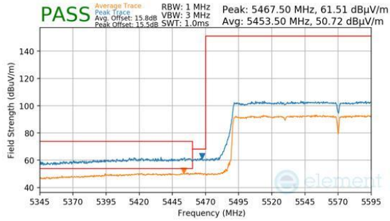
Plot 7-1181. ANTENNA WF7A (PK & AVG, CH.114, 802.11AX(SU), MCS2)
