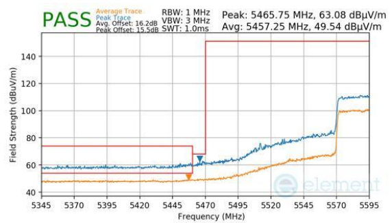
Plot 7-1155. ANTENNA WF7A (PK & AVG, CH.122, 802.11AX(SU), MCS11)
