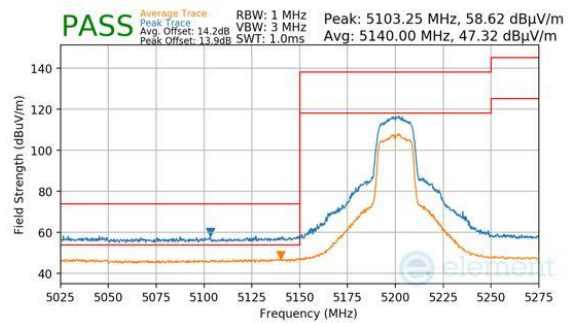
Plot 7-1190. ANTENNA WF2A (PK & AVG, CH.40, 802.11N, MCS2)
