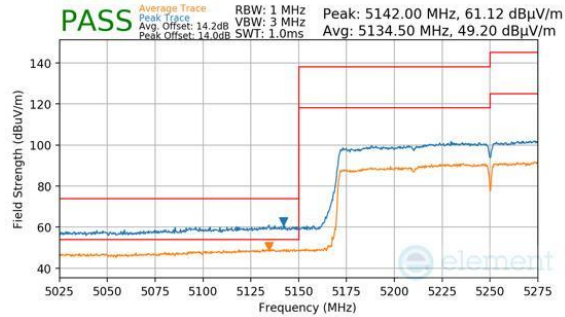
Plot 7-1175. ANTENNA WF7A (PK & AVG, CH.50, 802.11AX(SU), MCS2)
