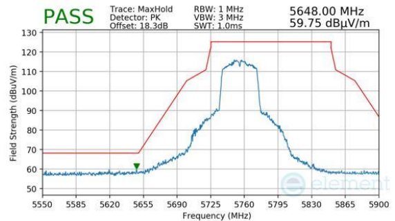
Plot 7-1119. ANTENNA WF7A (PK, CH.151, 802.11N, MCS4)
