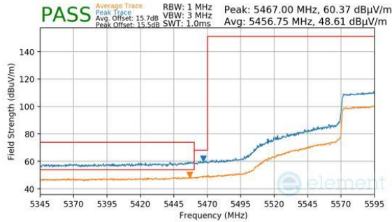
Plot 7-1435. ANTENNA WF7B (PK & AVG, CH.122, 802.11AX(SU), MCS2)
