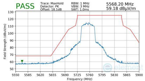
Plot 7-1260. ANTENNA WF2A (PK, CH.151, 802.11N, MCS4)
