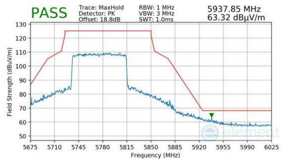
Plot 7-1303. ANTENNA WF2A (PK, CH.155, 802.11AX(SU), MCS11)
