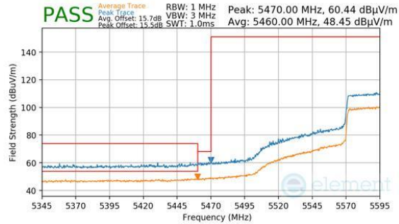
Plot 7-1292. ANTENNA WF2A (PK & AVG, CH.122, 802.11AX(SU), MCS2)
