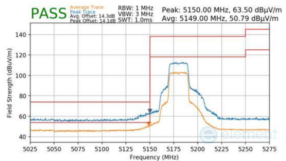
Plot 7-1357. ANTENNA WF7B (PK & AVG, CH.36, 802.11AX(SU), MCS2)
