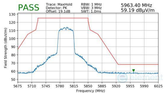
Plot 7-1261. ANTENNA WF2A (PK, CH.159, 802.11N, MCS2)
