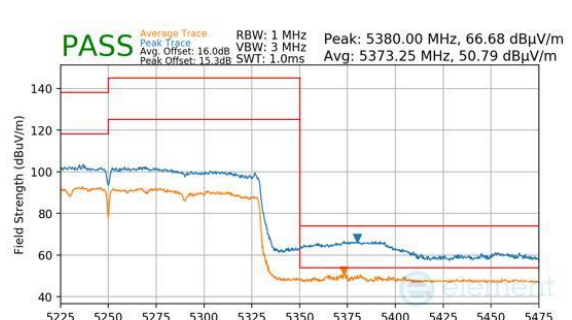
Plot 7-1321. ANTENNA WF2A (PK & AVG, CH.50, 802.11AX(SU), MCS11)
