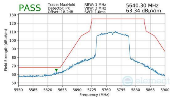
Plot 7-1422. ANTENNA WF7B (PK, CH.155, 802.11AC, MCS4)
