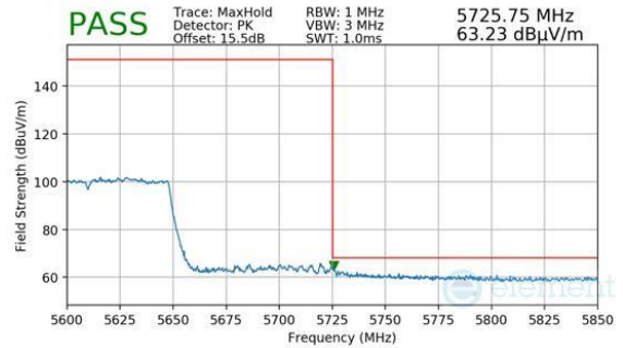
Plot 7-1315. ANTENNA WF2A (PK, CH.114, 802.11AC, MCS9)
