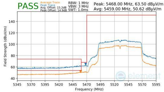
Plot 7-1268. ANTENNA WF2A (PK & AVG, CH.106, 802.11AC, MCS2)
