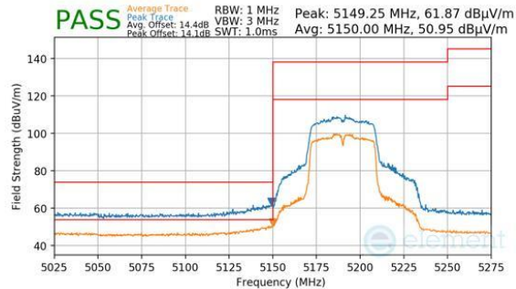
Plot 7-1388. ANTENNA WF7B (PK & AVG, CH.38, 802.11N, MCS4)
