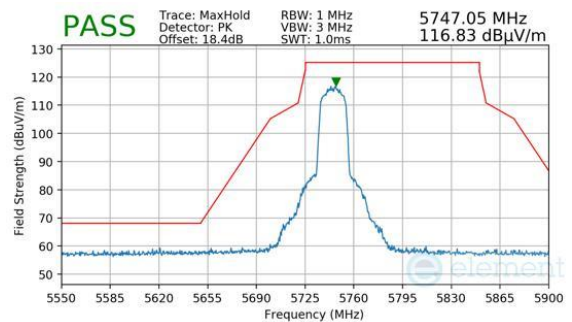
Plot 7-1351. ANTENNA WF7B (PK, CH.149, 802.11N, MCS2)
