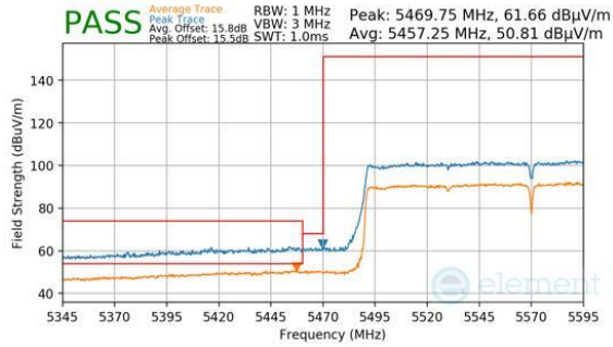
Plot 7-1322. ANTENNA WF2A (PK & AVG, CH.114, 802.11AX(SU), MCS2)
