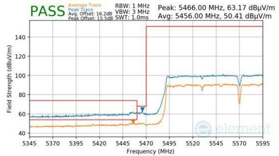
Plot 7-1314. ANTENNA WF2A (PK & AVG, CH.114, 802.11AC, MCS9)
