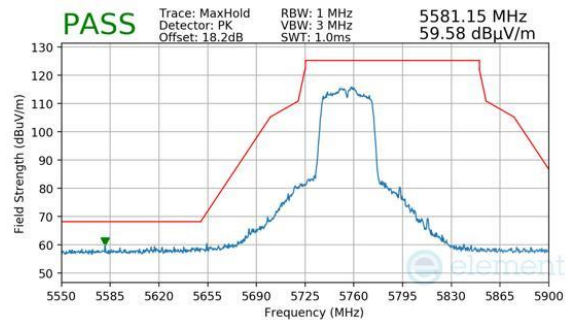
Plot 7-1538. CDD PRIMARY (PK, CH.151, 802.11N, MCS10)
