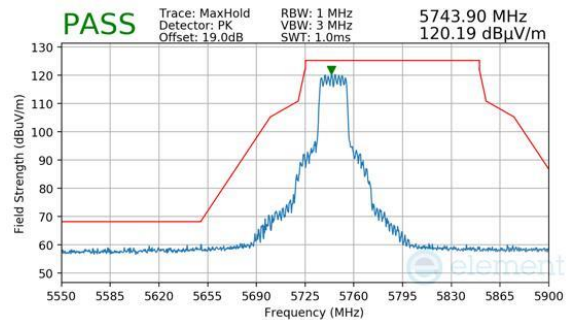
Plot 7-1511. CDD PRIMARY (PK, CH.149, 802.11AX(SU), MCS11)
