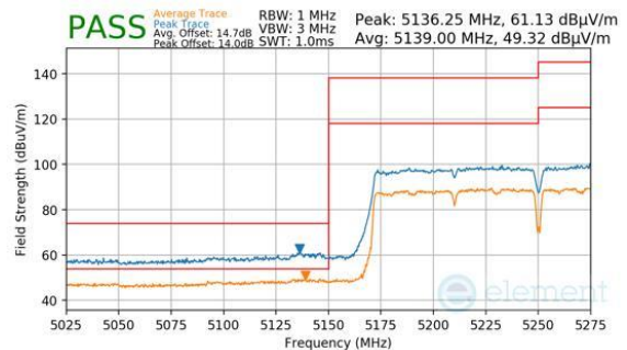
Plot 7-1451. ANTENNA WF7B (PK & AVG, CH.50, 802.11AC, MCS9)
