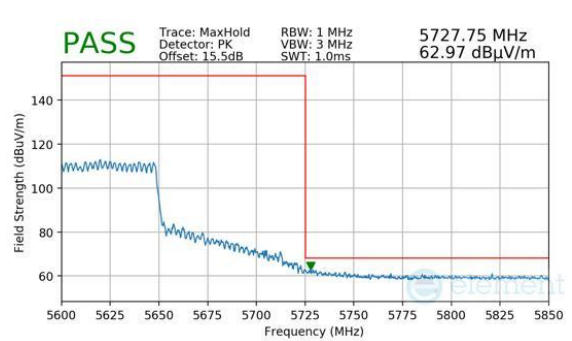
Plot 7-1608. CDD PRIMARY (PK, CH.122, 802.11AX(SU), MCS11)
