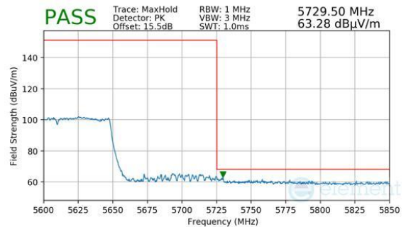
Plot 7-1626. CDD PRIMARY (PK, CH.114, 802.11AC, MCS9)
