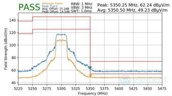
Plot 7-1475. CDD PRIMARY (PK & AVG, CH.60, 802.11N, MCS15)
