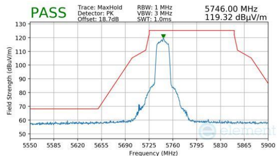
Plot 7-1488. CDD PRIMARY (PK, CH.149, 802.11N, MCS10)
