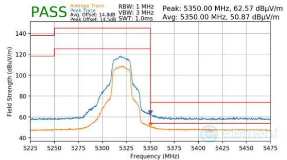
Plot 7-1476. CDD PRIMARY (PK & AVG, CH.64, 802.11N, MCS10)
