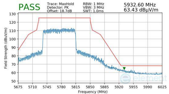
Plot 7-1614. CDD PRIMARY (PK, CH.155, 802.11AX(SU), MCS11)
