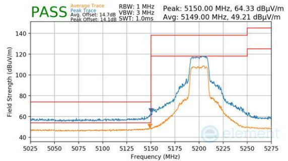
Plot 7-1474. CDD PRIMARY (PK & AVG, CH.40, 802.11N, MCS15)
