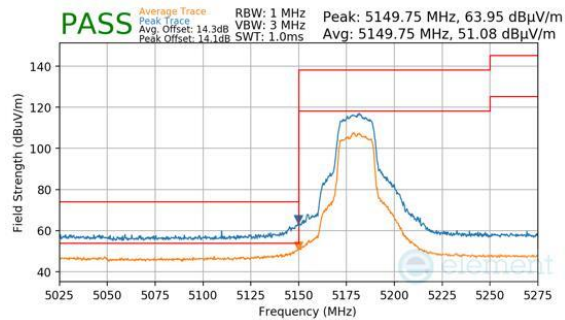
Plot 7-1471. CDD PRIMARY (PK & AVG, CH.36, 802.11N, MCS10)
