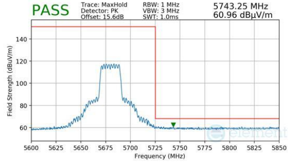
Plot 7-1504. CDD PRIMARY (PK, CH.136, 802.11AX(SU), MCS4)
