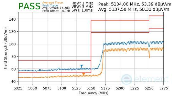
Plot 7-1627. CDD PRIMARY (PK & AVG, CH.50, 802.11AX(SU), MCS2)
