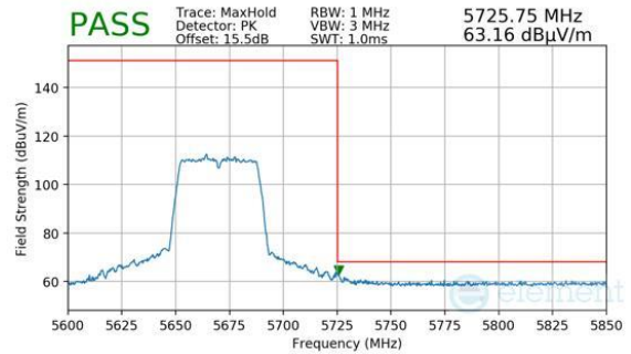
Plot 7-1537. CDD PRIMARY (PK, CH.134, 802.11N, MCS15)
