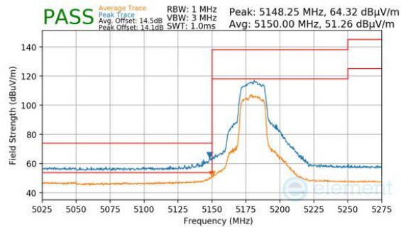
Plot 7-1472. CDD PRIMARY (PK & AVG, CH.36, 802.11N, MCS12)
