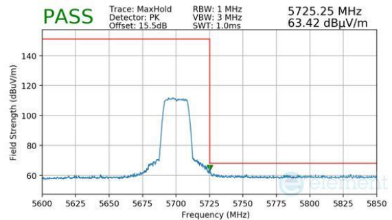
Plot 7-1487. CDD PRIMARY (PK, CH.140, 802.11N, MCS15)
