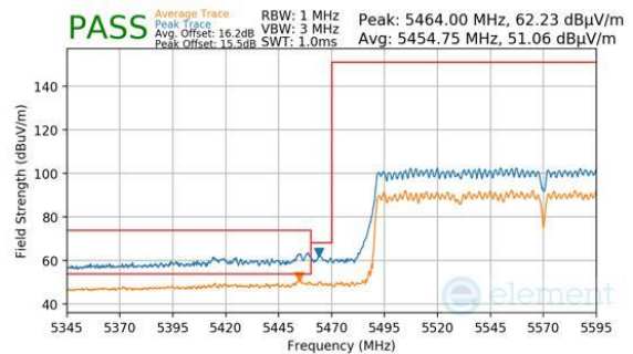
Plot 7-1637. CDD PRIMARY (PK & AVG, CH.114, 802.11AX(SU), MCS11)
