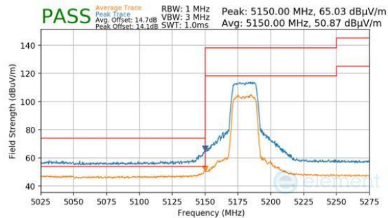
Plot 7-1473. CDD PRIMARY (PK & AVG, CH.36, 802.11N, MCS15)
