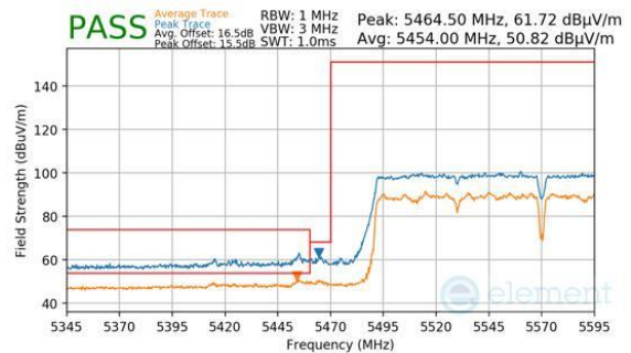
Plot 7-1625. CDD PRIMARY (PK & AVG, CH.114, 802.11AC, MCS9)
