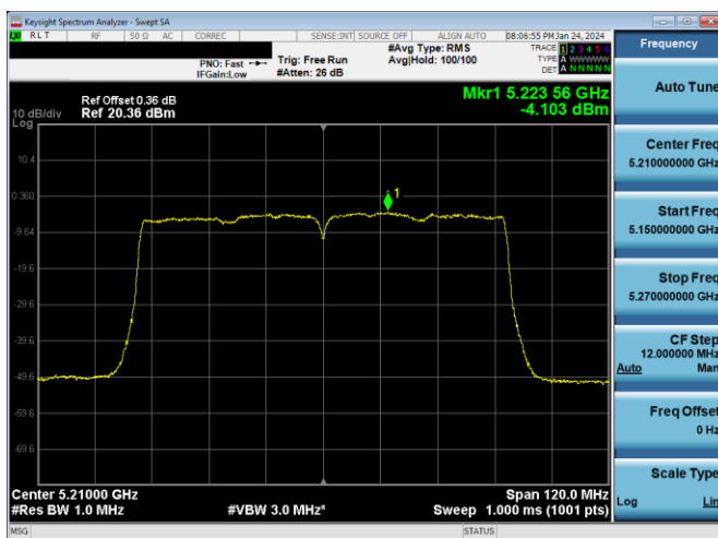
Plot 7-357. ISED PSD Antenna WF7a (80MHz BW 11ac – Ch.42, MCS9)
