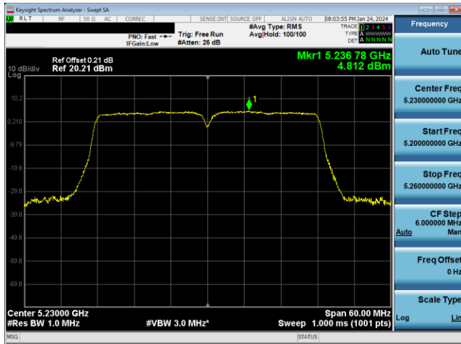
Plot 7-355. ISED PSD Antenna WF7a (40MHz BW 11n – Ch.46, MCS7)
