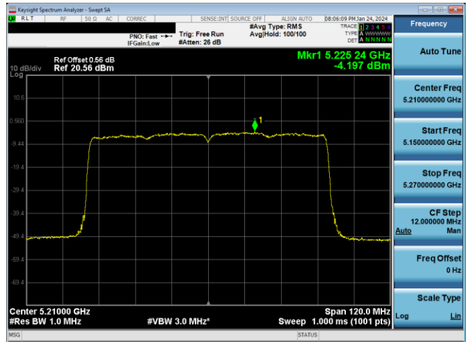
Plot 7-358. ISED PSD Antenna WF7a (80MHz BW 11ax (SU) – Ch.42, MCS11)
