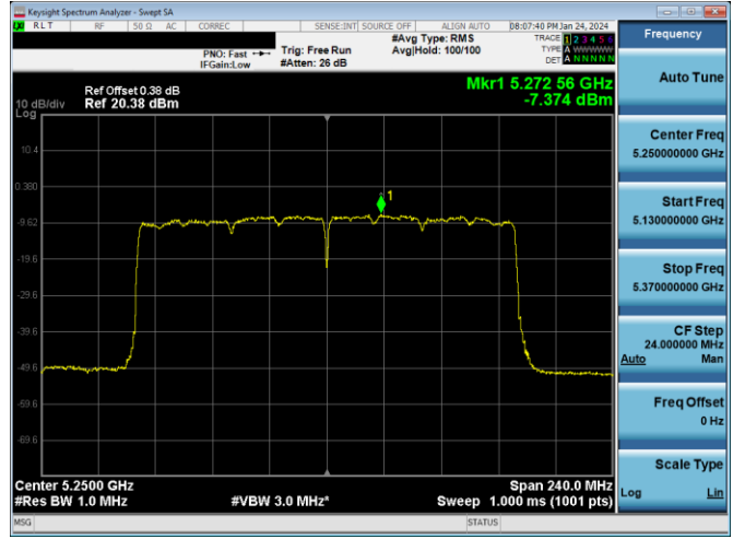
Plot 7-360. ISED PSD Antenna WF7a (160MHz BW 11ax (SU) – Ch.50, MCS11)
