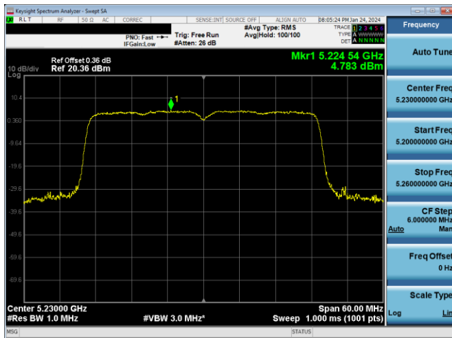
Plot 7-356. ISED PSD Antenna WF7a (40MHz BW 11ax(SU) – Ch.46, MCS11)
