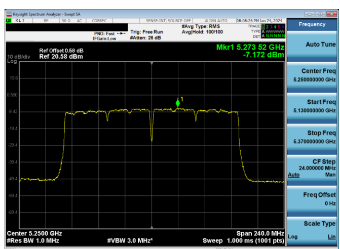
Plot 7-359. ISED PSD Antenna WF7a (160MHz BW 11ac – Ch.50, MCS9)
