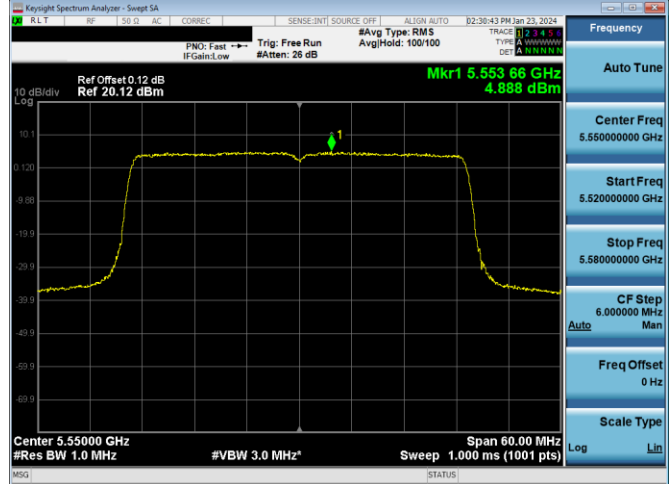
Plot 7-486. PSD Antenna WF7b (40MHz BW 802.11ax(SU) – Ch. 110, MCS2)
