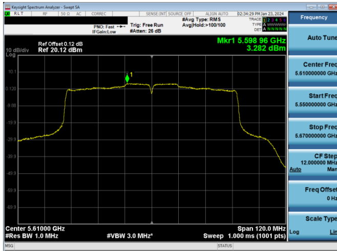
Plot 7-487. PSD Antenna WF7b (80MHz BW 802.11ac – Ch. 122, MCS2)
