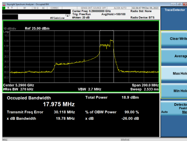
Plot 7-27. 26dB BW & 99% OBW Antenna WF7a (80MHz BW 11ax Index 52 – RU52 – Ch.58)
