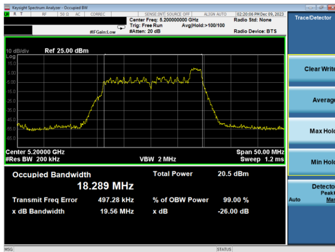
Plot 7-3. 26dB BW & 99% OBW Antenna WF7a (20MHz BW 11ax Index 8– RU26 – Ch.40)
