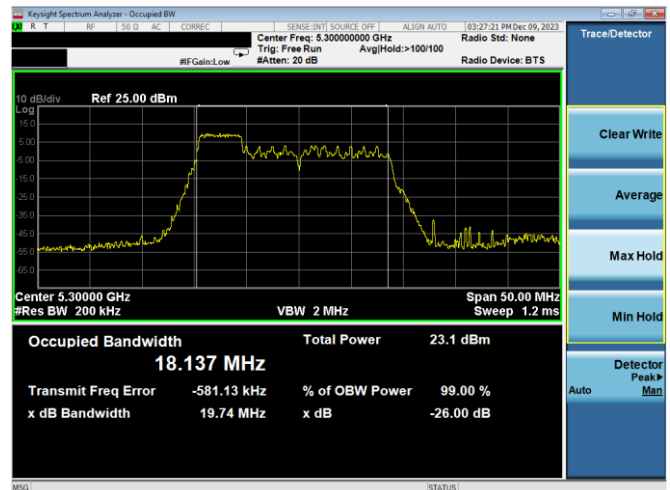
Plot 7-61. 26dB BW & 99% OBW Antenna WF2a (20MHz BW 11ax Index 37 – RU52 – Ch.60)
