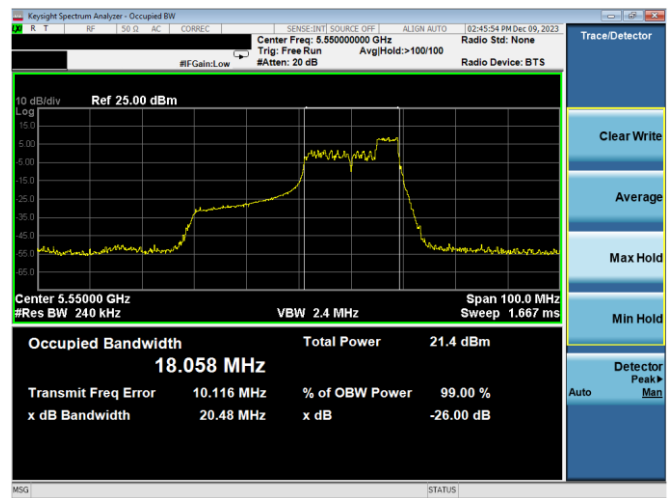
Plot 7-35. 26dB BW & 99% OBW Antenna WF7a (40MHz BW 11ax Index 44 - RU52 - Ch.110)
