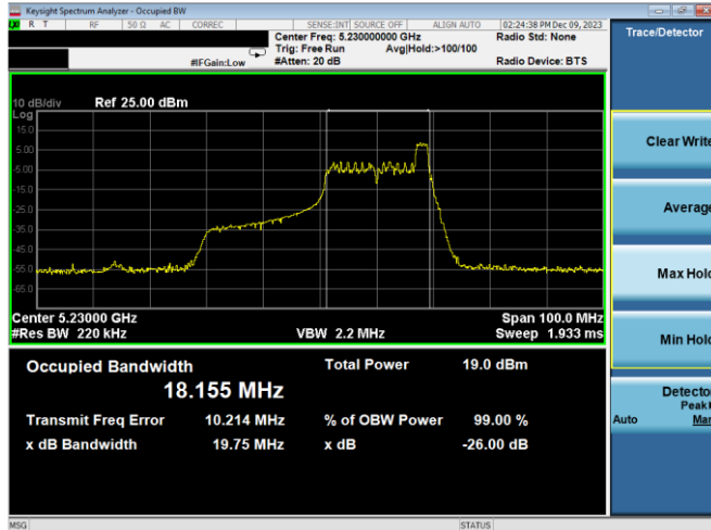
Plot 7-7. 26dB BW & 99% OBW Antenna WF7a (40MHz BW 11ax Index 17 – RU26 – Ch.46)
