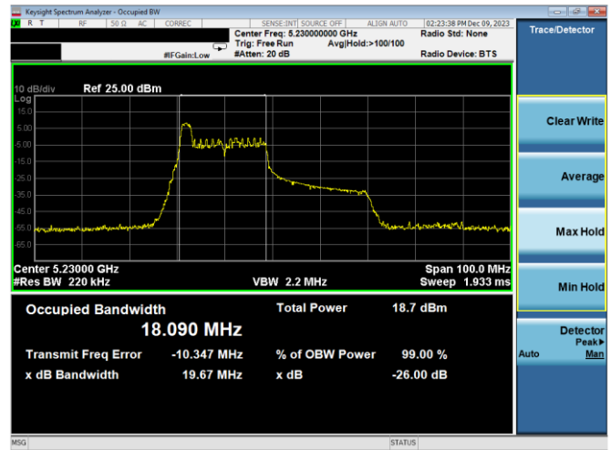
Plot 7-5. 26dB BW & 99% OBW Antenna WF7a (40MHz BW 11ax Index 0 – RU26 – Ch.46)
