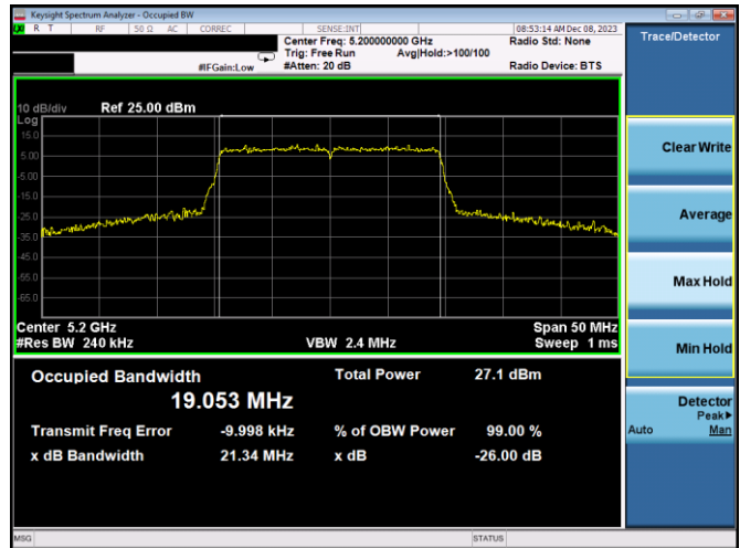
Plot 7-4. 26dB BW & 99% OBW Antenna WF7a (20MHz BW 11ax– RU242 – Ch.40)
