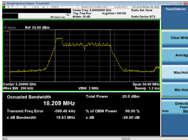
Plot 7-45. 26dB BW & 99% OBW Antenna WF2a (20MHz BW 11ax Index 0 – RU26 – Ch.40)
