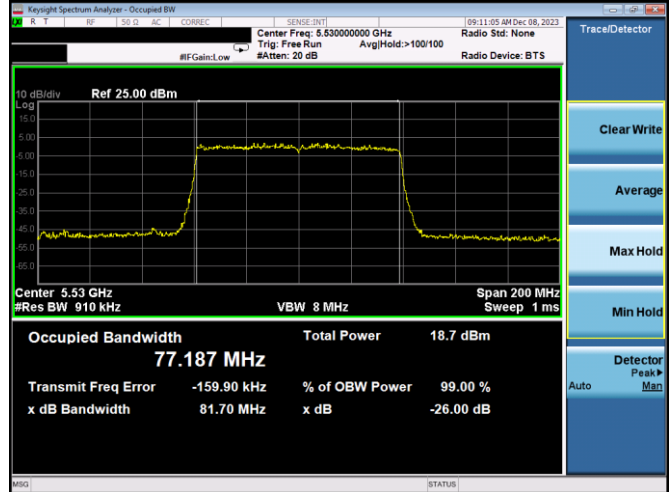
Plot 7-40. 26dB BW & 99% OBW Antenna WF7a (80MHz BW 11ax - RU996 - Ch.106)
