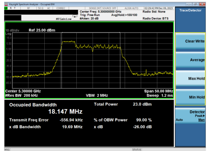
Plot 7-17. 26dB BW & 99% OBW Antenna WF7a (20MHz BW 11ax Index 37 - RU52 - Ch.60)
