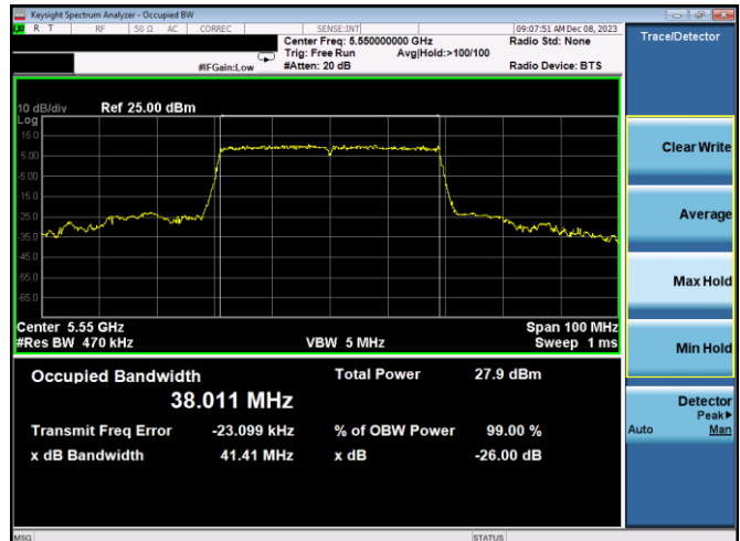
Plot 7-36. 26dB BW & 99% OBW Antenna WF7a (40MHz BW 11ax - RU484 - Ch.110)
