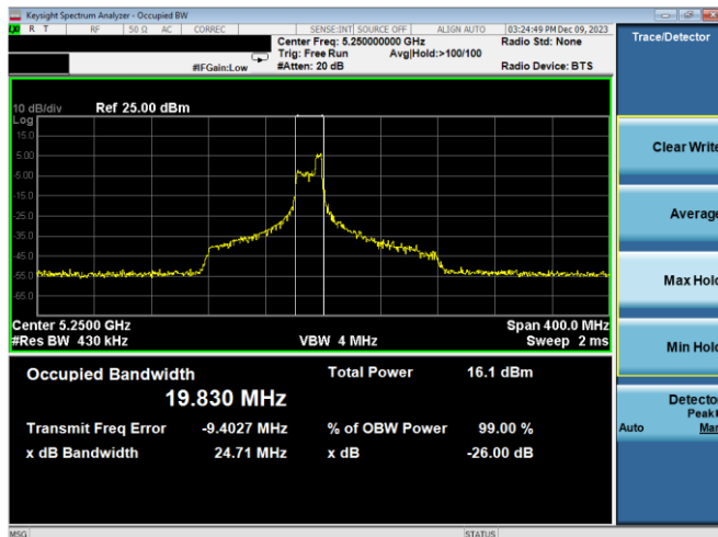
Plot 7-58. 26dB BW & 99% OBW Antenna WF2a (160MHz BW 11ax Index 52 – RU52 – Ch.50 (L))
