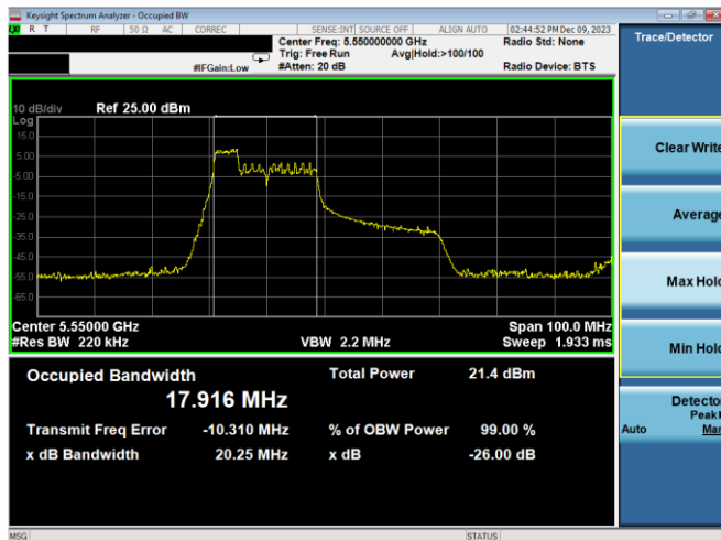
Plot 7-33. 26dB BW & 99% OBW Antenna WF7a (40MHz BW 11ax Index 37 - RU52 - Ch.110)
