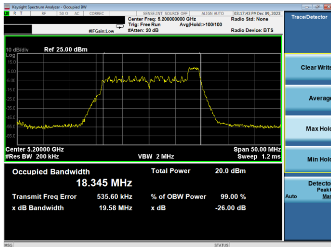
Plot 7-47. 26dB BW & 99% OBW Antenna WF2a (20MHz BW 11ax Index 8 – RU26 – Ch.40)
