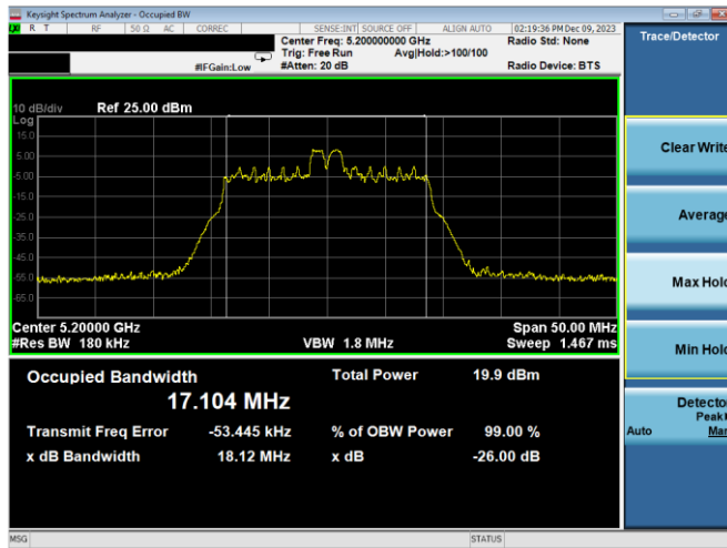
Plot 7-2. 26dB BW & 99% OBW Antenna WF7a (20MHz BW 11ax Index 4 – RU26 – Ch.40)
