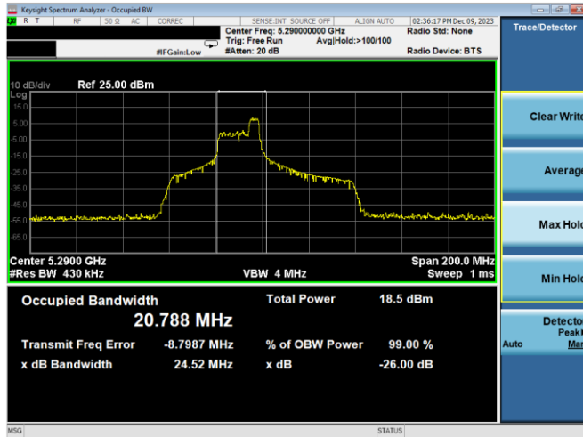
Plot 7-26. 26dB BW & 99% OBW Antenna WF7a (80MHz BW 11ax Index 44 – RU52 – Ch.58)
