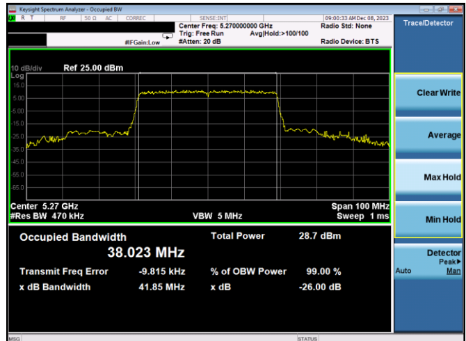
Plot 7-24. 26dB BW & 99% OBW Antenna WF7a (40MHz BW 11ax – RU484 – Ch.54)
