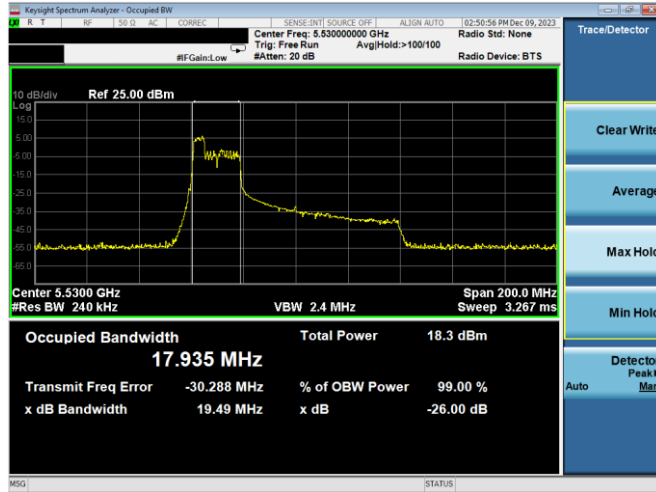
Plot 7-37. 26dB BW & 99% OBW Antenna WF7a (80MHz BW 11ax Index 37 - RU52 - Ch.106)
