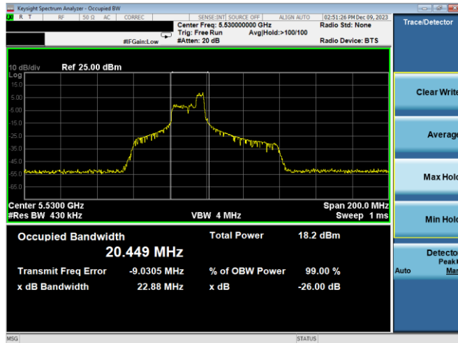
Plot 7-38. 26dB BW & 99% OBW Antenna WF7a (80MHz BW 11ax Index 44 - RU52 - Ch.106)
