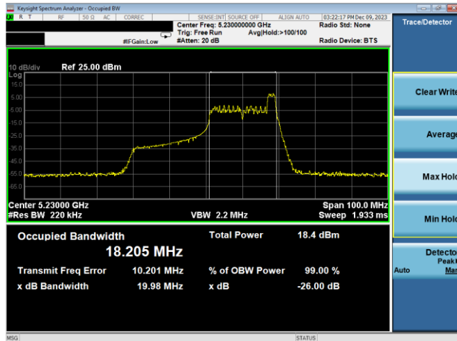
Plot 7-51. 26dB BW & 99% OBW Antenna WF2a (40MHz BW 11ax Index 17 – RU26 – Ch.46)
