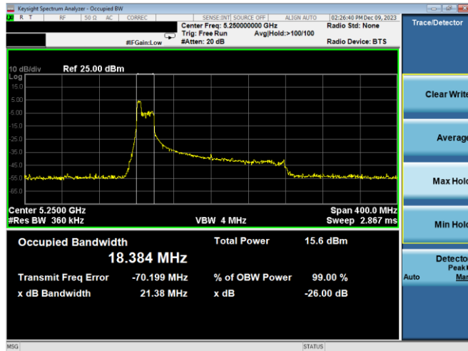
Plot 7-13. 26dB BW & 99% OBW Antenna WF7a (160MHz BW 11ax Index 37 - RU52 - Ch.50 (L))
