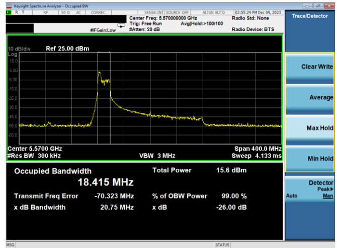
Plot 7-41. 26dB BW & 99% OBW Antenna WF7a (160MHz BW 11ax Index 37 - RU52 - Ch.114 (L))
