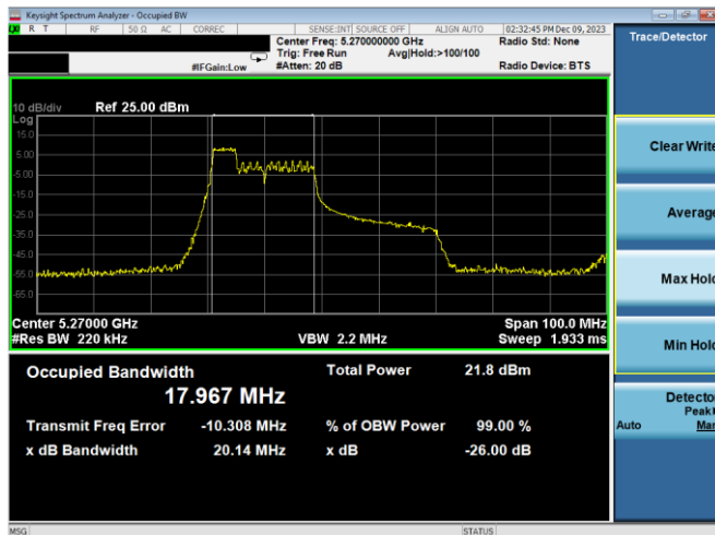
Plot 7-21. 26dB BW & 99% OBW Antenna WF7a (40MHz BW 11ax Index 37 – RU52 – Ch.54)
