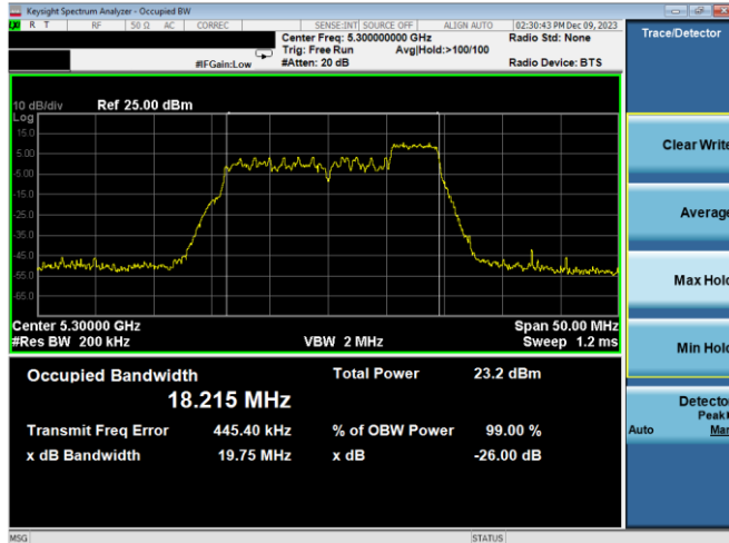
Plot 7-19. 26dB BW & 99% OBW Antenna WF7a (20MHz BW 11ax Index 40 – RU52 – Ch.60)
