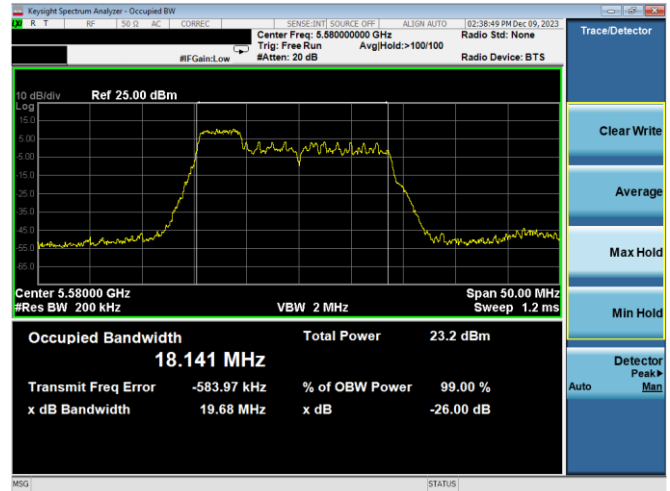
Plot 7-29. 26dB BW & 99% OBW Antenna WF7a (20MHz BW 11ax Index 37 – RU52 – Ch.116)
