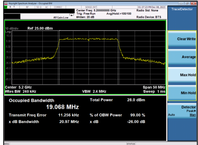
Plot 7-48. 26dB BW & 99% OBW Antenna WF2a (20MHz BW 11ax – RU242 – Ch.40)
