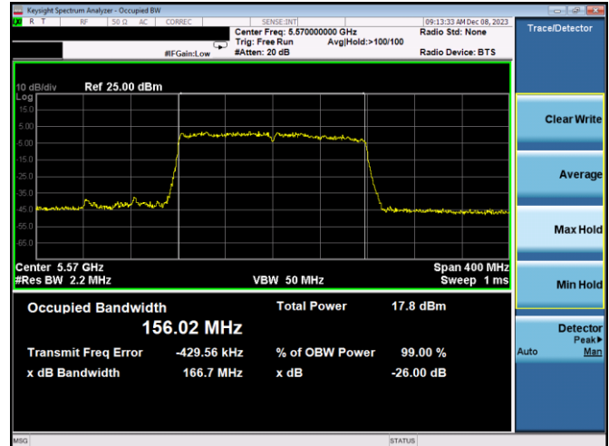
Plot 7-44. 26dB BW & 99% OBW Antenna WF7a (160MHz BW 11ax – RU996x2 – Ch.114)
