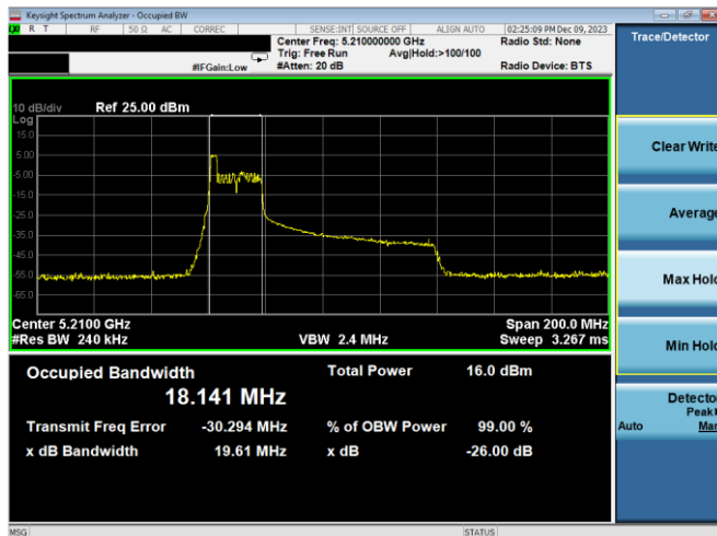
Plot 7-9. 26dB BW & 99% OBW Antenna WF7a (80MHz BW 11ax Index 0 – RU26 – Ch.42)
