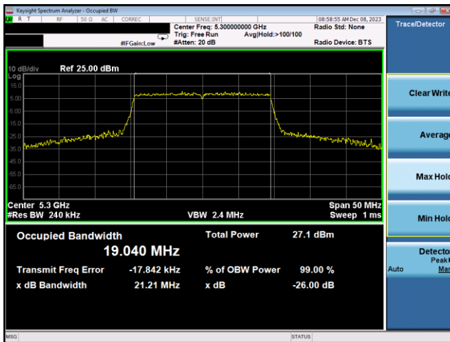
Plot 7-20. 26dB BW & 99% OBW Antenna WF7a (20MHz BW 11ax-- RU242 – Ch.60)
