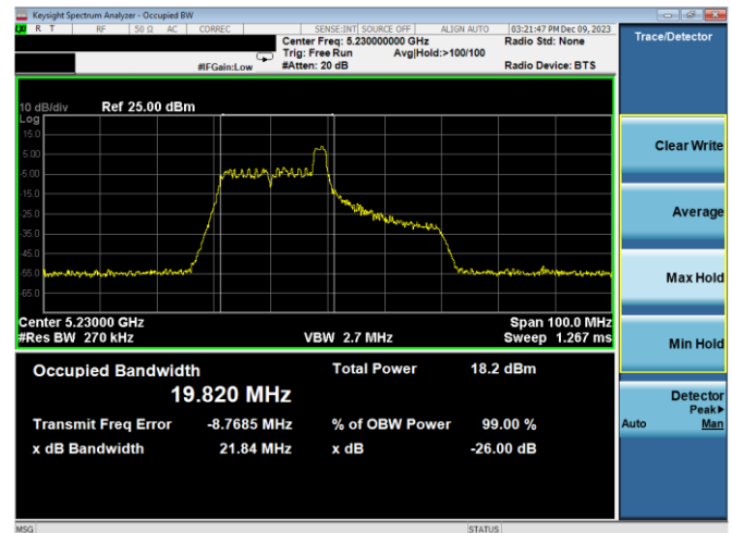
Plot 7-50. 26dB BW & 99% OBW Antenna WF2a (40MHz BW 11ax Index 8 – RU26 – Ch.46)
