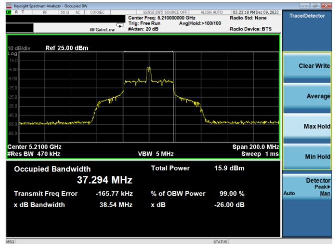
Plot 7-54. 26dB BW & 99% OBW Antenna WF2a (80MHz BW 11ax Index 18 – RU26 – Ch.42)
