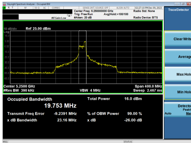
Plot 7-14. 26dB BW & 99% OBW Antenna WF7a (160MHz BW 11ax Index 52 - RU52 - Ch.50 (L))
