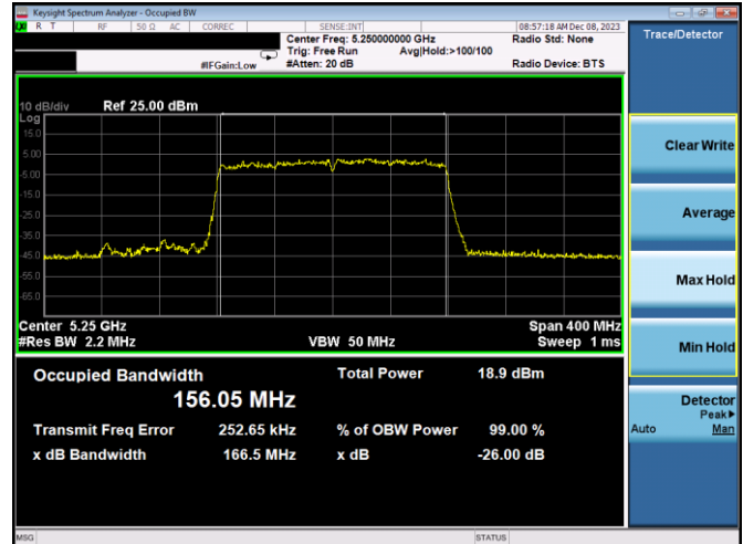
Plot 7-16. 26dB BW & 99% OBW Antenna WF7a (160MHz BW 11ax - RU96x2 - Ch.50)
