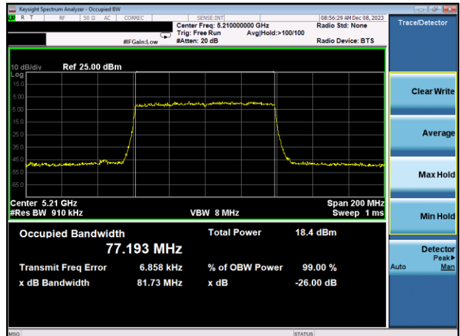
Plot 7-12. 26dB BW & 99% OBW Antenna WF7a (80MHz BW 11ax – RU996 – Ch.42)
