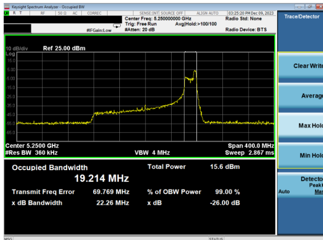
Plot 7-59. 26dB BW & 99% OBW Antenna WF2a (160MHz BW 11ax Index 52 – RU52 – Ch.50 (U))
