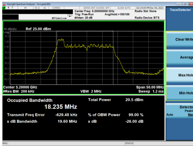
Plot 7-1. 26dB BW & 99% OBW Antenna WF7a (20MHz BW 11ax Index 0 – RU26 – Ch.40)
