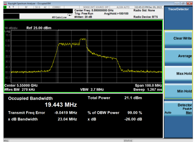
Plot 7-34. 26dB BW & 99% OBW Antenna WF7a (40MHz BW 11ax Index 40 - RU52 - Ch.110)
