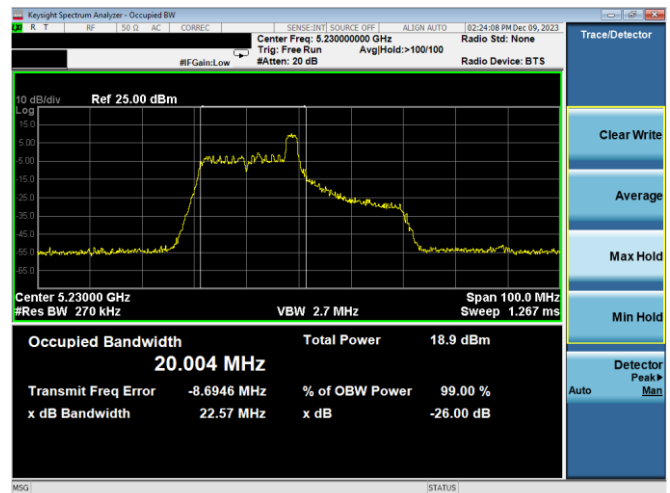
Plot 7-6. 26dB BW & 99% OBW Antenna WF7a (40MHz BW 11ax Index 8 – RU26 – Ch.46)
