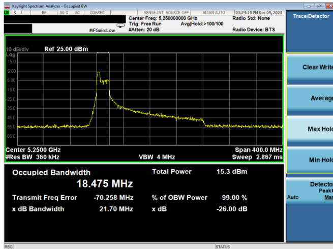
Plot 7-57. 26dB BW & 99% OBW Antenna WF2a (160MHz BW 11ax Index 37 – RU52 – Ch.50 (L))
