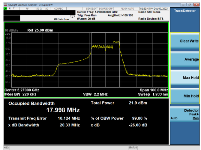
Plot 7-23. 26dB BW & 99% OBW Antenna WF7a (40MHz BW 11ax Index 44 – RU52 – Ch.54)
