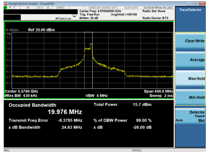
Plot 7-42. 26dB BW & 99% OBW Antenna WF7a (160MHz BW 11ax Index 52 - RU52 - Ch.114 (L))
