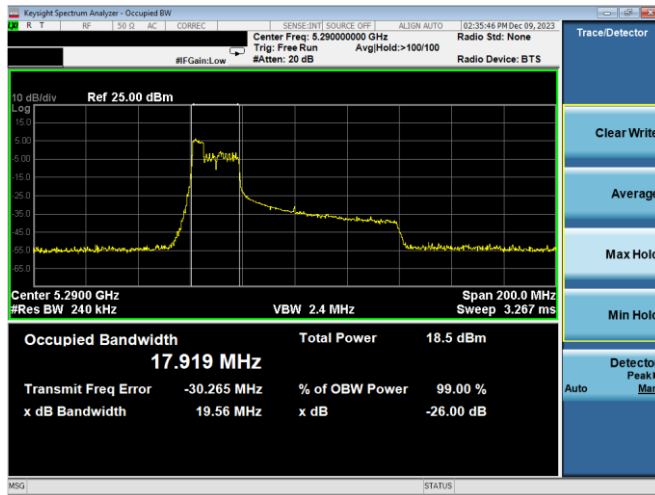
Plot 7-25. 26dB BW & 99% OBW Antenna WF7a (80MHz BW 11ax Index 37 – RU52 – Ch.58)
