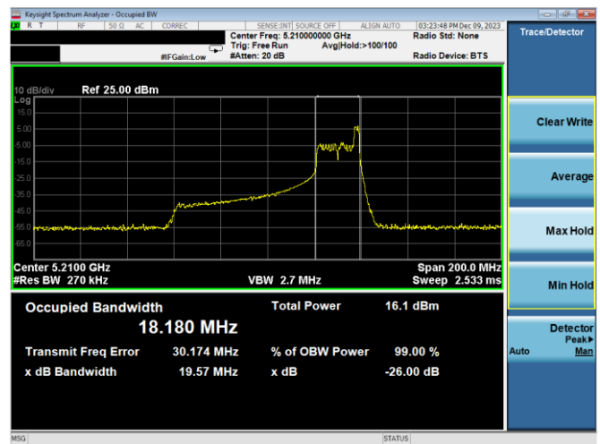
Plot 7-55. 26dB BW & 99% OBW Antenna WF2a (80MHz BW 11ax Index 36 – RU26 – Ch.42)
