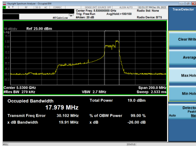
Plot 7-39. 26dB BW & 99% OBW Antenna WF7a (80MHz BW 11ax Index 52 - RU52 - Ch.106)
