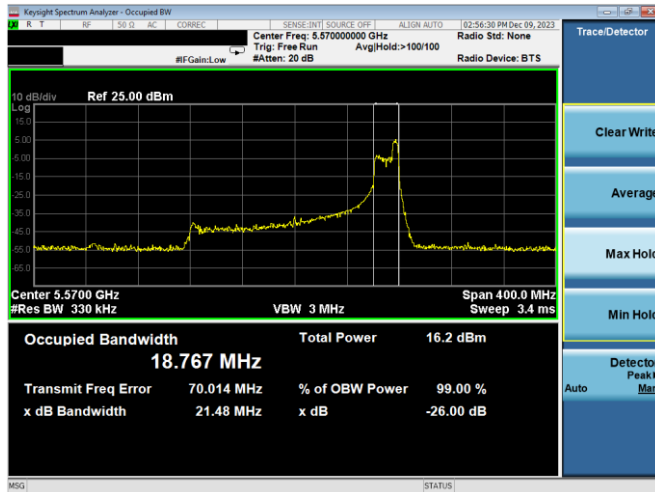
Plot 7-43. 26dB BW & 99% OBW Antenna WF7a (160MHz BW 11ax Index 52 – RU52 – Ch.114 (U))
