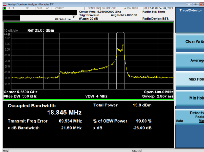
Plot 7-15. 26dB BW & 99% OBW Antenna WF7a (160MHz BW 11ax Index 52 - RU52 - Ch.50 (U))
