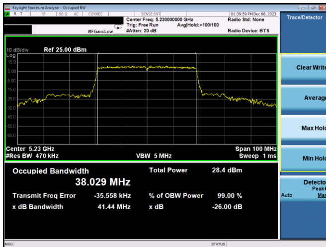
Plot 7-52. 26dB BW & 99% OBW Antenna WF2a (40MHz BW 11ax – RU484 – Ch.46)
