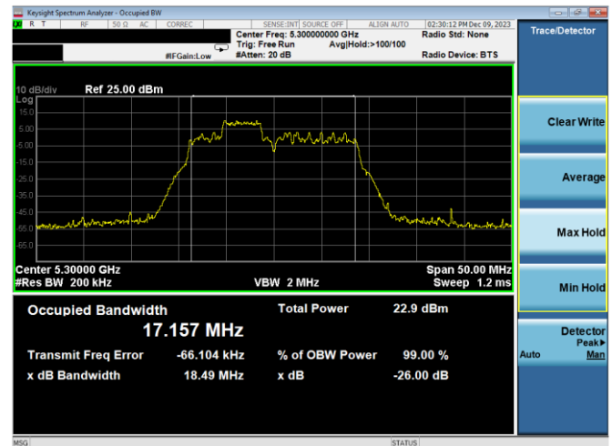
Plot 7-18. 26dB BW & 99% OBW Antenna WF7a (20MHz BW 11ax Index 38 - RU52 - Ch.60)
