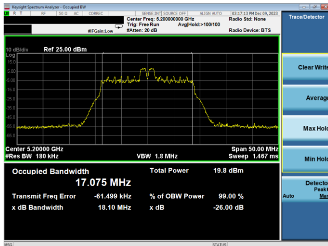
Plot 7-46. 26dB BW & 99% OBW Antenna WF2a (20MHz BW 11ax Index 4 – RU26 – Ch.40)
