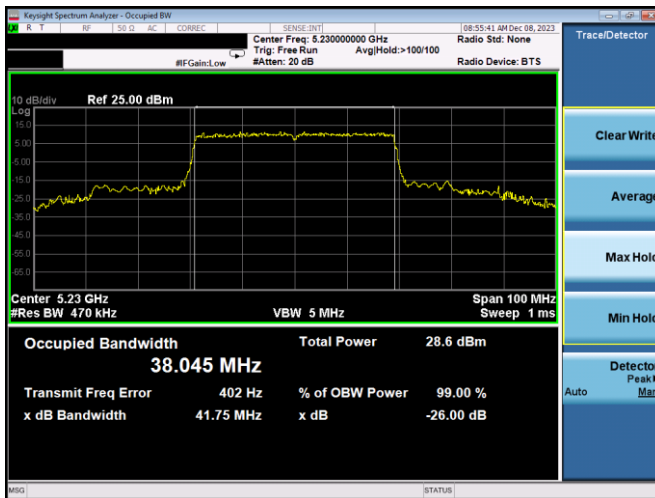
Plot 7-8. 26dB BW & 99% OBW Antenna WF7a (40MHz BW 11ax – RU484 – Ch.46)
