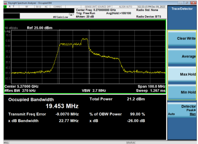
Plot 7-22. 26dB BW & 99% OBW Antenna WF7a (40MHz BW 11ax Index 40 – RU52 – Ch.54)
