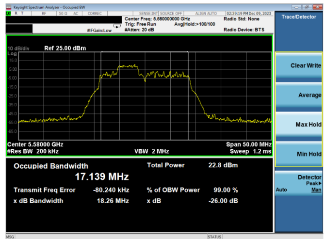
Plot 7-30. 26dB BW & 99% OBW Antenna WF7a (20MHz BW 11ax Index 38 – RU52 – Ch.116)
