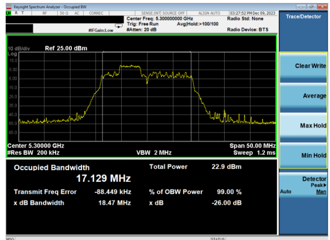
Plot 7-62. 26dB BW & 99% OBW Antenna WF2a (20MHz BW 11ax Index 38 – RU52 – Ch.60)
