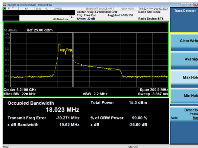
Plot 7-53. 26dB BW & 99% OBW Antenna WF2a (80MHz BW 11ax Index 0 – RU26 – Ch.42)
