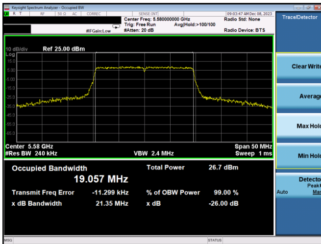
Plot 7-32. 26dB BW & 99% OBW Antenna WF7a (20MHz BW 11ax- RU242 - Ch.116)
