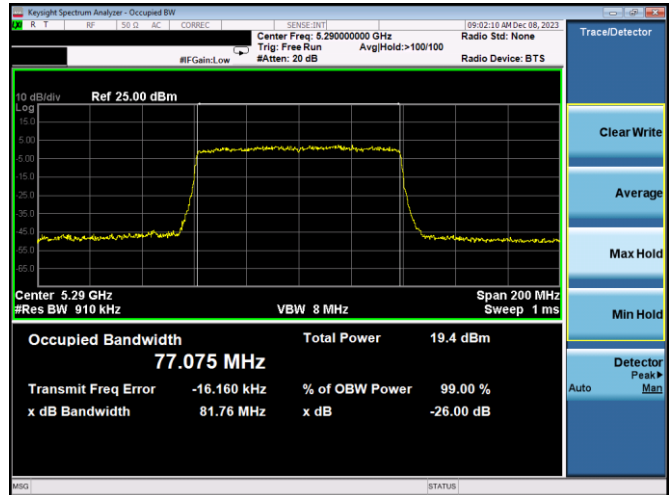
Plot 7-28. 26dB BW & 99% OBW Antenna WF7a (80MHz BW 11ax – RU996 – Ch.58)
