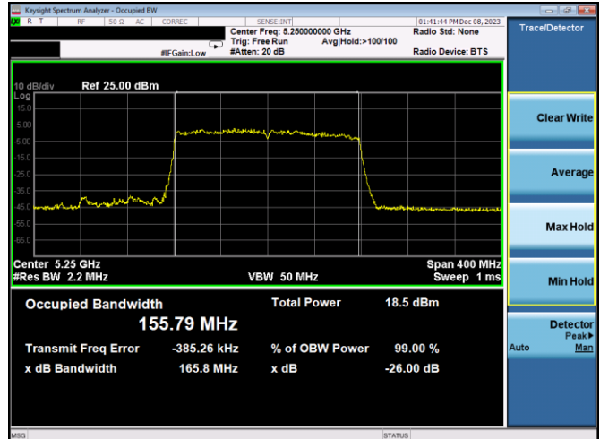
Plot 7-60. 26dB BW & 99% OBW Antenna WF2a (160MHz BW 11ax – RU996x2 – Ch.50)
