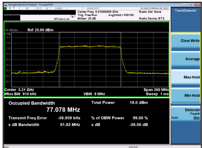
Plot 7-56. 26dB BW & 99% OBW Antenna WF2a (80MHz BW 11ax – RU996 – Ch.42)
