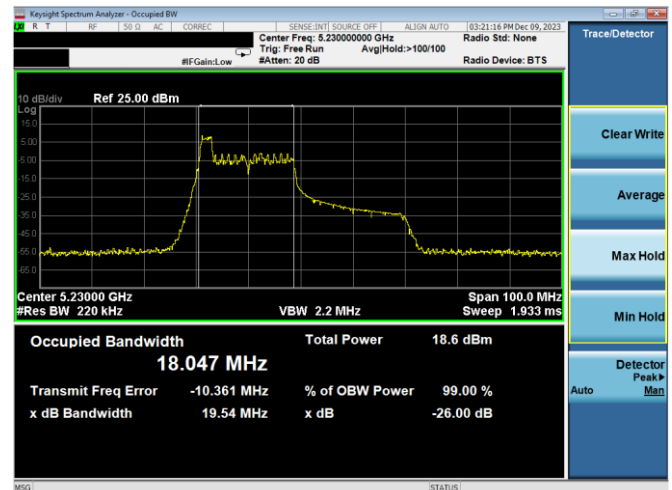
Plot 7-49. 26dB BW & 99% OBW Antenna WF2a (40MHz BW 11ax Index 0 – RU26 – Ch.46)
