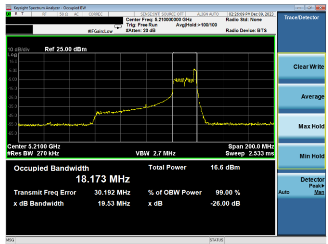
Plot 7-11. 26dB BW & 99% OBW Antenna WF7a (80MHz BW 11ax Index 36 – RU26 – Ch.42)
