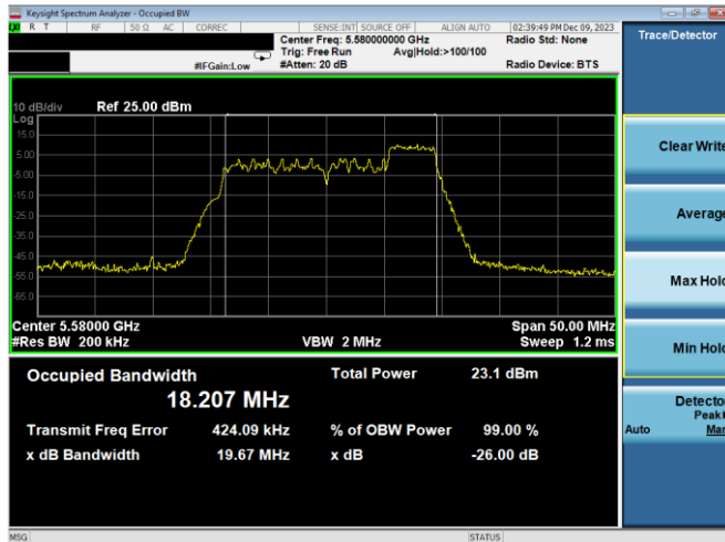
Plot 7-31. 26dB BW & 99% OBW Antenna WF7a (20MHz BW 11ax Index 40 - RU52 - Ch.116)
