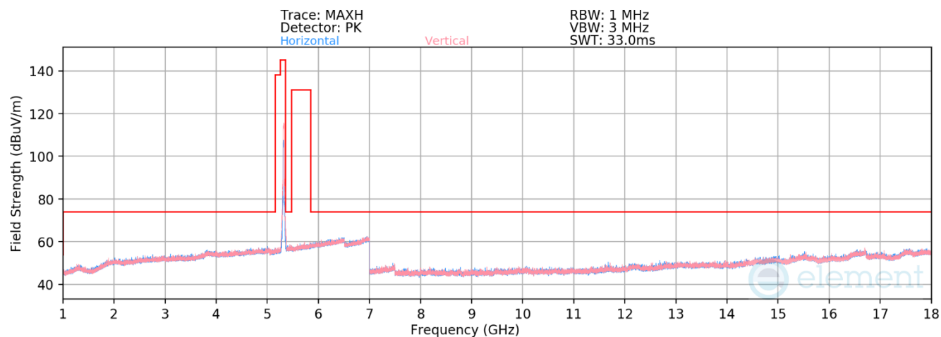
Plot 7-707. RSE above 1GHz Antenna WF2a (11ax – Ch.64 – RU242)
