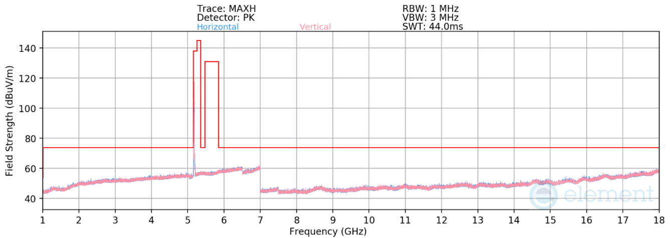
Plot 7-690. RSE above 1GHz Antenna WF2a (11ax – Ch.36 – RU26)
