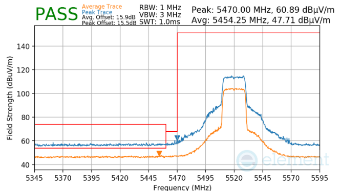
Plot 7-921. Antenna WF7b (Pk & Avg, RU242, Index 61, Ch.104, MCS11)
