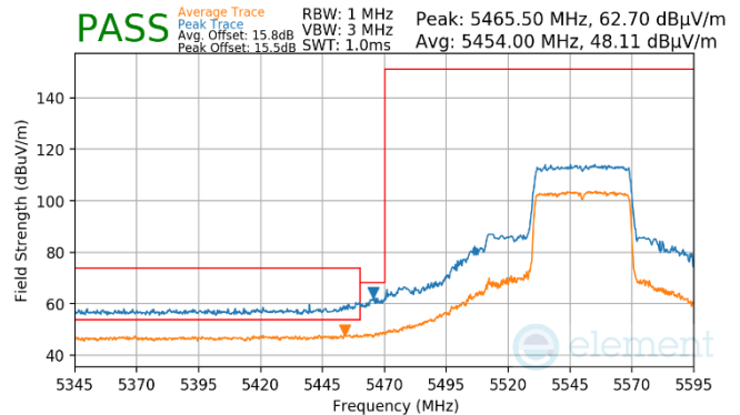
Plot 7-884. Antenna WF2a (Pk & Avg, RU484, Index 65, Ch.110, MCS11)
