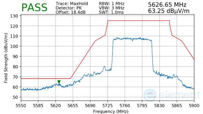
Plot 7-954. Antenna WF7b (Pk, RU996, Index 67, Ch.155, MCS11)
