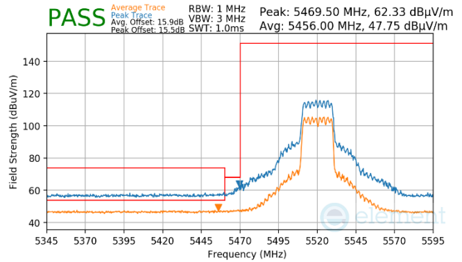
Plot 7-975. CDD Primary (Pk & Avg, RU242, Index 61, Ch.104, MCS11)
