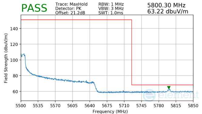
Plot 7-1013. (FCC Only) CDD Primary (Pk, RU52, Index 37, Ch.114 (U), MCS11)
