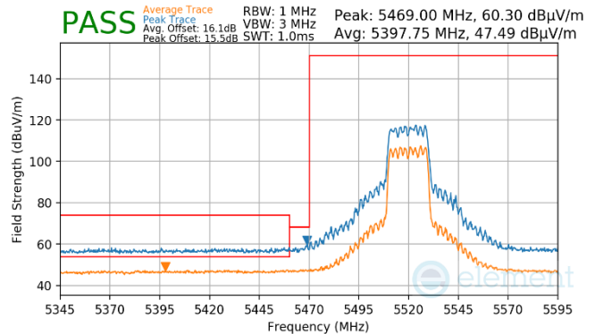
Plot 7-1029. CDD Diversity (Pk & Avg, RU242, Index 61, Ch.104, MCS11)
