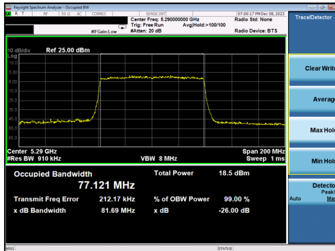
Plot 7-116. 26dB BW & 99% OBW Antenna WF7b (80MHz BW 11ax - RU996 - Ch.58)
