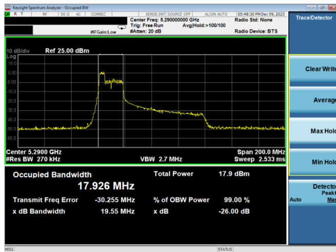
Plot 7-113. 26dB BW & 99% OBW Antenna WF7b (80MHz BW 11ax Index 37 - RU52 - Ch.58)
