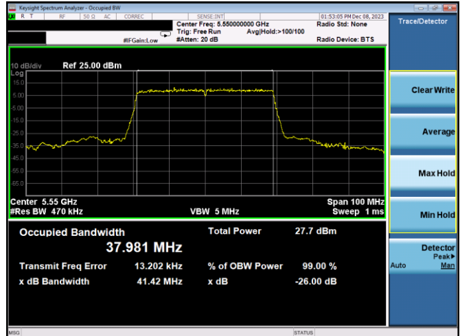
Plot 7-80. 26dB BW & 99% OBW Antenna WF2a (40MHz BW 11ax - RU484 - Ch.110)
