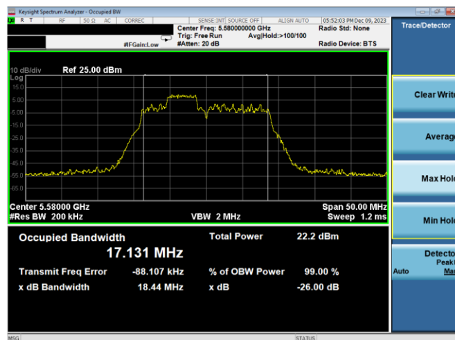
Plot 7-118. 26dB BW & 99% OBW Antenna WF7b (20MHz BW 11ax Index 38 - RU52 - Ch.116)
