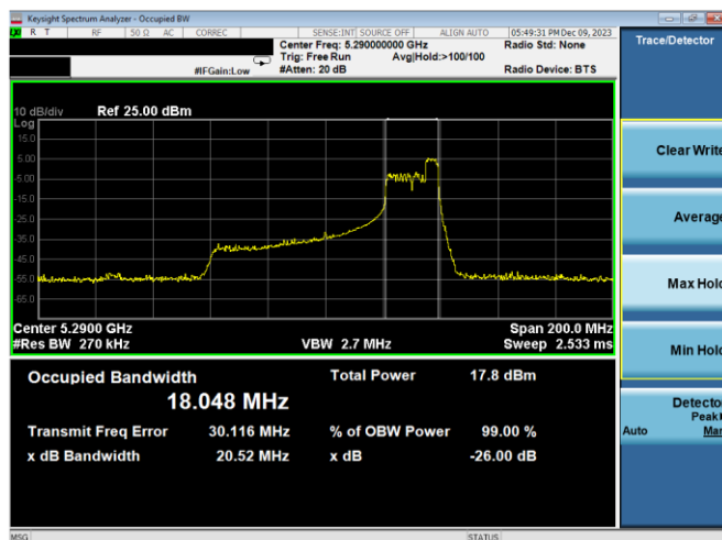
Plot 7-115. 26dB BW & 99% OBW Antenna WF7b (80MHz BW 11ax Index 52 - RU52 - Ch.58)
