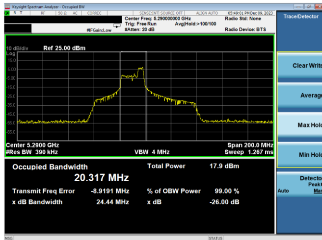
Plot 7-114. 26dB BW & 99% OBW Antenna WF7b (80MHz BW 11ax Index 44 - RU52 - Ch.58)
