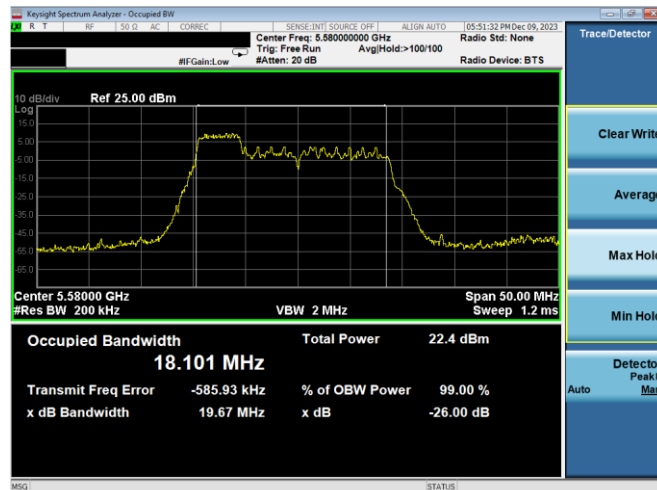
Plot 7-117. 26dB BW & 99% OBW Antenna WF7b (20MHz BW 11ax Index 37 - RU52 - Ch.116)
