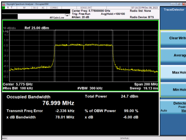
Plot 7-168. 6dB BW & 99% OBW Antenna WF7b (80MHz BW 11ax – RU996 – Ch.155)
