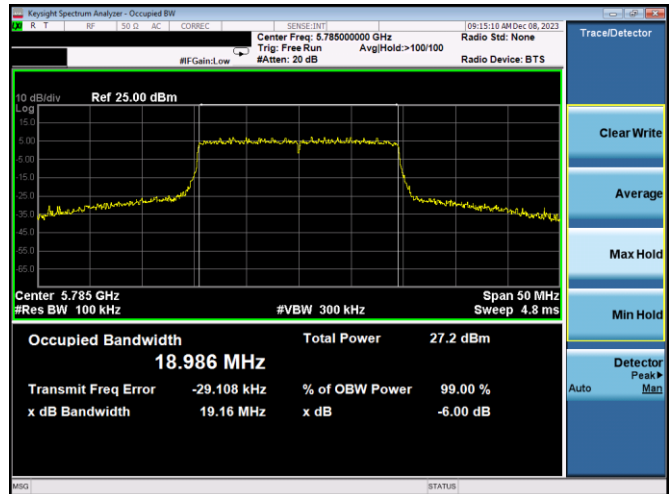
Plot 7-136. 6dB BW & 99% OBW Antenna WF7a (20MHz BW 11ax – RU242 – Ch.157)
