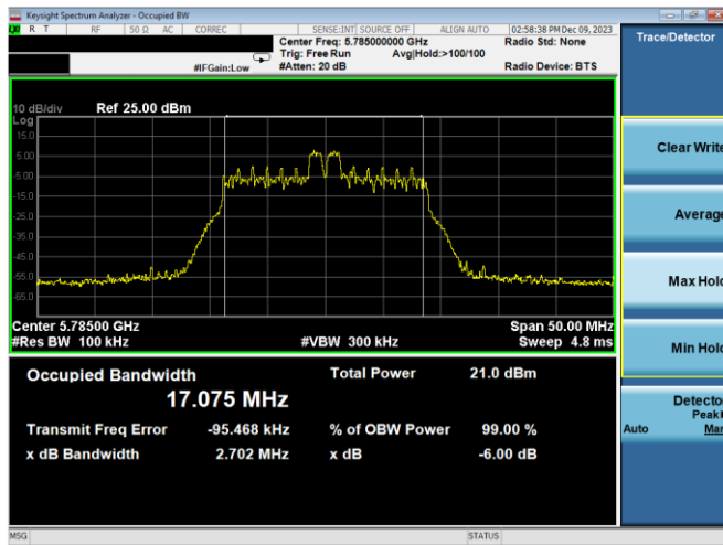
Plot 7-134. 6dB BW & 99% OBW Antenna WF7a (20MHz BW 11ax Index 4 – RU26 – Ch.157)
