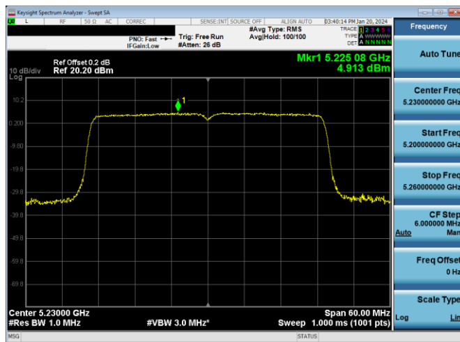
Plot 7-176. PSD Antenna WF7a (40MHz BW 11ax - RU484 - Ch.46)
