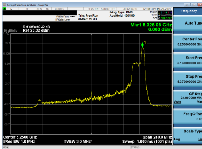
Plot 7-183. PSD Antenna WF7a (160MHz BW 11ax Index 52 - RU52 - Ch.50 (U))
