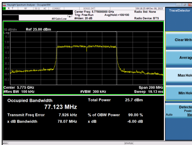
Plot 7-144. 6dB BW & 99% OBW Antenna WF7a (80MHz BW 11ax – RU996 – Ch.155)
