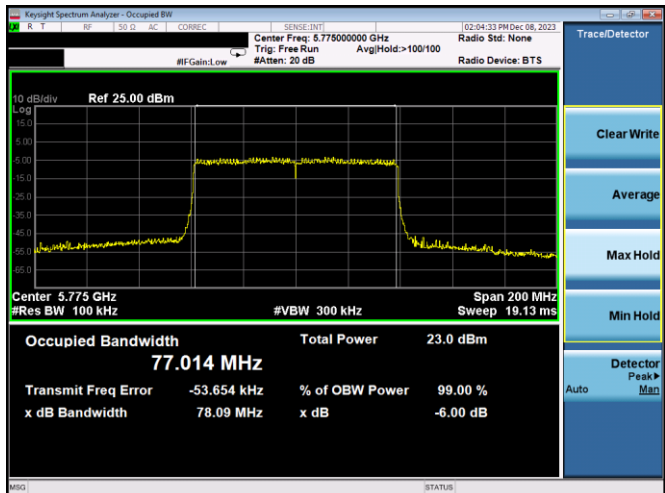
Plot 7-156. 6dB BW & 99% OBW Antenna WF2a (80MHz BW 11ax – RU996 – Ch.155)
