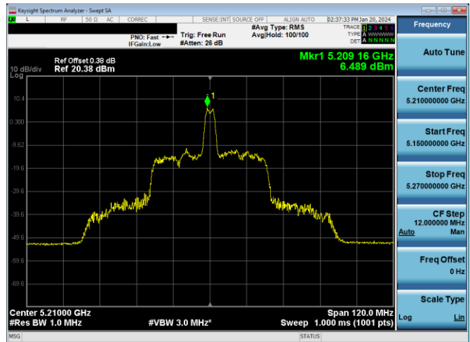
Plot 7-178. PSD Antenna WF7a (80MHz BW 11ax Index 18 - RU26 - Ch.42)
