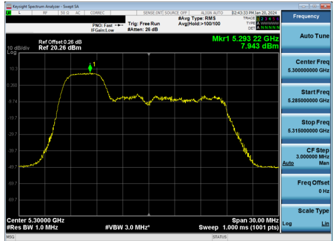
Plot 7-185. PSD Antenna WF7a (20MHz BW 11ax Index 37 - RU52 - Ch.60)
