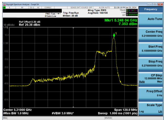
Plot 7-179. PSD Antenna WF7a (80MHz BW 11ax Index 36 - RU26 - Ch.42)
