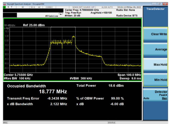
Plot 7-138. 6dB BW & 99% OBW Antenna WF7a (40MHz BW 11ax Index 8 – RU26 – Ch.151)
