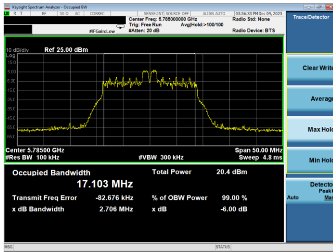
Plot 7-146. 6dB BW & 99% OBW Antenna WF2a (20MHz BW 11ax Index 4 - RU26 - Ch.157)
