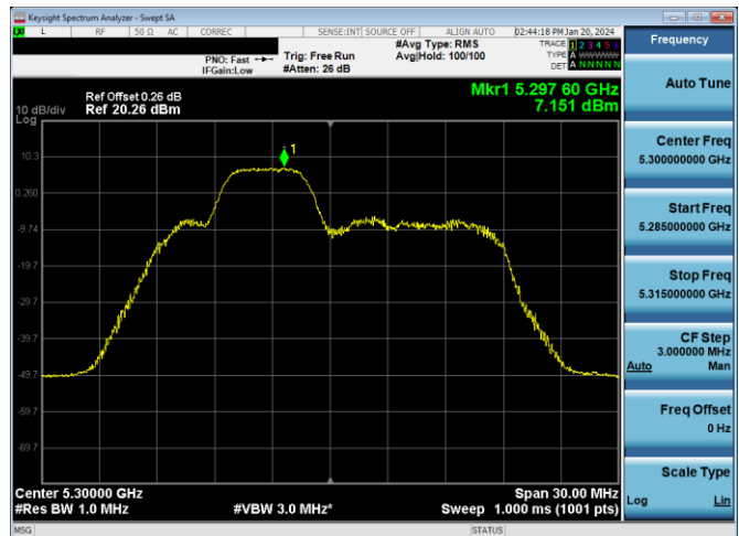
Plot 7-186. PSD Antenna WF7a (20MHz BW 11ax Index 38 - RU52 - Ch.60)
