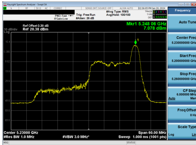
Plot 7-175. PSD Antenna WF7a (40MHz BW 11ax Index 17 - RU26 - Ch.46)
