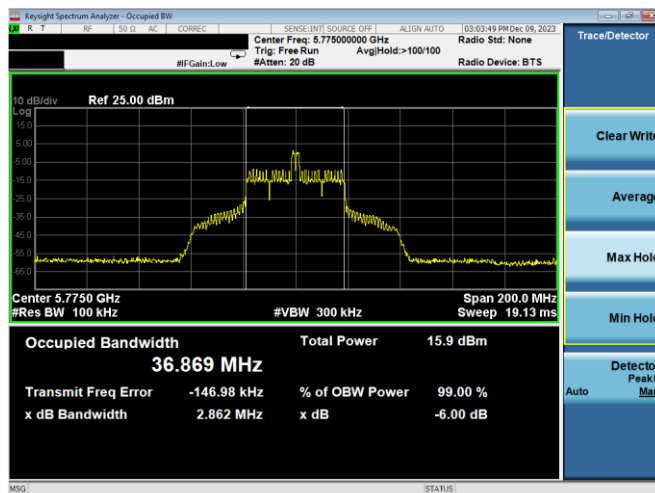
Plot 7-142. 6dB BW & 99% OBW Antenna WF7a (80MHz BW 11ax Index 18 – RU26 – Ch.155)
