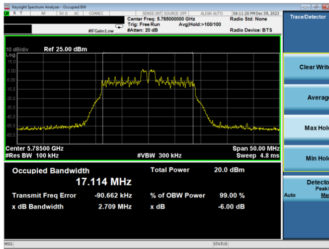
Plot 7-158. 6dB BW & 99% OBW Antenna WF7b (20MHz BW 11ax Index 4 - RU26 - Ch.157)
