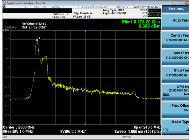
Plot 7-181. PSD Antenna WF7a (160MHz BW 11ax Index 37 - RU52 - Ch.50 (L))
