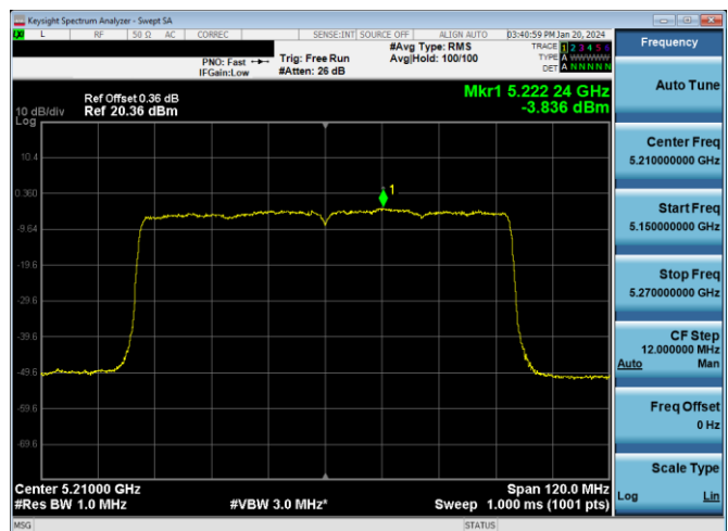
Plot 7-180. PSD Antenna WF7a (80MHz BW 11ax - RU996 - Ch.42)
