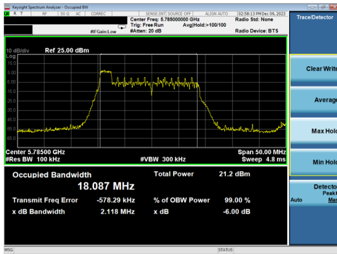
Plot 7-133. 6dB BW & 99% OBW Antenna WF7a (20MHz BW 11ax Index 0 – RU26 – Ch.157)
