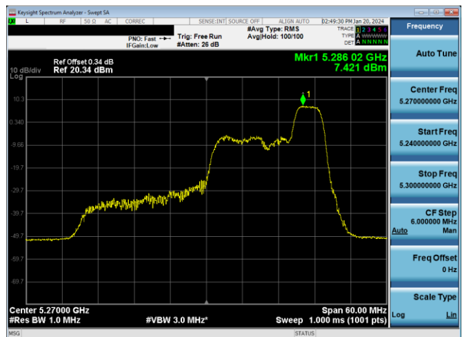
Plot 7-191. PSD Antenna WF7a (40MHz BW 11ax Index 44 - RU52 - Ch.54)
