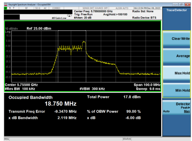
Plot 7-162. 6dB BW & 99% OBW Antenna WF7b (40MHz BW 11ax Index 8 - RU26 - Ch.151)
