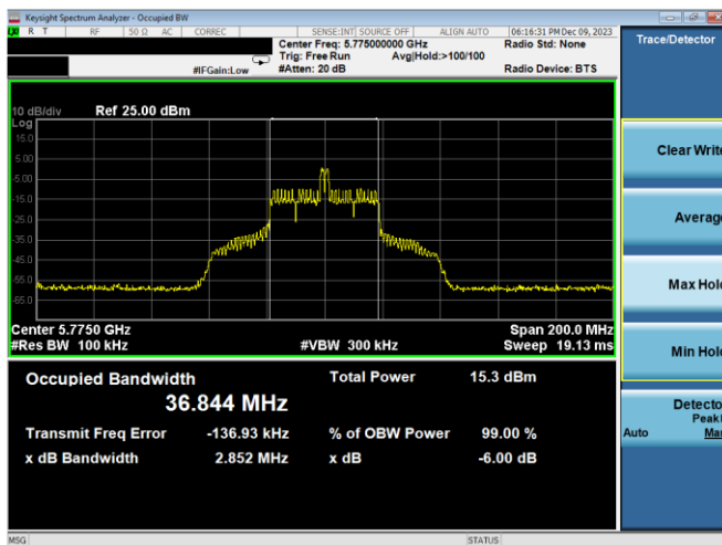
Plot 7-166. 6dB BW & 99% OBW Antenna WF7b (80MHz BW 11ax Index 18 – RU26 – Ch.155)
