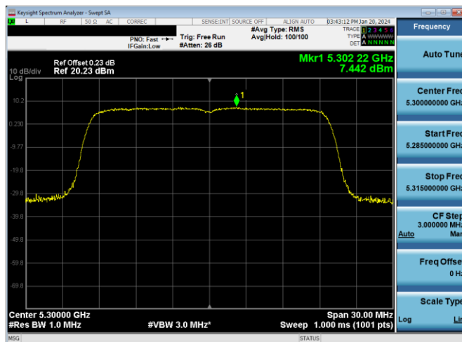
Plot 7-188. PSD Antenna WF7a (20MHz BW 11ax - RU242 - Ch.60)
