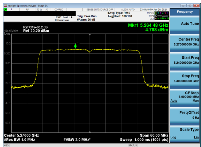
Plot 7-192. PSD Antenna WF7a (40MHz BW 11ax - RU484 - Ch.54)
