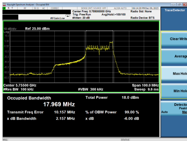
Plot 7-163. 6dB BW & 99% OBW Antenna WF7b (40MHz BW 11ax Index 17 – RU26 – Ch.151)
