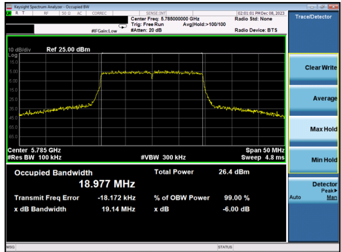
Plot 7-148. 6dB BW & 99% OBW Antenna WF2a (20MHz BW 11ax - RU242 - Ch.157)
