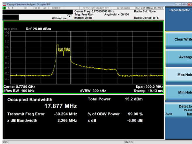
Plot 7-165. 6dB BW & 99% OBW Antenna WF7b (80MHz BW 11ax Index 0 – RU26 – Ch.155)
