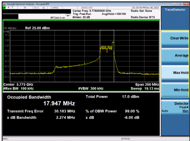
Plot 7-155. 6dB BW & 99% OBW Antenna WF2a (80MHz BW 11ax Index 36 – RU26 – Ch.155)
