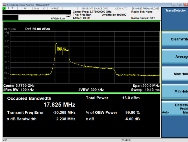
Plot 7-141. 6dB BW & 99% OBW Antenna WF7a (80MHz BW 11ax Index 0 – RU26 – Ch.155)
