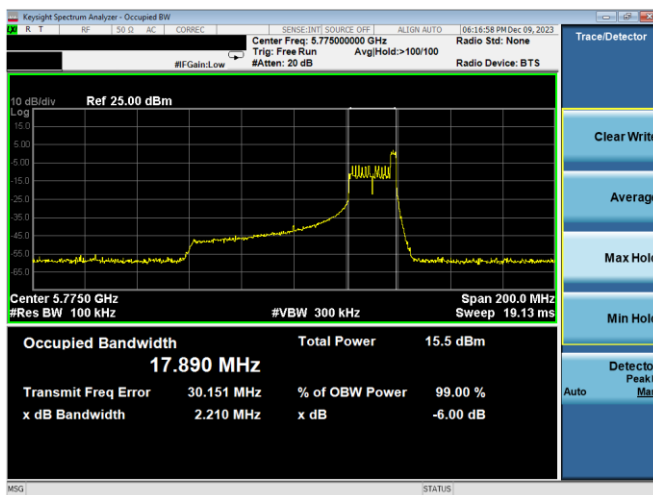
Plot 7-167. 6dB BW & 99% OBW Antenna WF7b (80MHz BW 11ax Index 36 – RU26 – Ch.155)
