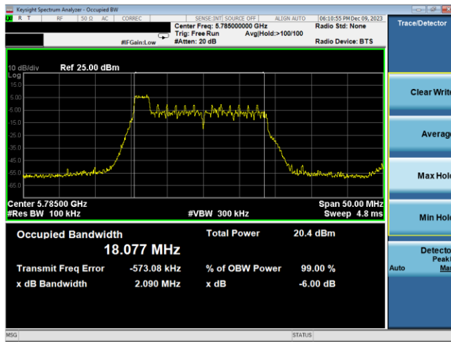
Plot 7-157. 6dB BW & 99% OBW Antenna WF7b (20MHz BW 11ax Index 0 - RU26 - Ch.157)
