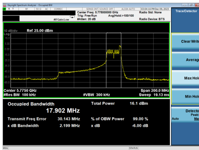
Plot 7-143. 6dB BW & 99% OBW Antenna WF7a (80MHz BW 11ax Index 36 – RU26 – Ch.155)
