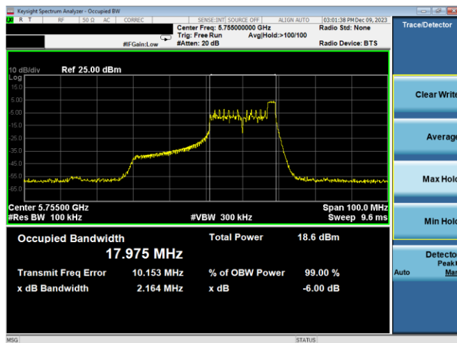
Plot 7-139. 6dB BW & 99% OBW Antenna WF7a (40MHz BW 11ax Index 17 – RU26 – Ch.151)
