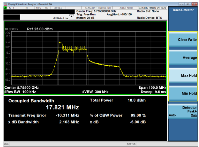
Plot 7-149. 6dB BW & 99% OBW Antenna WF2a (40MHz BW 11ax Index 0 - RU26 - Ch.151)
