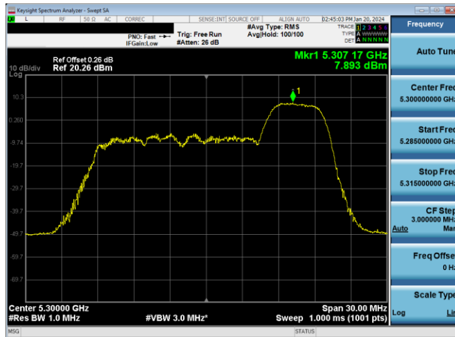
Plot 7-187. PSD Antenna WF7a (20MHz BW 11ax Index 40 - RU52 - Ch.60)
