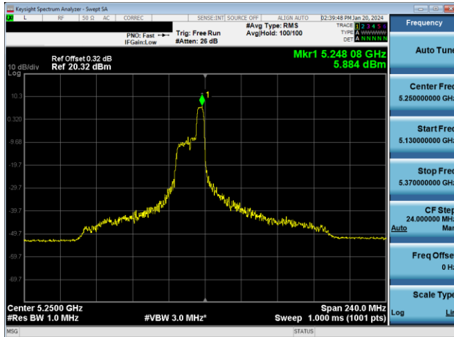
Plot 7-182. PSD Antenna WF7a (160MHz BW 11ax Index 52 - RU52 - Ch.50 (L))
