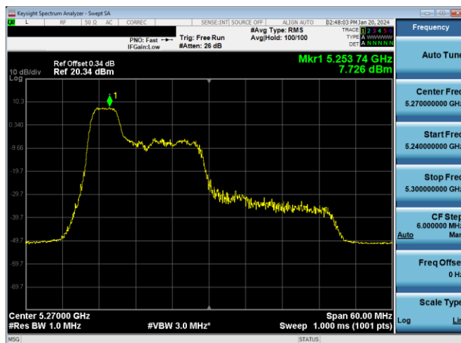
Plot 7-189. PSD Antenna WF7a (40MHz BW 11ax Index 37 - RU52 - Ch.54)
