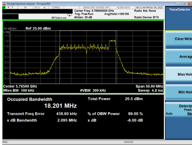
Plot 7-159. 6dB BW & 99% OBW Antenna WF7b (20MHz BW 11ax Index 8 - RU26 - Ch.157)
