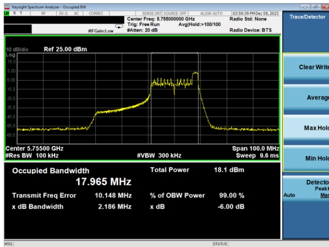
Plot 7-151. 6dB BW & 99% OBW Antenna WF2a (40MHz BW 11ax Index 17 – RU26 – Ch.151)
