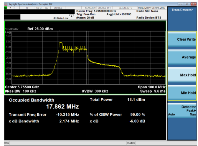
Plot 7-161. 6dB BW & 99% OBW Antenna WF7b (40MHz BW 11ax Index 0 - RU26 - Ch.151)
