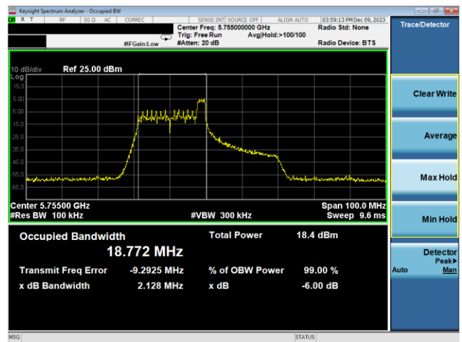
Plot 7-150. 6dB BW & 99% OBW Antenna WF2a (40MHz BW 11ax Index 8 - RU26 - Ch.151)
