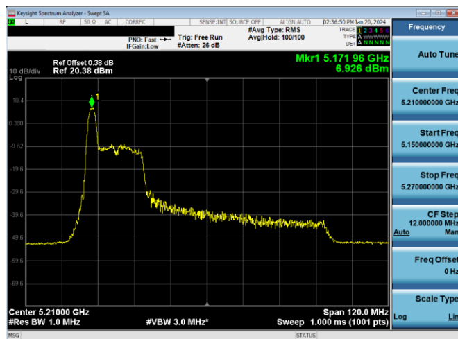
Plot 7-177. PSD Antenna WF7a (80MHz BW 11ax Index 0 - RU26 - Ch.42)
