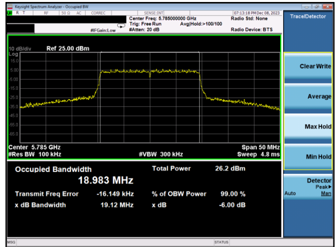
Plot 7-160. 6dB BW & 99% OBW Antenna WF7b (20MHz BW 11ax - RU242 - Ch.157)
