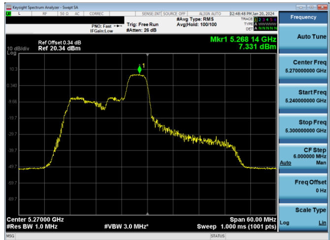
Plot 7-190. PSD Antenna WF7a (40MHz BW 11ax Index 40 - RU52 - Ch.54)
