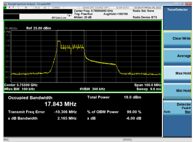
Plot 7-137. 6dB BW & 99% OBW Antenna WF7a (40MHz BW 11ax Index 0 – RU26 – Ch.151)
