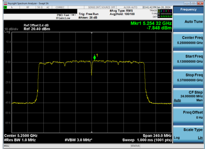
Plot 7-184. PSD Antenna WF7a (160MHz BW 11ax - RU996x2 - Ch.50)
