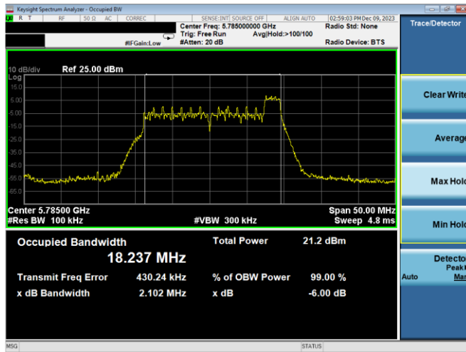
Plot 7-135. 6dB BW & 99% OBW Antenna WF7a (20MHz BW 11ax Index 8 – RU26 – Ch.157)
