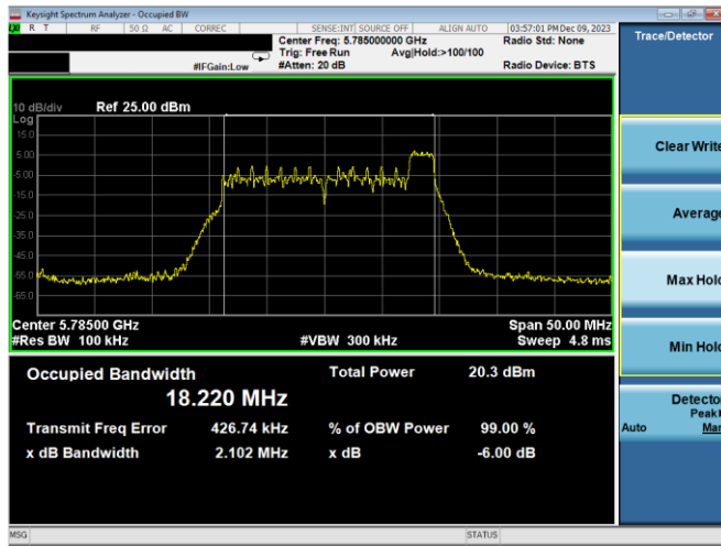
Plot 7-147. 6dB BW & 99% OBW Antenna WF2a (20MHz BW 11ax Index 8 - RU26 - Ch.157)
