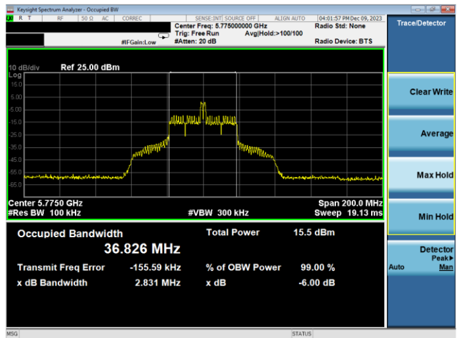
Plot 7-154. 6dB BW & 99% OBW Antenna WF2a (80MHz BW 11ax Index 18 – RU26 – Ch.155)
