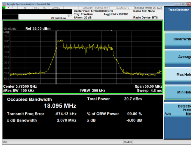
Plot 7-145. 6dB BW & 99% OBW Antenna WF2a (20MHz BW 11ax Index 0 - RU26 - Ch.157)
