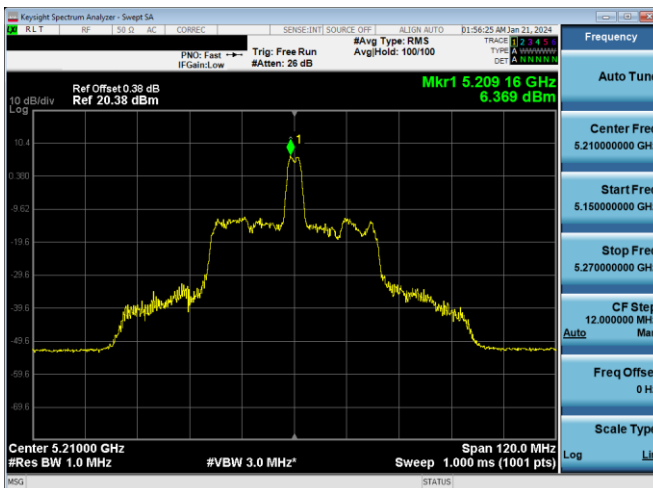
Plot 7-249. PSD Antenna WF2a (80MHz BW 11ax Index 18 - RU26 - Ch.42)
