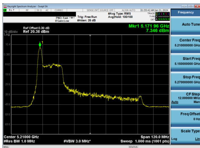
Plot 7-248. PSD Antenna WF2a (80MHz BW 11ax Index 0 - RU26 - Ch.42)
