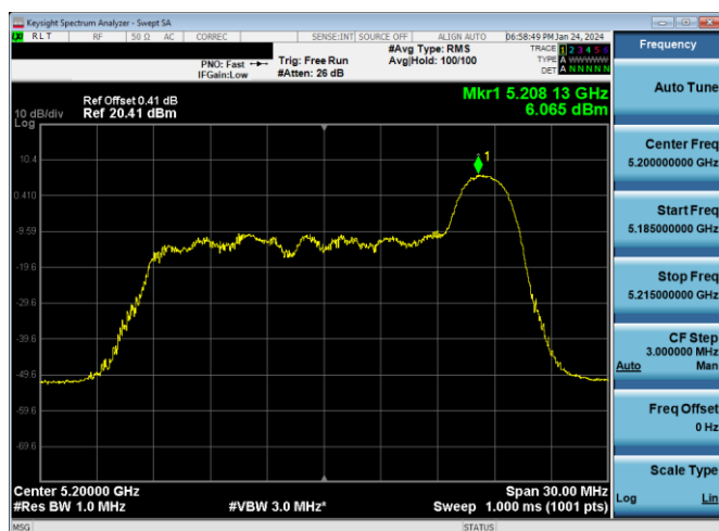
Plot 7-227. ISD PSD Antenna WF7a (20MHz BW 11ax Index 8 - RU26 - Ch.40)
