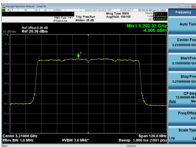
Plot 7-251. PSD Antenna WF2a (80MHz BW 11ax - RU996 - Ch.42)
