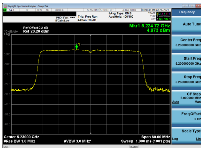
Plot 7-247. PSD Antenna WF2a (40MHz BW 11ax - RU484 - Ch.46)
