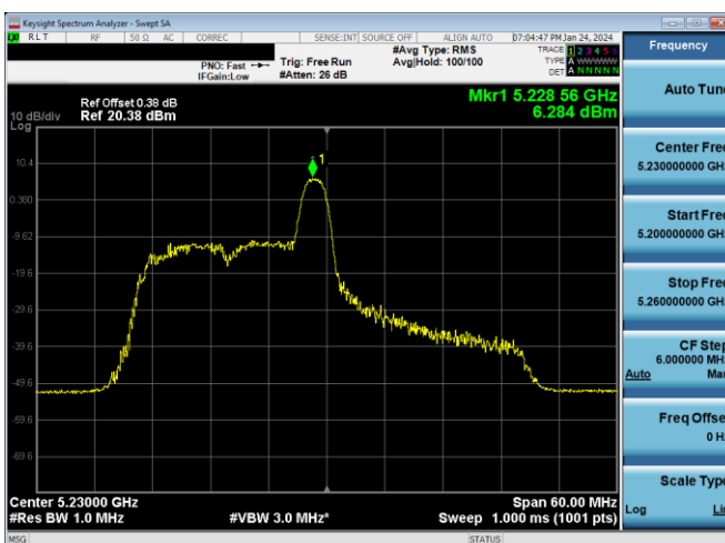
Plot 7-230. ISD PSD Antenna WF7a (40MHz BW 11ax Index 8 - RU26 - Ch.46)
