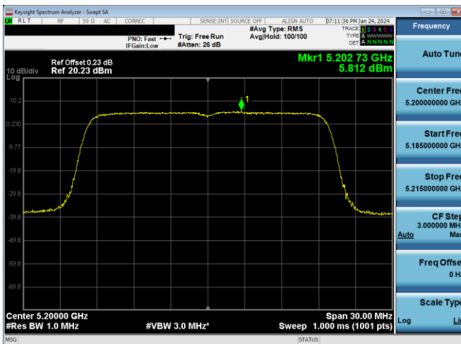
Plot 7-228. ISD PSD Antenna WF7a (20MHz BW 11ax- RU242 - Ch.40)
