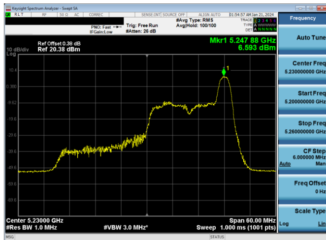
Plot 7-246. PSD Antenna WF2a (40MHz BW 11ax Index 17 - RU26 - Ch.46)
