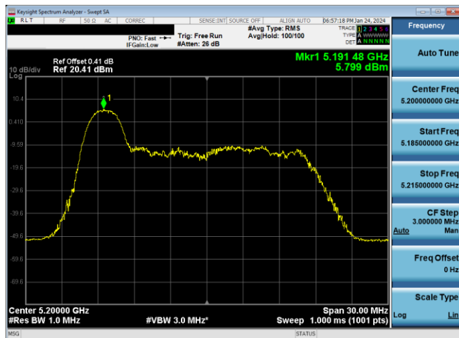
Plot 7-225. ISD PSD Antenna WF7a (20MHz BW 11ax Index 0 - RU26 - Ch.40)
