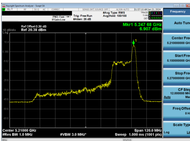
Plot 7-250. PSD Antenna WF2a (80MHz BW 11ax Index 18 - RU26 - Ch.42)
