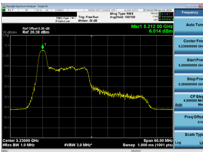
Plot 7-229. ISD PSD Antenna WF7a (40MHz BW 11ax- RU26 - Ch.46)
