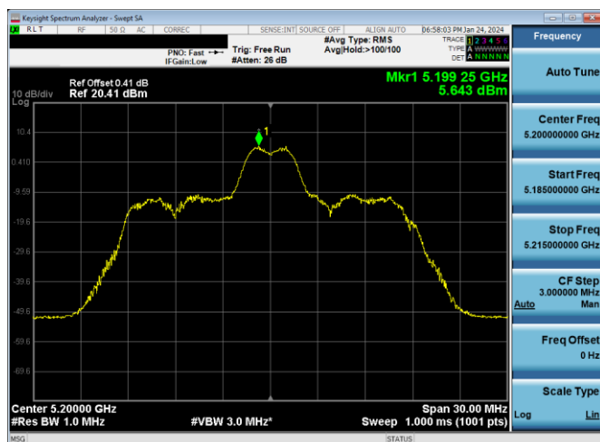
Plot 7-226. ISD PSD Antenna WF7a (20MHz BW 11ax Index 4 - RU26 - Ch.40)
