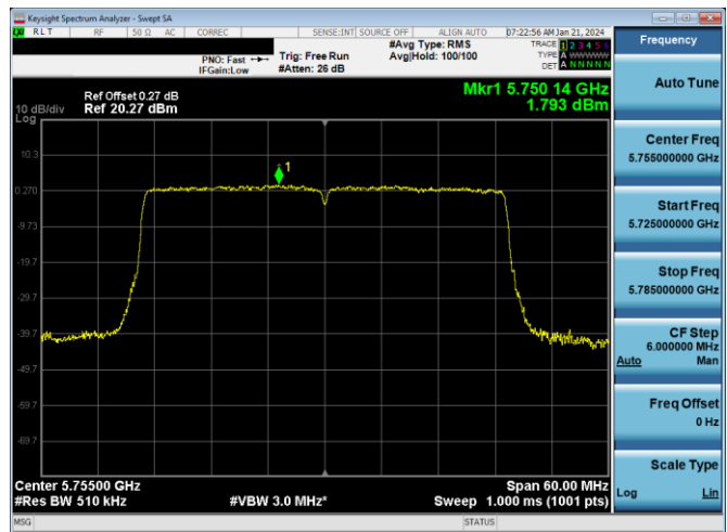
Plot 7-485. PSD CDD Primary Antenna WF2a (40MHz BW 11ax - RU484 - Ch.151)
