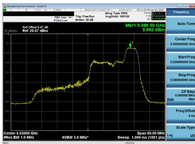
Plot 7-450. PSD CDD Primary Antenna WF7a (40MHz BW 11ax Index 44 - RU52 - Ch.110)
