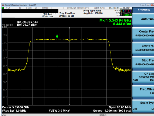
Plot 7-453. PSD CDD Primary Antenna WF2a (40MHz BW 11ax - RU484 - Ch.110)
