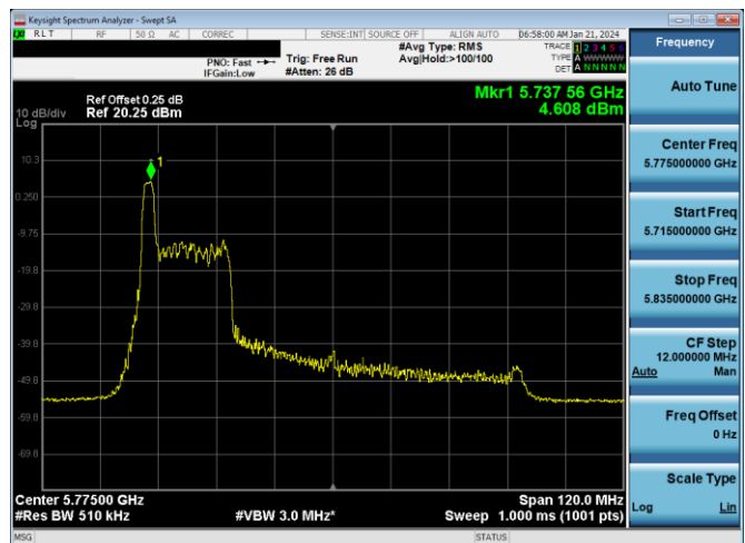
Plot 7-487. PSD CDD Primary Antenna WF2a (80MHz BW 11ax Index 0 - RU26 - Ch.155)
