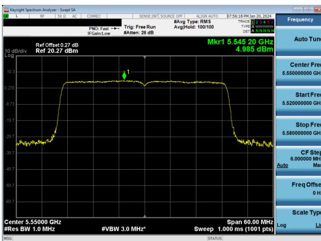
Plot 7-452. PSD CDD Primary Antenna WF7a (40MHz BW 11ax - RU484 - Ch.110)
