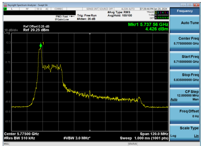
Plot 7-486. PSD CDD Primary Antenna WF7a (80MHz BW 11ax Index 0 - RU26 - Ch.155)
