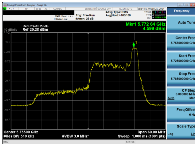
Plot 7-483. PSD CDD Primary Antenna WF2a (40MHz BW 11ax Index 17 - RU26 - Ch.151)
