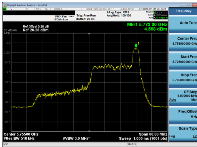
Plot 7-482. PSD CDD Primary Antenna WF7a (40MHz BW 11ax Index 17 - RU26 - Ch.151)
