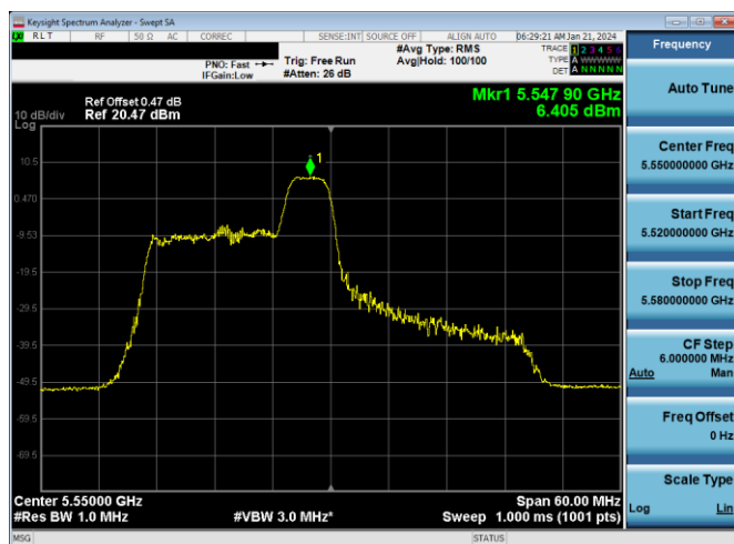
Plot 7-449. PSD CDD Primary Antenna WF2a (40MHz BW 11ax Index 40 - RU52 - Ch.110)
