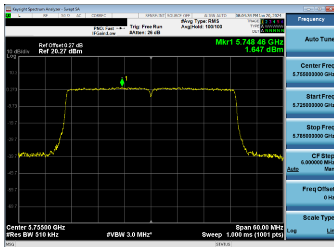
Plot 7-484. PSD CDD Primary Antenna WF7a (40MHz BW 11ax - RU484 - Ch.151)
