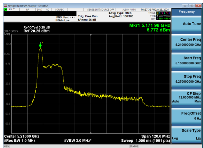
Plot 7-541. PSD CDD Diversity Antenna WF7b (80MHz BW 11ax Index 0 - RU26 - Ch.42)
