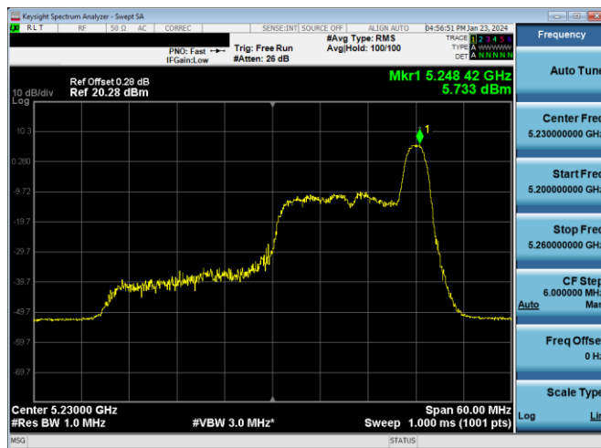
Plot 7-537. PSD CDD Diversity Antenna WF7a (40MHz BW 11ax Index 17 - RU26 - Ch.46)
