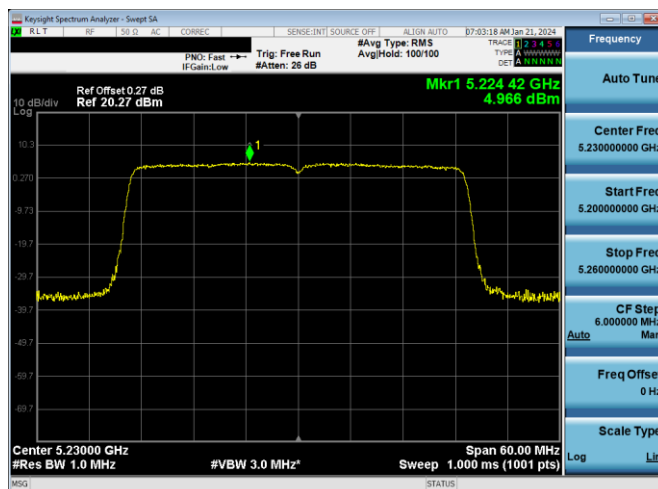
Plot 7-538. PSD CDD Diversity Antenna WF7a (40MHz BW 11ax - RU484 - Ch.46)
