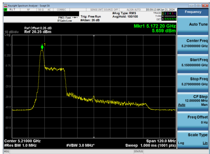
Plot 7-540. PSD CDD Diversity Antenna WF7a (80MHz BW 11ax Index 0 - RU26 - Ch.42)
