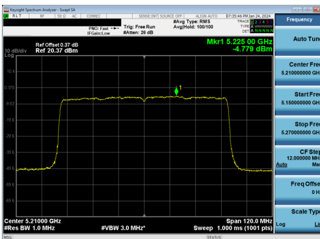
Plot 7-516. ISED PSD SDM Primary Antenna WF7a (80MHz BW 11ax - RU96 - Ch.42)
