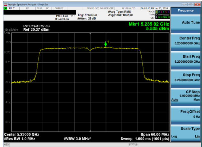
Plot 7-539. PSD CDD Diversity Antenna WF7b (40MHz BW 11ax - RU484 - Ch.46)
