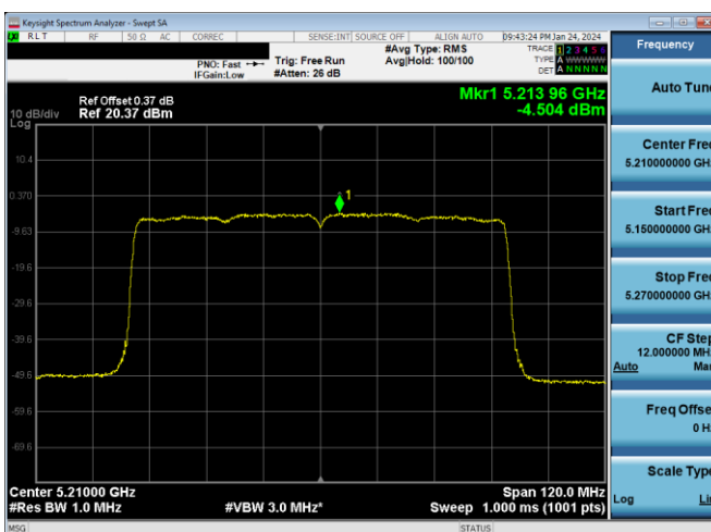
Plot 7-517. ISED PSD SDM Primary Antenna WF2a (80MHz BW 11ax - RU96 - Ch.42)
