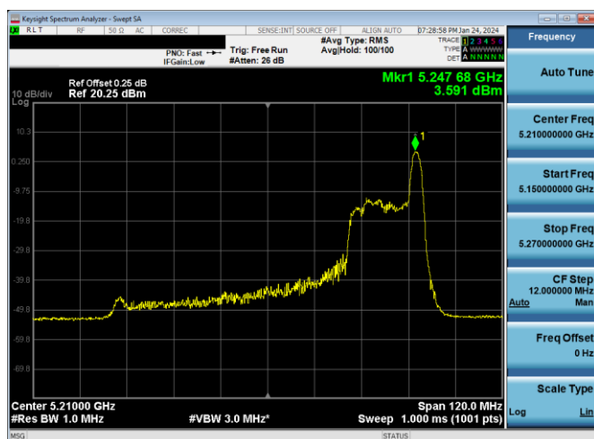
Plot 7-514. ISED PSD SDM Primary Antenna WF7a (80MHz BW 11ax Index 36 - RU26 - Ch.42)
