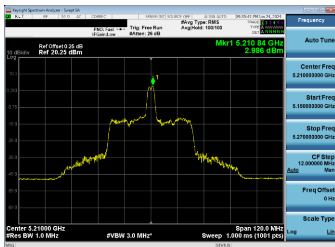
Plot 7-513. ISED PSD SDM Primary Antenna WF2a (80MHz BW 11ax Index 18 - RU26 - Ch.42)
