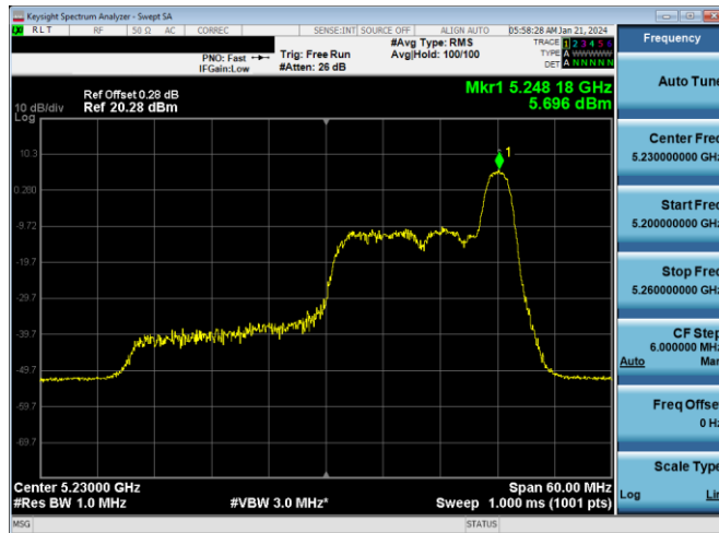
Plot 7-536. PSD CDD Diversity Antenna WF7a (40MHz BW 11ax Index 17 - RU26 - Ch.46)
