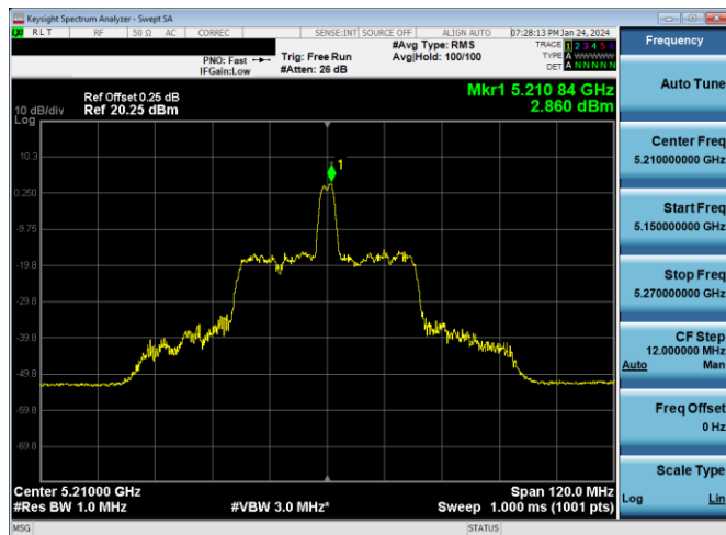
Plot 7-512. ISED PSD SDM Primary Antenna WF7a (80MHz BW 11ax Index 18 - RU26 - Ch.42)
