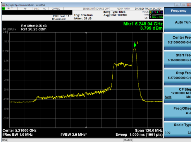
Plot 7-515. ISED PSD SDM Primary Antenna WF2a (80MHz BW 11ax Index 36 - RU26 - Ch.42)
