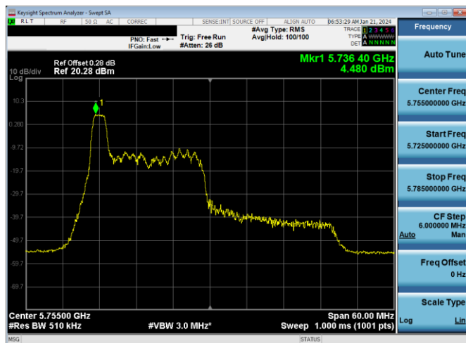
Plot 7-620. PSD CDD Diversity Antenna WF7a (40MHz BW 11ax Index 0 - RU26 - Ch.151)
