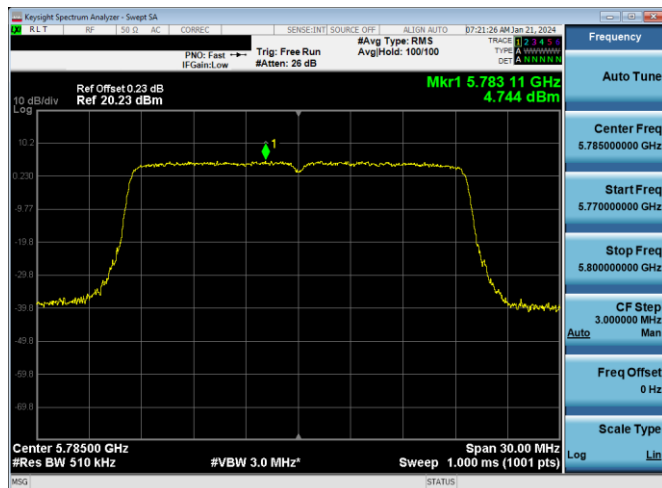
Plot 7-618. PSD CDD Diversity Antenna WF7a (20MHz BW 11ax - RU242 - Ch.157)
