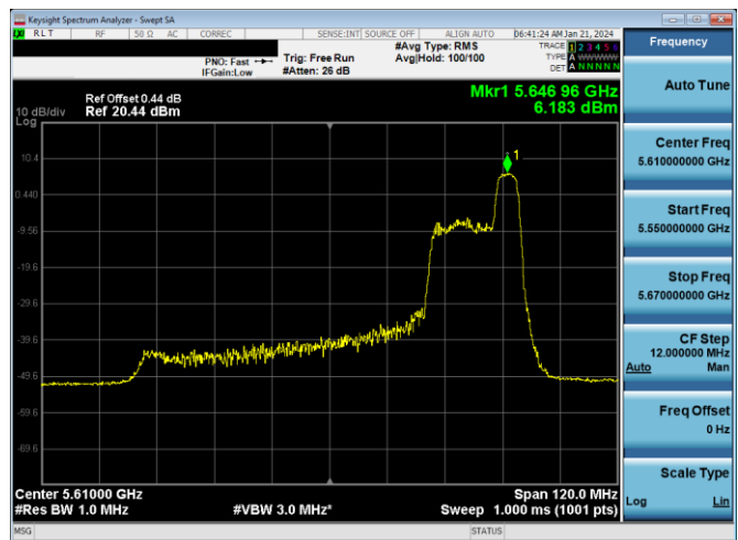
Plot 7-600. PSD CDD Diversity Antenna WF7a (80MHz BW 11ax Index 52 - RU52 - Ch.122)
