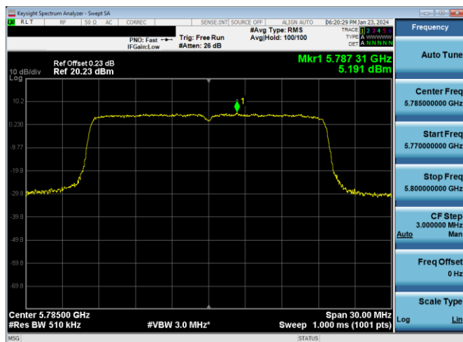
Plot 7-619. PSD CDD Diversity Antenna WF7b (20MHz BW 11ax - RU242 - Ch.157)
