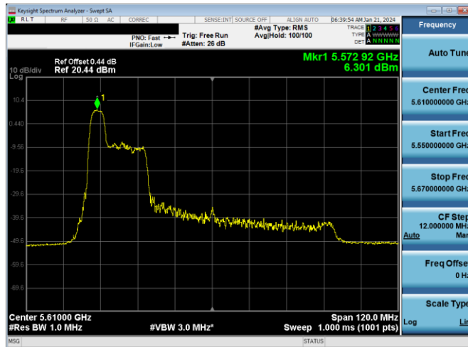
Plot 7-596. PSD CDD Diversity Antenna WF7a (80MHz BW 11ax Index 37 - RU52 - Ch.122)
