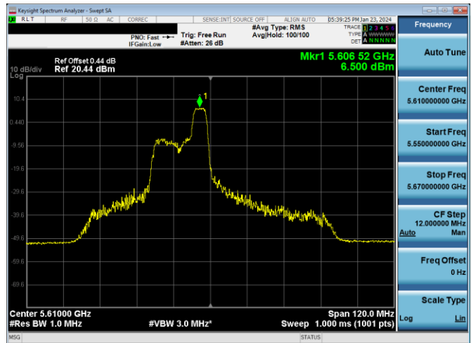
Plot 7-599. PSD CDD Diversity Antenna WF7b (80MHz BW 11ax Index 44 - RU52 - Ch.122)
