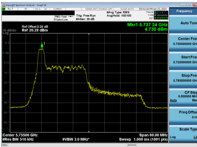
Plot 7-621. PSD CDD Diversity Antenna WF7b (40MHz BW 11ax Index 0 - RU26 - Ch.151)
