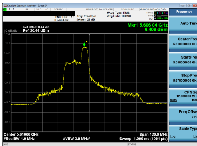
Plot 7-598. PSD CDD Diversity Antenna WF7a (80MHz BW 11ax Index 44 - RU52 - Ch.122)
