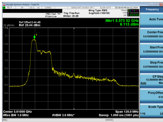
Plot 7-597. PSD CDD Diversity Antenna WF7b (80MHz BW 11ax Index 37 - RU52 - Ch.122)
