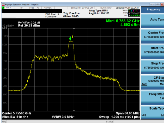
Plot 7-623. PSD CDD Diversity Antenna WF7b (40MHz BW 11ax Index 8 - RU26 - Ch.151)
