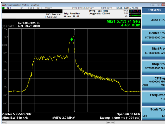
Plot 7-622. PSD CDD Diversity Antenna WF7a (40MHz BW 11ax Index 8 - RU26 - Ch.151)
