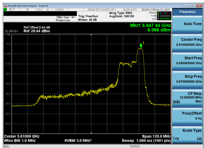
Plot 7-601. PSD CDD Diversity Antenna WF7b (80MHz BW 11ax Index 52 - RU52 - Ch.122)
