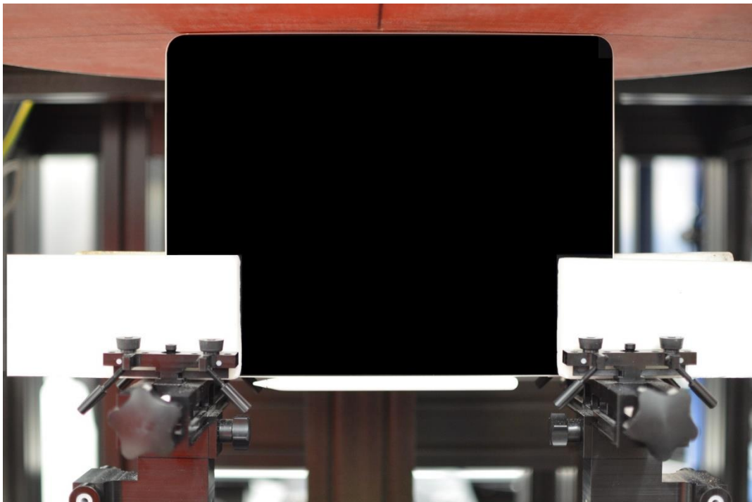
Wireless Power Transfer (wPT) Test Setup Photo 15: Left Edge
