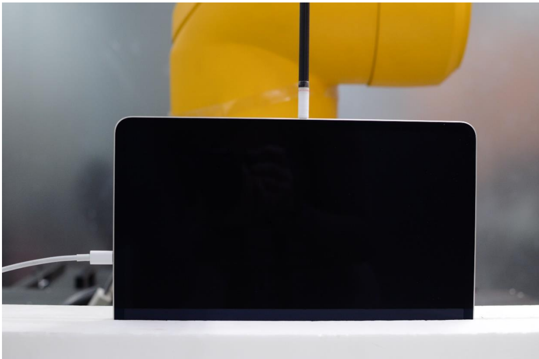
Near Field Power Density Test Setup Photo 21: Left Edge at 2mm – WF7a/7b/2a
