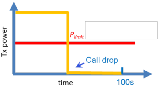
Figure 2-1 Transmit at high power when needed and permitted
