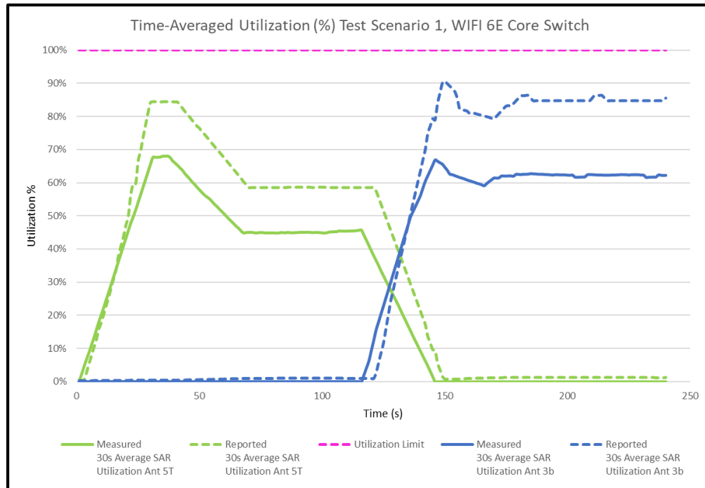
Figure J-5 30s Average SAR Utilization vs. Time, 6 GHz #1
