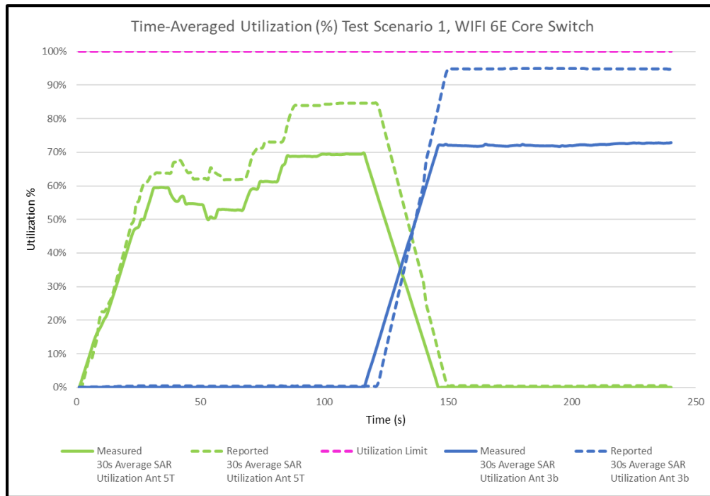
Figure J-5 30s Average SAR Utilization vs. Time, 6 GHz #2
