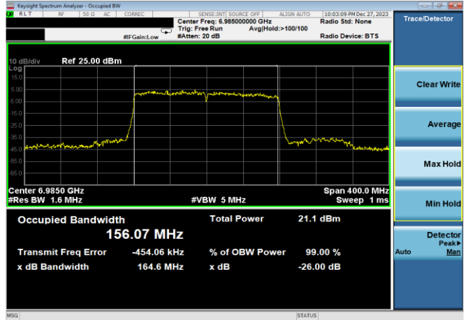
Plot 7-60. 26dB & 99% Bandwidth Plot Antenna 5T (160MHz 802.11ax (UNII Band 8) – Ch. 207, MCS11)
