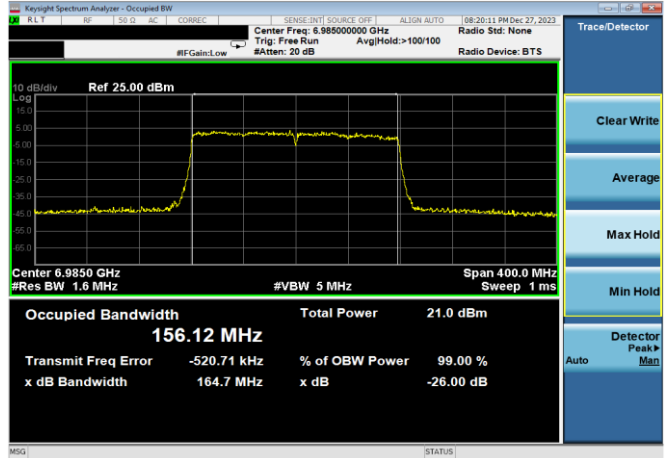
Plot 7-20. 26dB & 99% Bandwidth Plot Antenna 5T (160MHz 802.11ax (UNII Band 8) – Ch. 207, MCS2)
