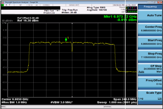
Plot 7-689. Power Spectral Density Plot SDM Diversity Antenna 3b LPI (160MHz 802.11ax (UNII Band 8) – Ch. 207, MCS11)
