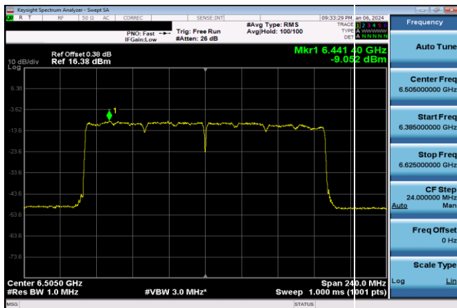
Plot 7-673. Power Spectral Density Plot SDM Diversity Antenna 3b LPI (160MHz 802.11ax (UNII Band 6) – Ch. 111, MCS11)
