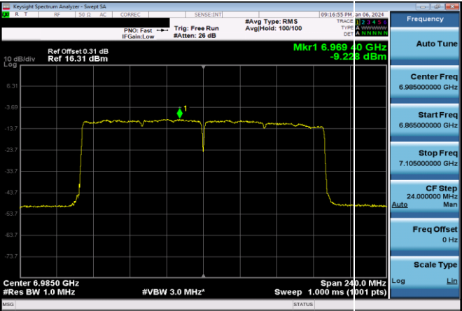
Plot 7-657. Power Spectral Density Plot SDM Diversity Antenna 3b LPI (160MHz 802.11ax (UNII Band 8) – Ch. 207, MCS4)
