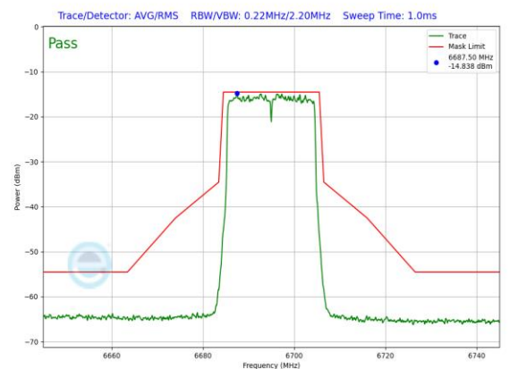
Plot 7-950. LPI In-Band Emission Plot Antenna 1b (20MHz 802.11ax (UNII Band 7) – Ch. 149, MCS4)
