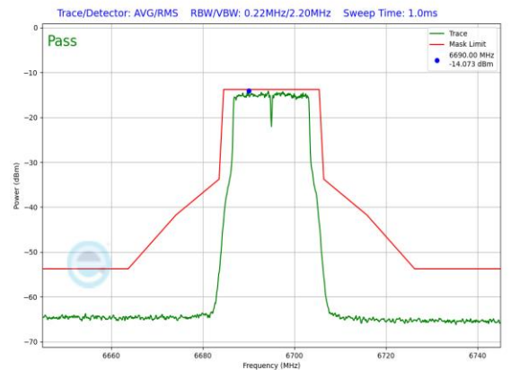
Plot 7-859. LPI In-Band Emission Plot Antenna 3b (20MHz 802.11a (UNII Band 7) – Ch. 149, 24Mbps)
