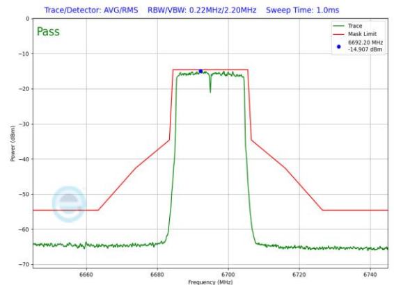
Plot 7-930. LPI In-Band Emission Plot Antenna 1b (20MHz 802.11ax (UNII Band 7) – Ch. 149, MCS2)
