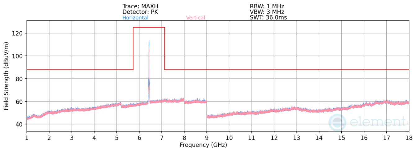
Plot 7-1288. Radiated Spurious Emission Antenna 1b (802.11ax – Ch.97)
