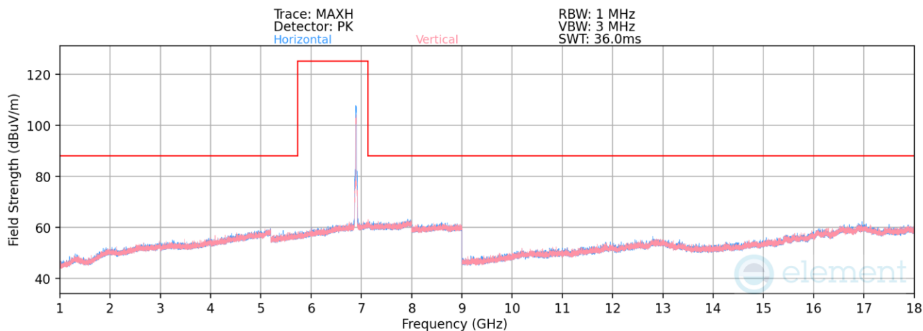
Plot 7-1294. Radiated Spurious Emission Antenna 1b (802.11ax – Ch.189)
