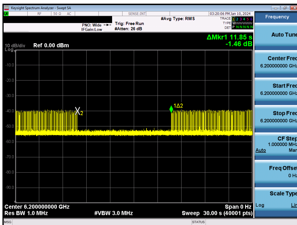
Plot 7-1242. Contention Based Protocol Timing Plot – UNII 5 – 160MHz Channel 47 – Low
