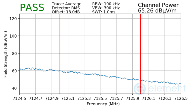
Plot 7-1340 Antenna 5T Radiated Upper Band Edge (Average – UNII Band 8)
