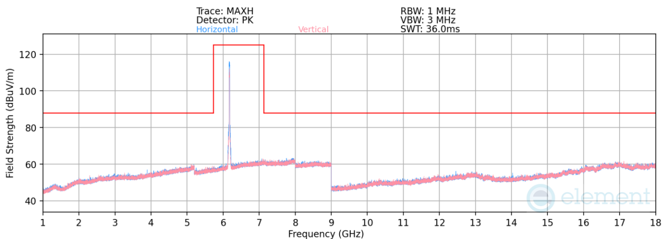
Plot 7-1315. Radiated Spurious Emission SDM Diversity (802.11ax – Ch.45)
