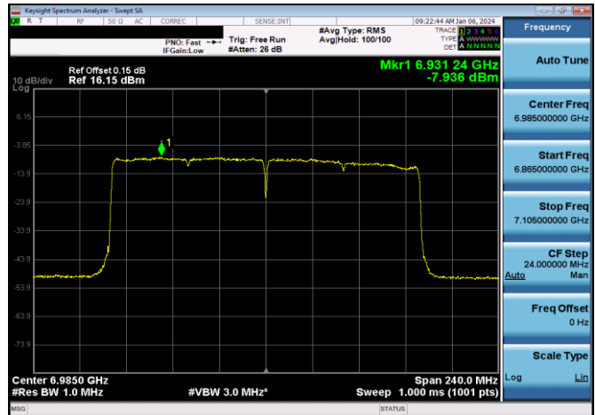
Plot 7-200. Power Spectral Density Plot Antenna 5T LPI (160MHz 802.11ax (UNII Band 8) – Ch. 207, MCS2)
