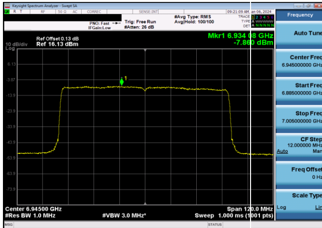
Plot 7-199. Power Spectral Density Plot Antenna 5T LPI (80MHz 802.11ax (UNII Band 8) – Ch. 199, MCS2)
